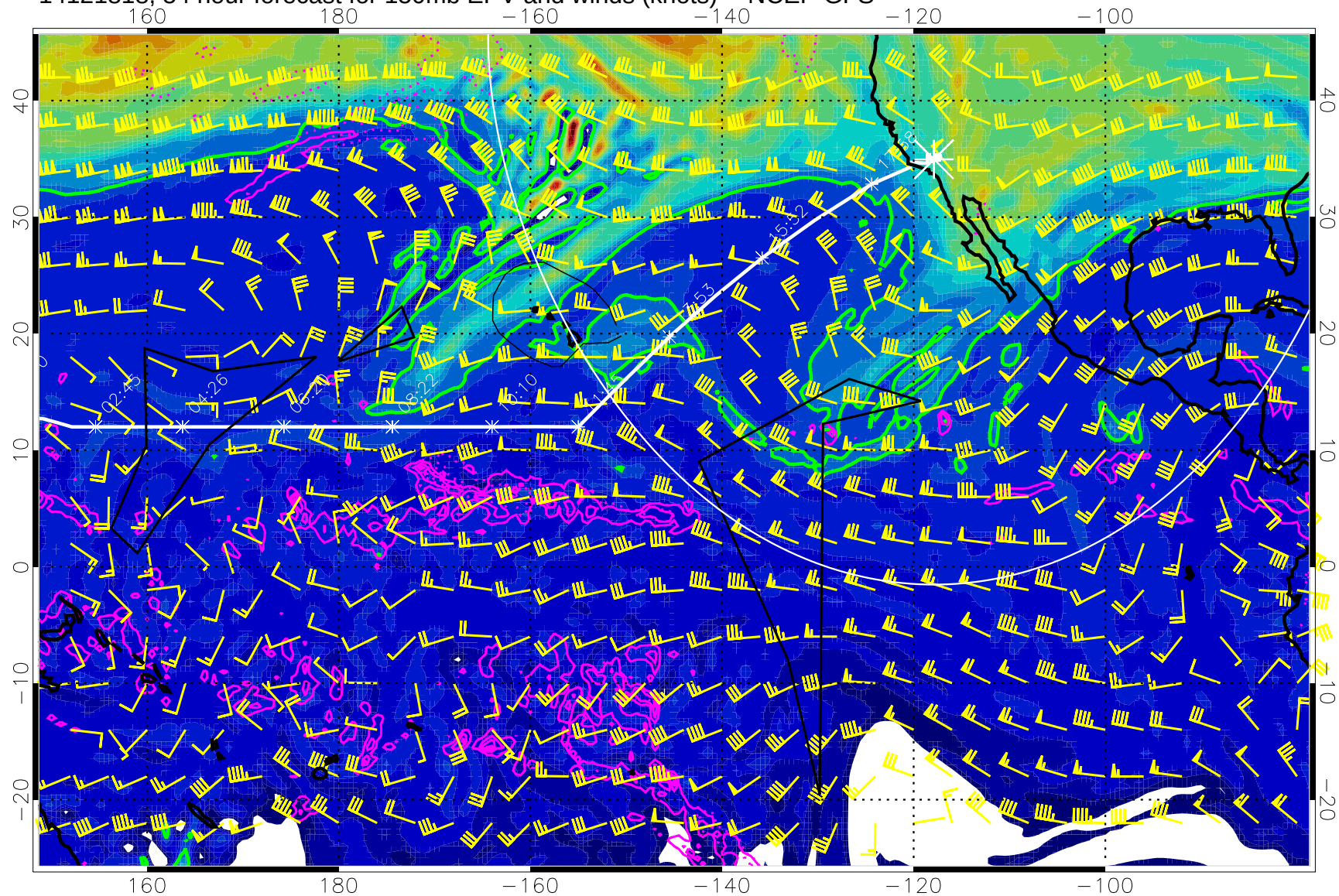
14121818, 54 hour forecast for 150mb EPV and winds (knots) -- NCEP GFS
