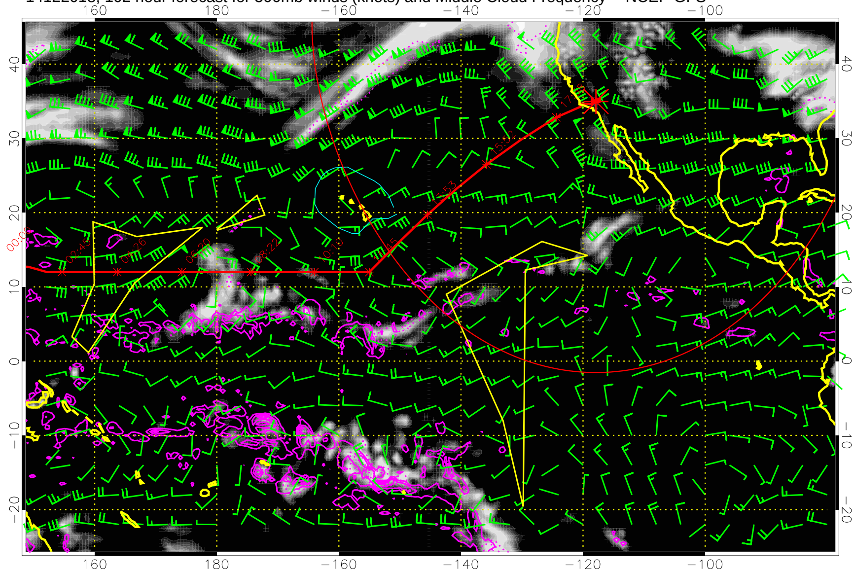
14122018, 102 hour forecast for 500mb winds (knots) and Middle Cloud Frequency -- NCEP GFS
