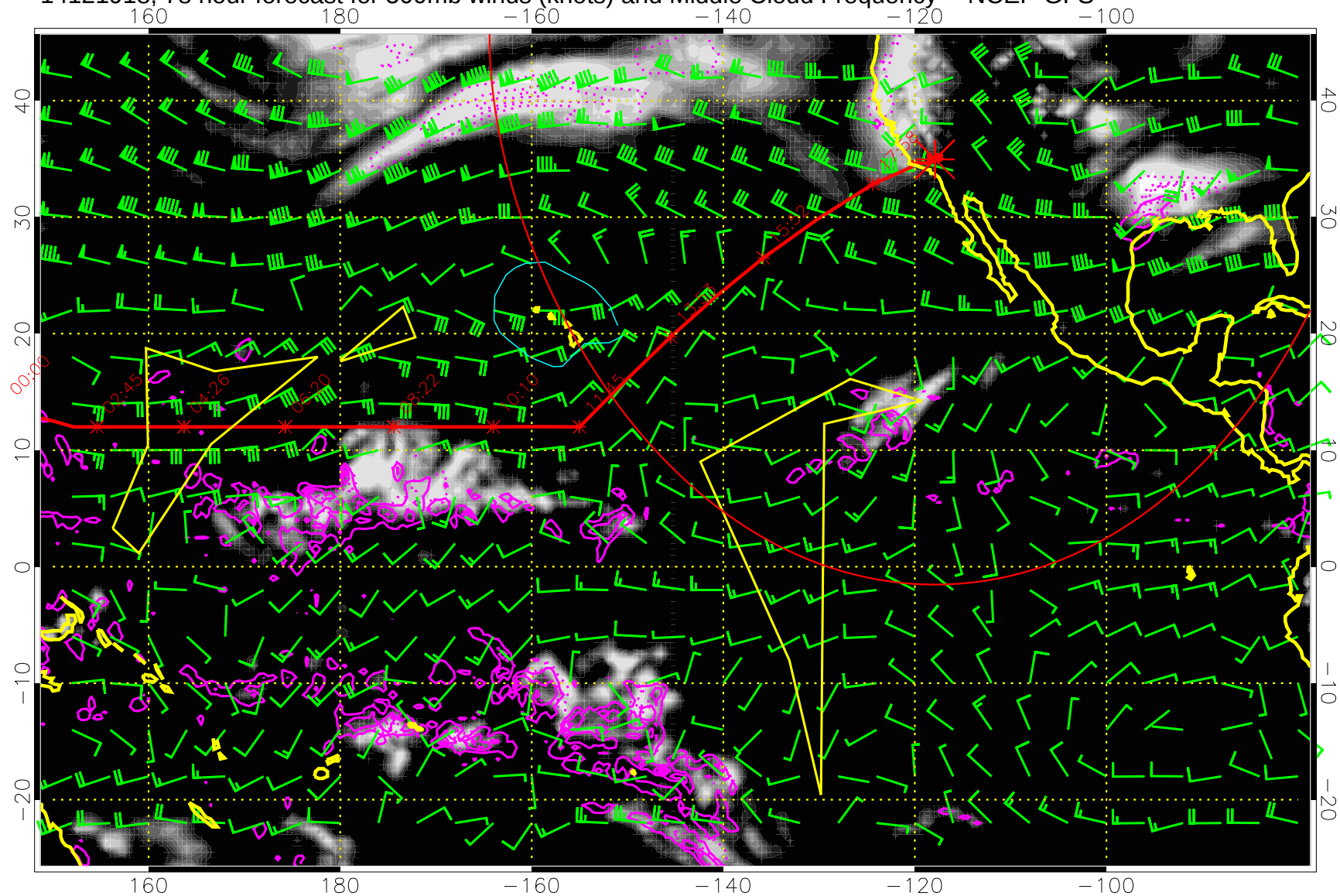
14121918, 78 hour forecast for 500mb winds (knots) and Middle Cloud Frequency -- NCEP GFS
