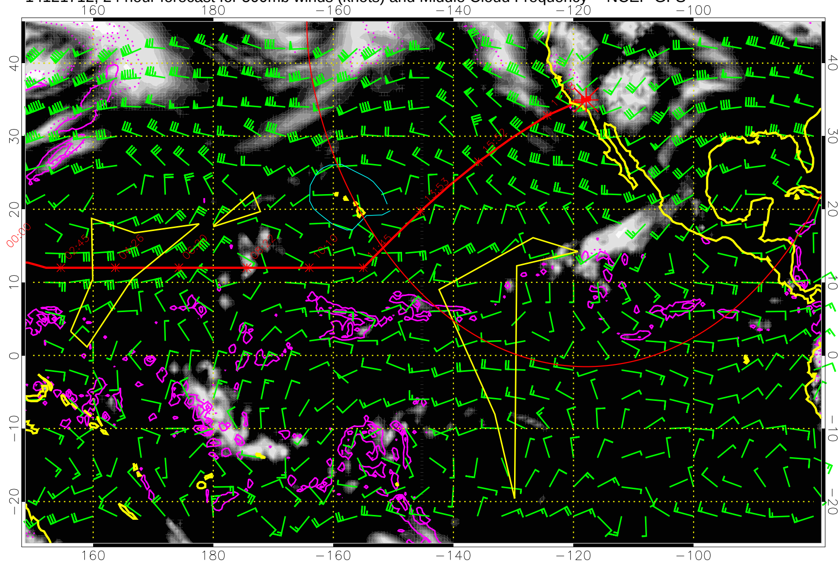
14121712, 24 hour forecast for 500mb winds (knots) and Middle Cloud Frequency -- NCEP GFS
