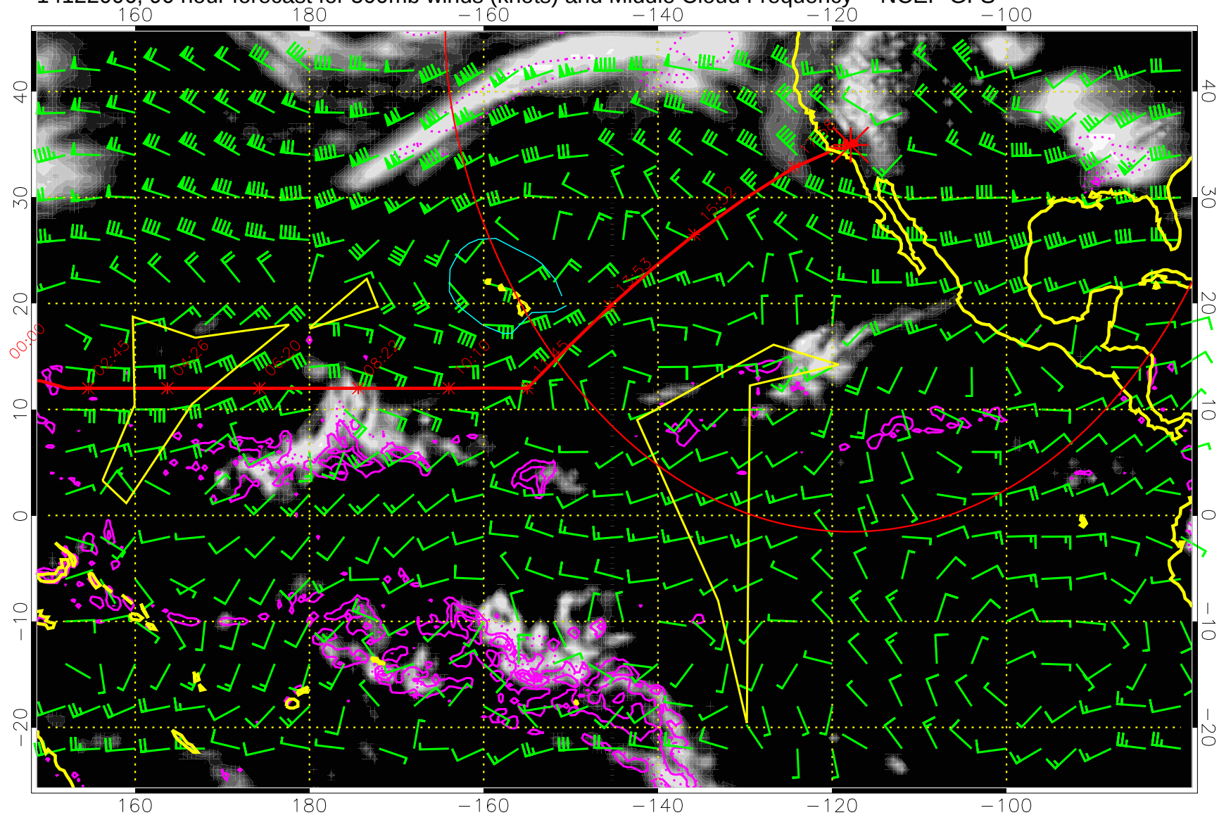
14122006, 90 hour forecast for 500mb winds (knots) and Middle Cloud Frequency -- NCEP GFS
