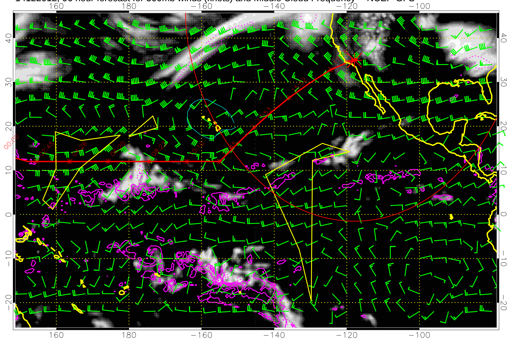
14122012, 96 hour forecast for 500mb winds (knots) and Middle Cloud Frequency -- NCEP GFS
