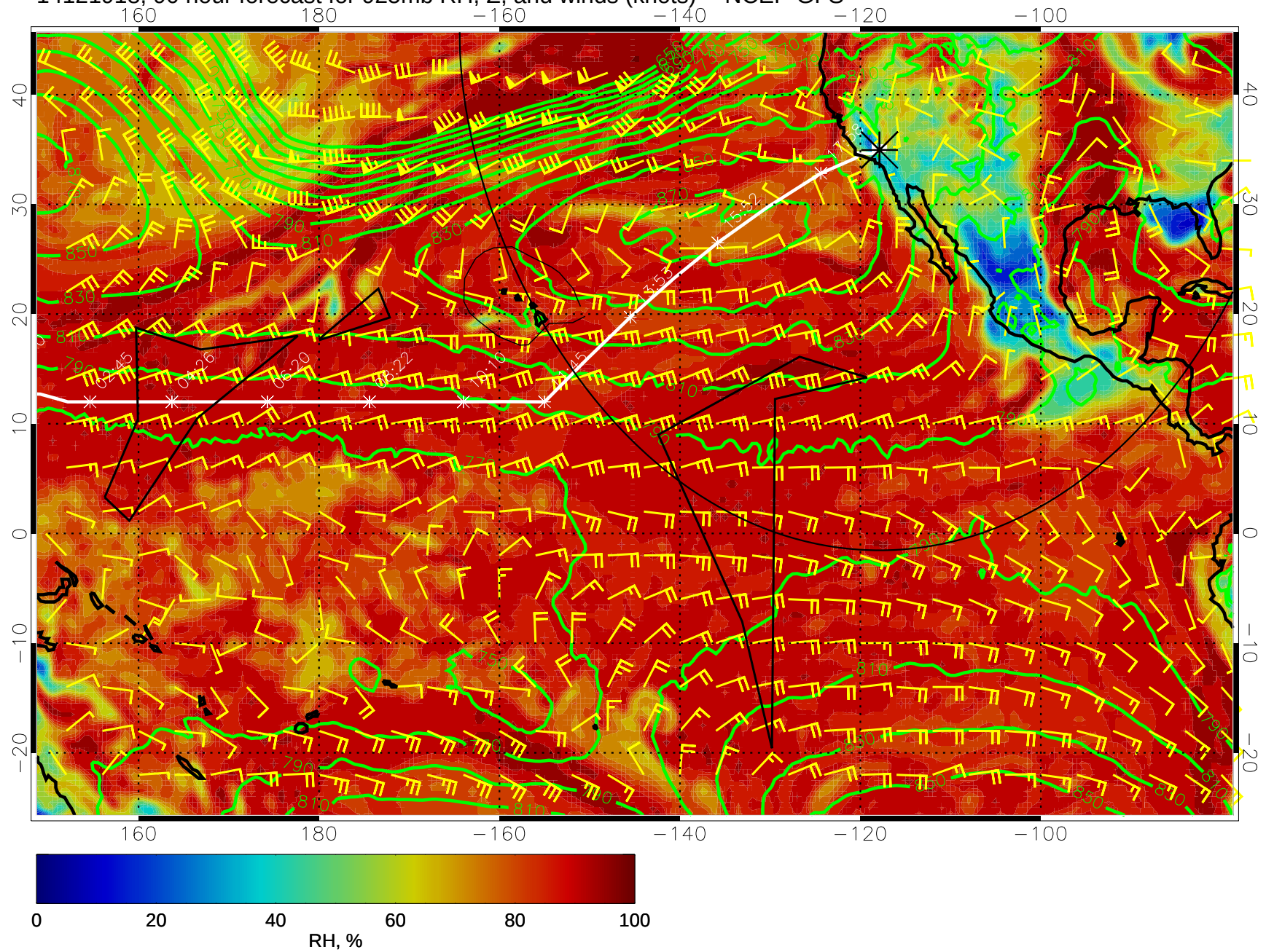
14121918, 90 hour forecast for 925mb RH, Z, and winds (knots) -- NCEP GFS
