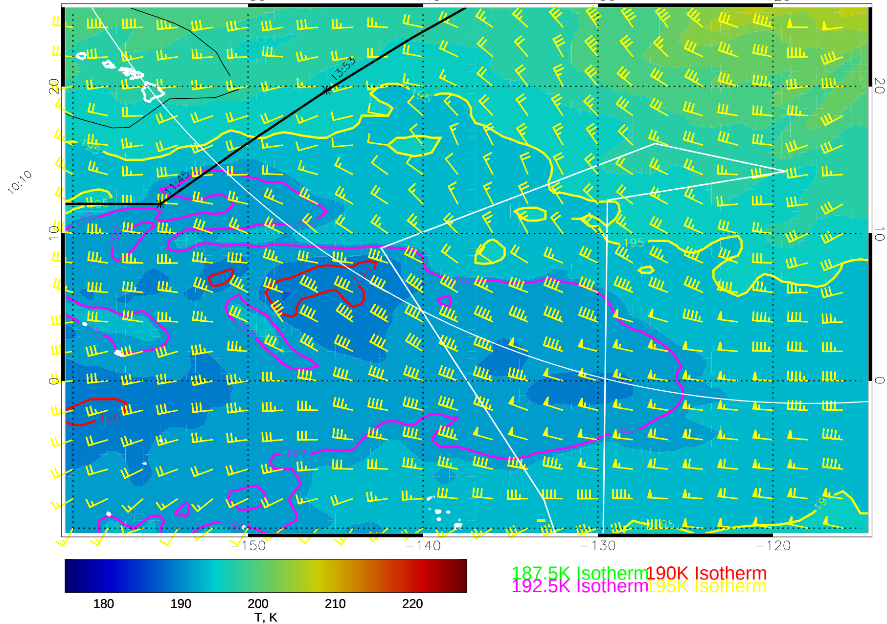
14121812, 60 hour forecast for 100mb T and winds (knots) -- NCEP GFS
