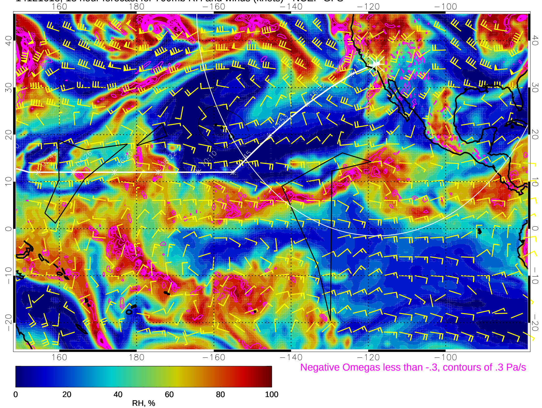
14121618, 18 hour forecast for 700mb RH and winds (knots) - NCEP GFS
