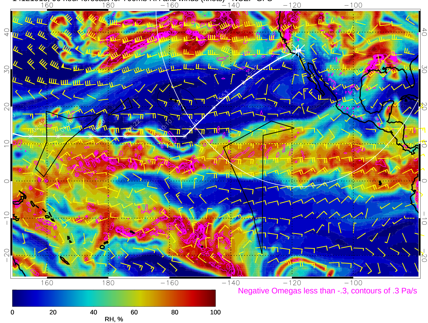
14121918, 90 hour forecast for 700mb RH and winds (knots) - NCEP GFS
