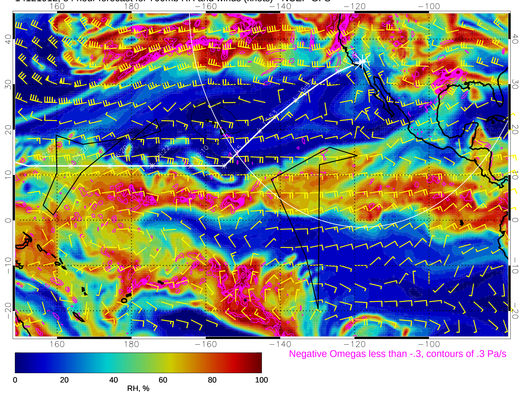
14121912, 84 hour forecast for 700mb RH and winds (knots) - NCEP GFS
