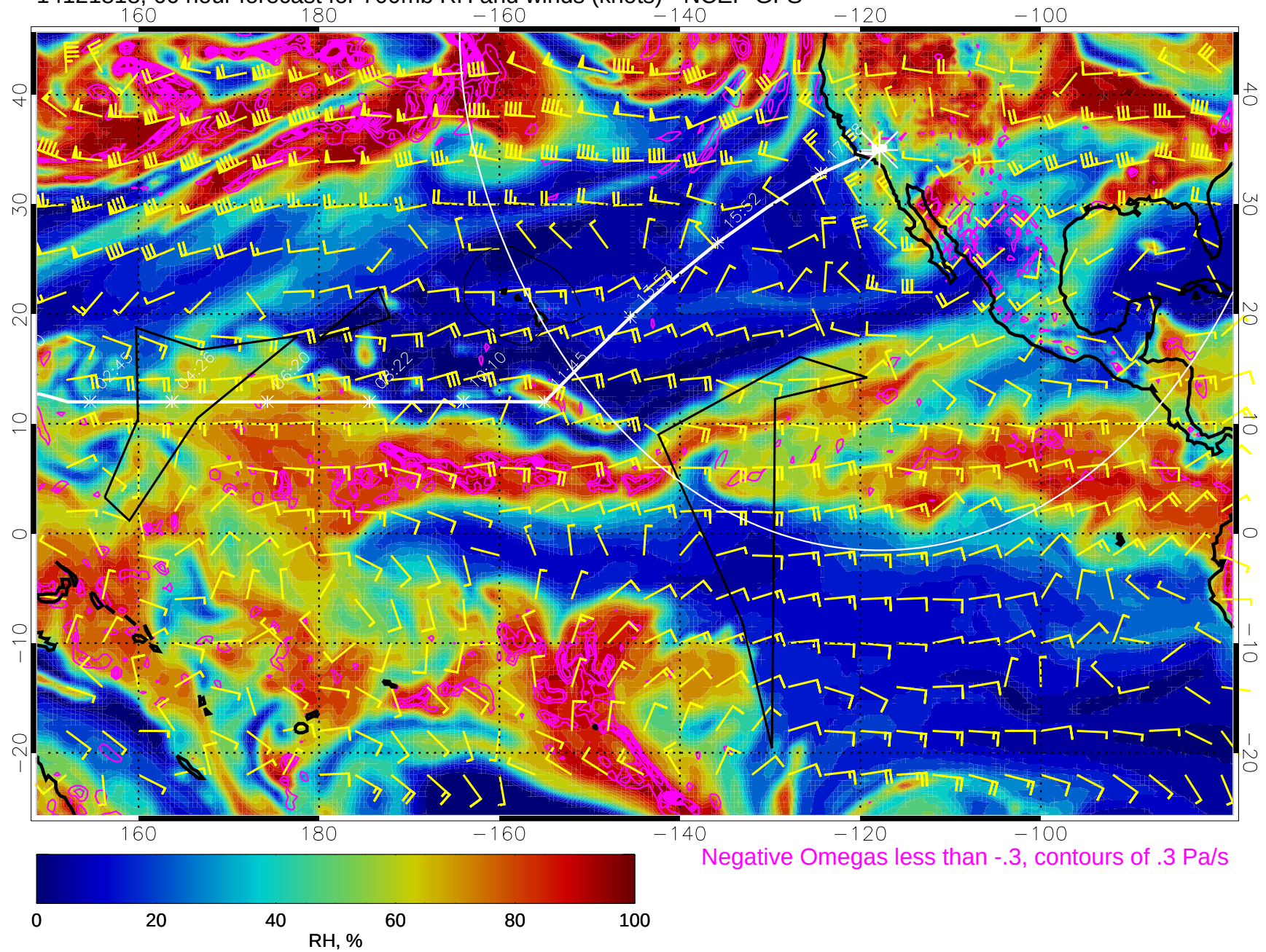
14121818, 66 hour forecast for 700mb RH and winds (knots) - NCEP GFS
