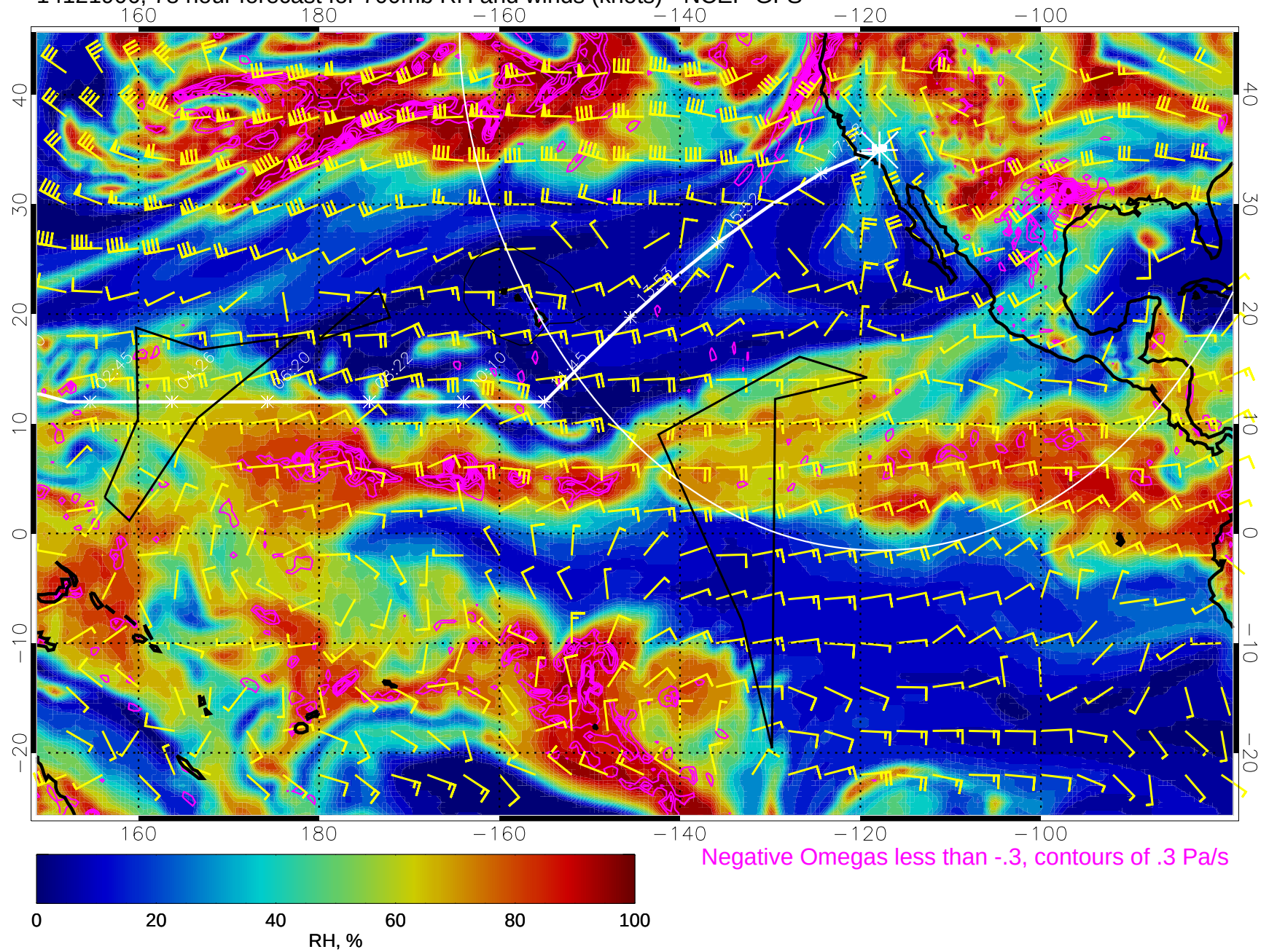
14121906, 78 hour forecast for 700mb RH and winds (knots) - NCEP GFS
