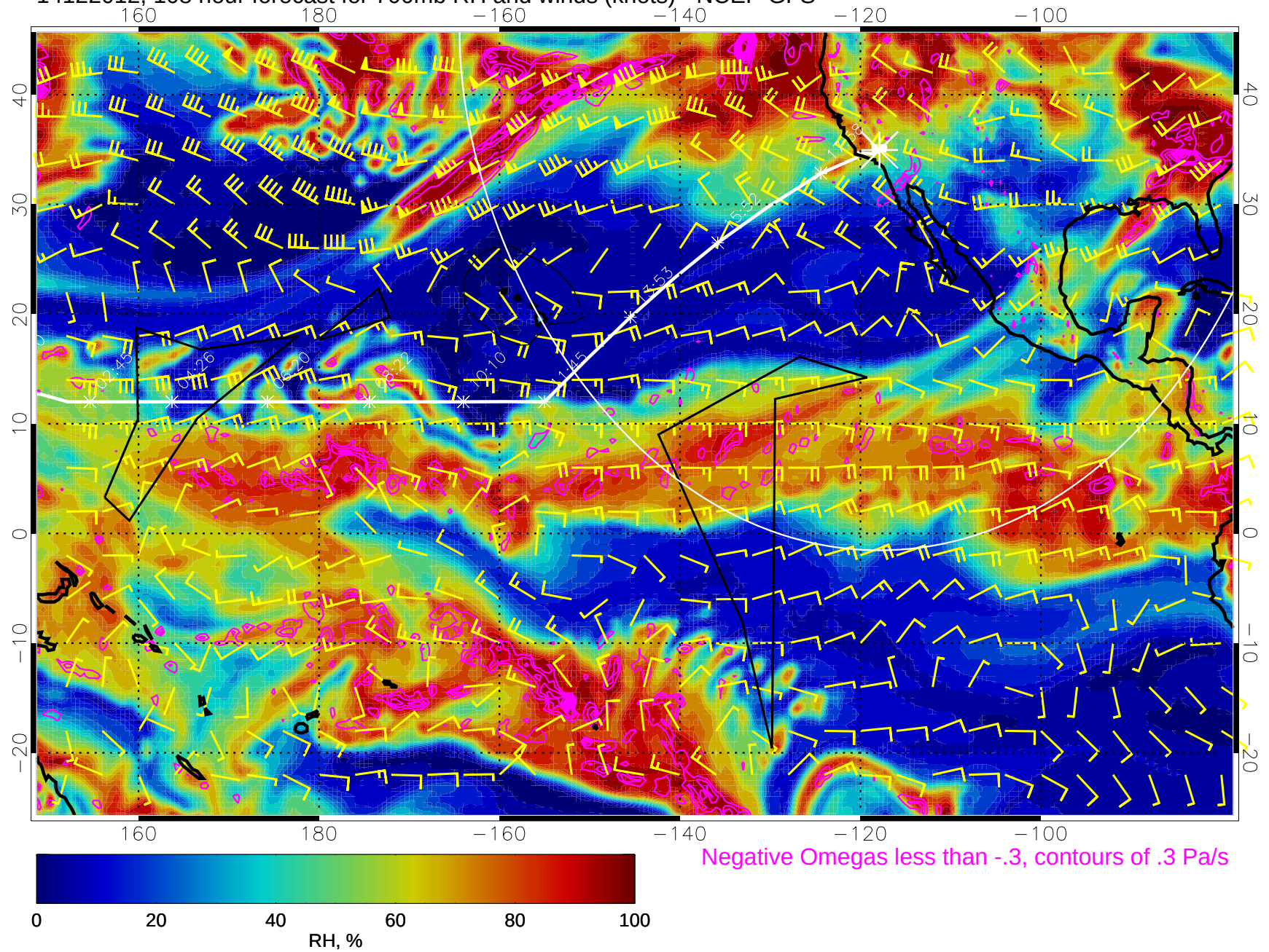
14122012, 108 hour forecast for 700mb RH and winds (knots) - NCEP GFS
