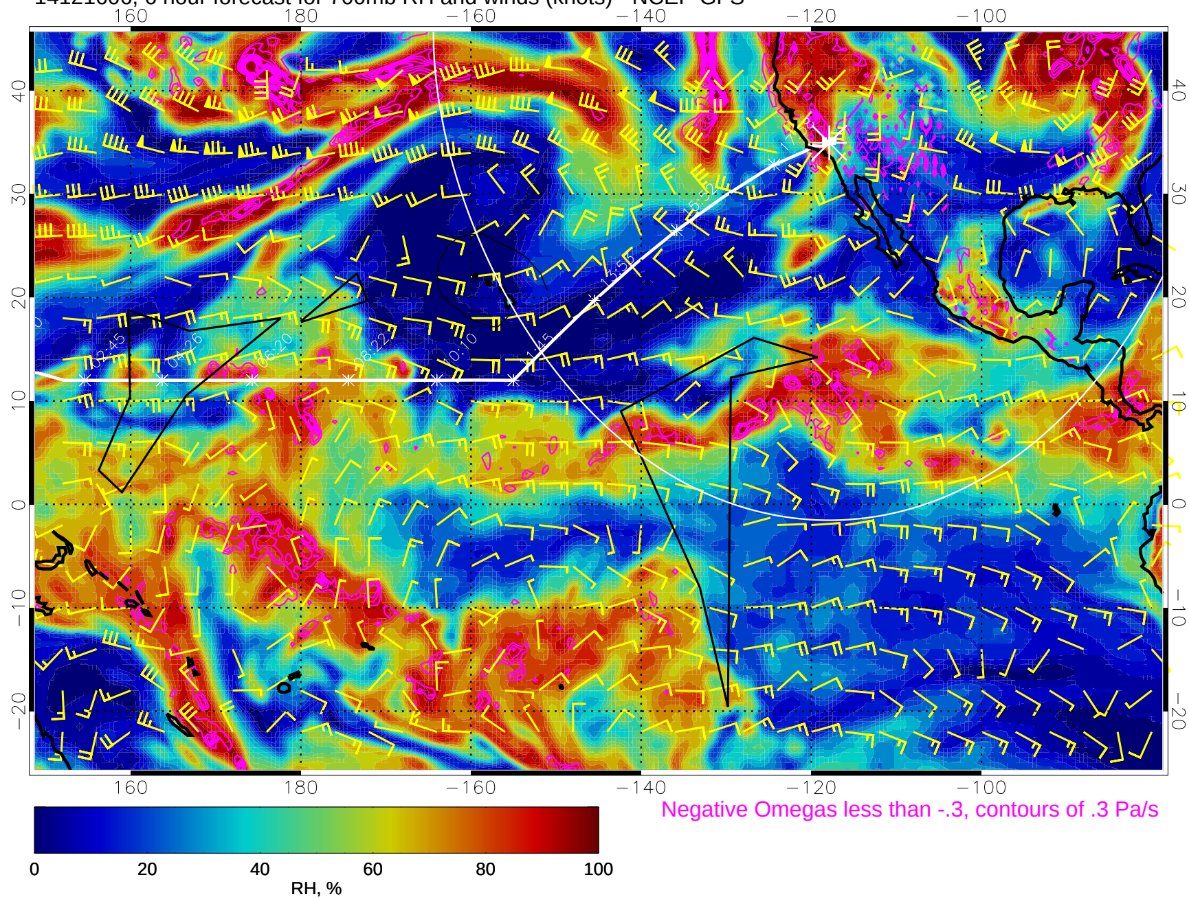
14121606, 6 hour forecast for 700mb RH and winds (knots) - NCEP GFS
