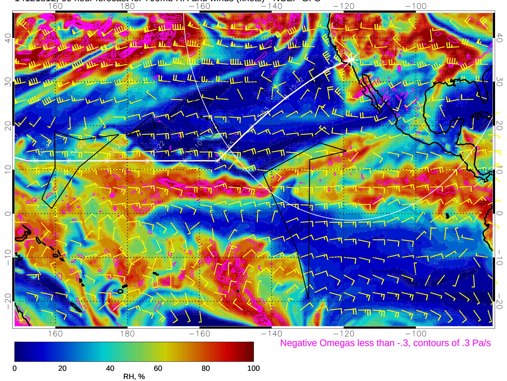
14121812, 60 hour forecast for 700mb RH and winds (knots) - NCEP GFS
