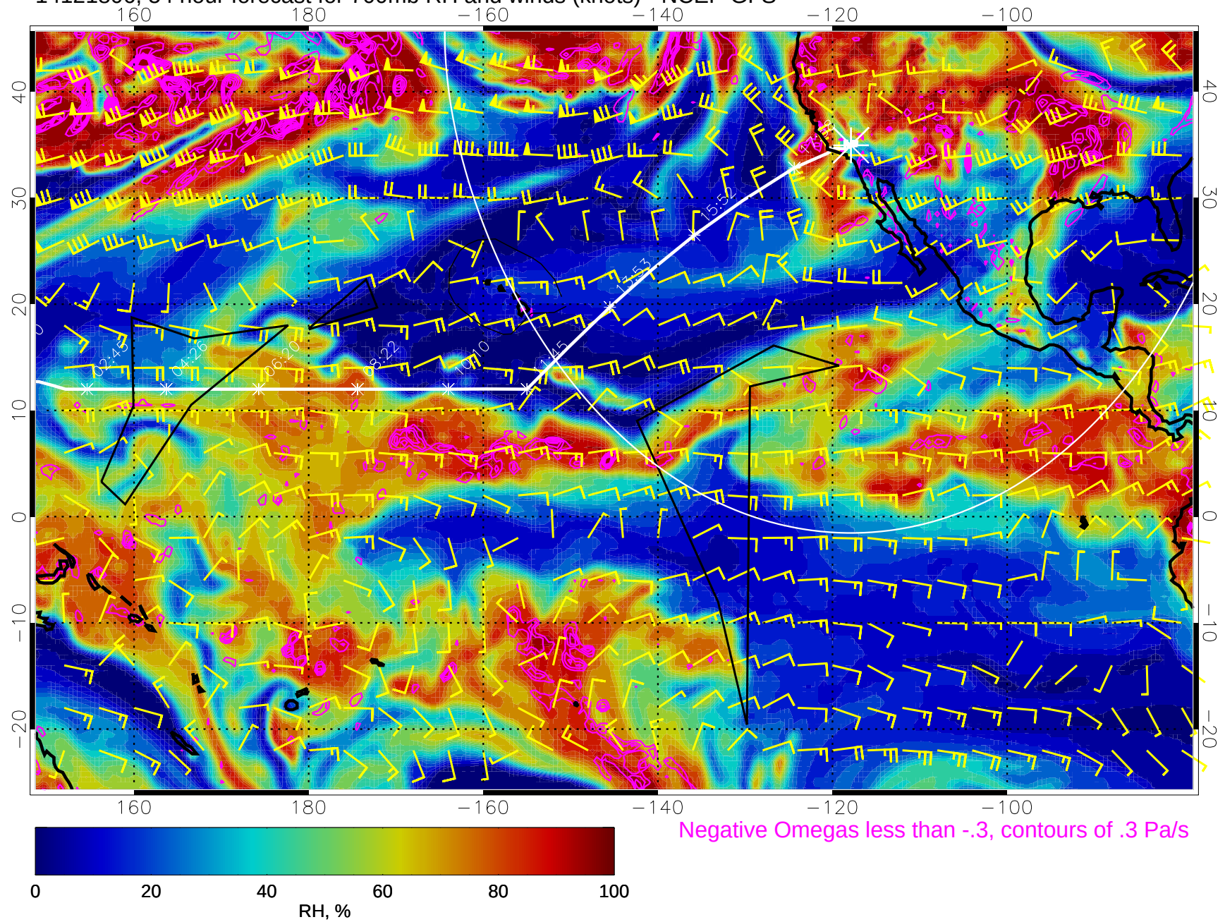
14121806, 54 hour forecast for 700mb RH and winds (knots) - NCEP GFS
