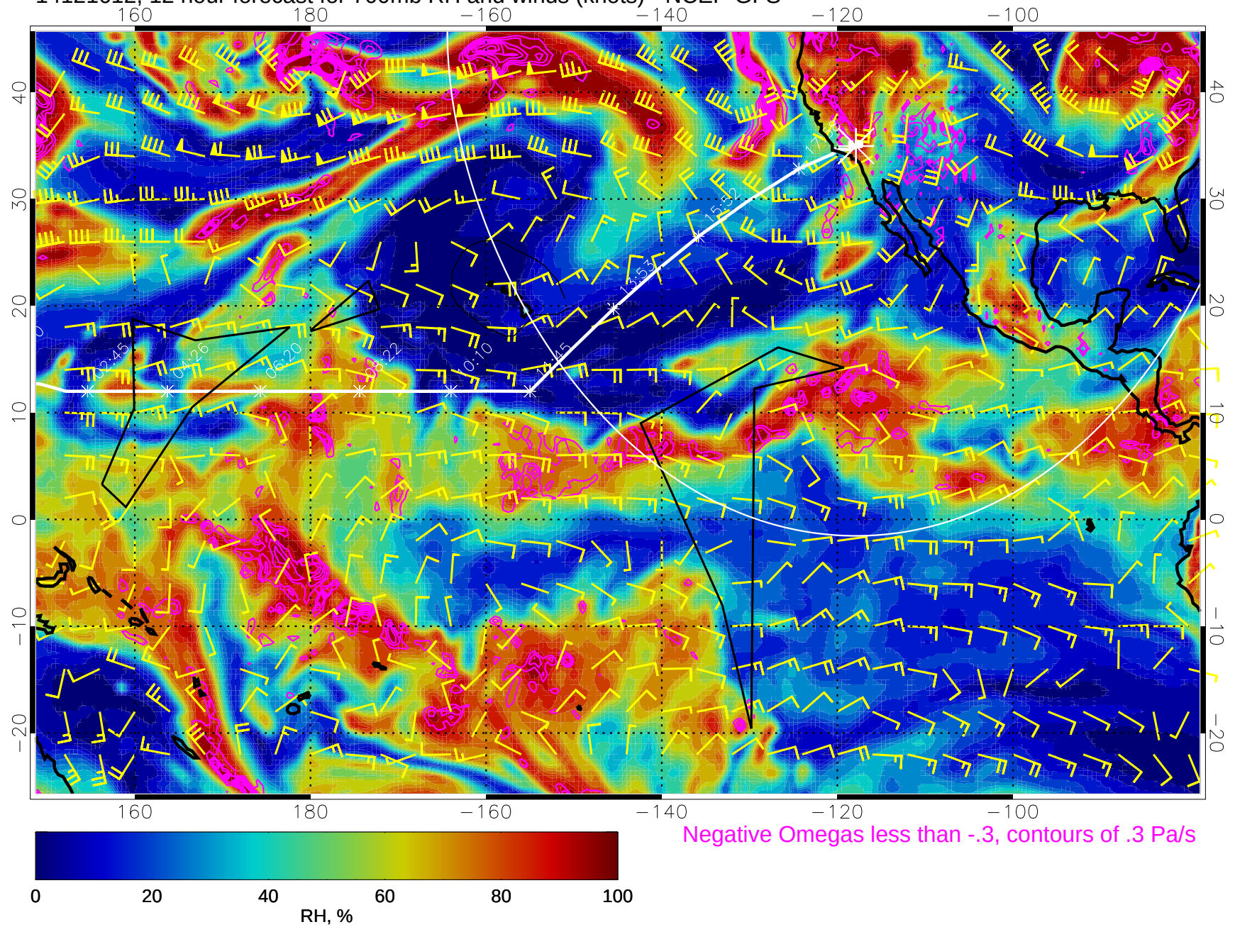
14121612, 12 hour forecast for 700mb RH and winds (knots) - NCEP GFS
