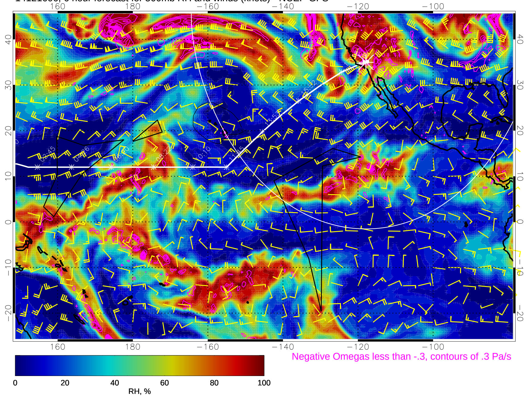
14121606, 6 hour forecast for 500mb RH and winds (knots) - NCEP GFS
