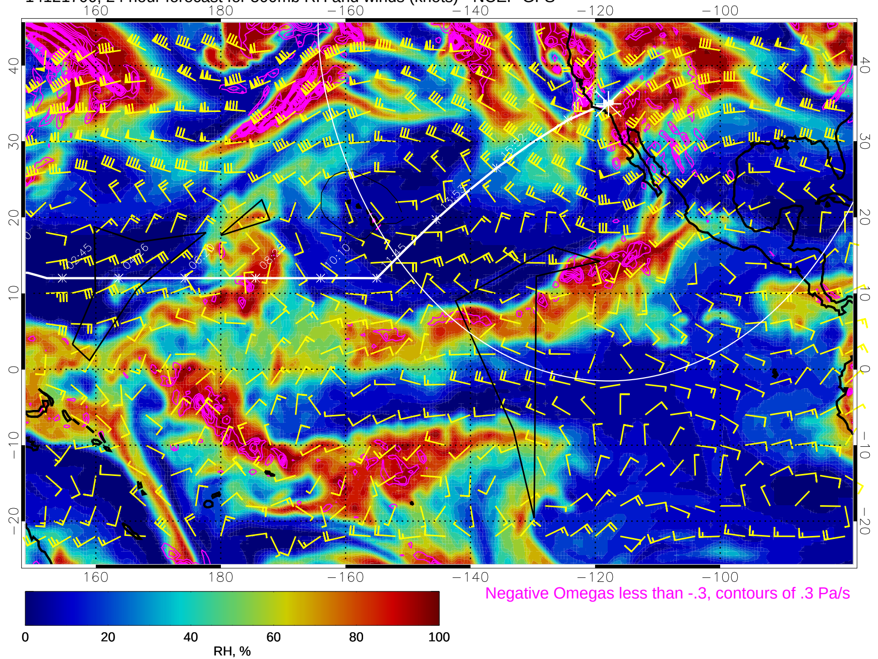
14121700, 24 hour forecast for 500mb RH and winds (knots) - NCEP GFS
