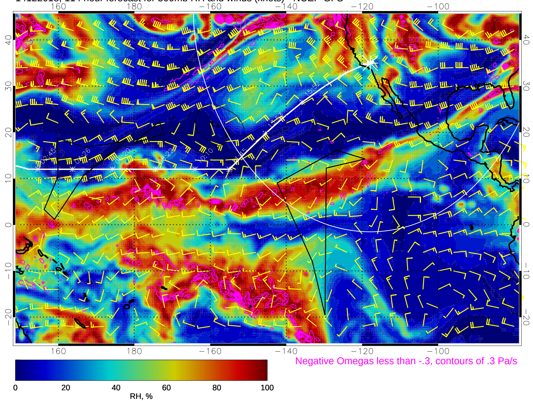
14122018, 114 hour forecast for 500mb RH and winds (knots) - NCEP GFS
