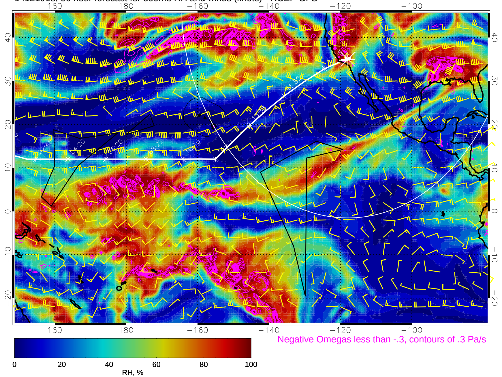
14121918, 90 hour forecast for 500mb RH and winds (knots) - NCEP GFS
