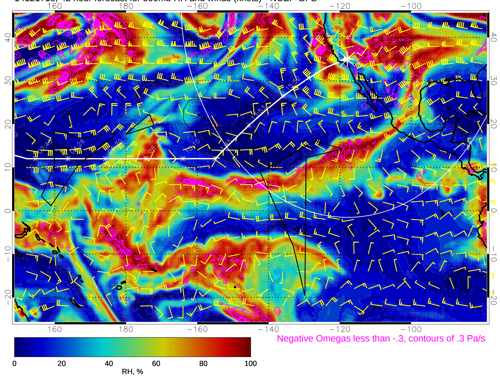
14121718, 42 hour forecast for 500mb RH and winds (knots) - NCEP GFS
