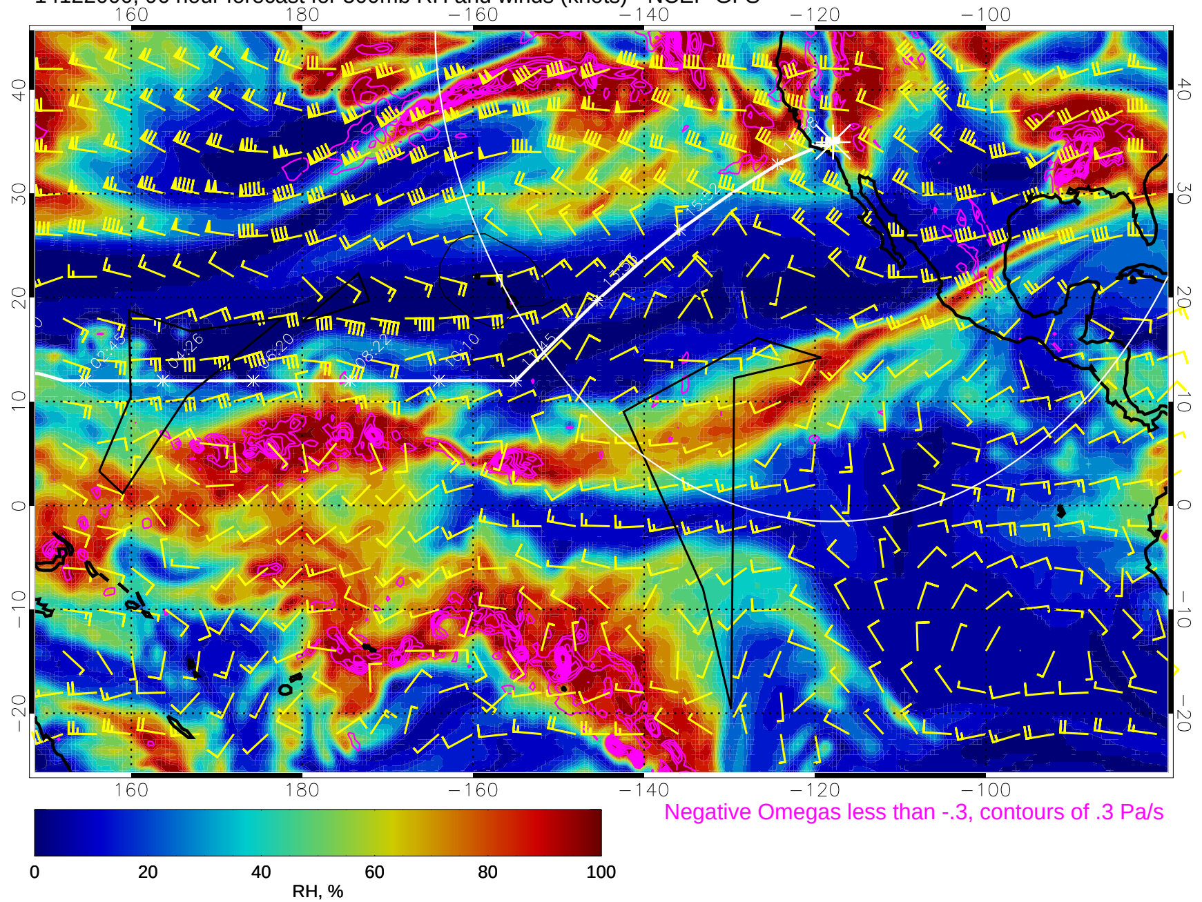
14122000, 96 hour forecast for 500mb RH and winds (knots) - NCEP GFS
