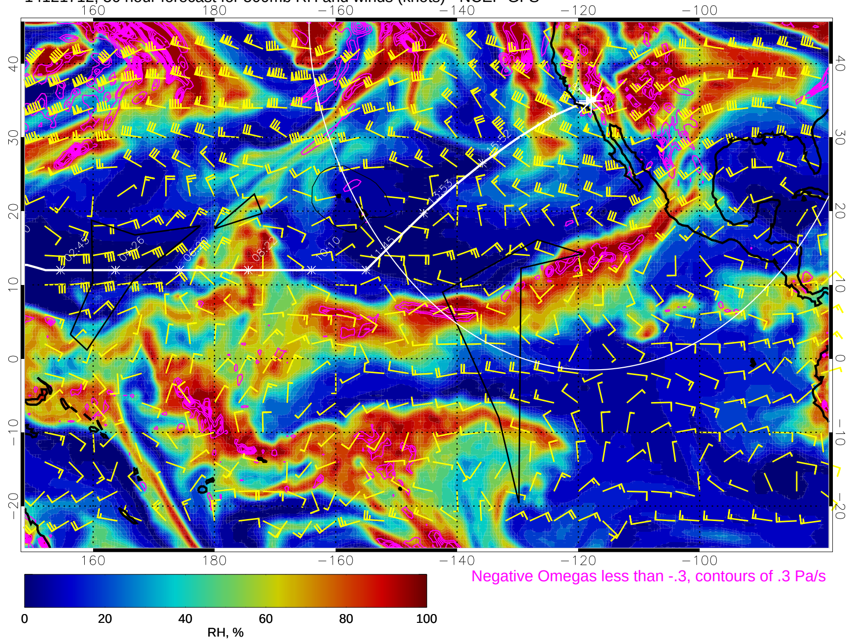
14121712, 36 hour forecast for 500mb RH and winds (knots) - NCEP GFS
