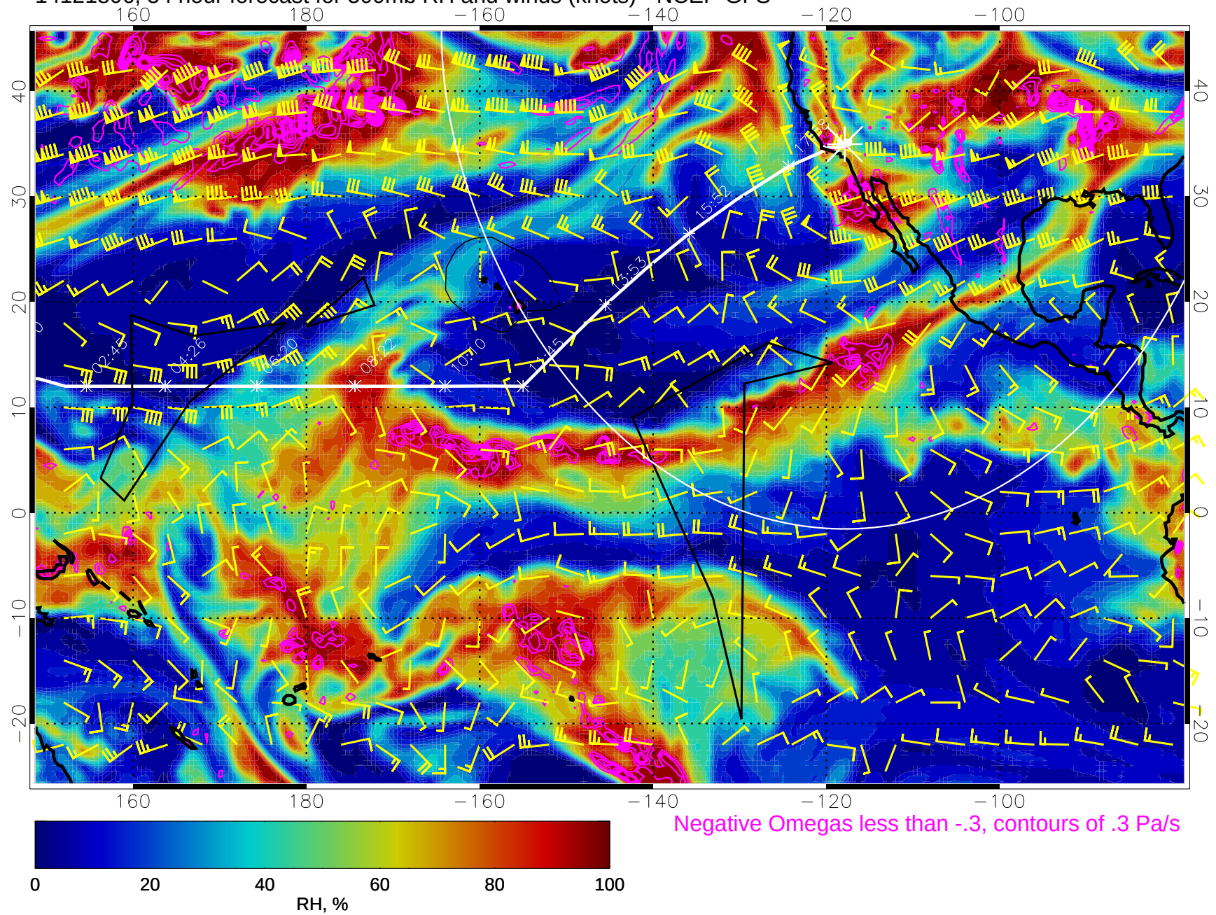
14121806, 54 hour forecast for 500mb RH and winds (knots) - NCEP GFS
