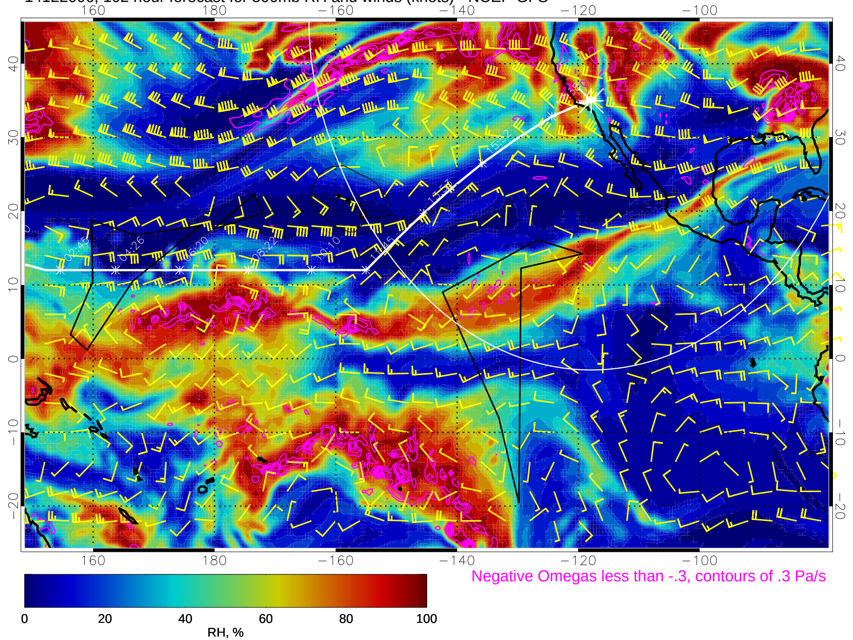
14122006, 102 hour forecast for 500mb RH and winds (knots) - NCEP GFS
