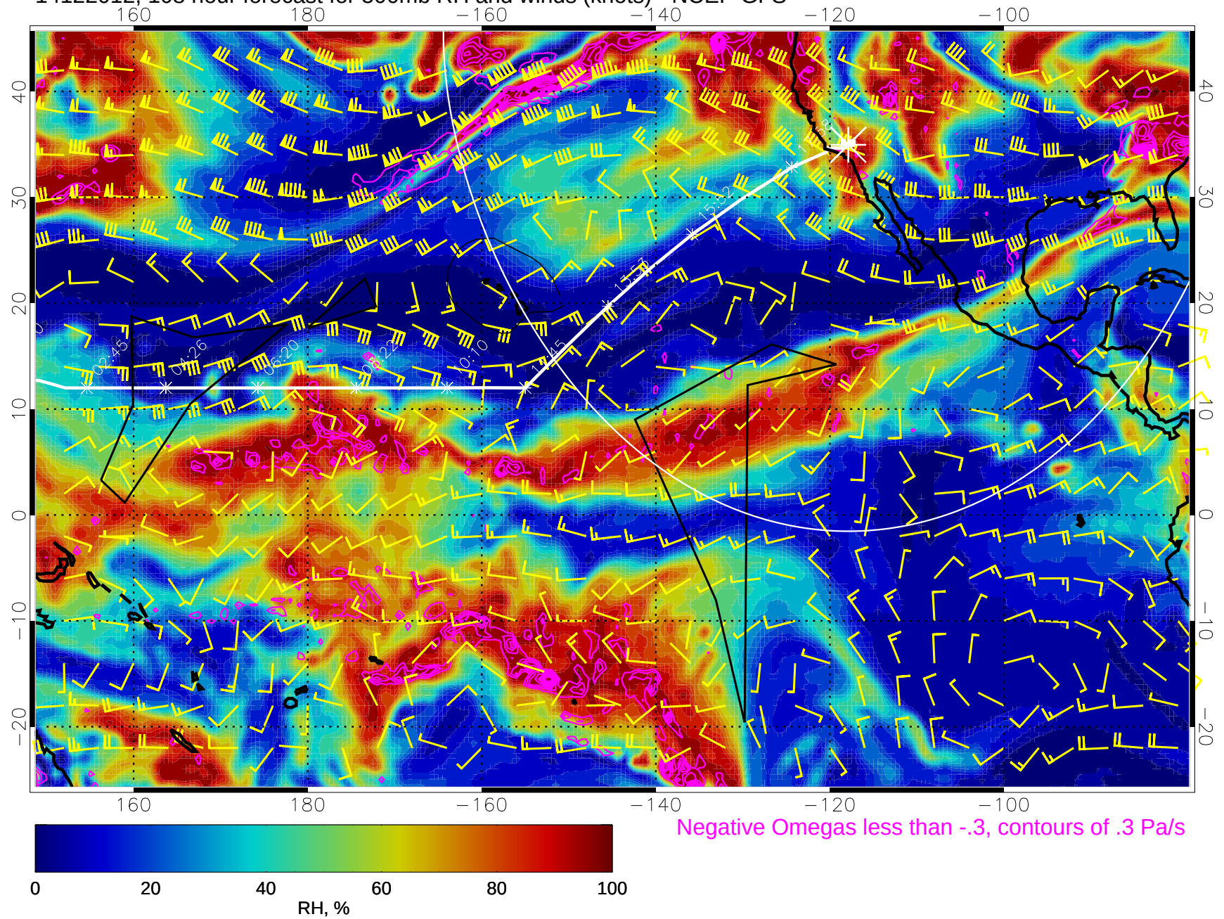
14122012, 108 hour forecast for 500mb RH and winds (knots) - NCEP GFS
