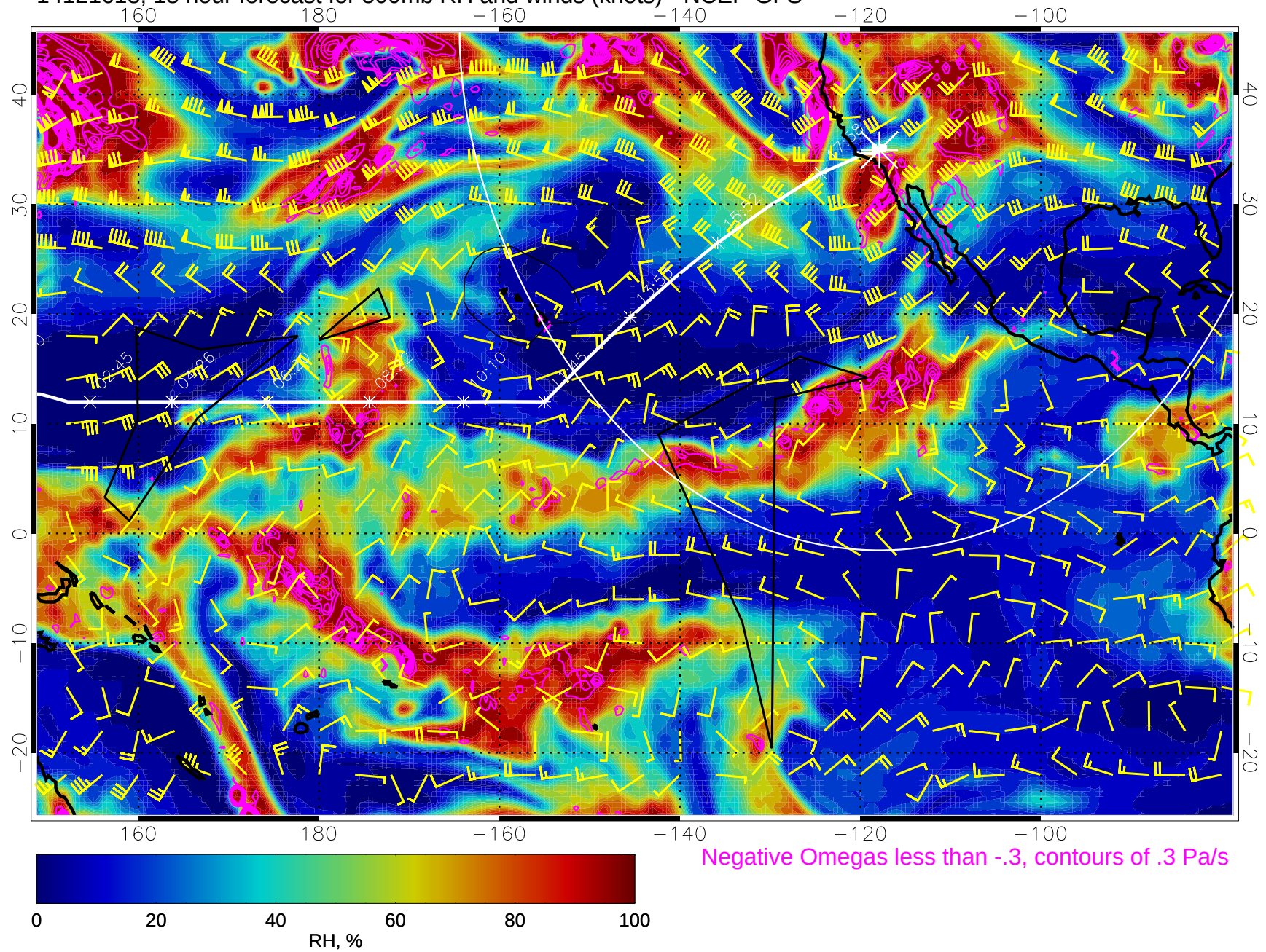
14121618, 18 hour forecast for 500mb RH and winds (knots) - NCEP GFS
