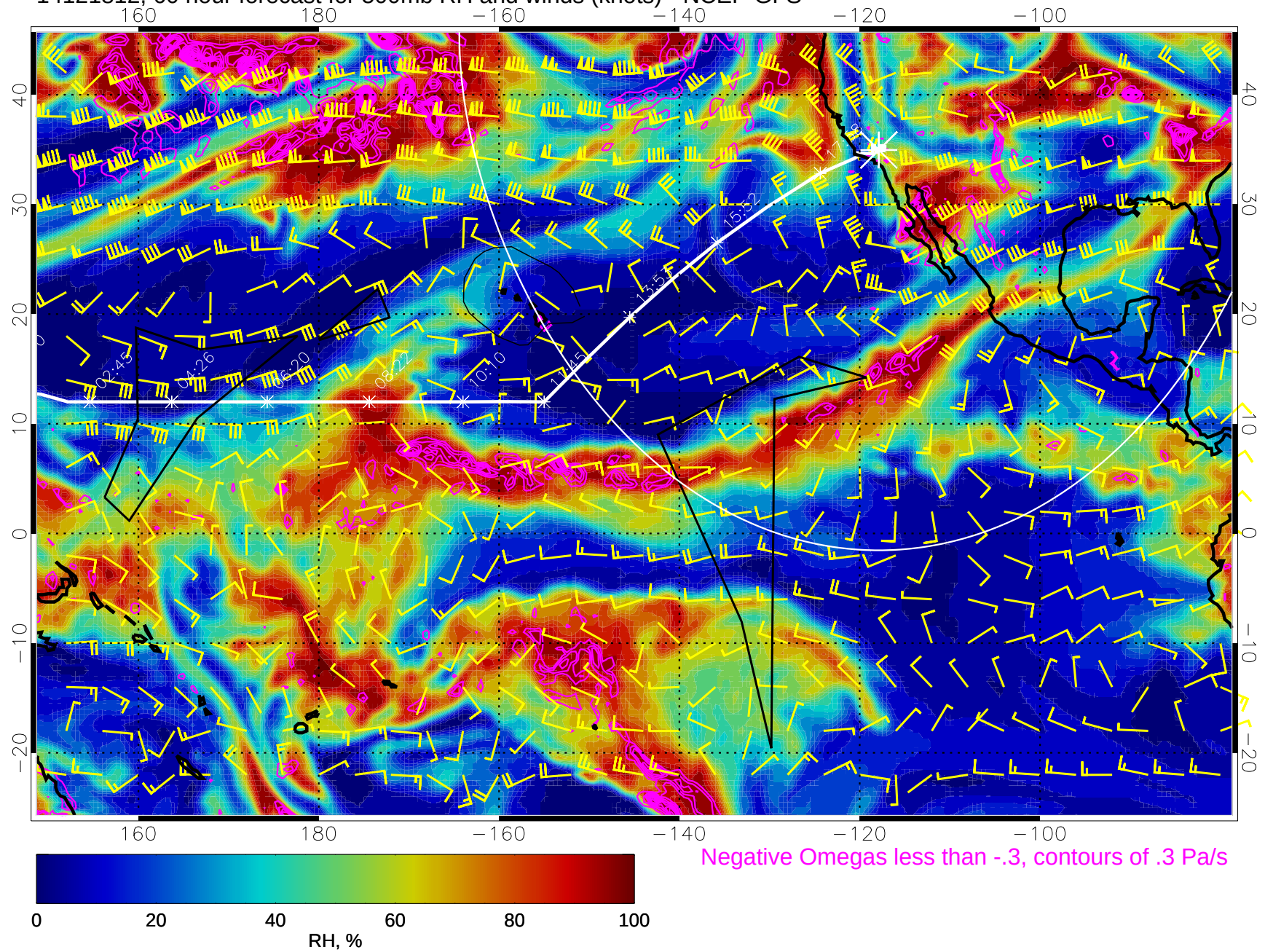
14121812, 60 hour forecast for 500mb RH and winds (knots) - NCEP GFS
