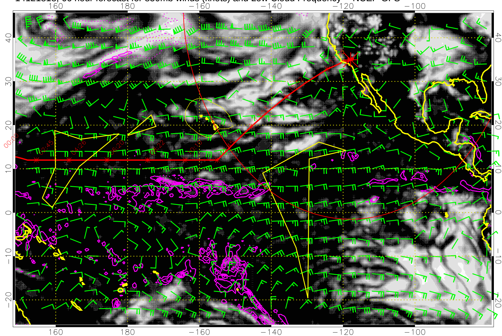
14121818, 66 hour forecast for 850mb winds (knots) and Low Cloud Frequency -- NCEP GFS
