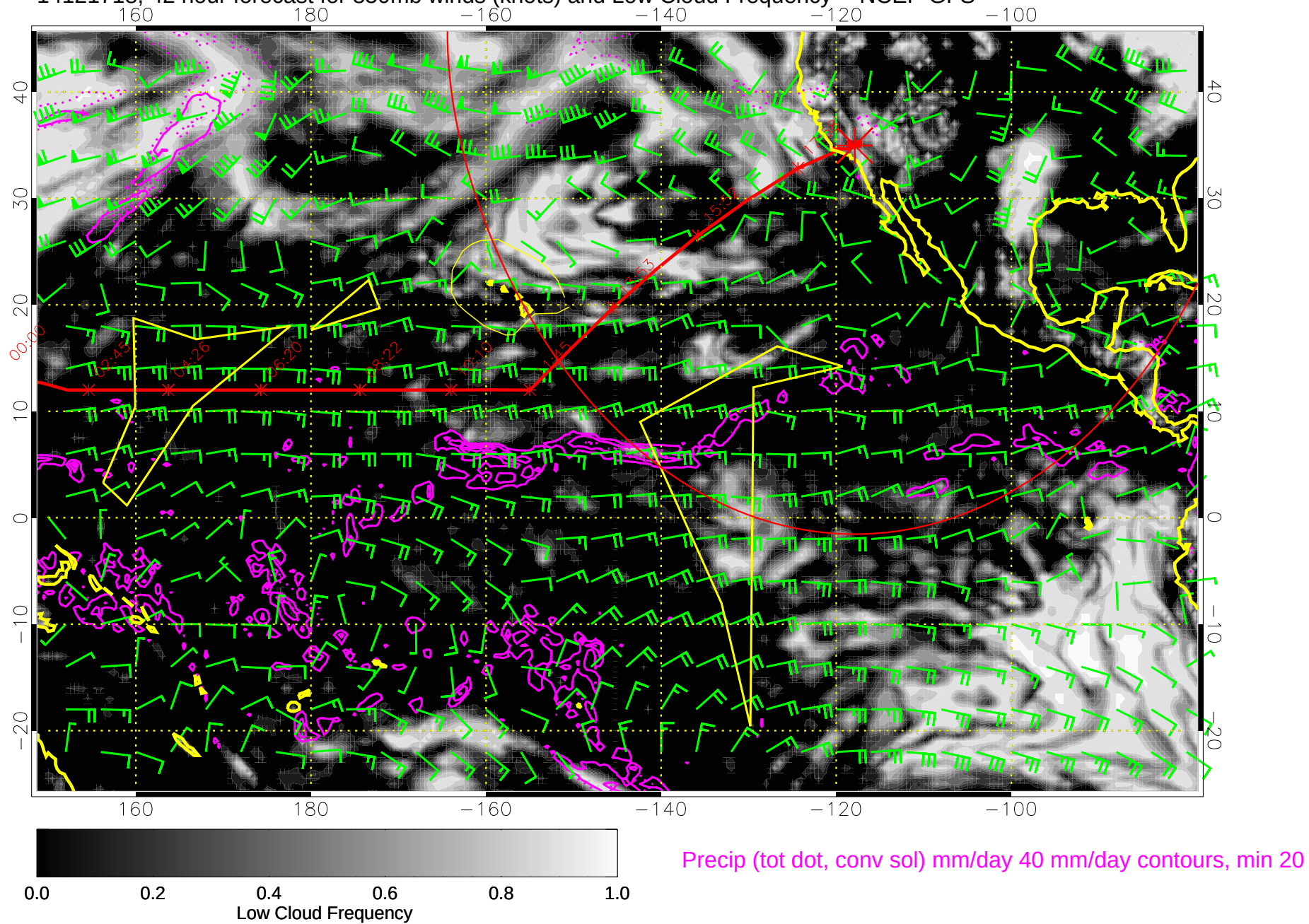
14121718, 42 hour forecast for 850mb winds (knots) and Low Cloud Frequency -- NCEP GFS
