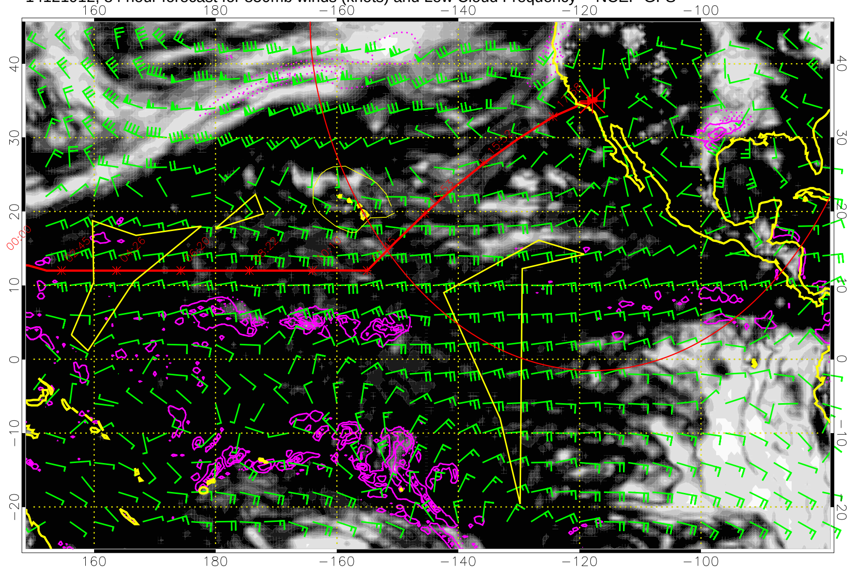
14121912, 84 hour forecast for 850mb winds (knots) and Low Cloud Frequency -- NCEP GFS
