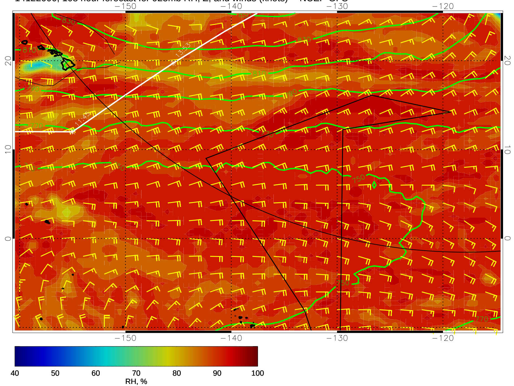
14122000, 108 hour forecast for 925mb RH, Z, and winds (knots) -- NCEP GFS
