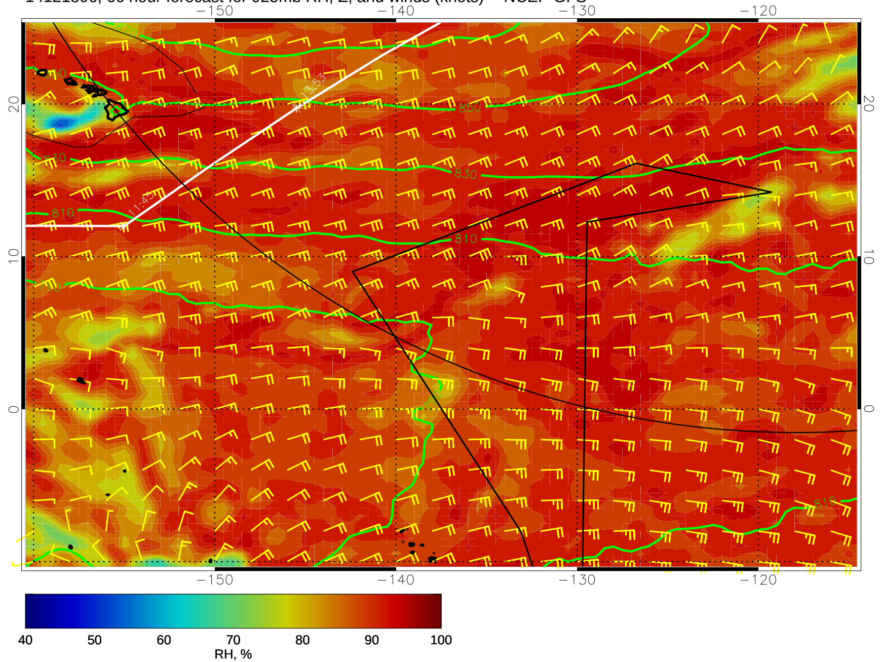
14121806, 66 hour forecast for 925mb RH, Z, and winds (knots) -- NCEP GFS
