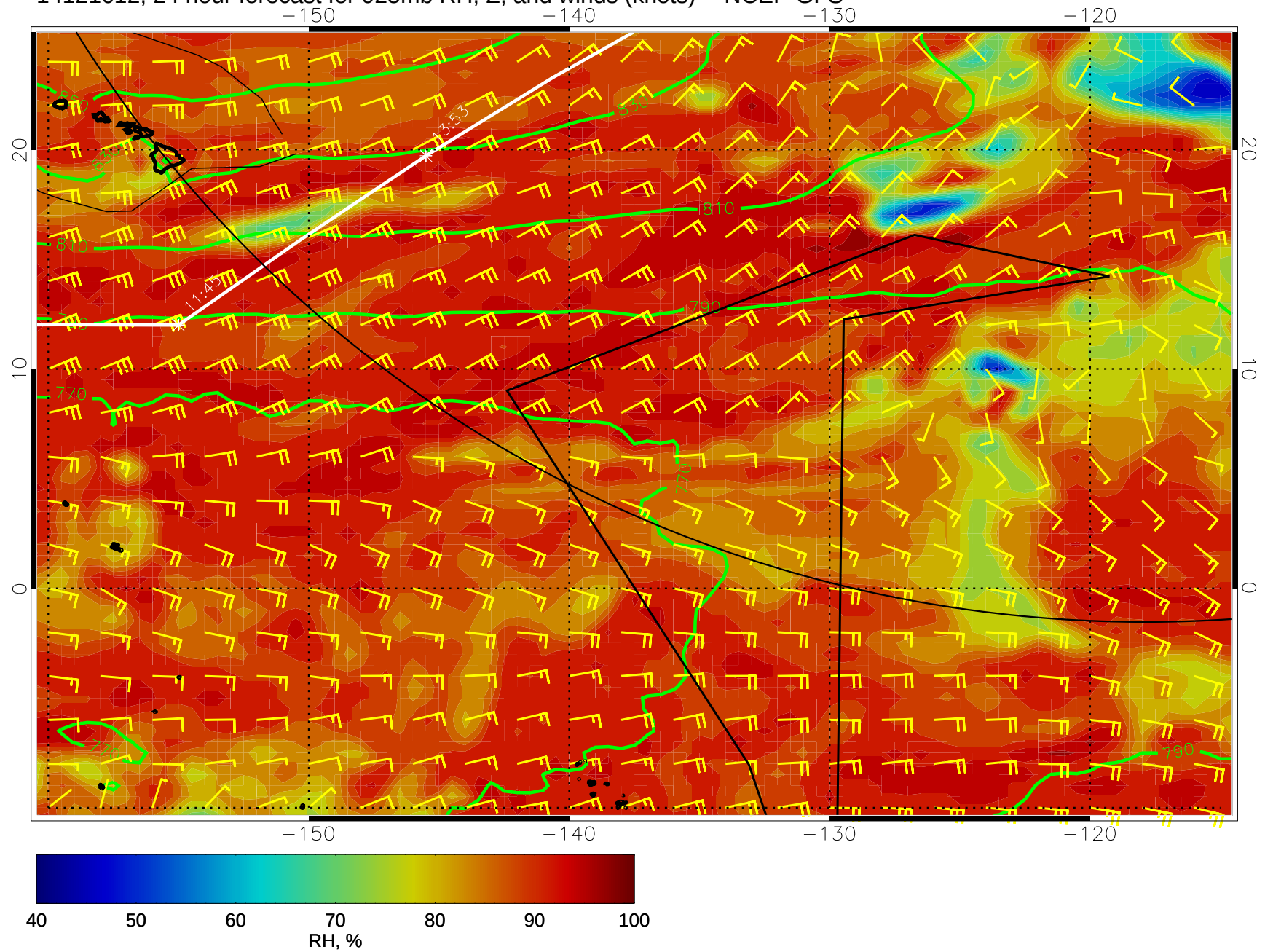
14121612, 24 hour forecast for 925mb RH, Z, and winds (knots) -- NCEP GFS
