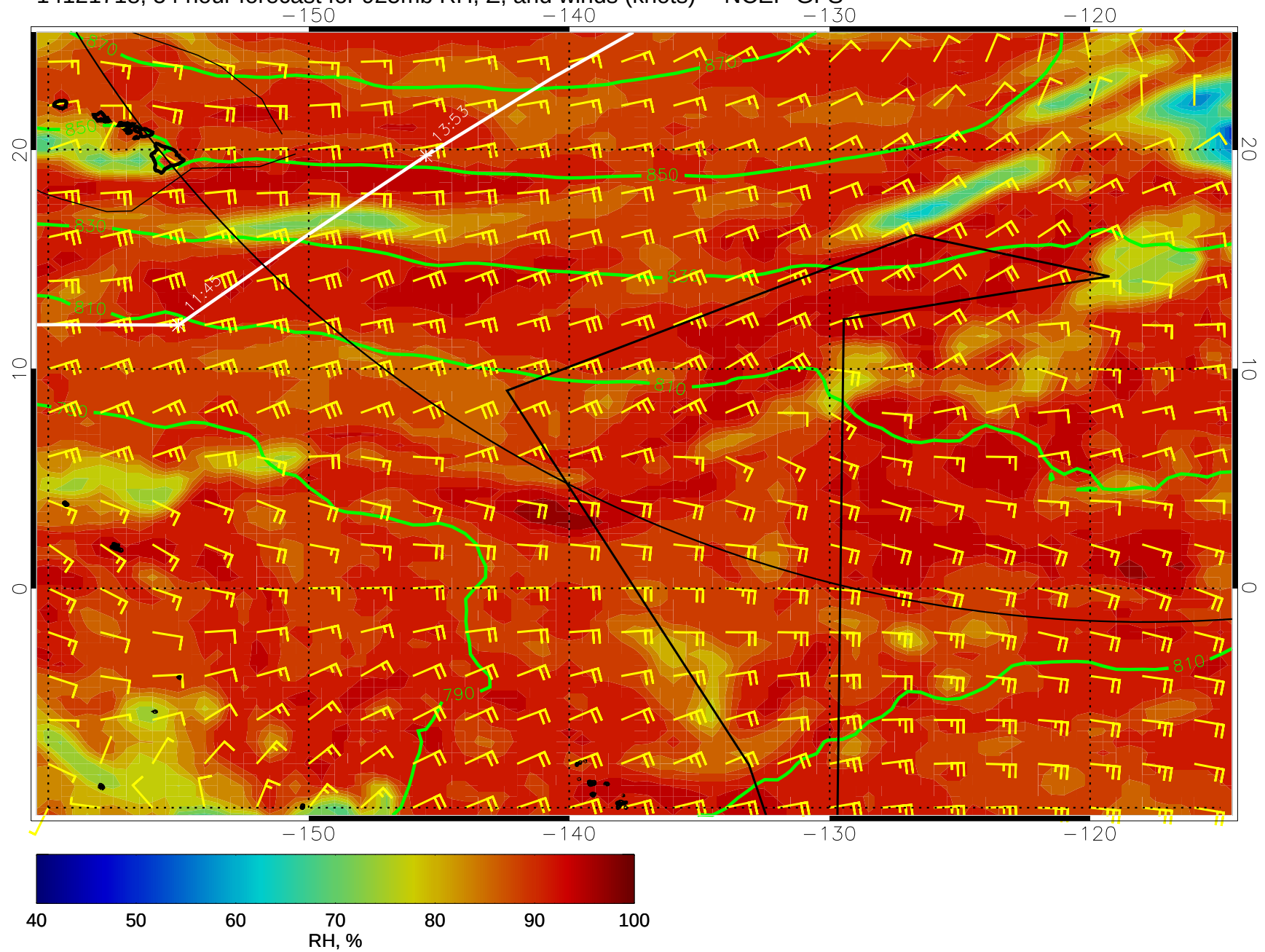
14121718, 54 hour forecast for 925mb RH, Z, and winds (knots) -- NCEP GFS
