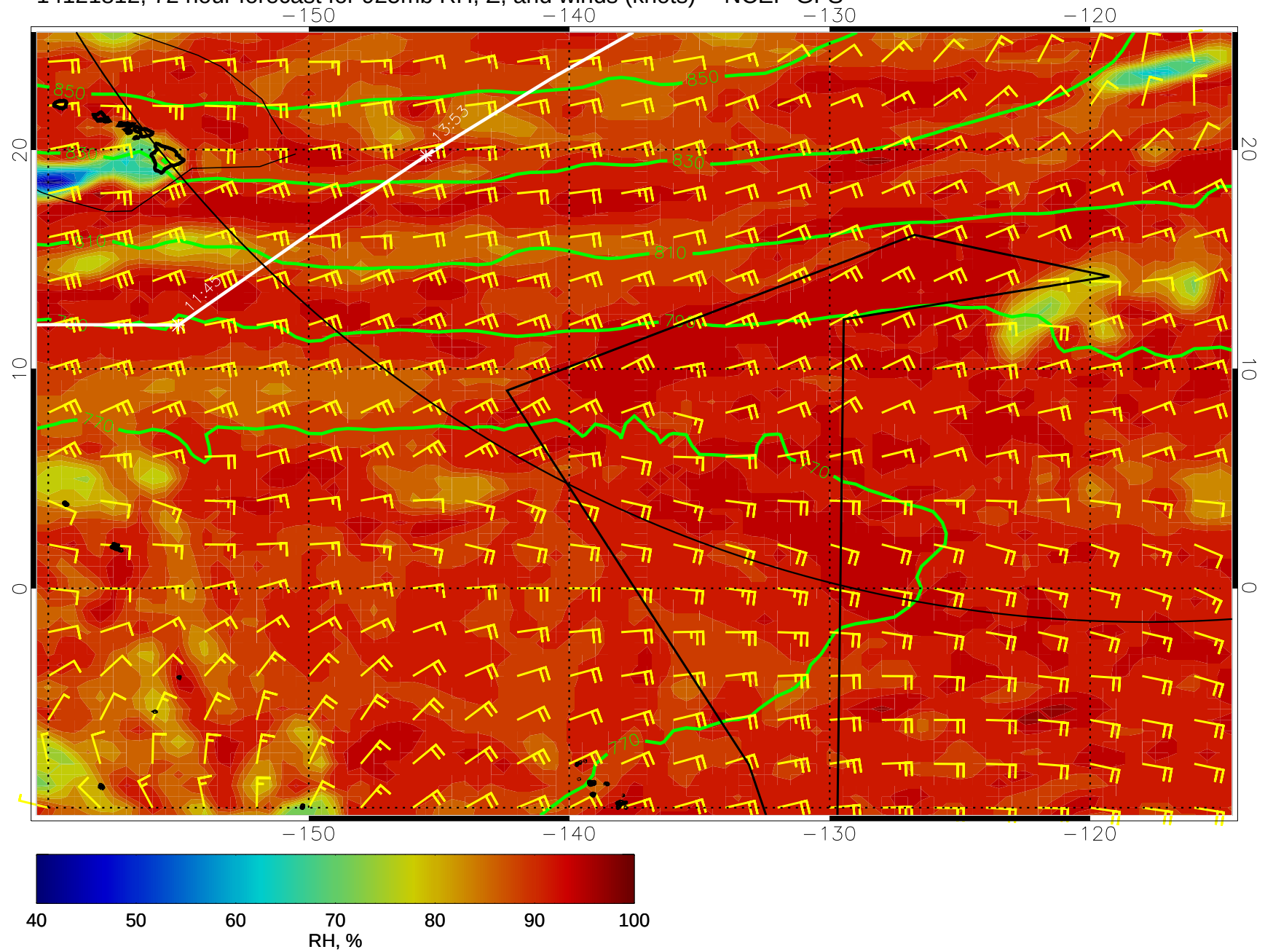
14121812, 72 hour forecast for 925mb RH, Z, and winds (knots) -- NCEP GFS
