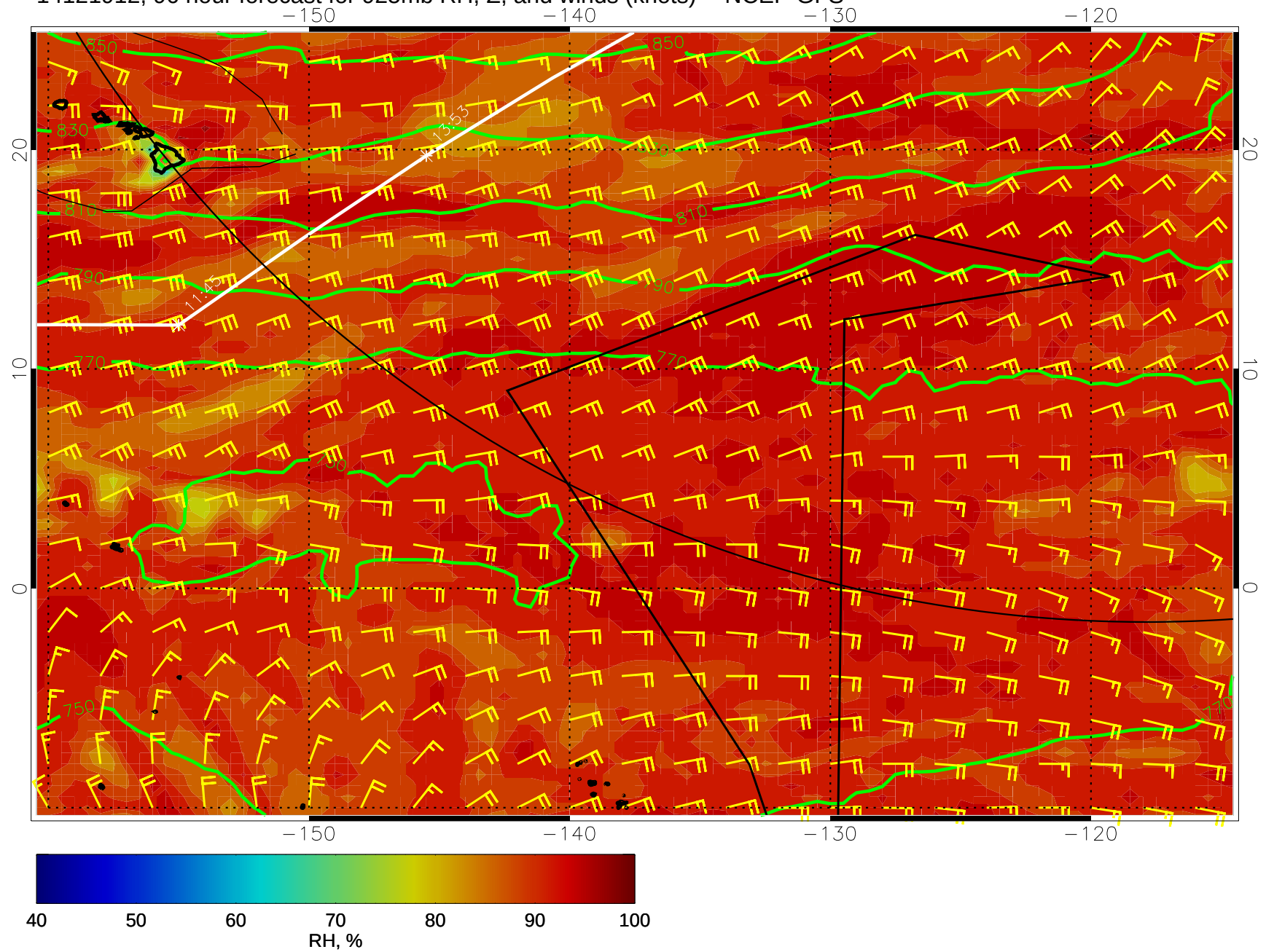
14121912, 96 hour forecast for 925mb RH, Z, and winds (knots) -- NCEP GFS
