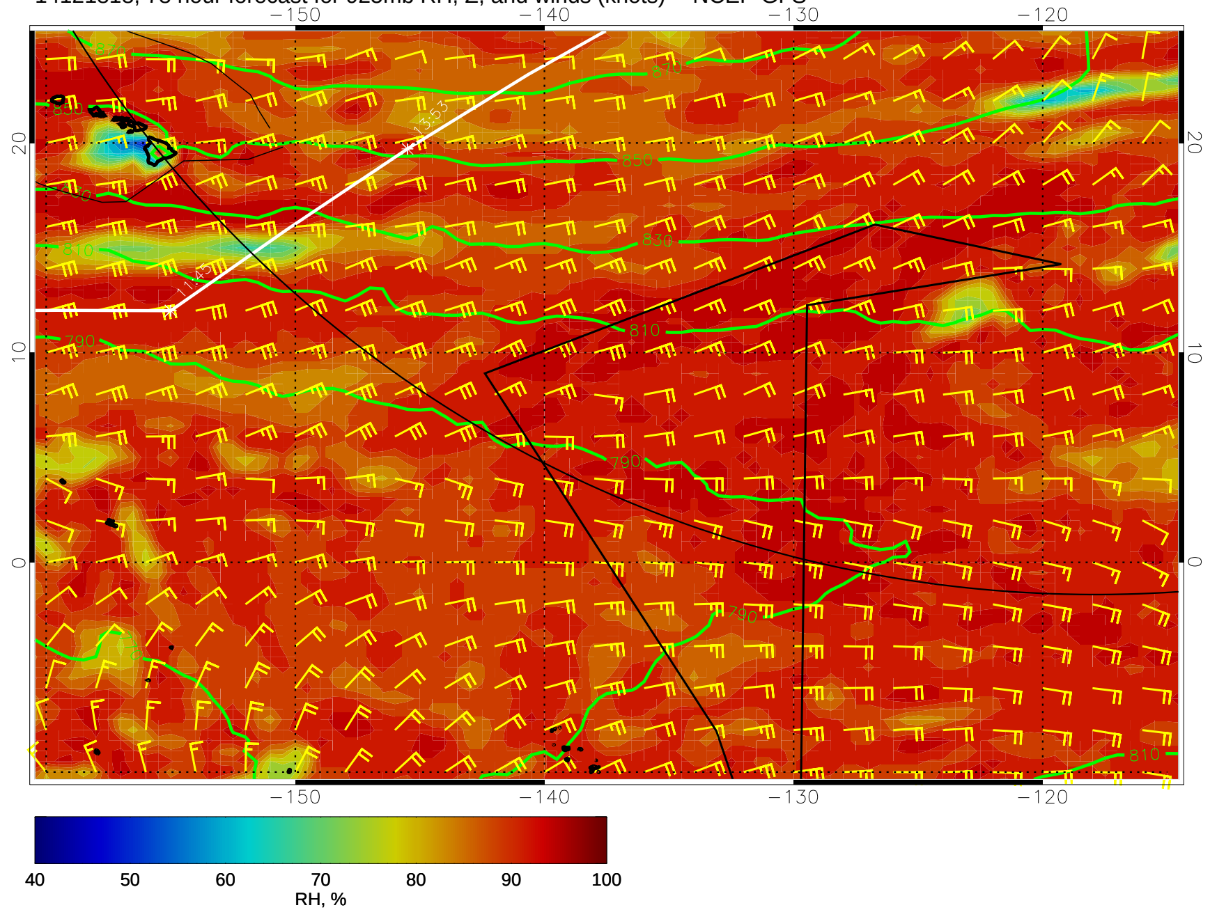
14121818, 78 hour forecast for 925mb RH, Z, and winds (knots) -- NCEP GFS
