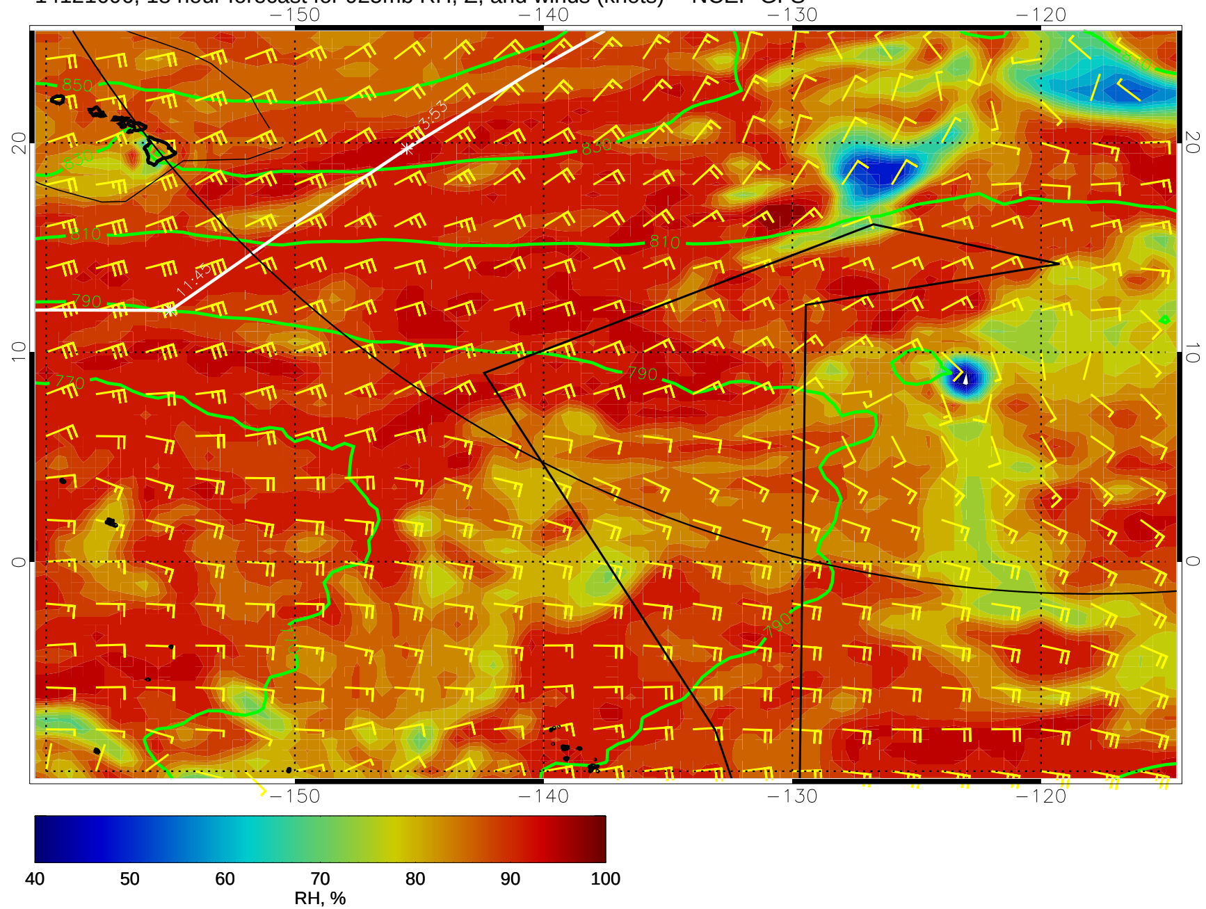
14121606, 18 hour forecast for 925mb RH, Z, and winds (knots) -- NCEP GFS
