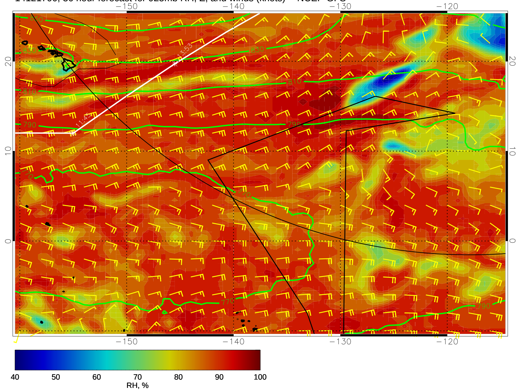
14121700, 36 hour forecast for 925mb RH, Z, and winds (knots) -- NCEP GFS
