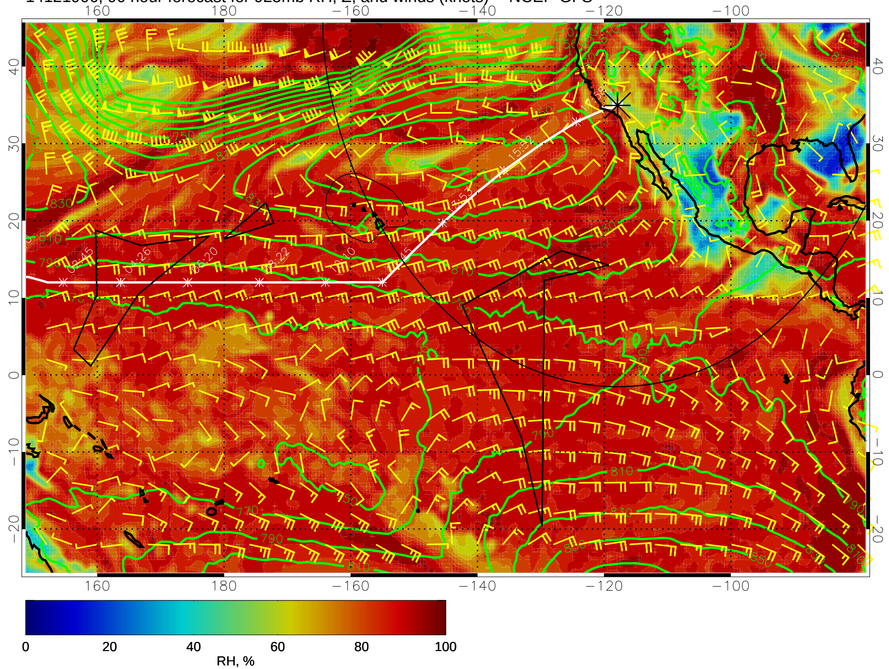
14121906, 90 hour forecast for 925mb RH, Z, and winds (knots) -- NCEP GFS
