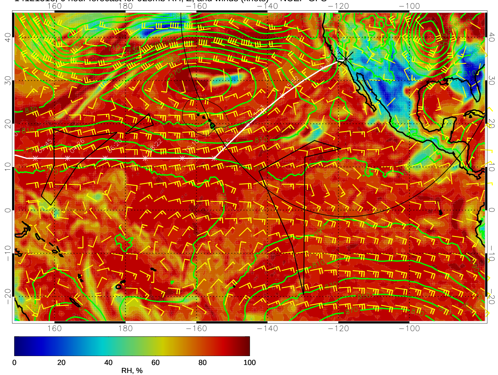
14121518, 6 hour forecast for 925mb RH, Z, and winds (knots) -- NCEP GFS
