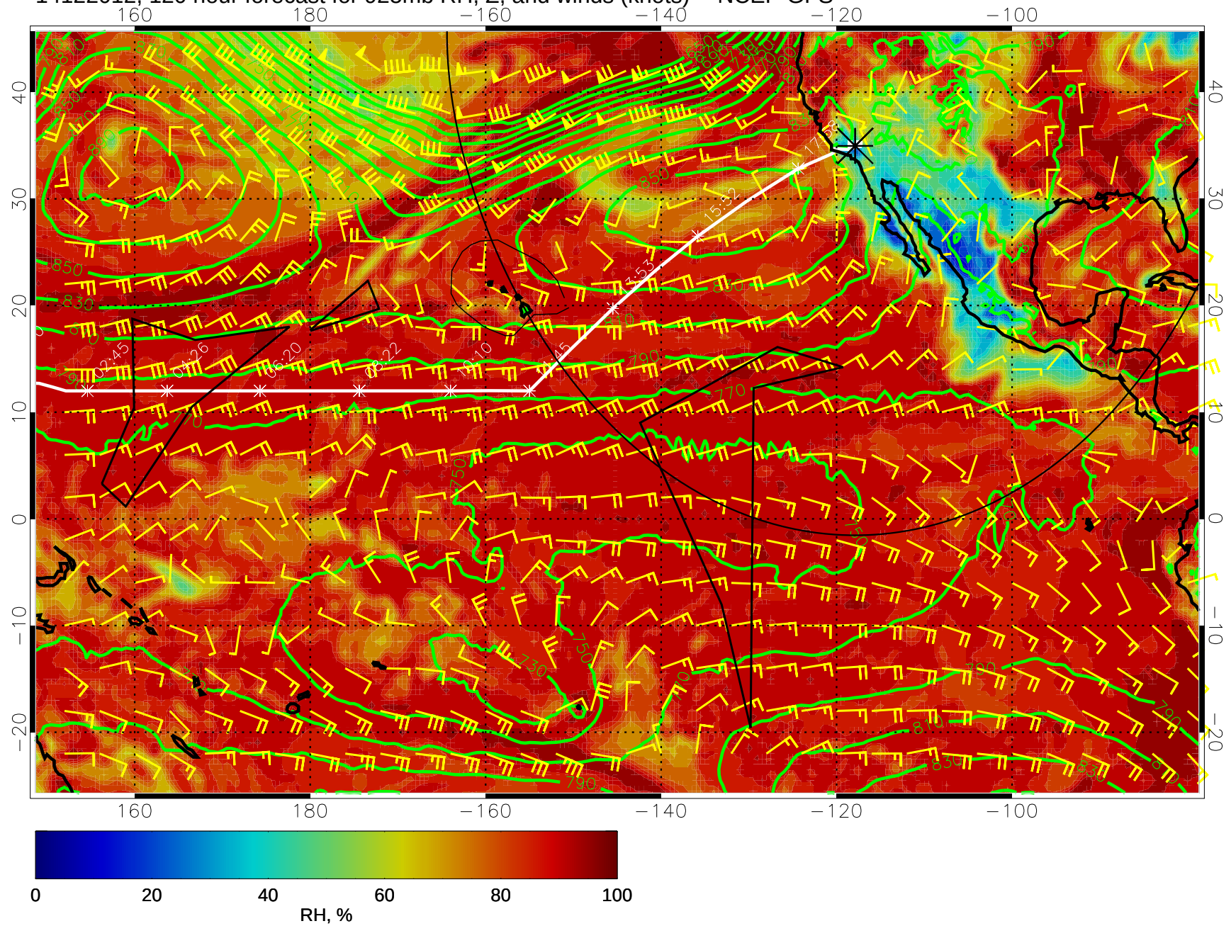
14122012, 120 hour forecast for 925mb RH, Z, and winds (knots) -- NCEP GFS
