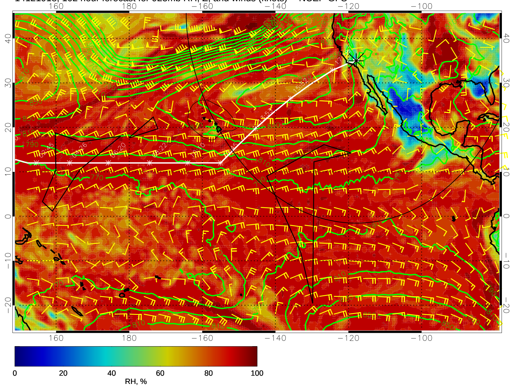
14121918, 102 hour forecast for 925mb RH, Z, and winds (knots) -- NCEP GFS
