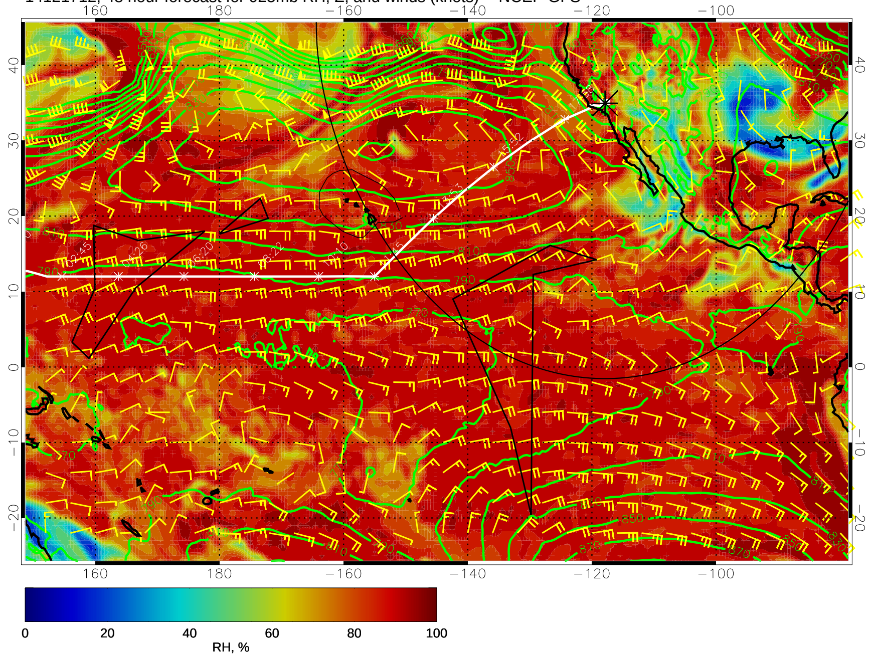
14121712, 48 hour forecast for 925mb RH, Z, and winds (knots) -- NCEP GFS
