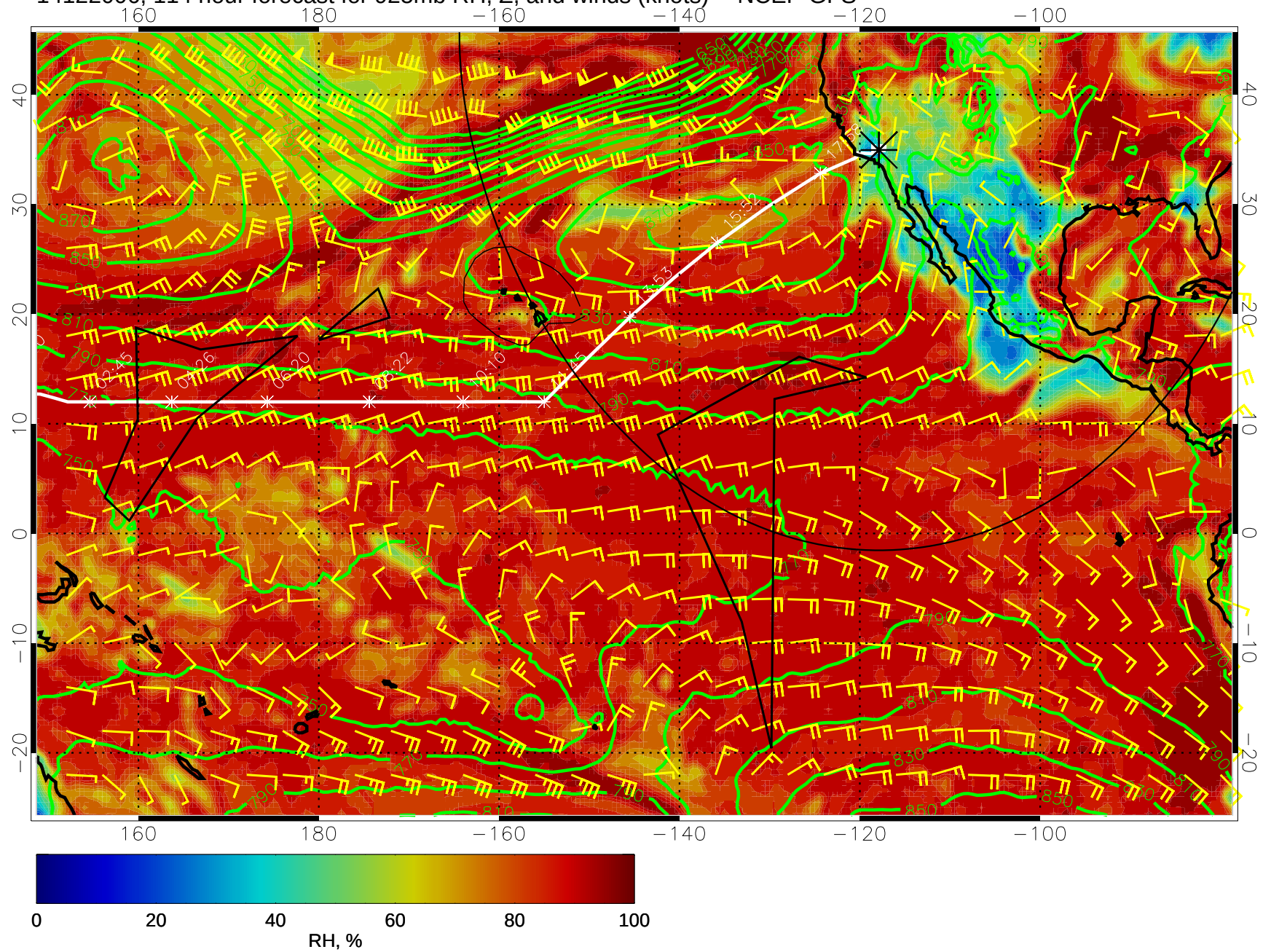
14122006, 114 hour forecast for 925mb RH, Z, and winds (knots) -- NCEP GFS
