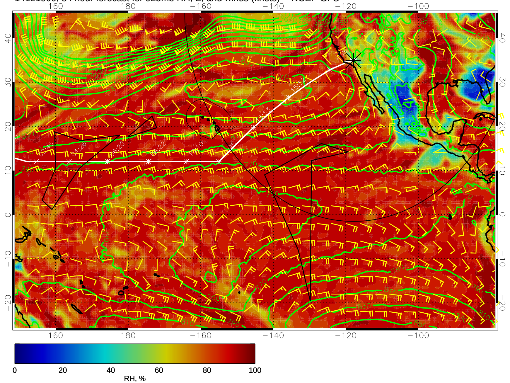
14121900, 84 hour forecast for 925mb RH, Z, and winds (knots) -- NCEP GFS
