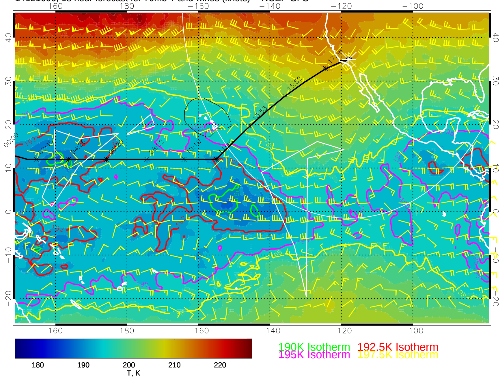
14121606, 18 hour forecast for 70mb T and winds (knots) -- NCEP GFS
