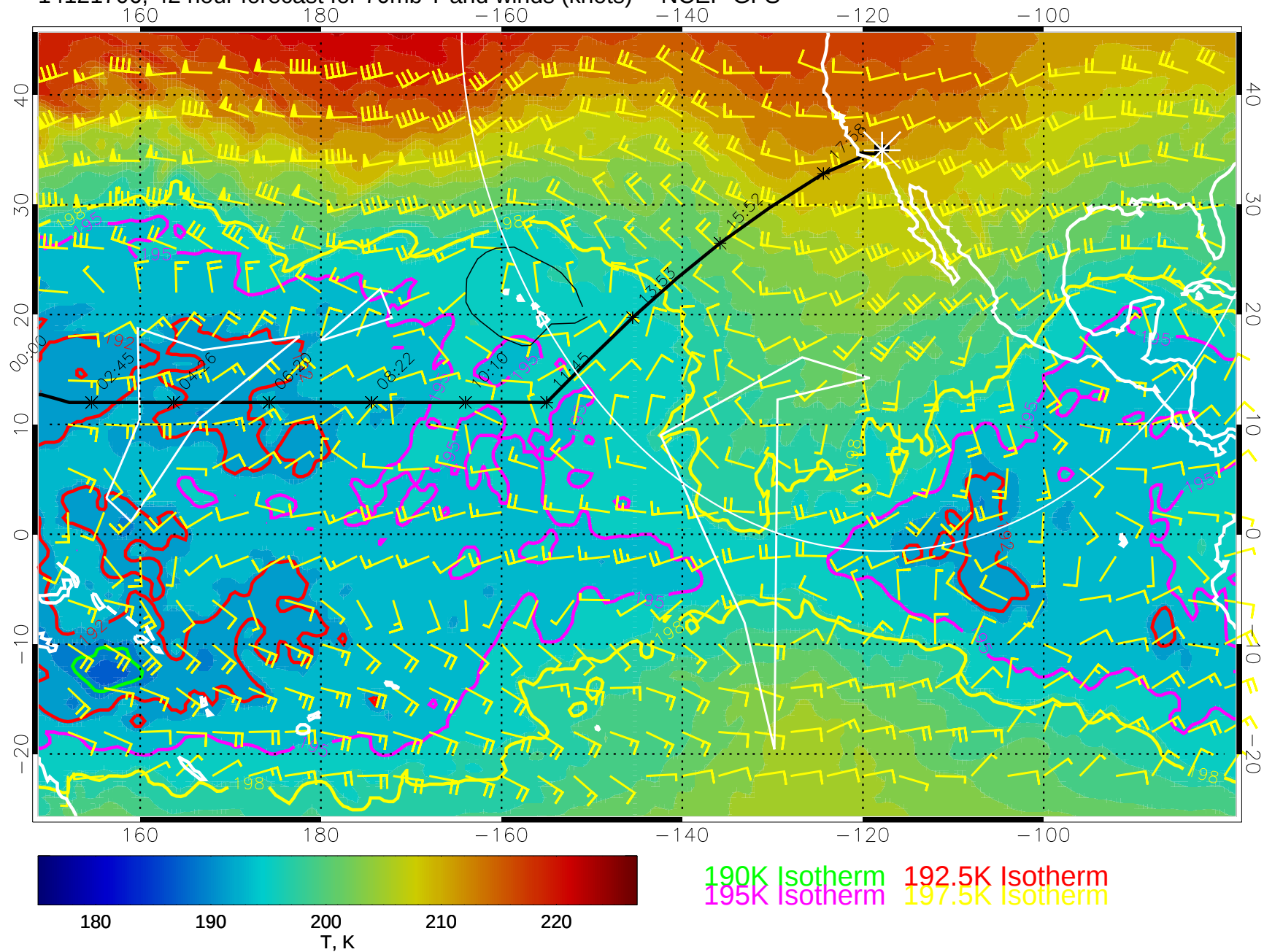
14121706, 42 hour forecast for 70mb T and winds (knots) -- NCEP GFS
