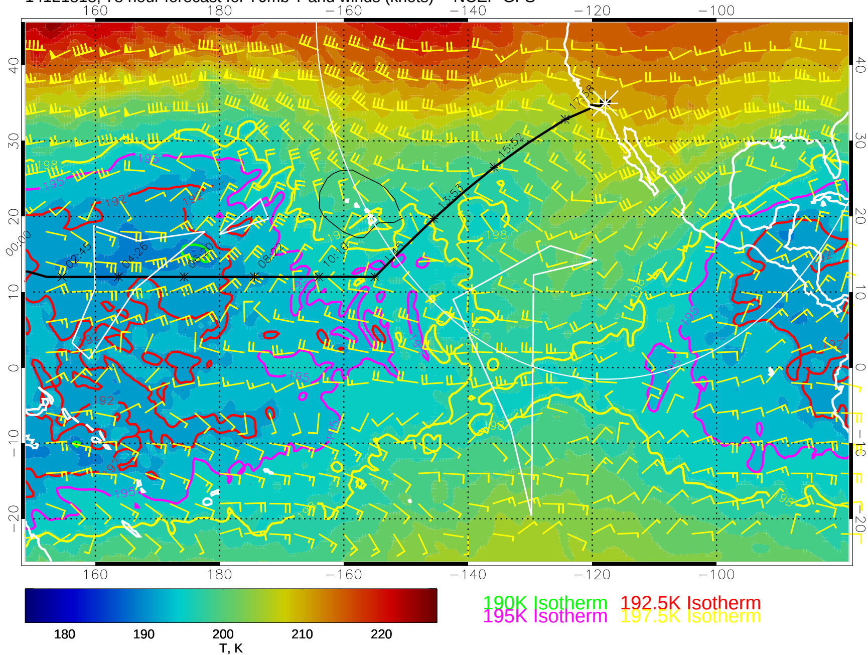
14121818, 78 hour forecast for 70mb T and winds (knots) -- NCEP GFS
