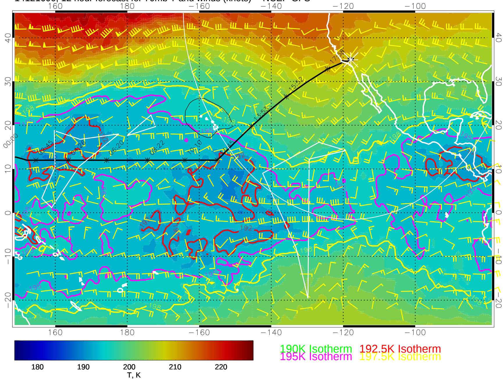
14121600, 12 hour forecast for 70mb T and winds (knots) -- NCEP GFS
