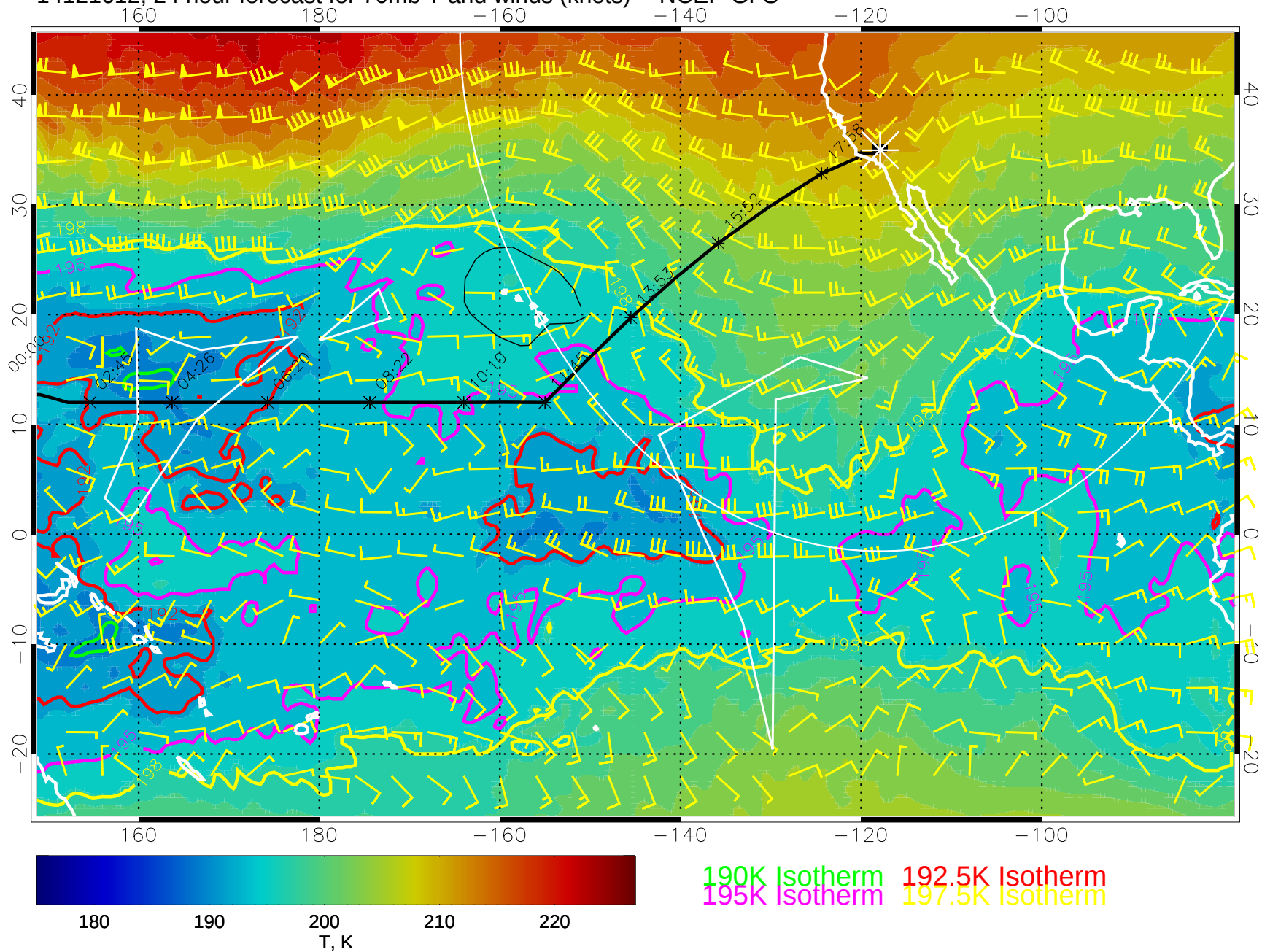
14121612, 24 hour forecast for 70mb T and winds (knots) -- NCEP GFS
