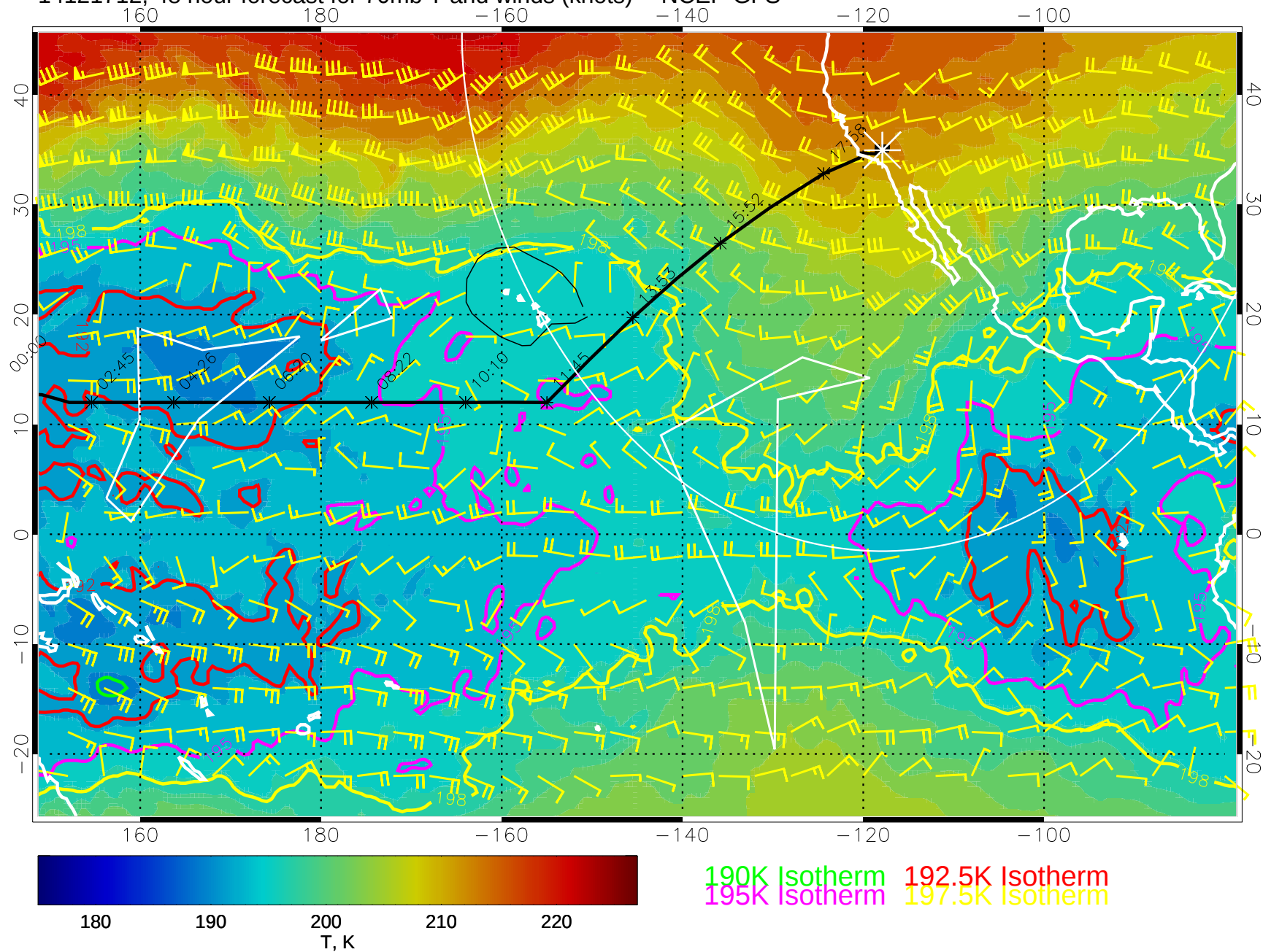
14121712, 48 hour forecast for 70mb T and winds (knots) -- NCEP GFS
