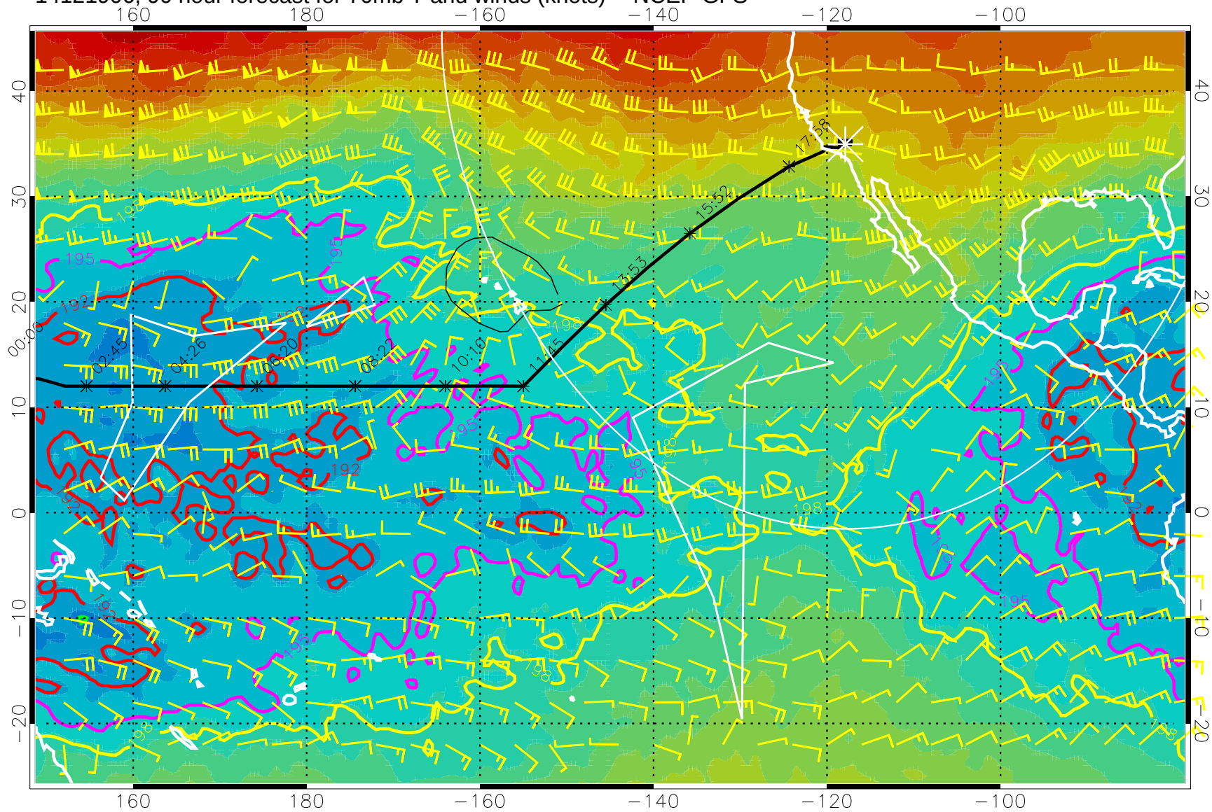
14121906, 90 hour forecast for 70mb T and winds (knots) -- NCEP GFS
