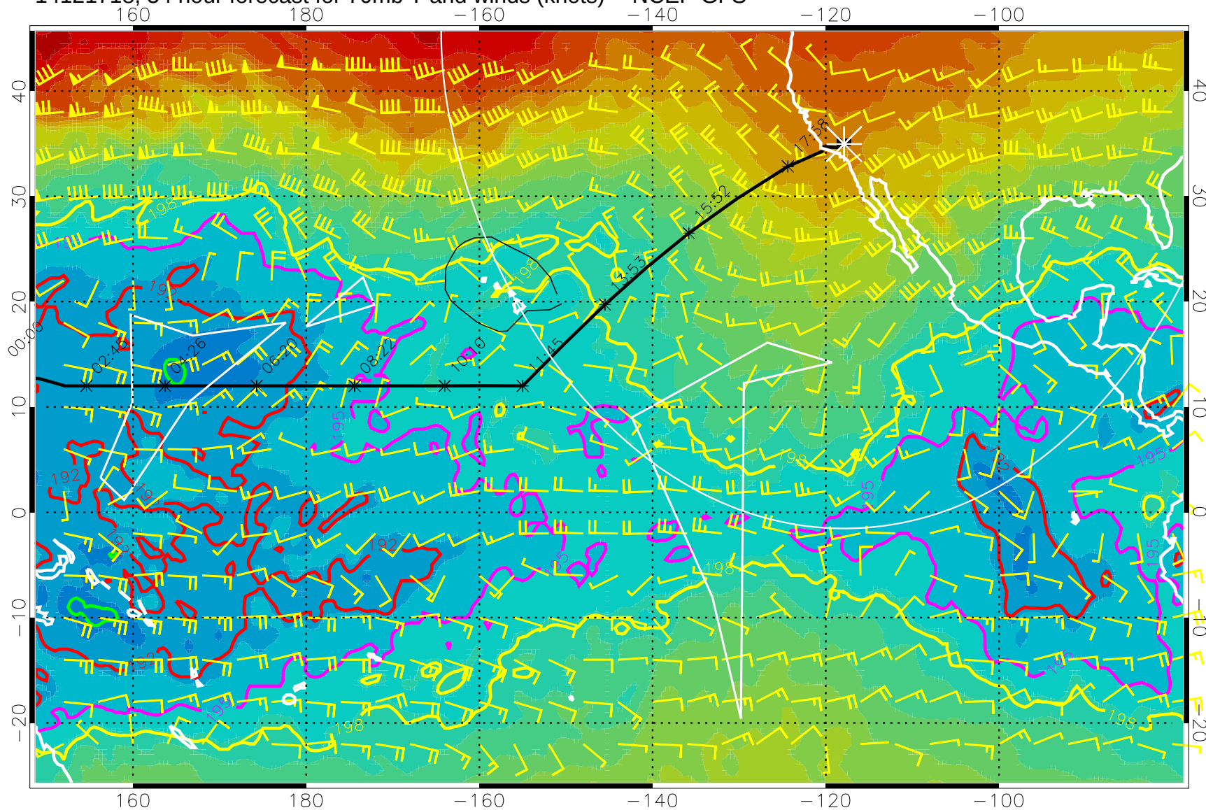
14121718, 54 hour forecast for 70mb T and winds (knots) -- NCEP GFS
