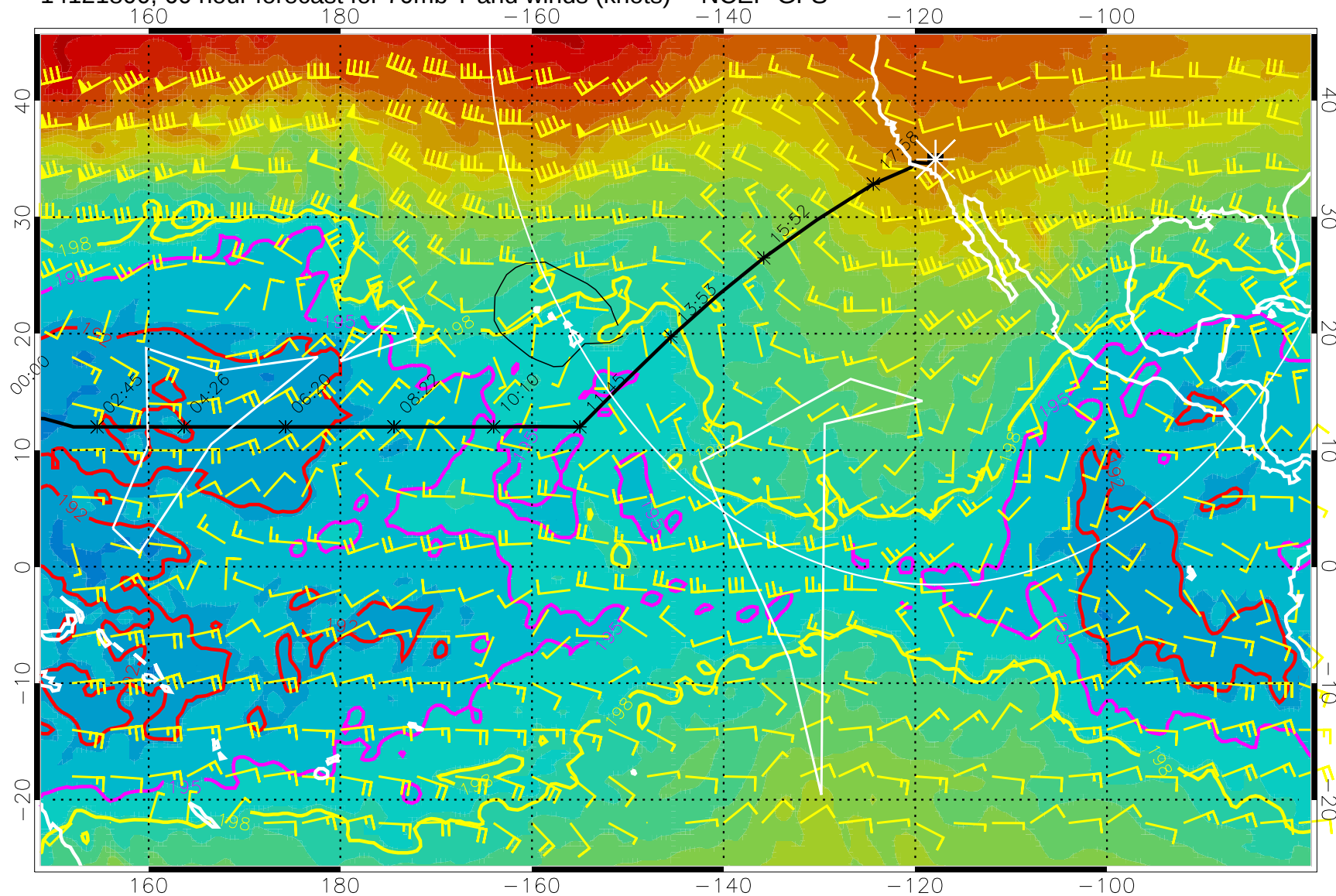
14121800, 60 hour forecast for 70mb T and winds (knots) -- NCEP GFS
