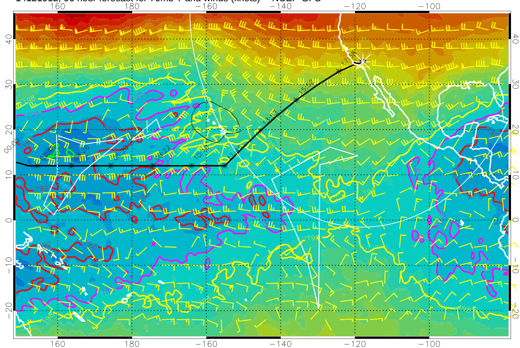
14121912, 96 hour forecast for 70mb T and winds (knots) -- NCEP GFS
