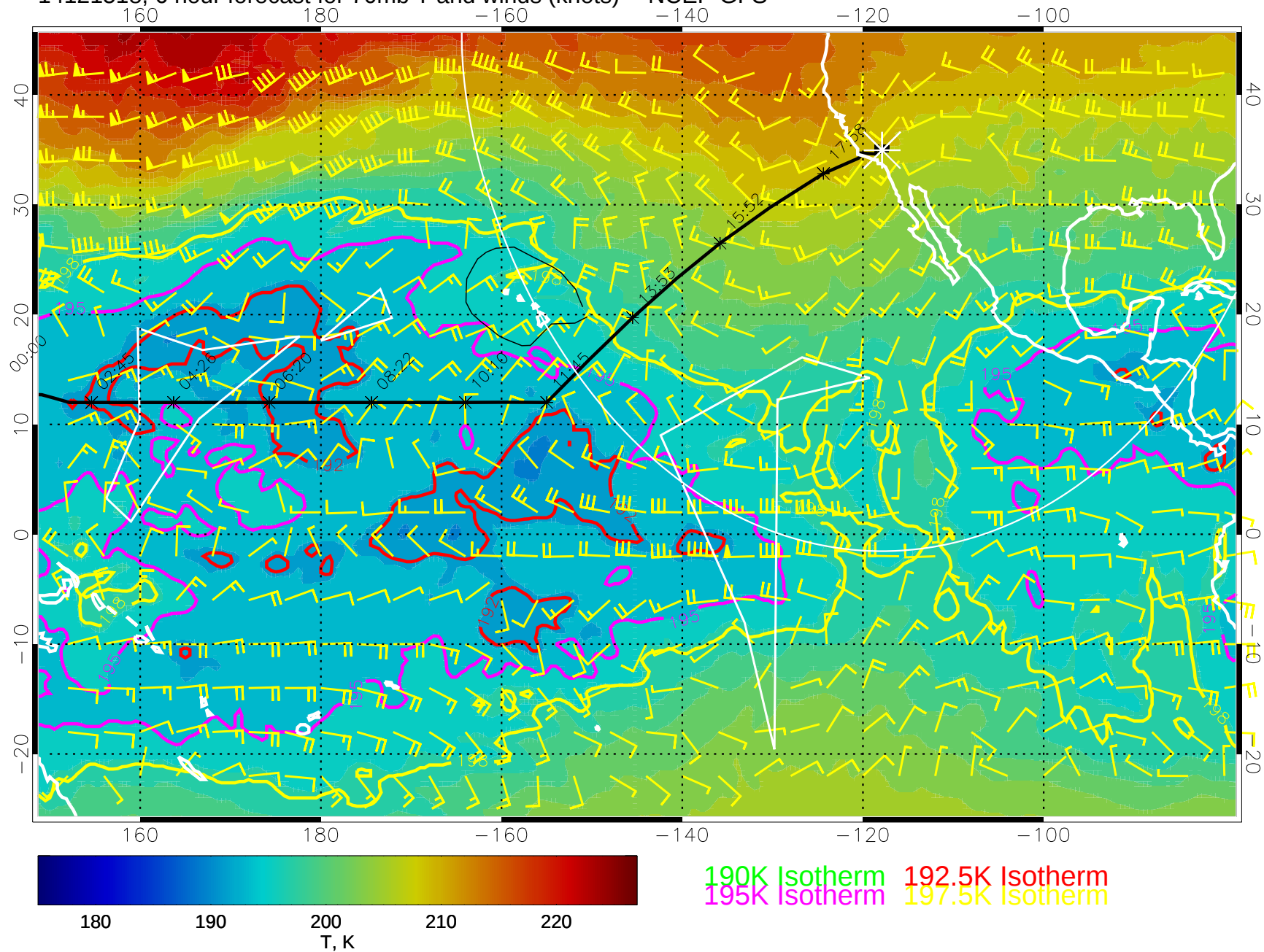
14121518, 6 hour forecast for 70mb T and winds (knots) -- NCEP GFS
