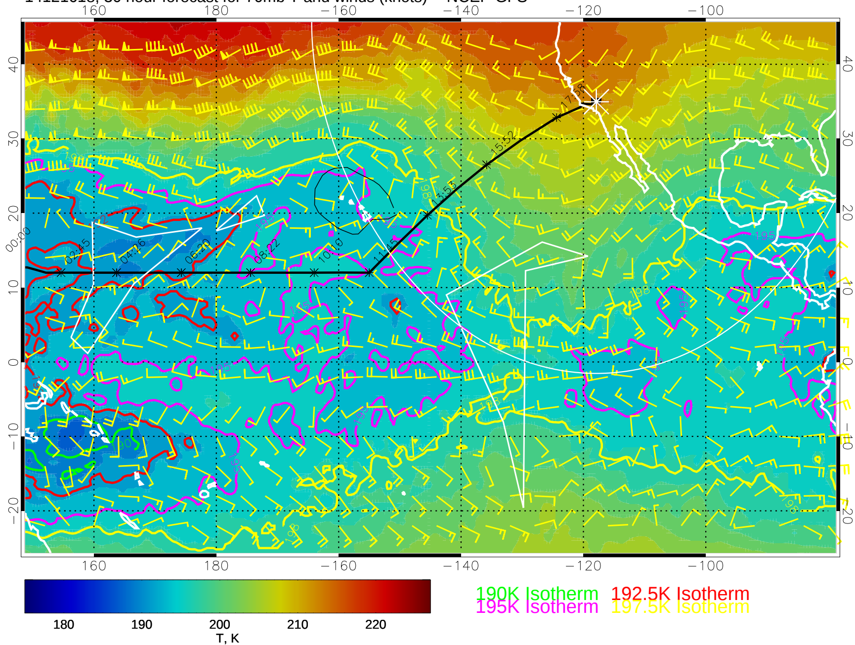
14121618, 30 hour forecast for 70mb T and winds (knots) -- NCEP GFS
