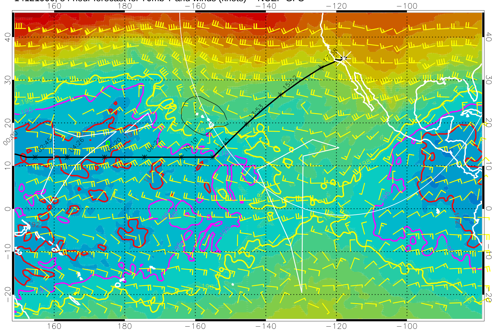
14121900, 84 hour forecast for 70mb T and winds (knots) -- NCEP GFS
