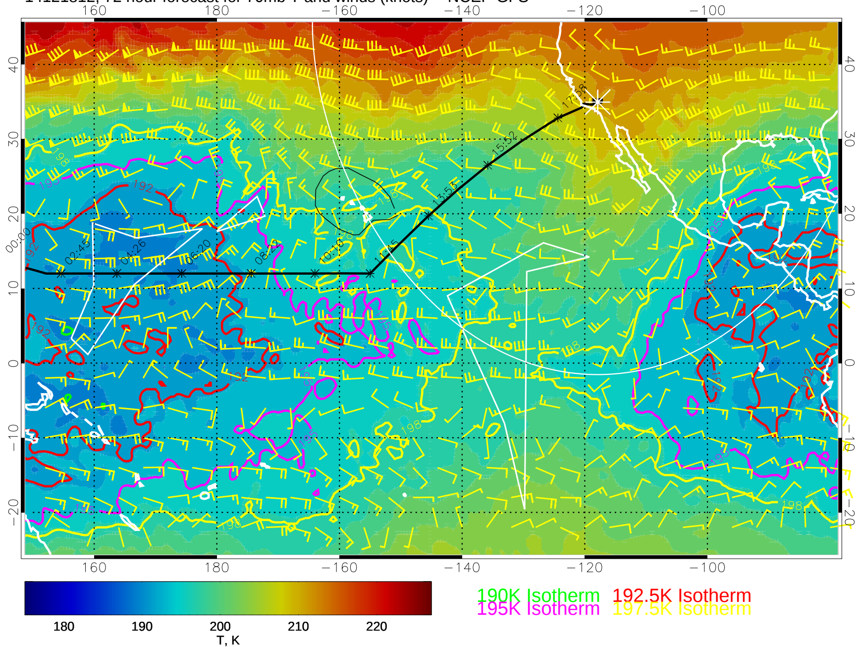
14121812, 72 hour forecast for 70mb T and winds (knots) -- NCEP GFS
