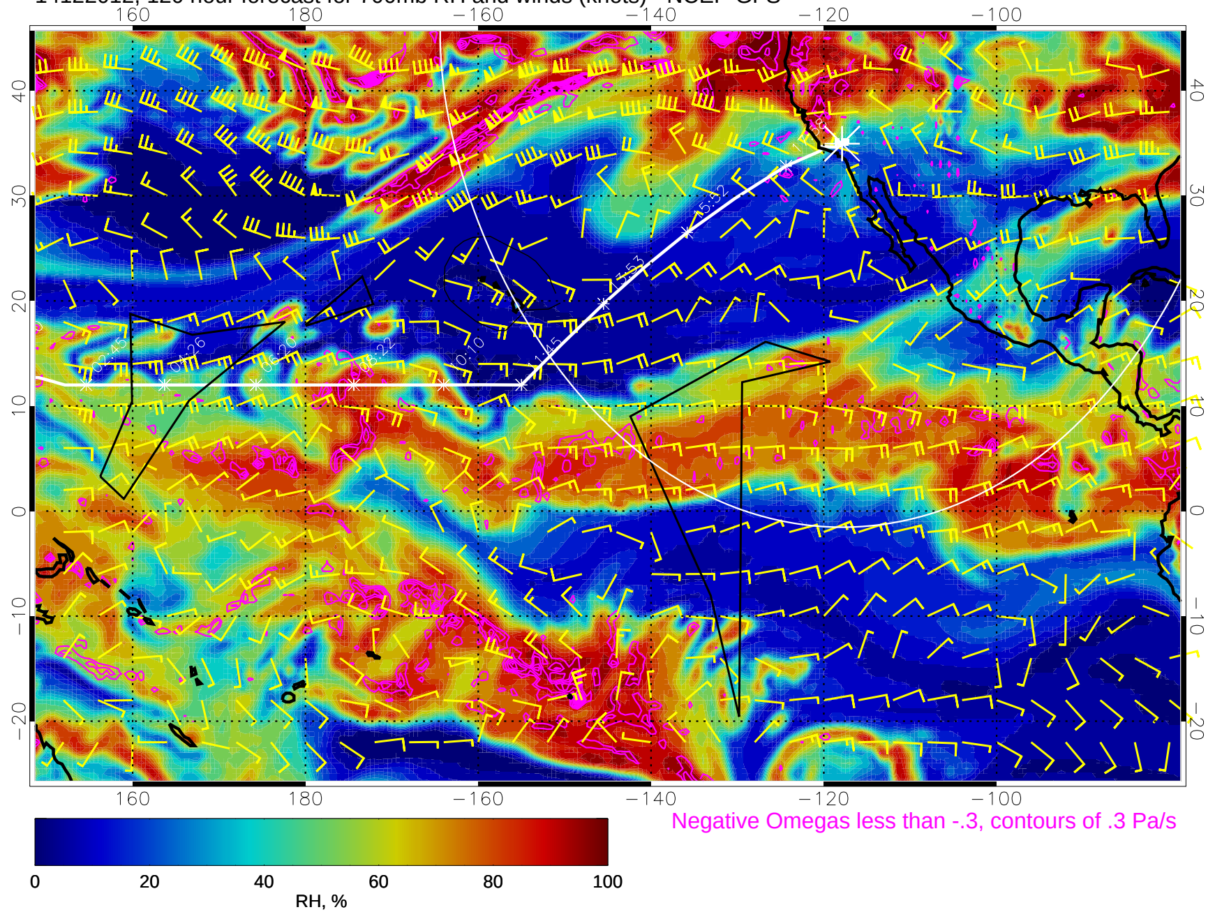
14122012, 120 hour forecast for 700mb RH and winds (knots) - NCEP GFS
