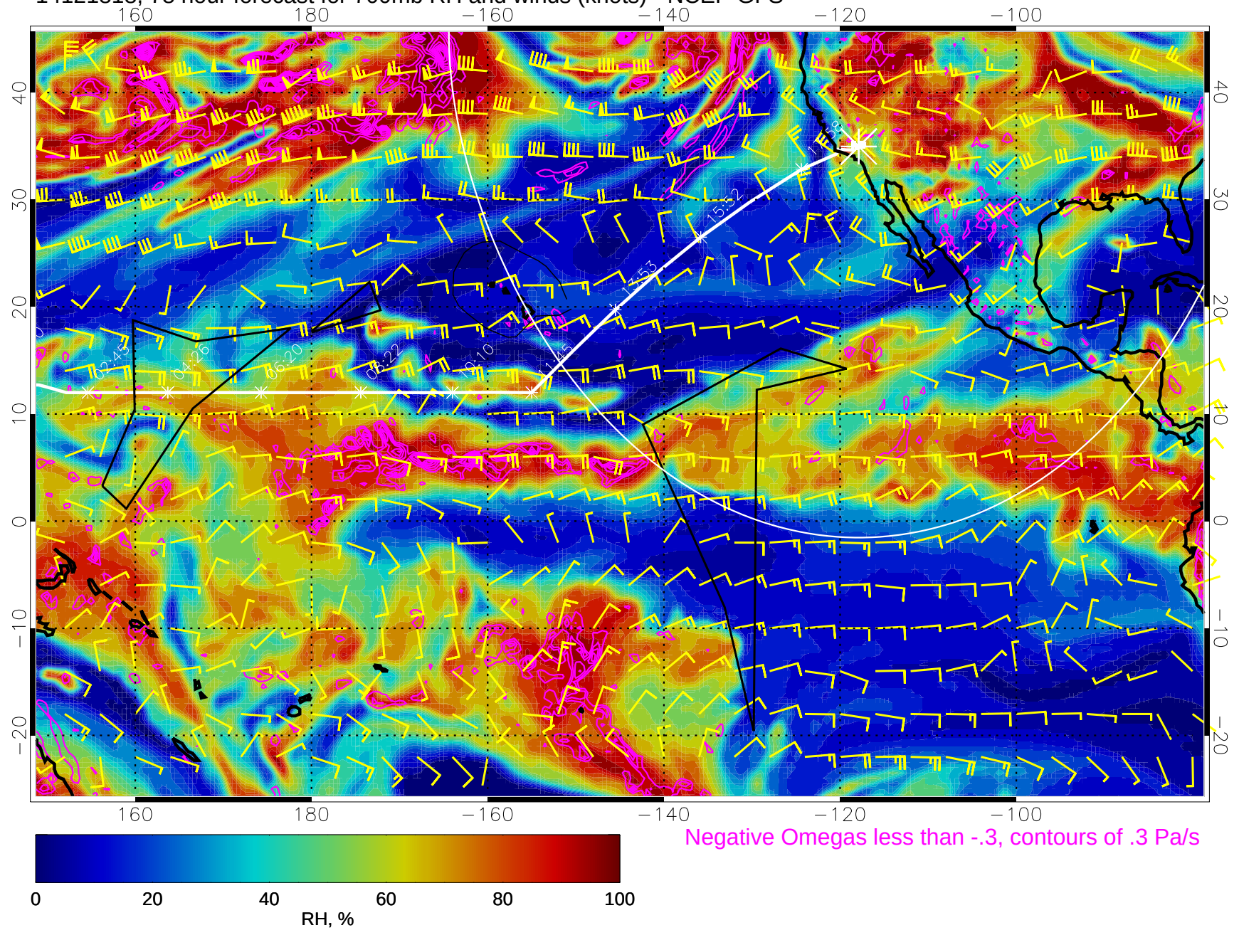
14121818, 78 hour forecast for 700mb RH and winds (knots) - NCEP GFS
