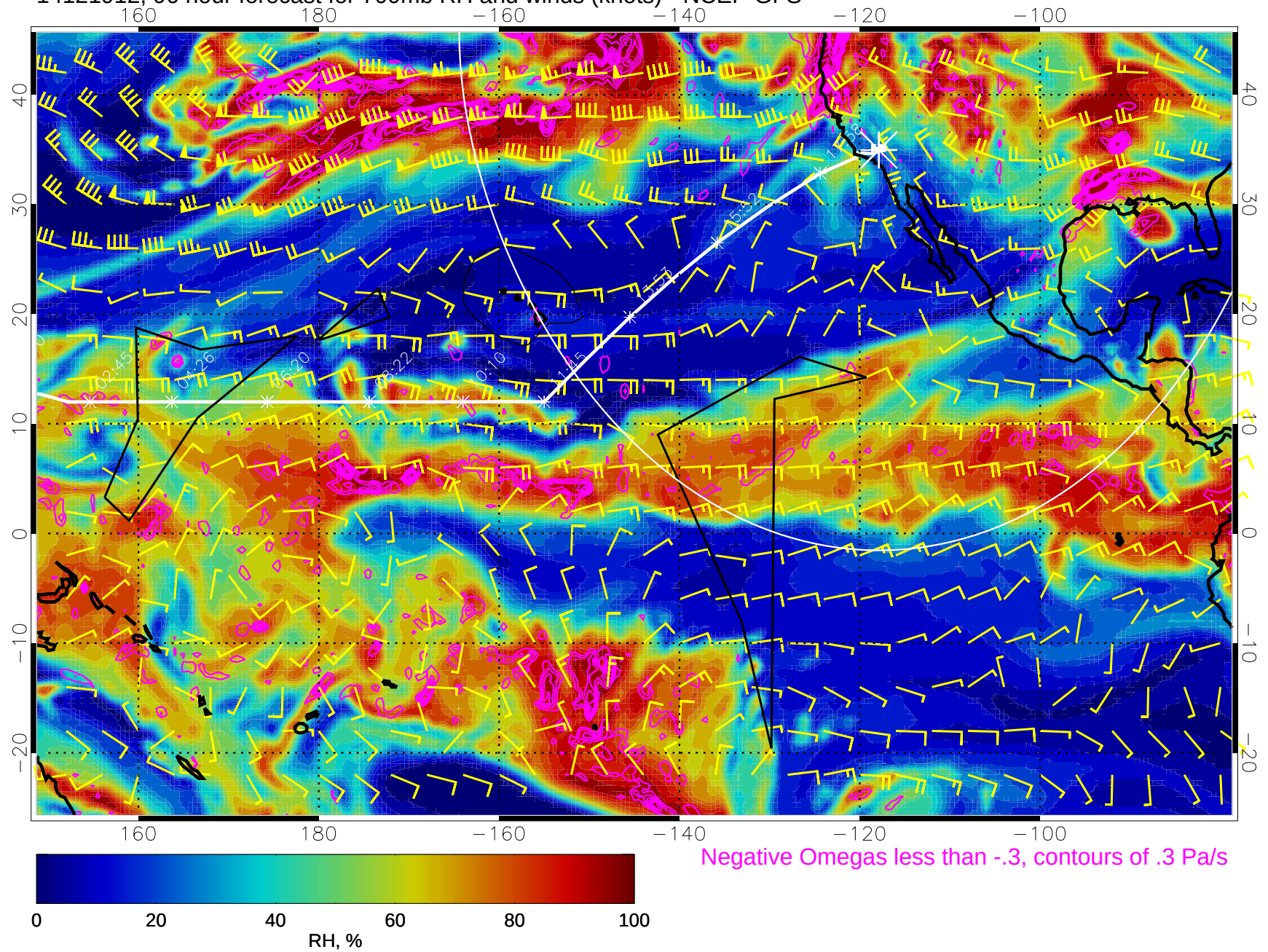
14121912, 96 hour forecast for 700mb RH and winds (knots) - NCEP GFS
