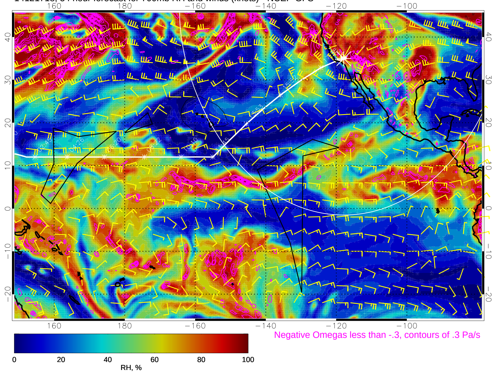
14121718, 54 hour forecast for 700mb RH and winds (knots) - NCEP GFS
