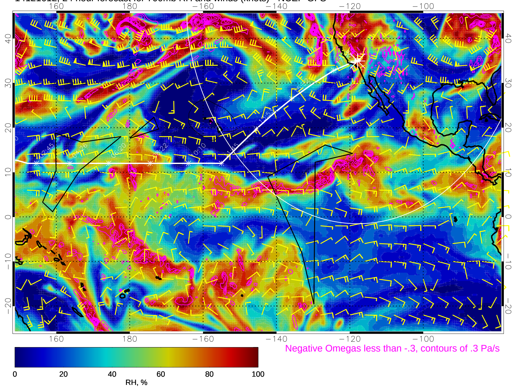
14121612, 24 hour forecast for 700mb RH and winds (knots) - NCEP GFS
