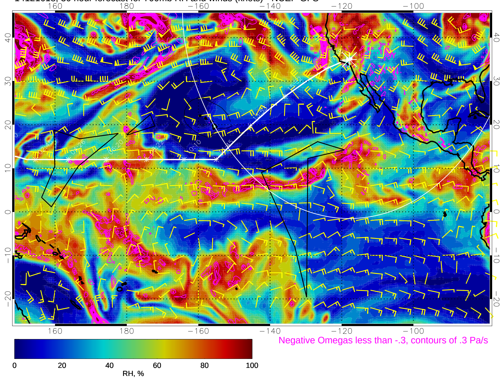
14121618, 30 hour forecast for 700mb RH and winds (knots) - NCEP GFS
