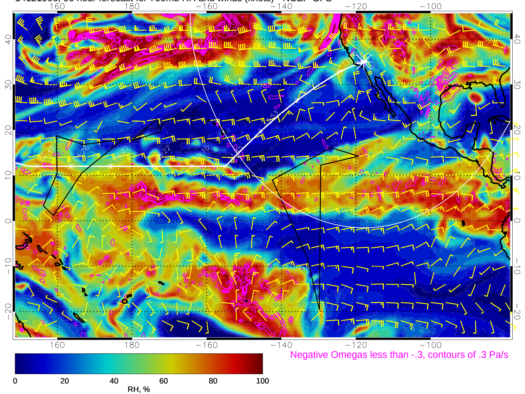
14121906, 90 hour forecast for 700mb RH and winds (knots) - NCEP GFS
