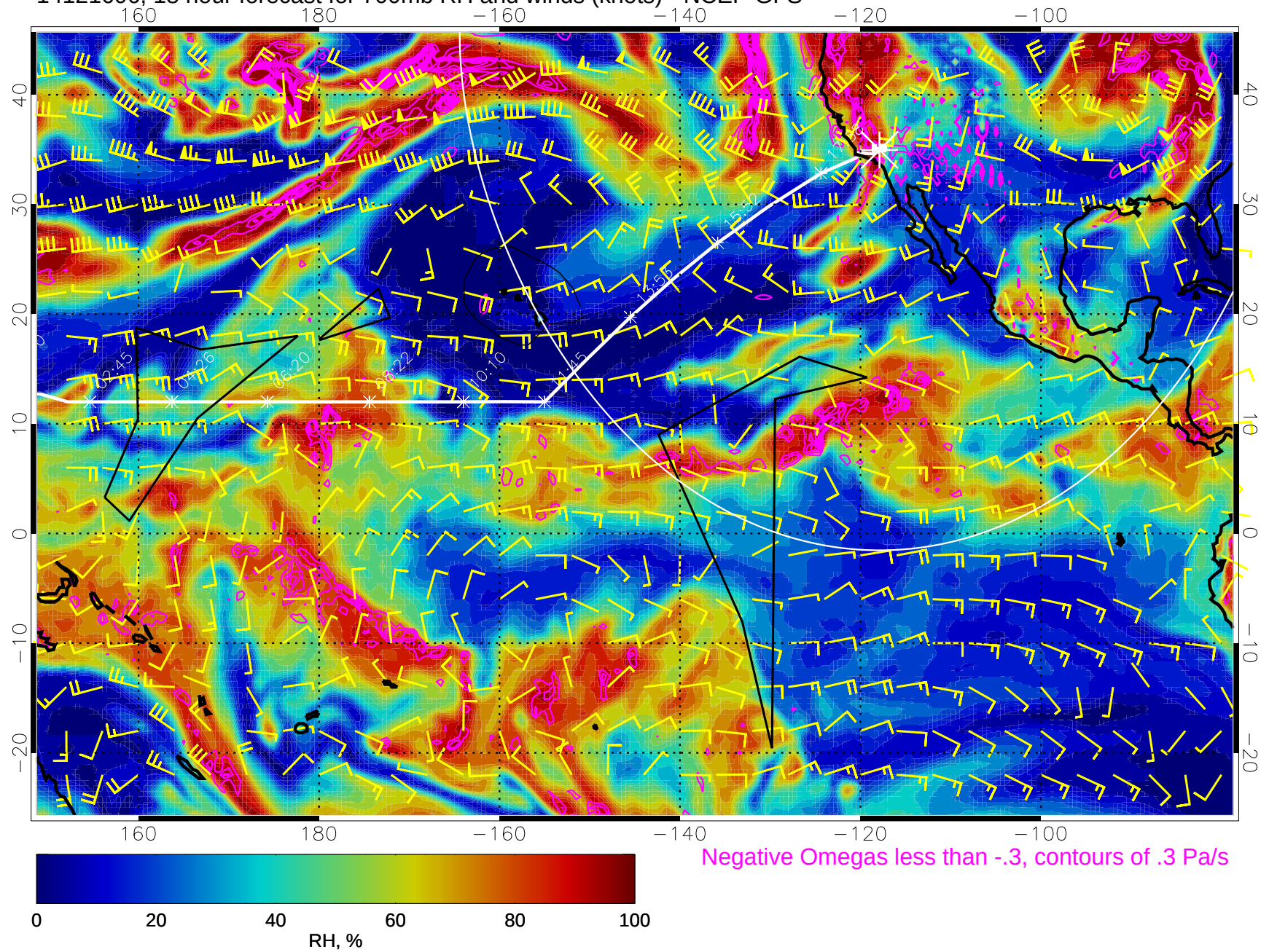
14121606, 18 hour forecast for 700mb RH and winds (knots) - NCEP GFS
