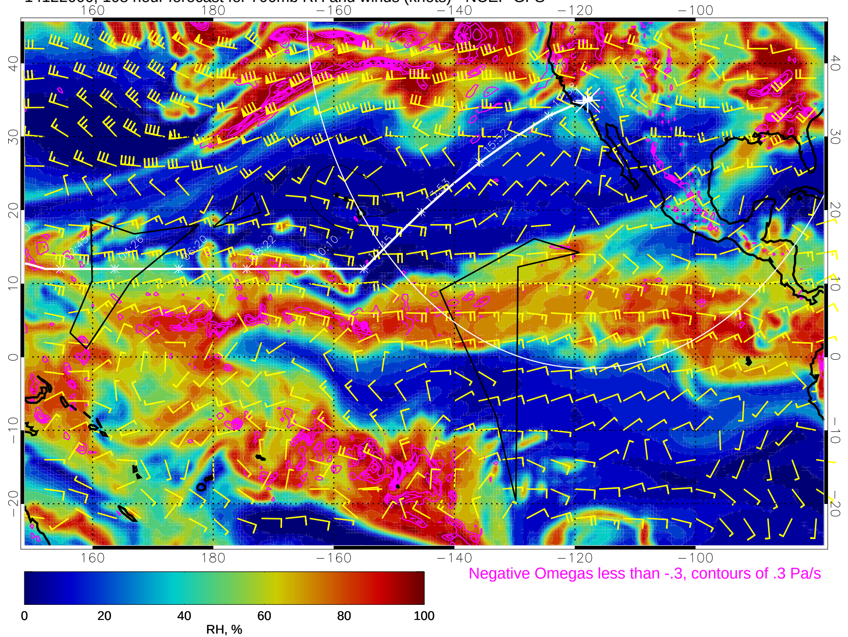
14122000, 108 hour forecast for 700mb RH and winds (knots) - NCEP GFS
