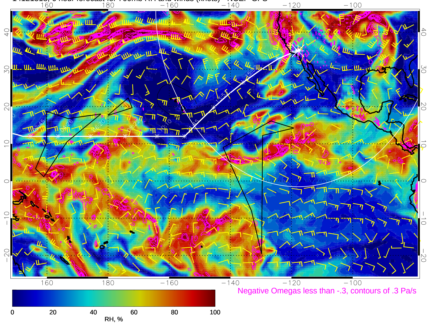
14121518, 6 hour forecast for 700mb RH and winds (knots) - NCEP GFS
