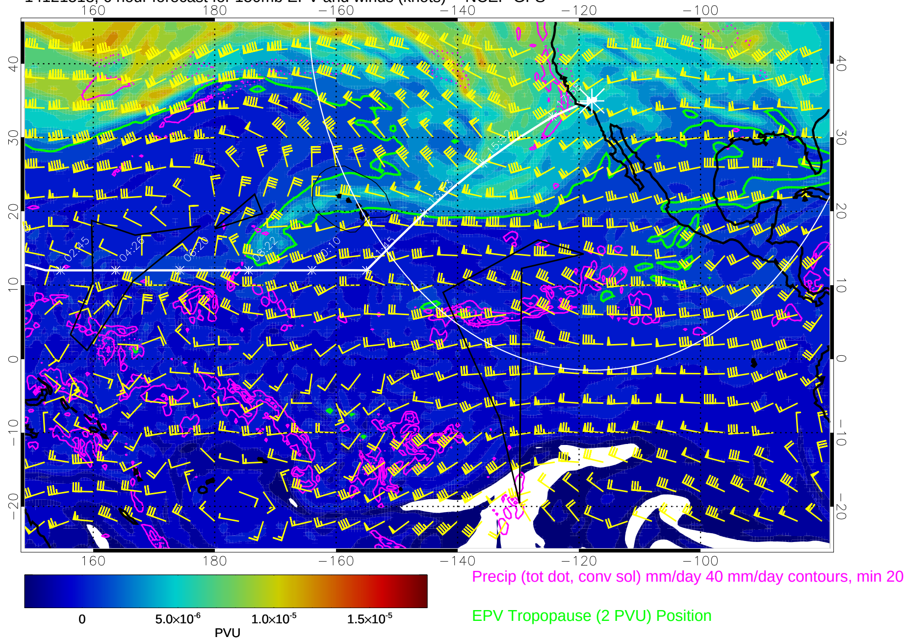
14121518, 6 hour forecast for 150mb EPV and winds (knots) -- NCEP GFS
