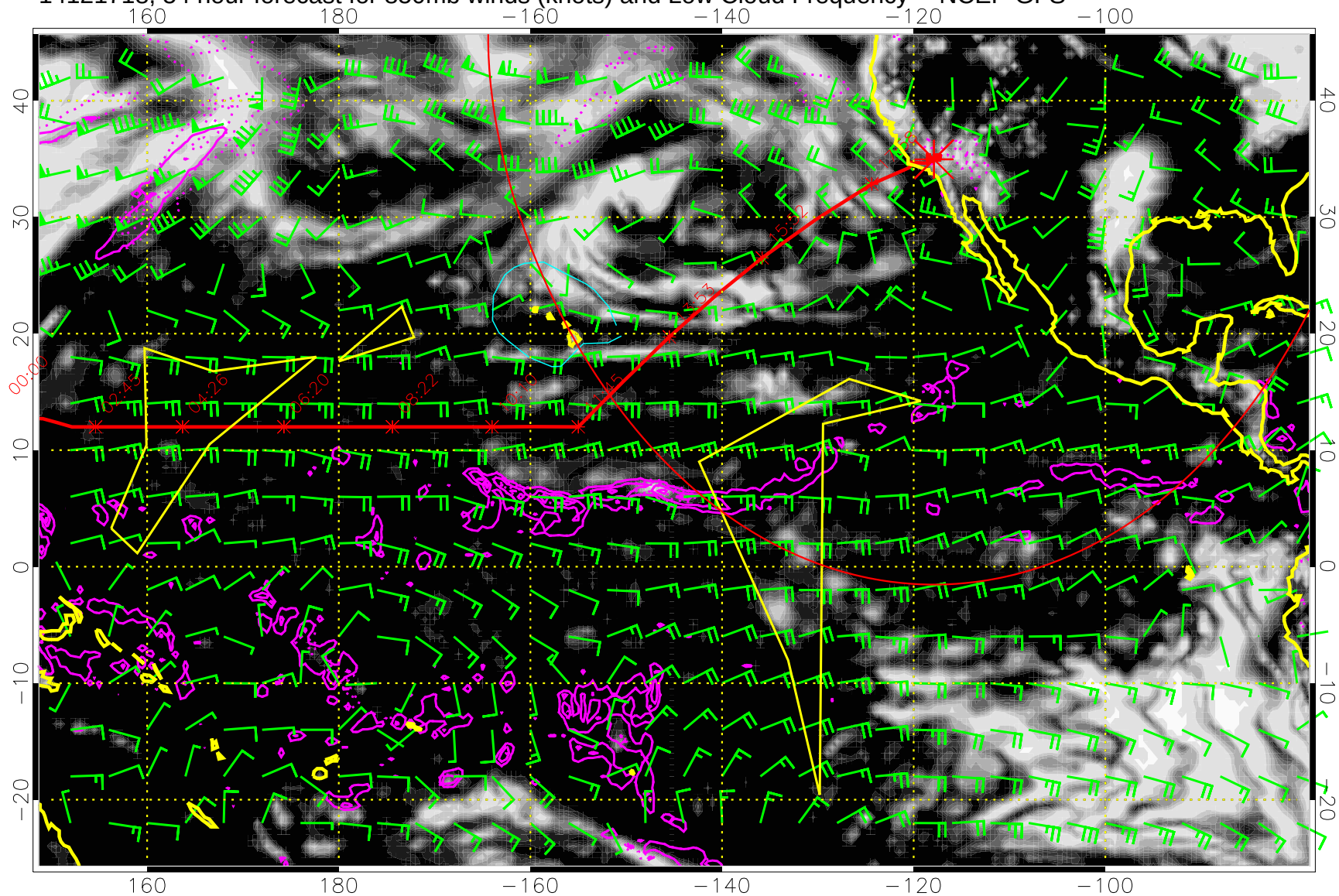
14121718, 54 hour forecast for 850mb winds (knots) and Low Cloud Frequency -- NCEP GFS
