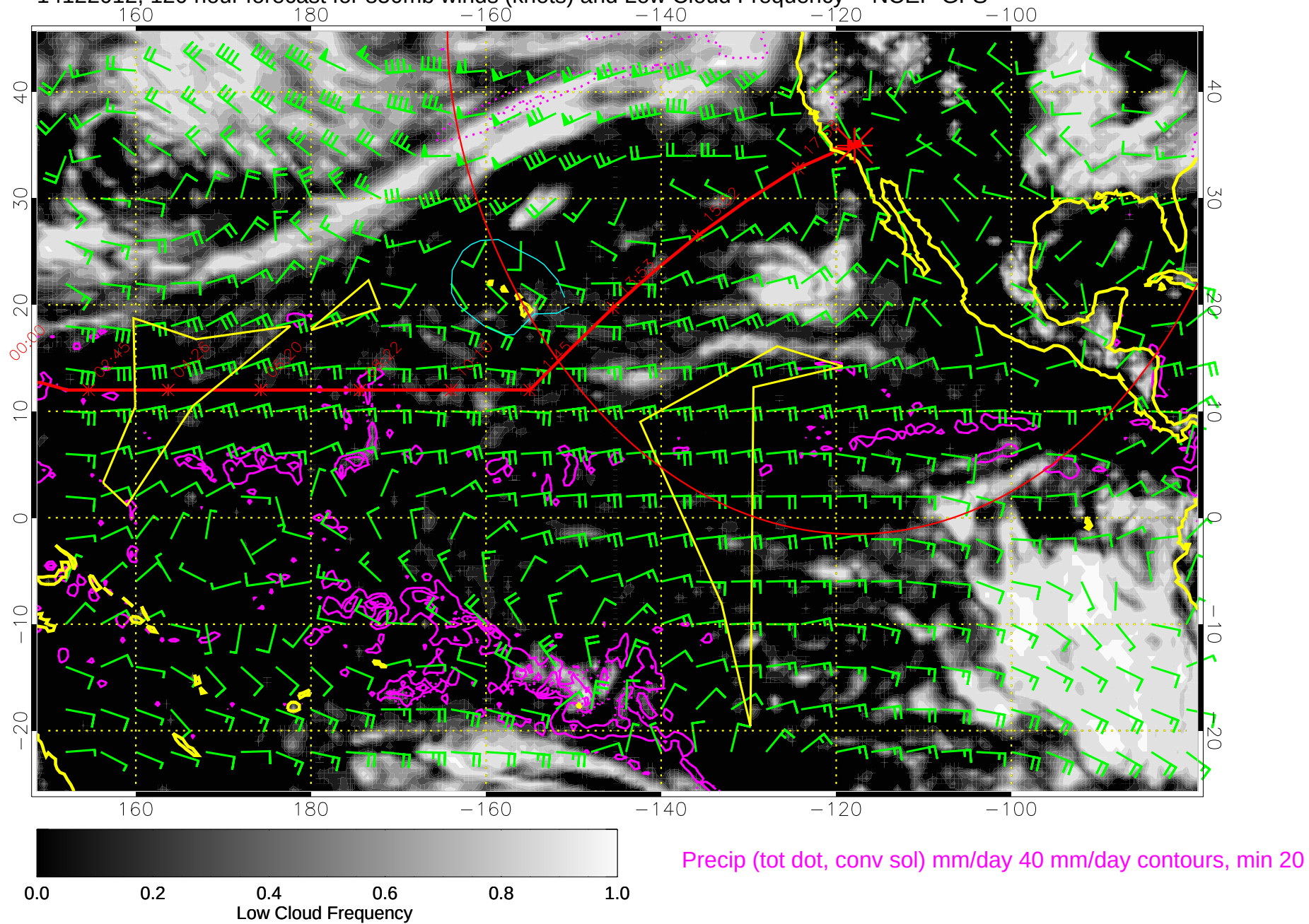
14122012, 120 hour forecast for 850mb winds (knots) and Low Cloud Frequency -- NCEP GFS
