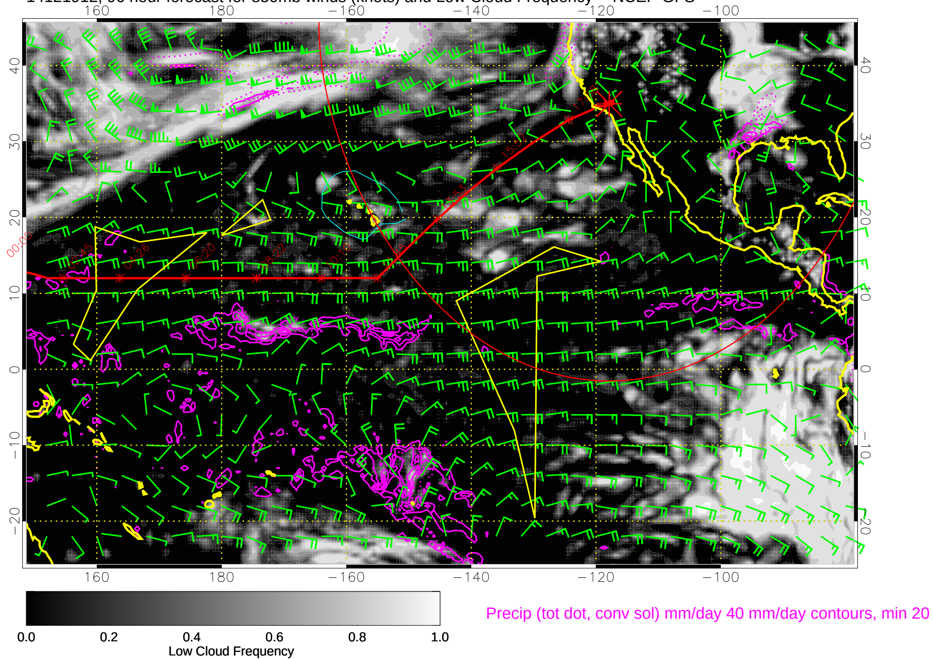
14121912, 96 hour forecast for 850mb winds (knots) and Low Cloud Frequency -- NCEP GFS
