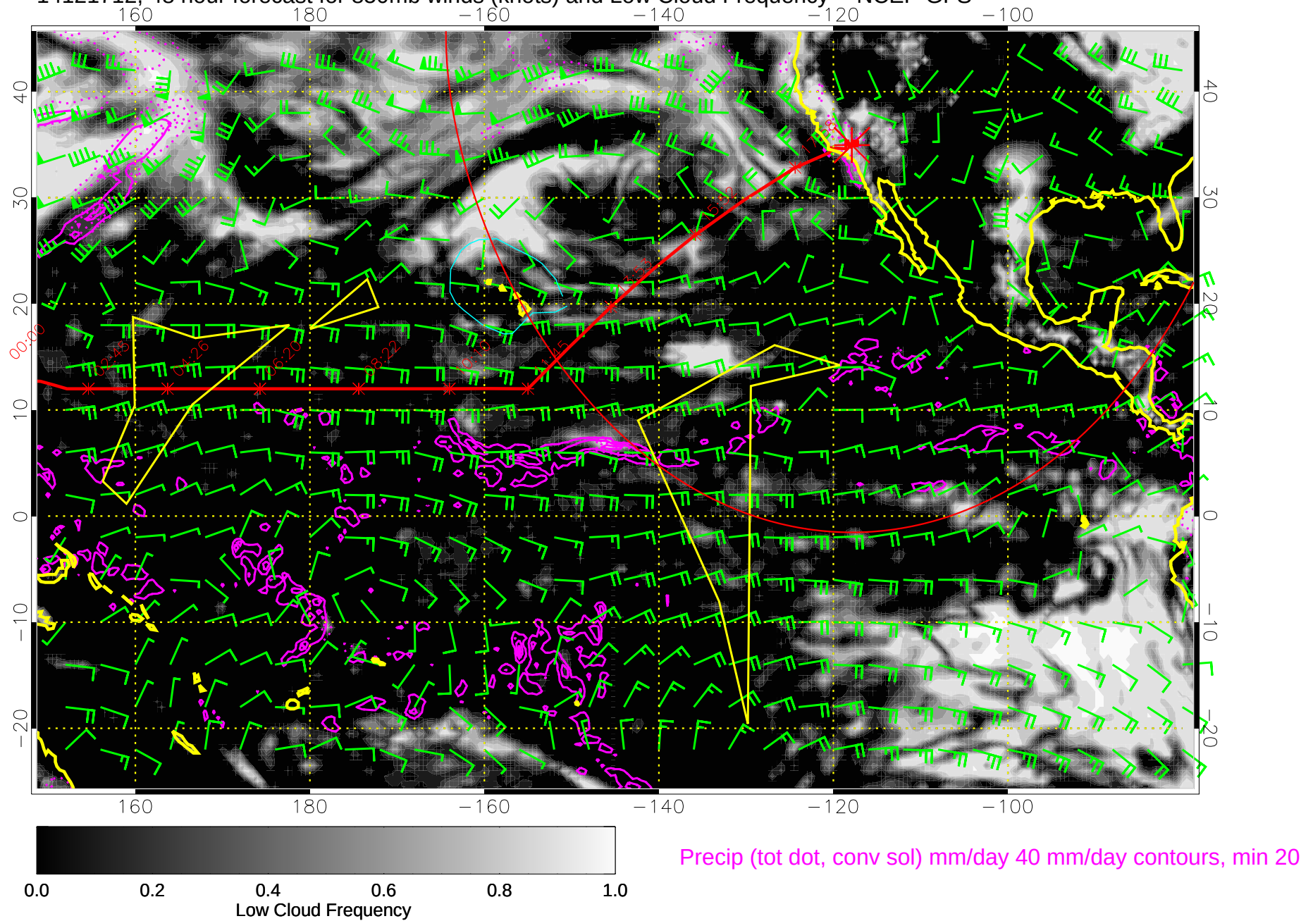
14121712, 48 hour forecast for 850mb winds (knots) and Low Cloud Frequency -- NCEP GFS
