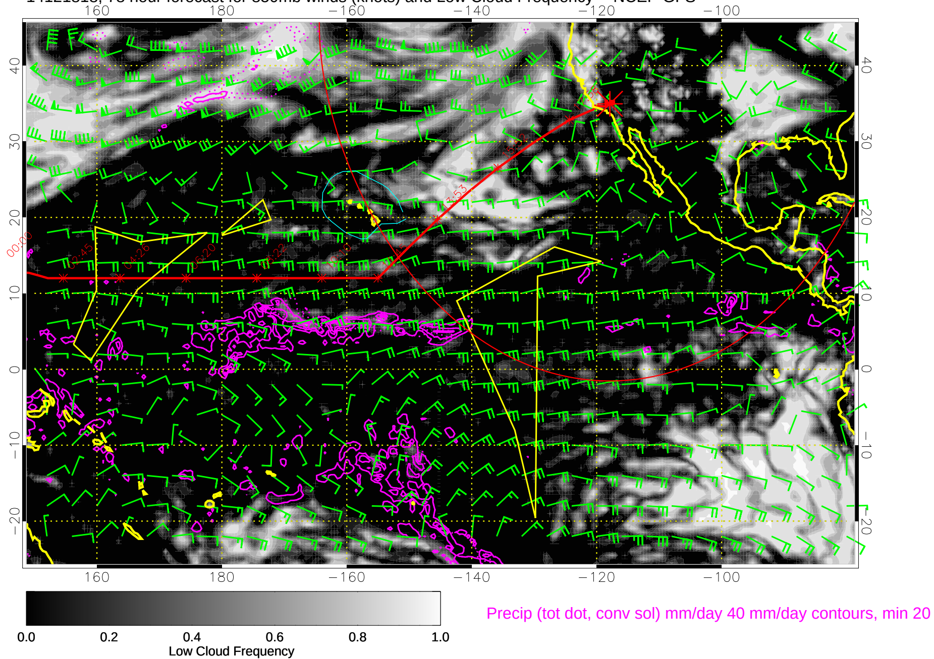
14121818, 78 hour forecast for 850mb winds (knots) and Low Cloud Frequency -- NCEP GFS
