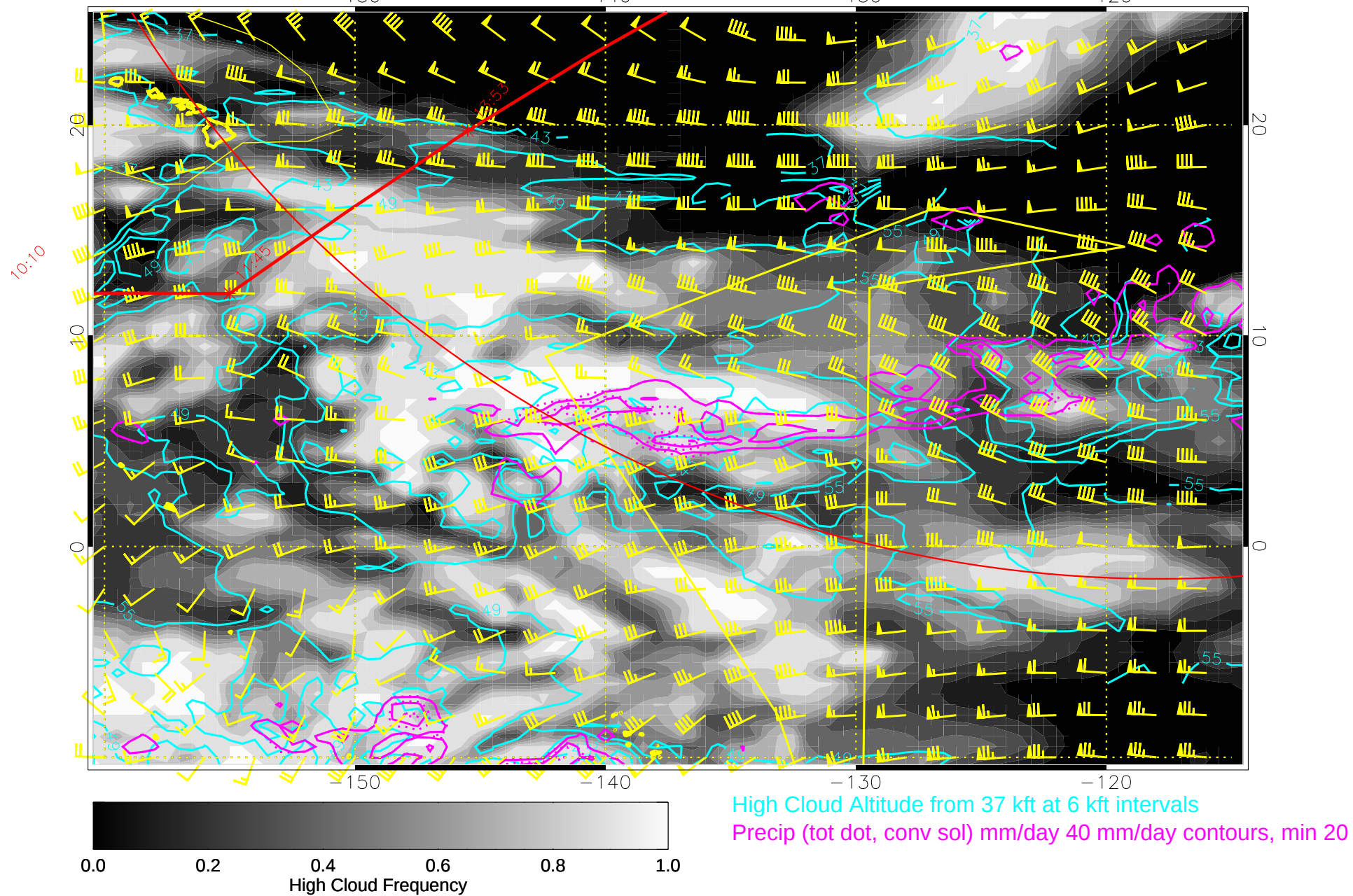
14121518, 6 hour forecast for 150mb winds (knots) and High Cloud Frequency -- NCEP GFS
