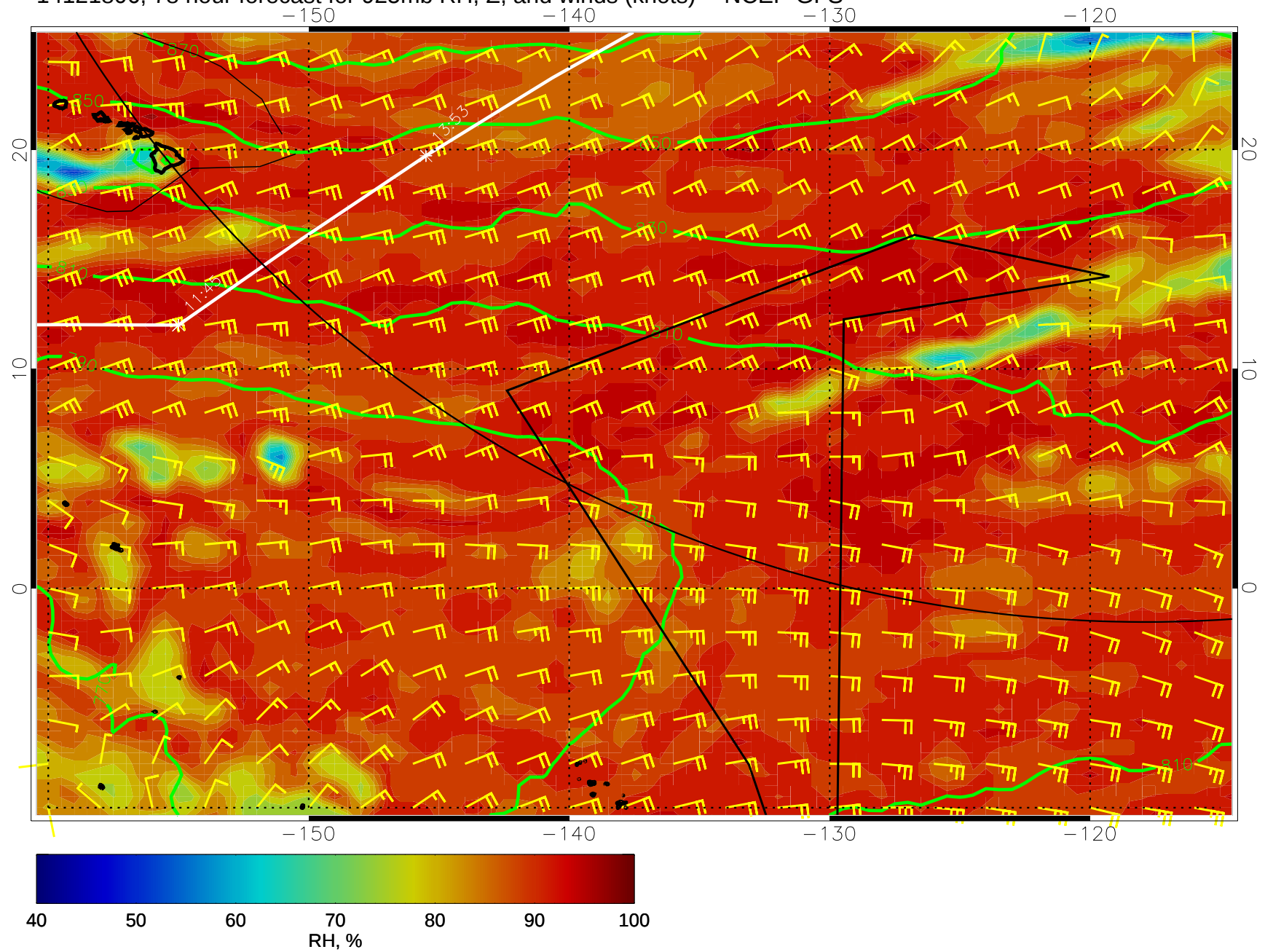
14121806, 78 hour forecast for 925mb RH, Z, and winds (knots) -- NCEP GFS
