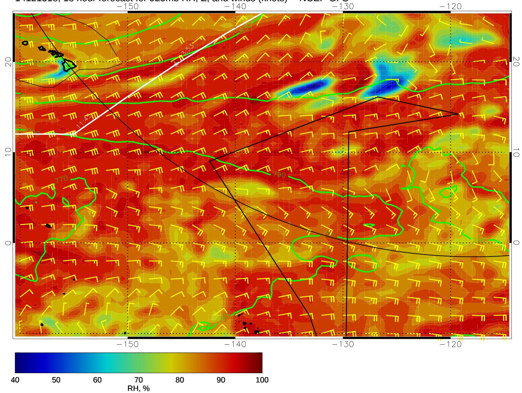
14121518, 18 hour forecast for 925mb RH, Z, and winds (knots) -- NCEP GFS
