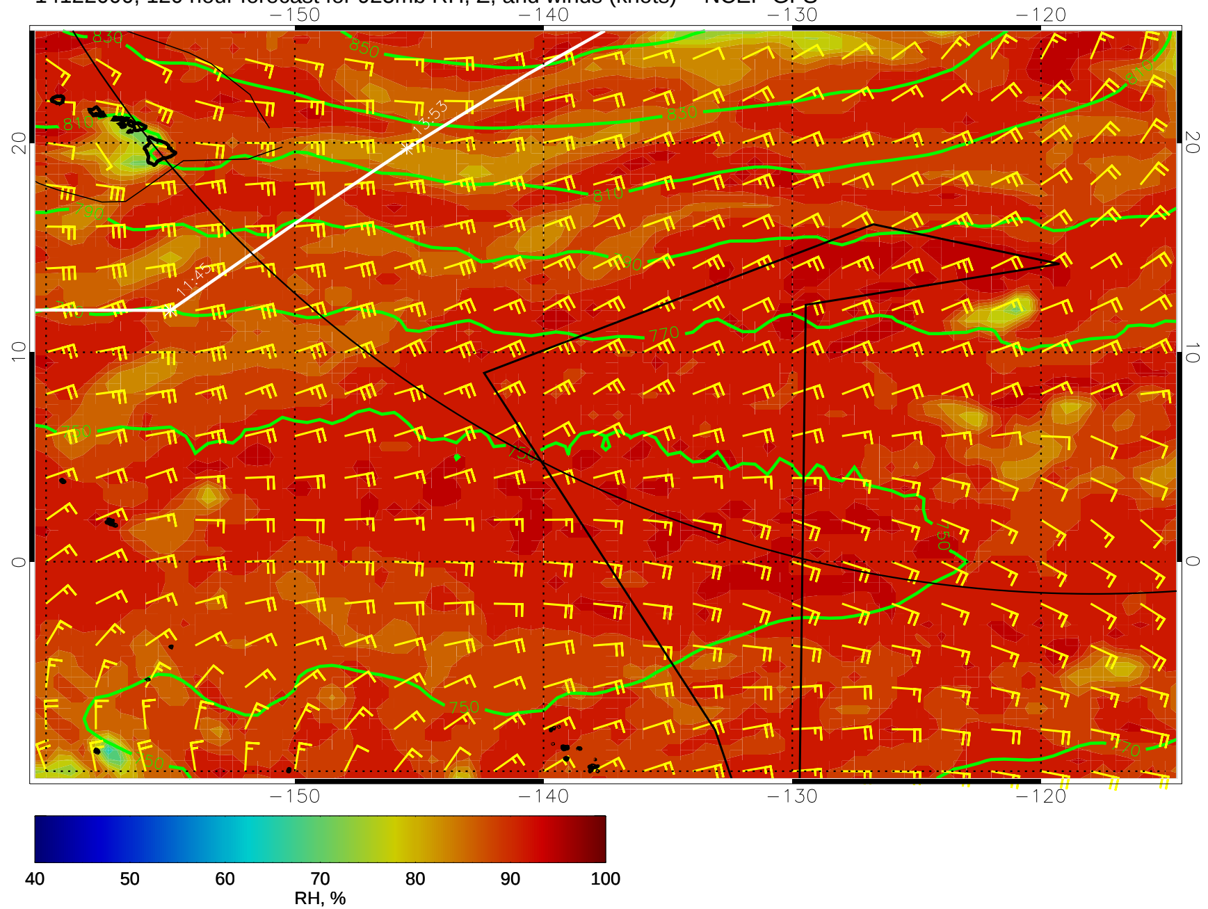
14122000, 120 hour forecast for 925mb RH, Z, and winds (knots) -- NCEP GFS
