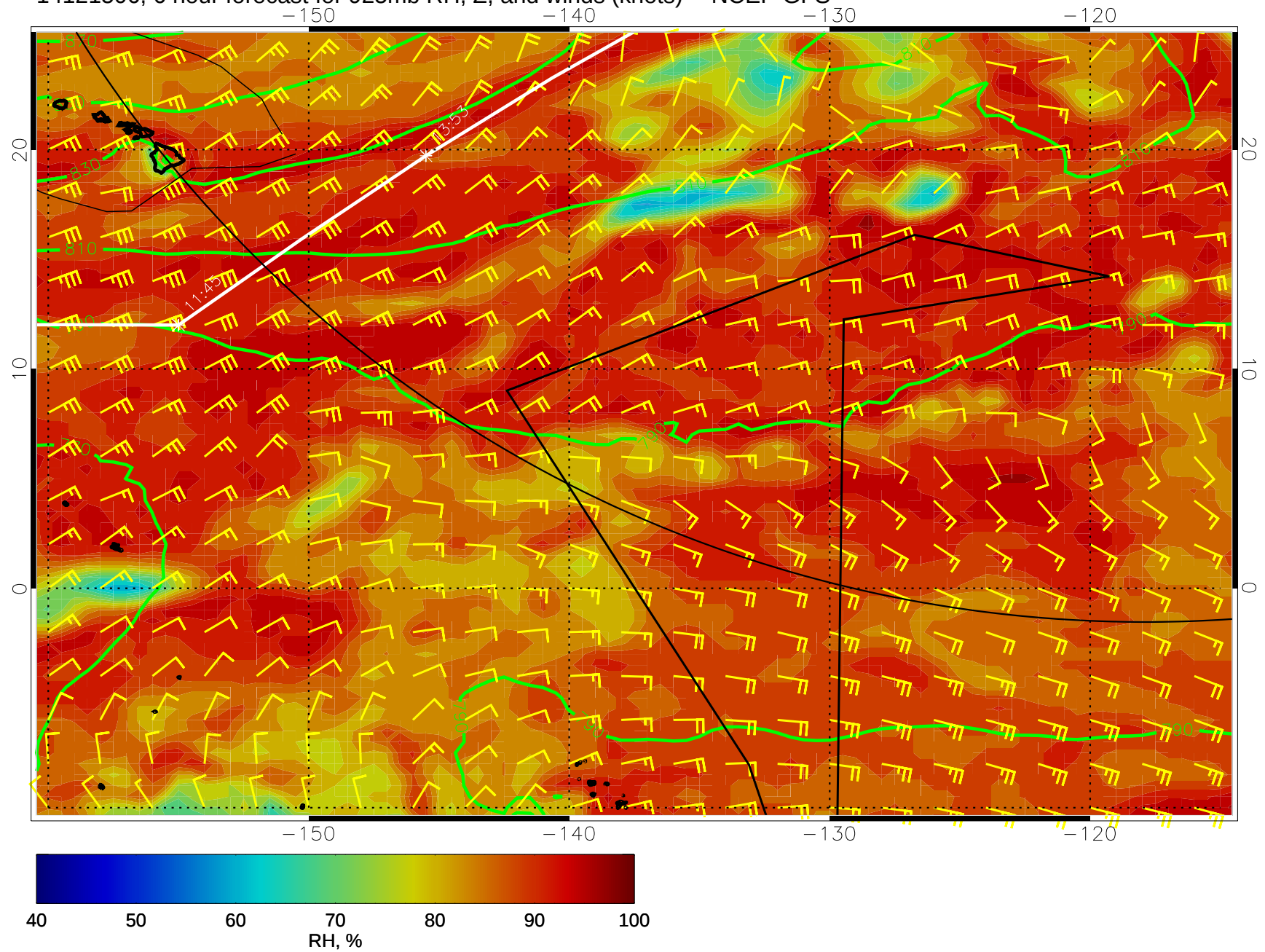
14121506, 6 hour forecast for 925mb RH, Z, and winds (knots) -- NCEP GFS
