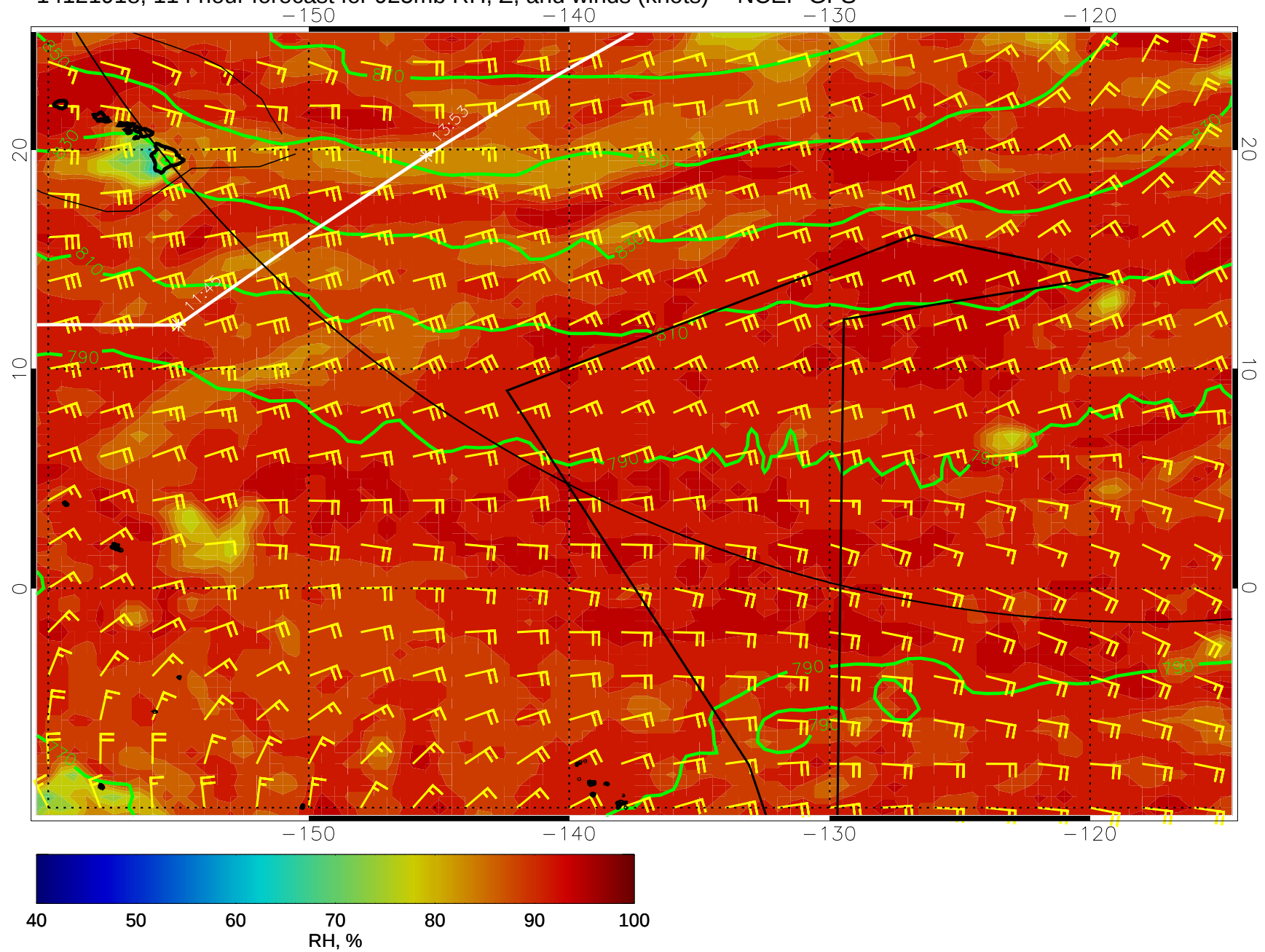
14121918, 114 hour forecast for 925mb RH, Z, and winds (knots) -- NCEP GFS
