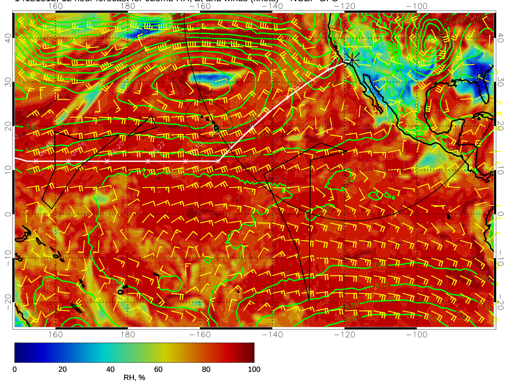
14121512, 12 hour forecast for 925mb RH, Z, and winds (knots) -- NCEP GFS
