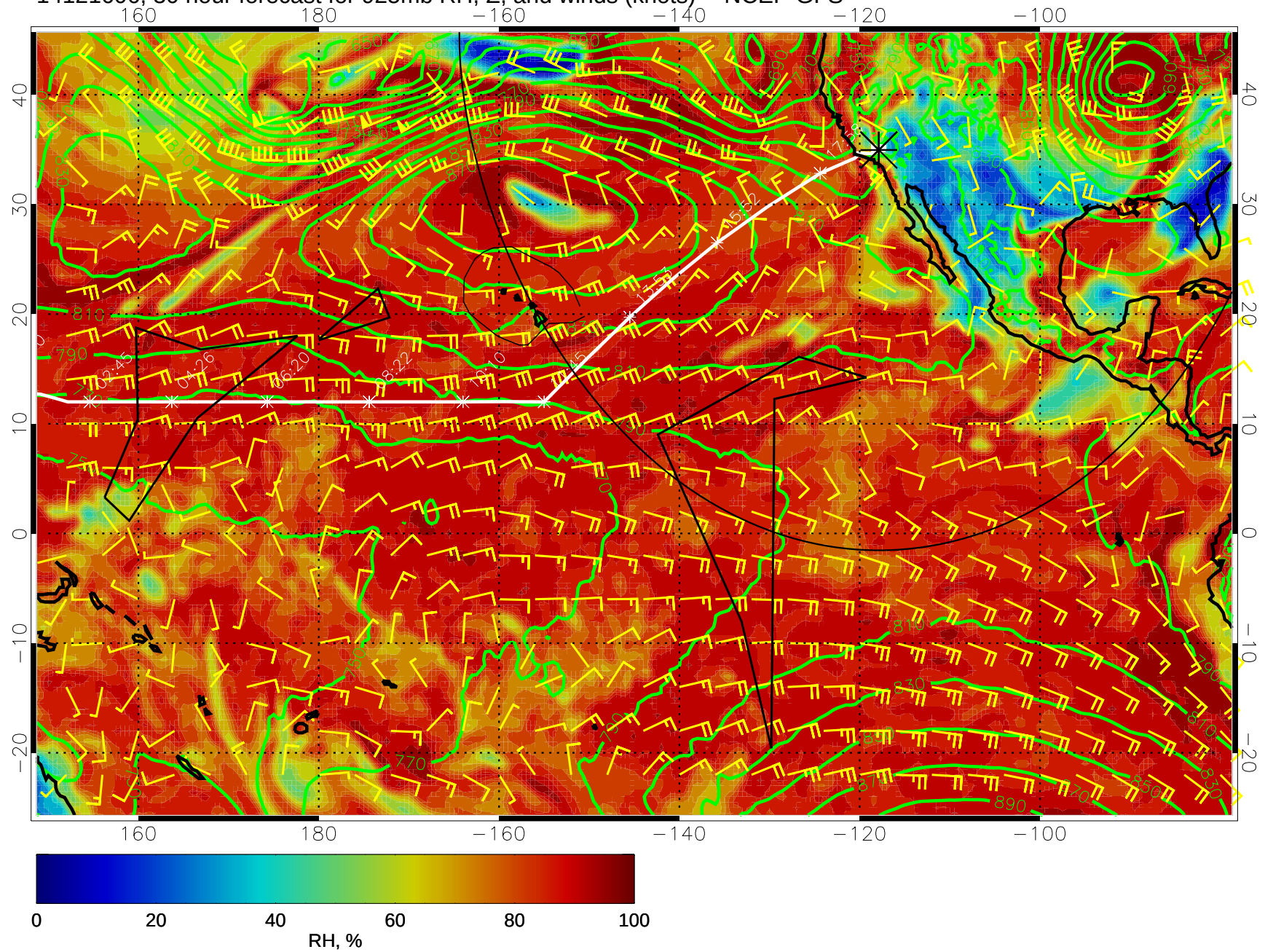
14121606, 30 hour forecast for 925mb RH, Z, and winds (knots) -- NCEP GFS
