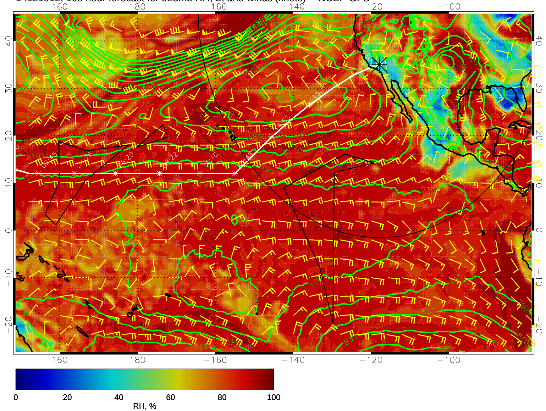
14121912, 108 hour forecast for 925mb RH, Z, and winds (knots) -- NCEP GFS
