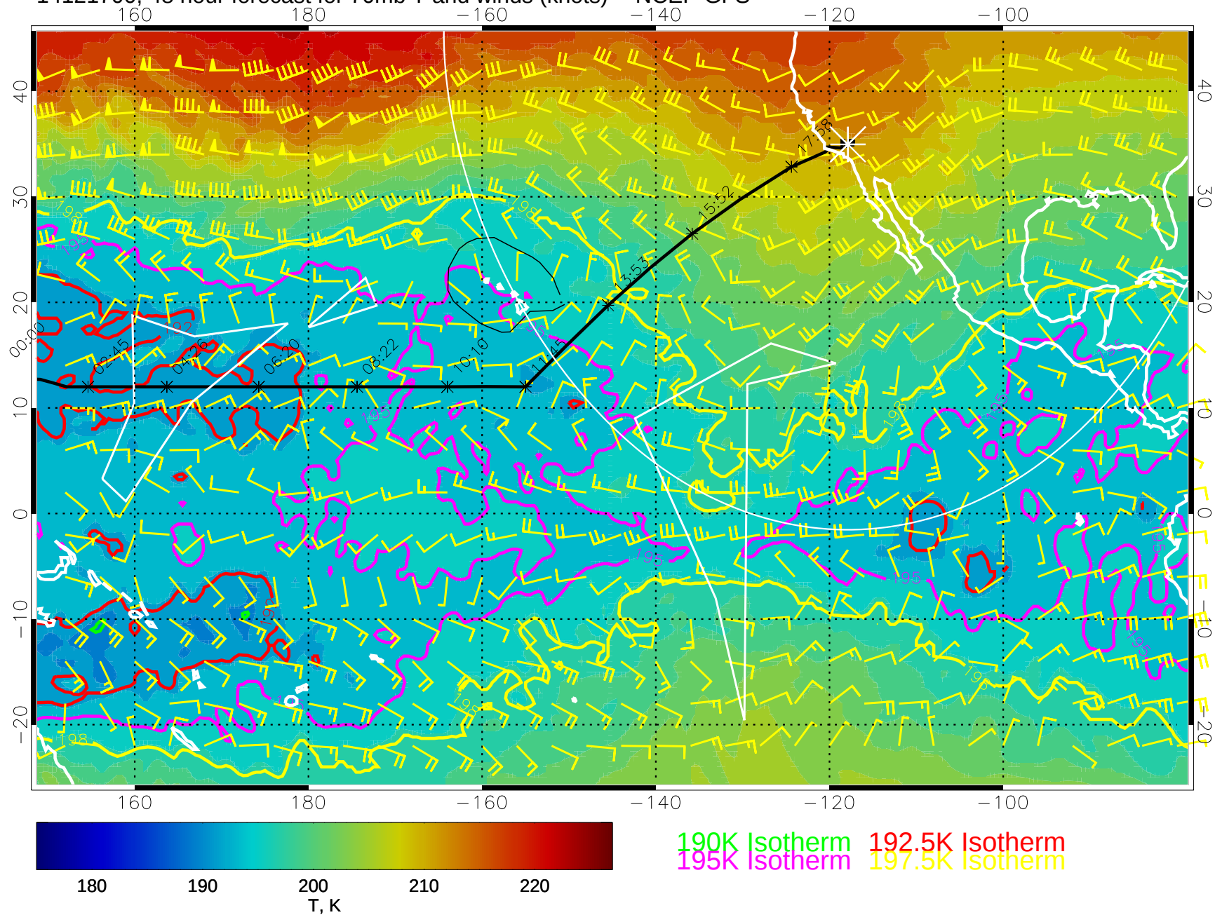
14121700, 48 hour forecast for 70mb T and winds (knots) -- NCEP GFS
