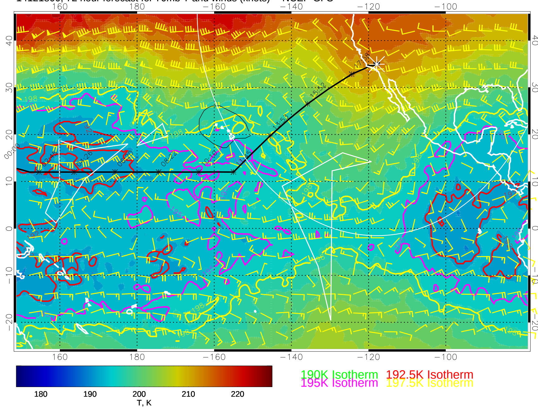
14121800, 72 hour forecast for 70mb T and winds (knots) -- NCEP GFS
