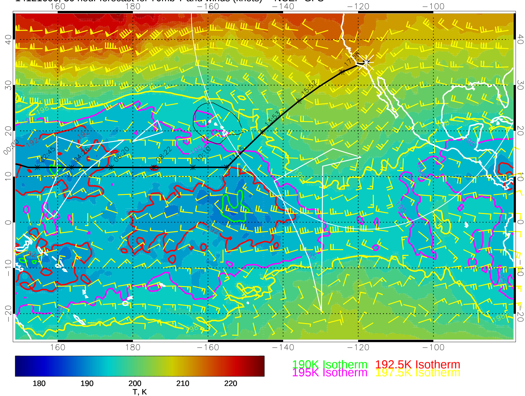
14121606, 30 hour forecast for 70mb T and winds (knots) -- NCEP GFS
