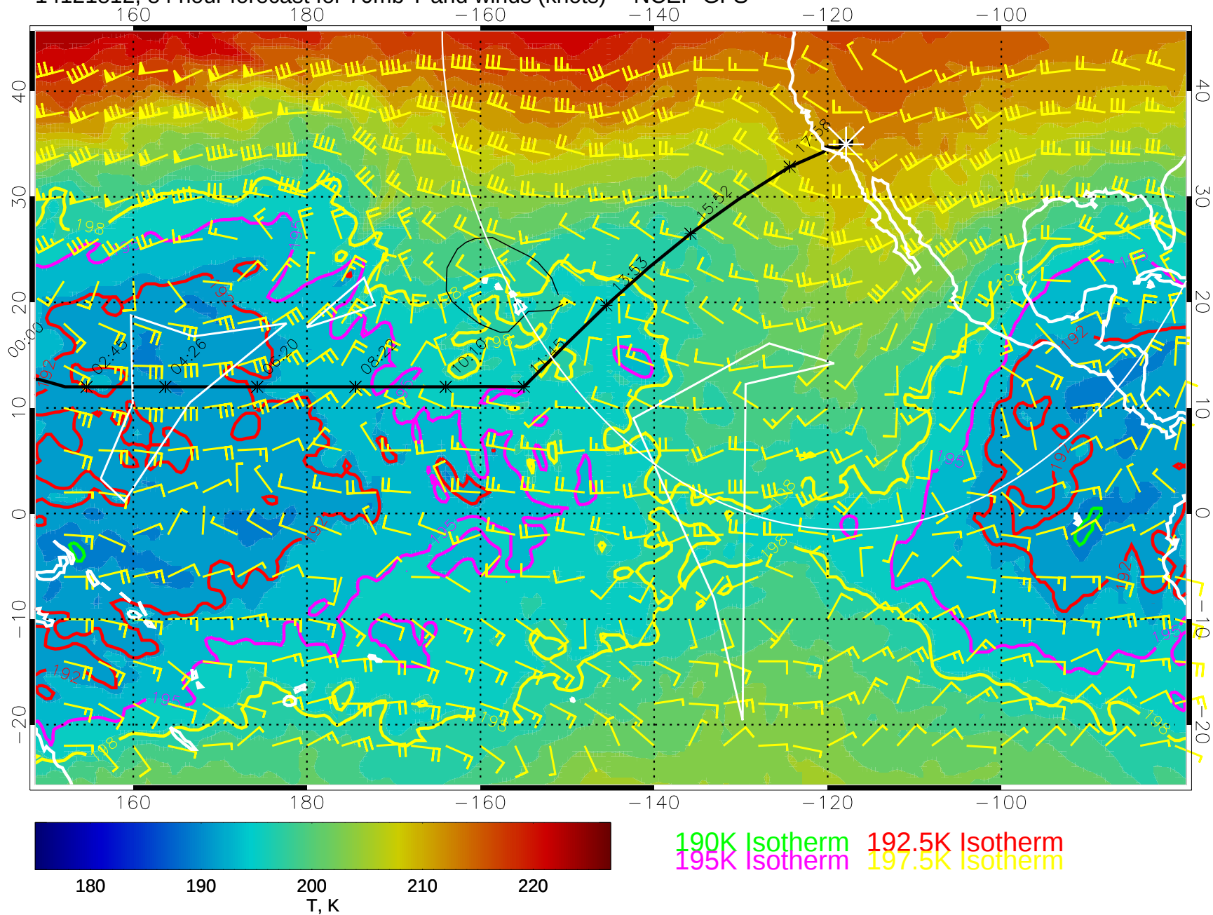
14121812, 84 hour forecast for 70mb T and winds (knots) -- NCEP GFS
