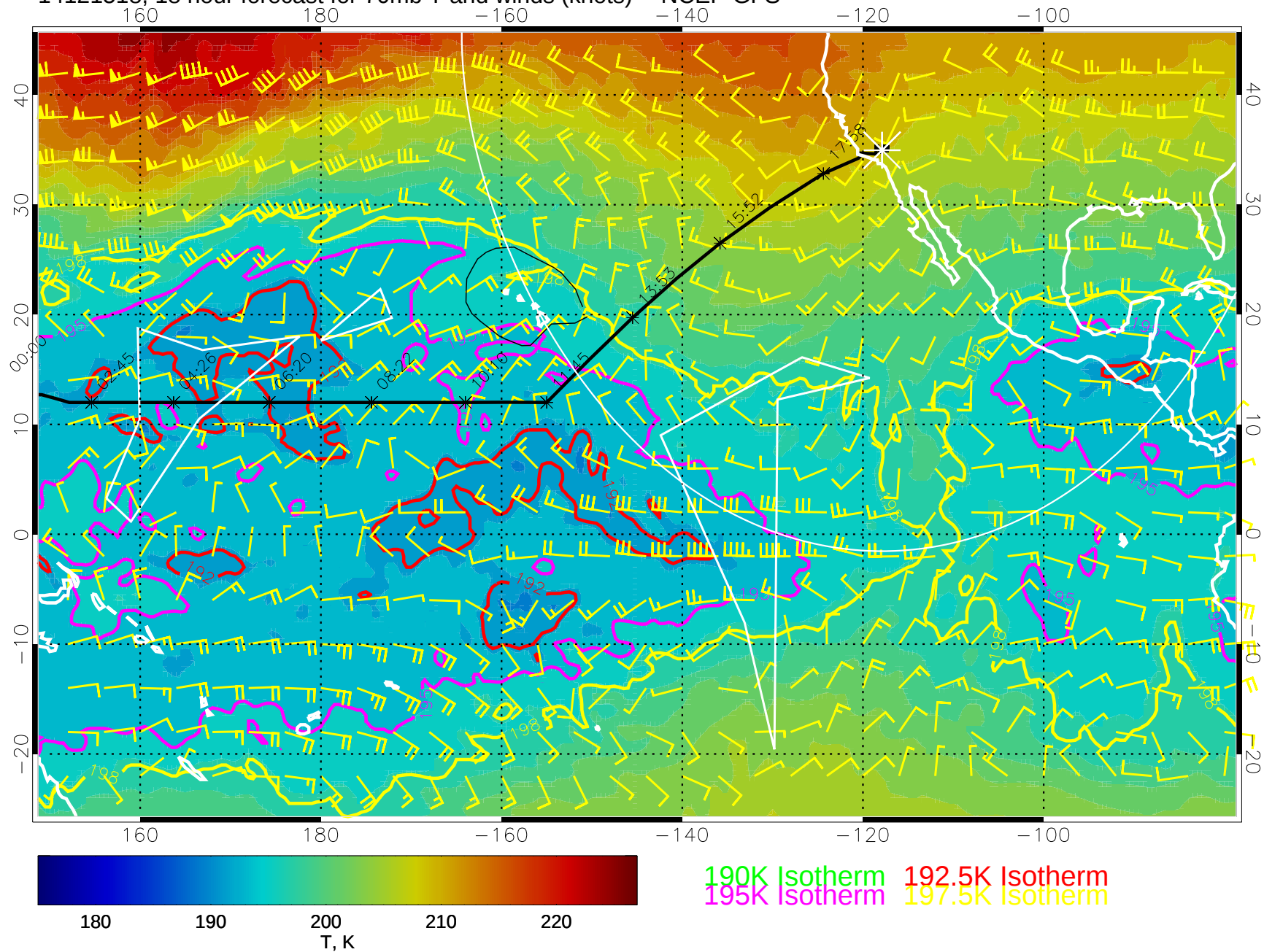
14121518, 18 hour forecast for 70mb T and winds (knots) -- NCEP GFS
