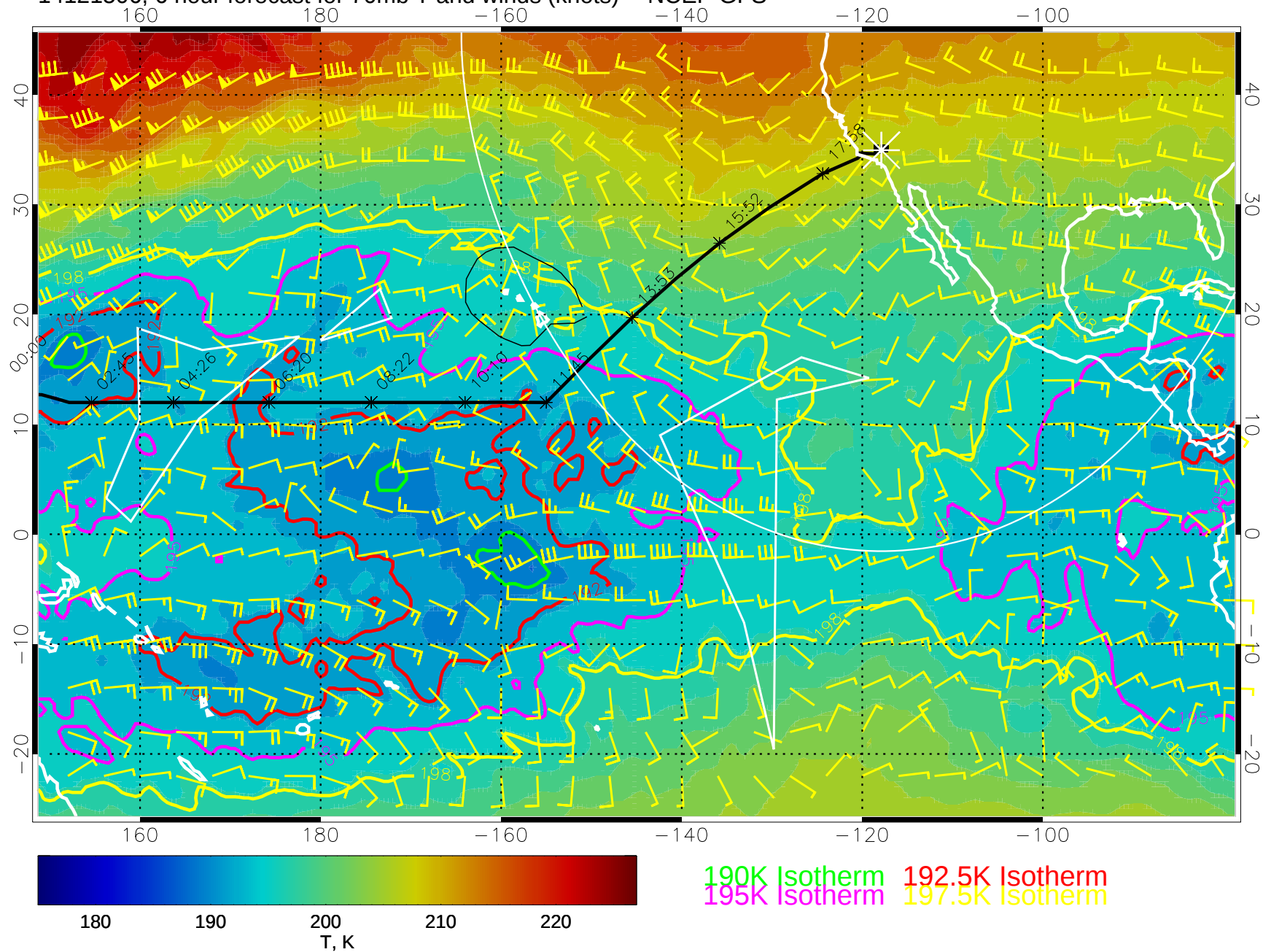
14121506, 6 hour forecast for 70mb T and winds (knots) -- NCEP GFS
