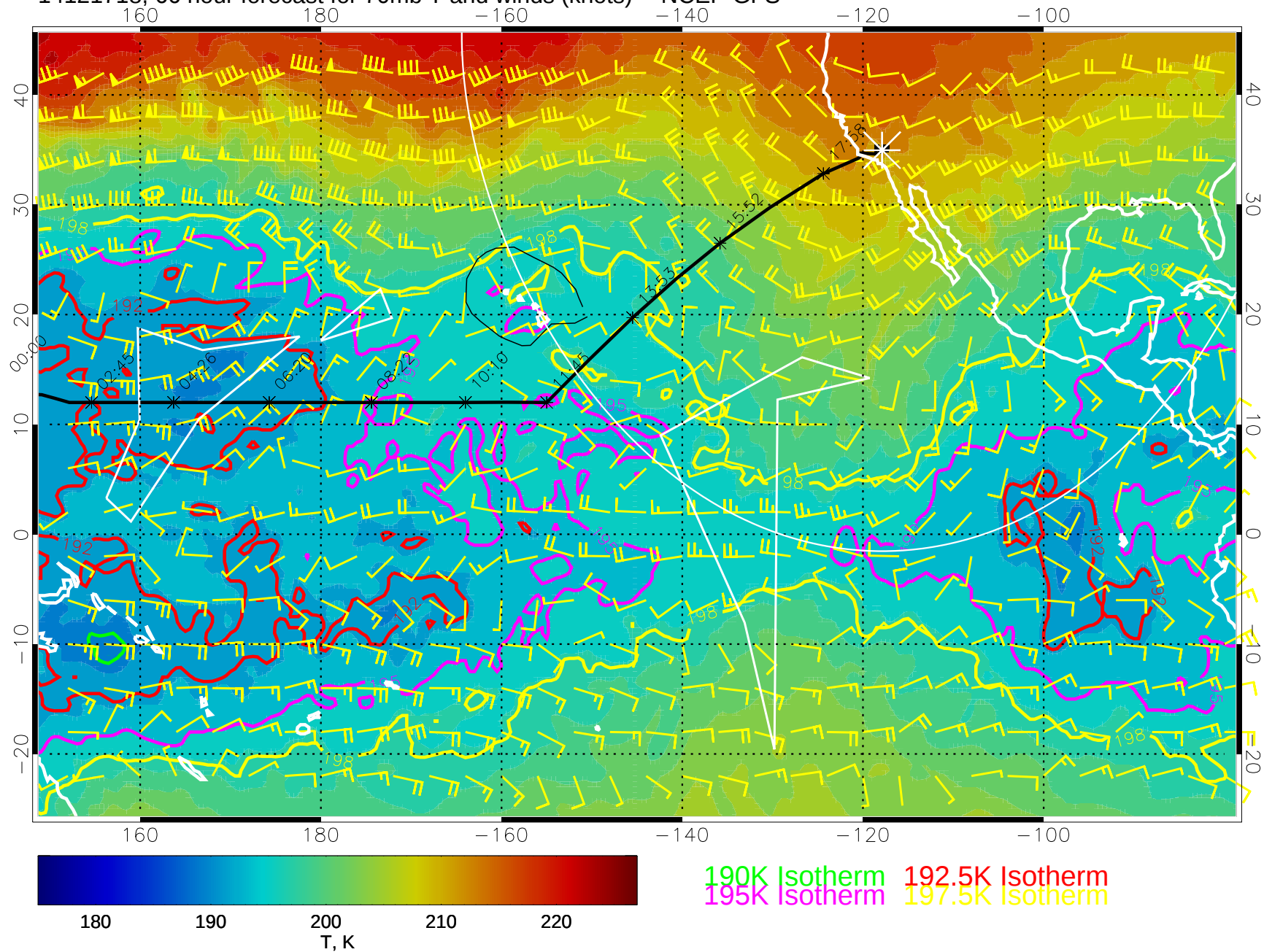
14121718, 66 hour forecast for 70mb T and winds (knots) -- NCEP GFS
