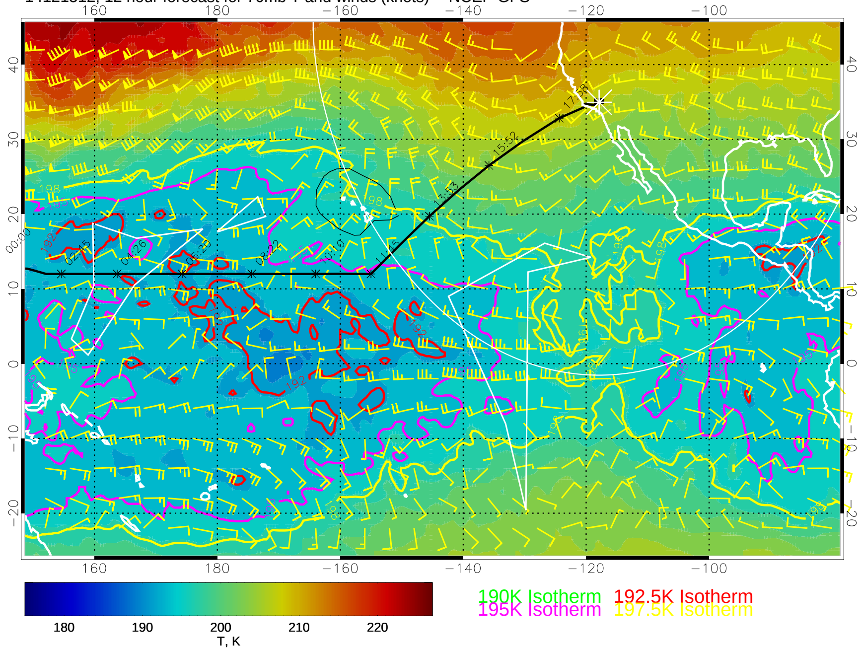
14121512, 12 hour forecast for 70mb T and winds (knots) -- NCEP GFS
