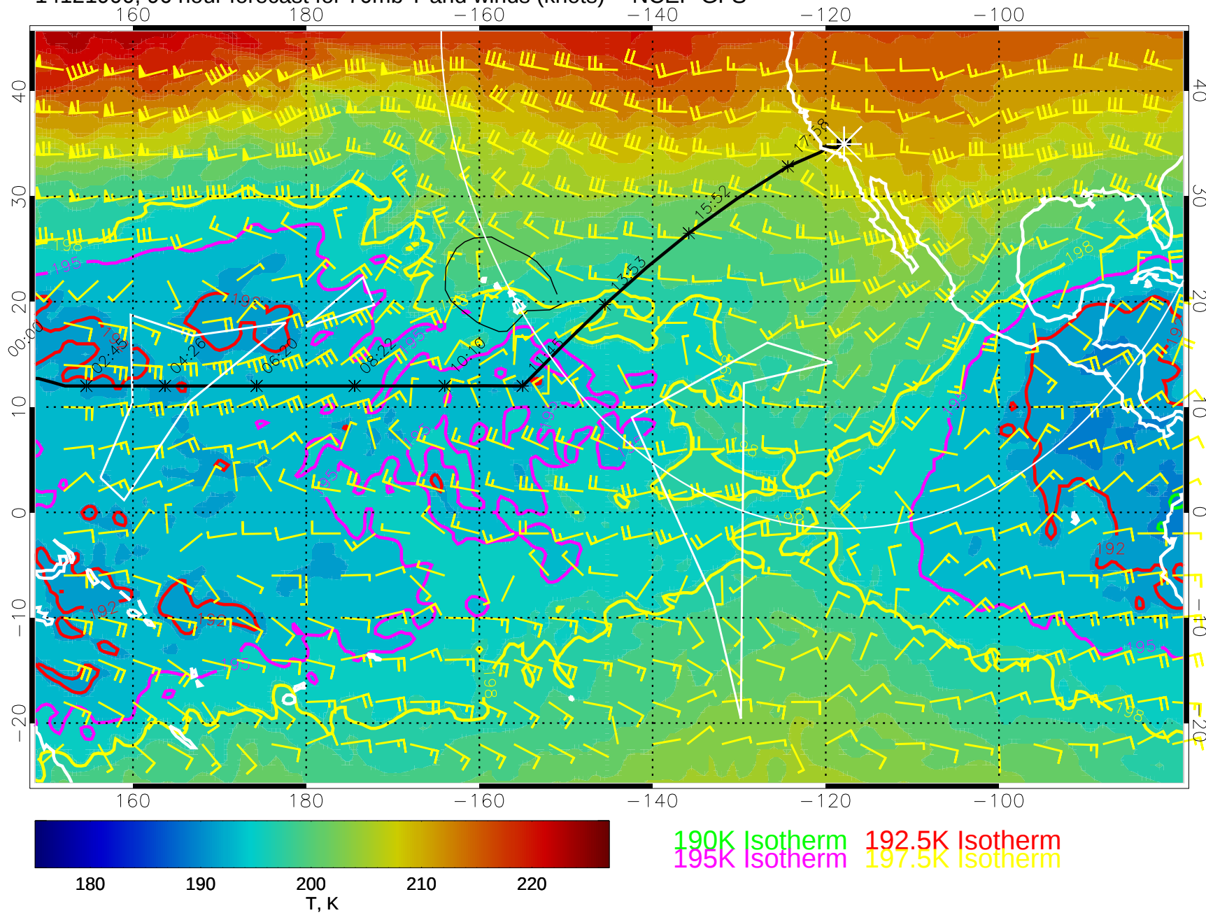
14121900, 96 hour forecast for 70mb T and winds (knots) -- NCEP GFS
