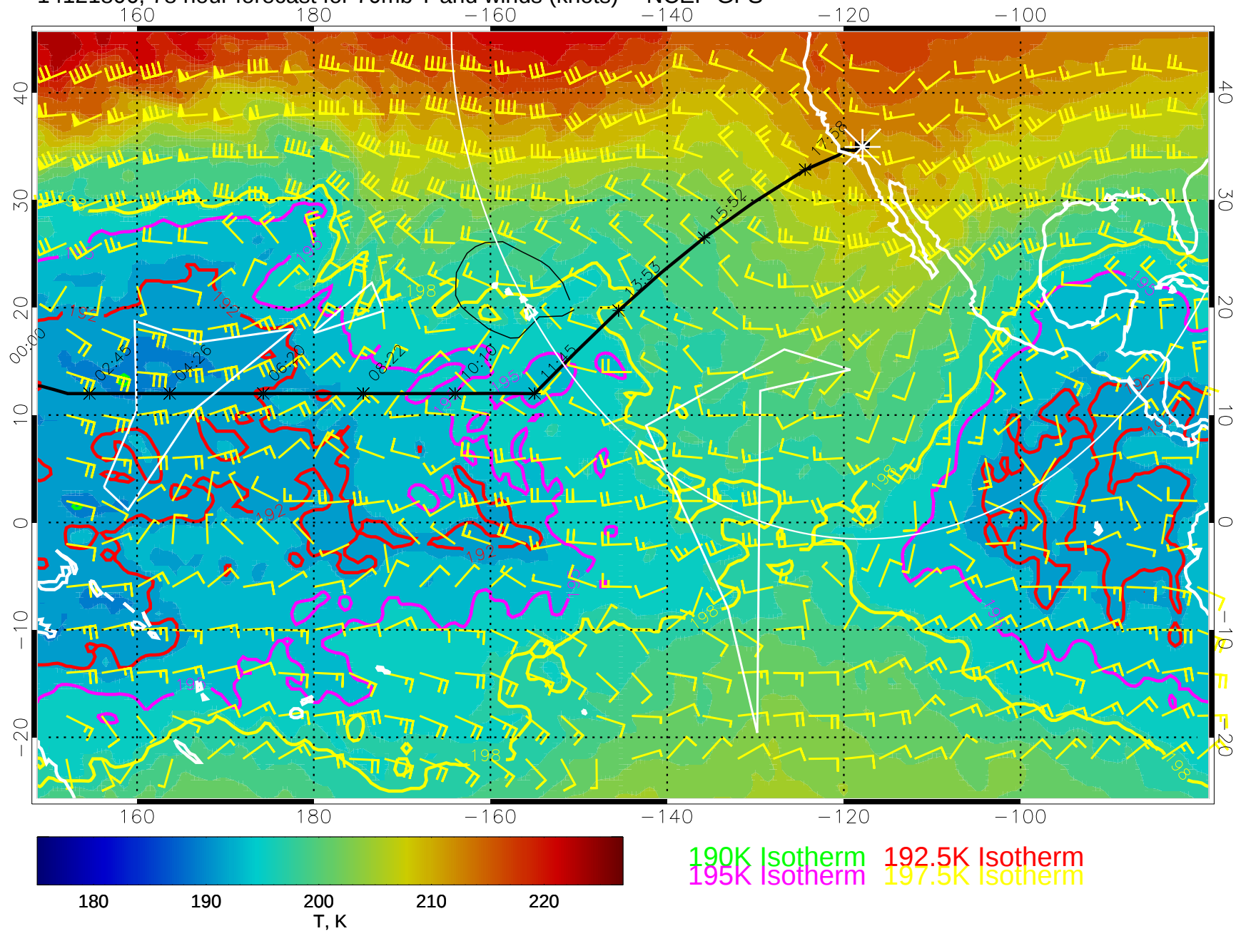
14121806, 78 hour forecast for 70mb T and winds (knots) -- NCEP GFS
