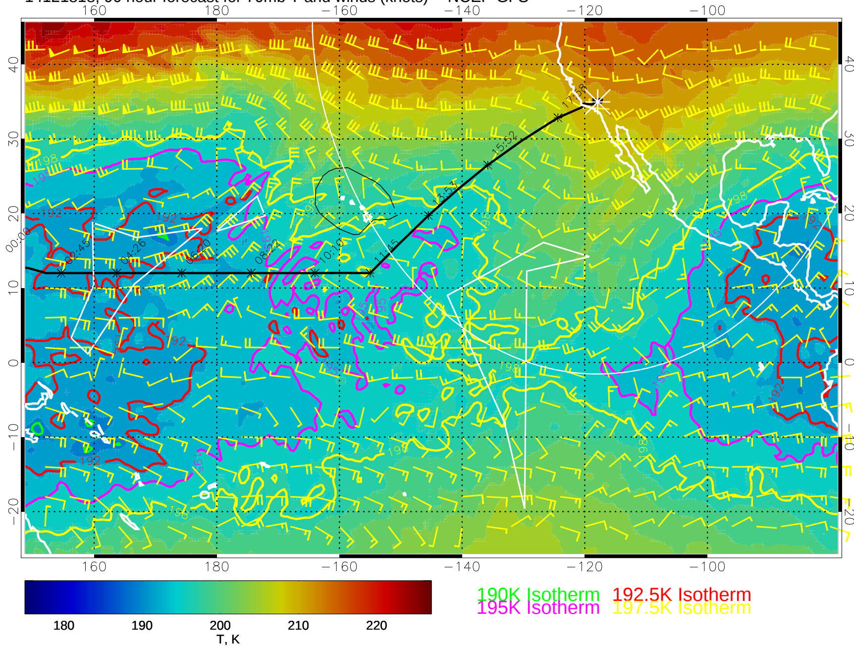
14121818, 90 hour forecast for 70mb T and winds (knots) -- NCEP GFS
