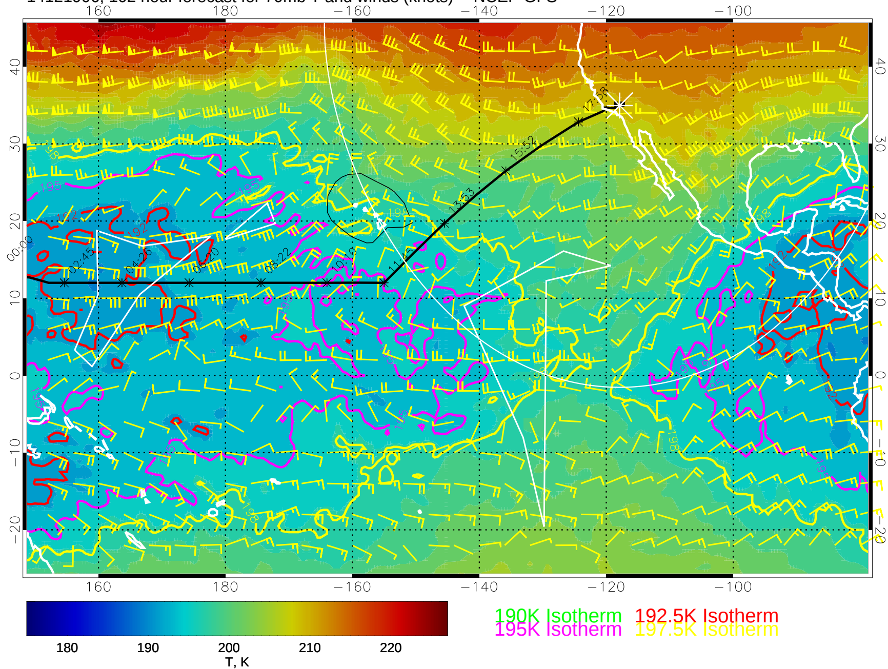
14121906, 102 hour forecast for 70mb T and winds (knots) -- NCEP GFS
