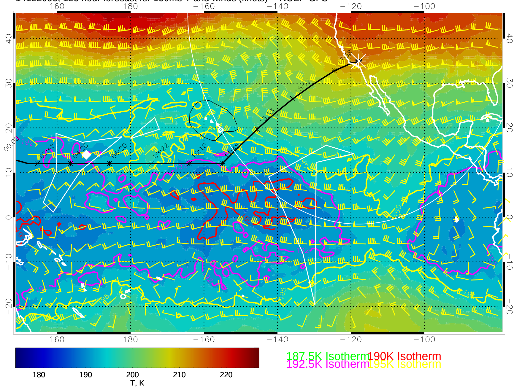
14122000, 120 hour forecast for 100mb T and winds (knots) -- NCEP GFS
