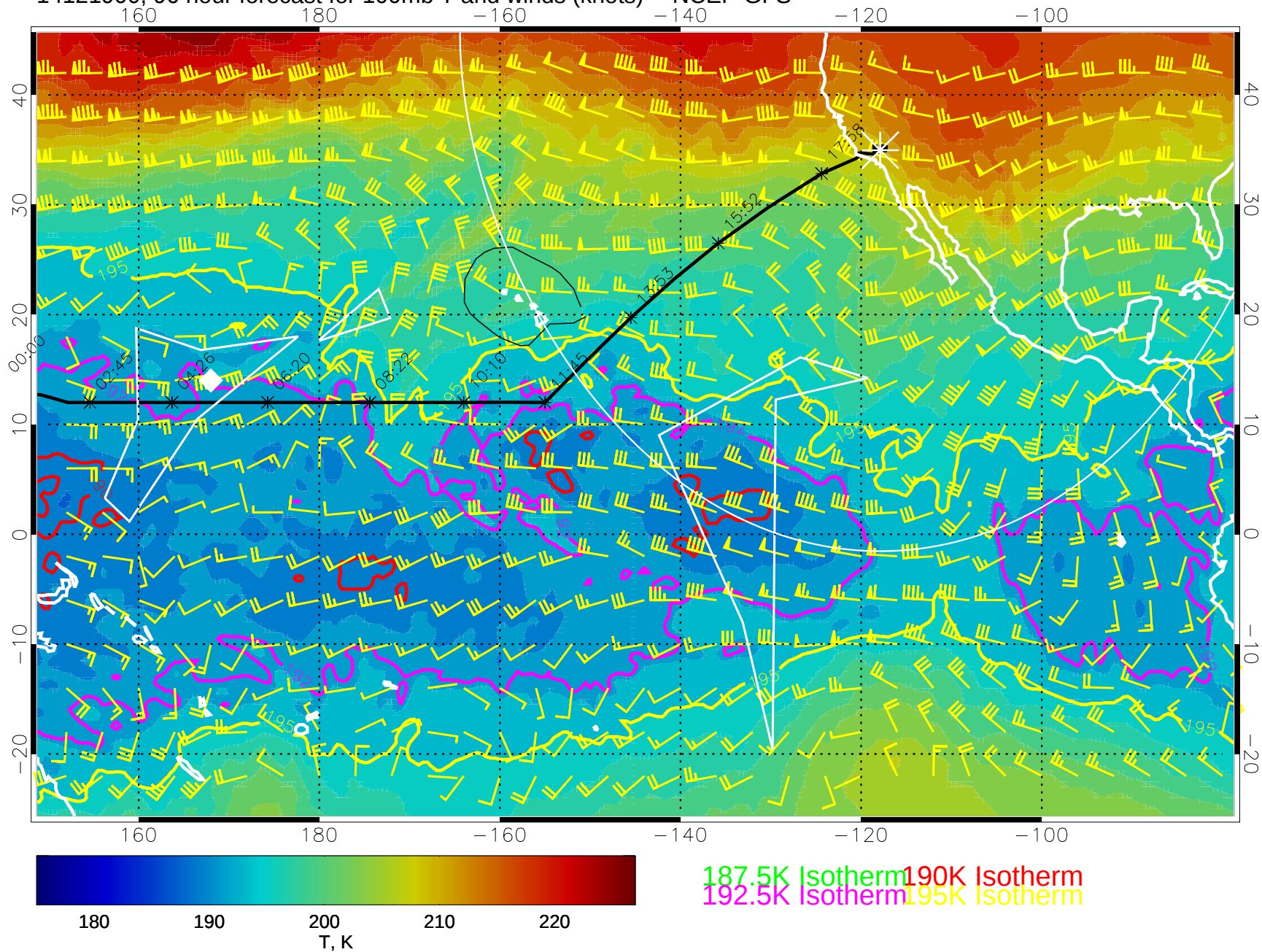
14121900, 96 hour forecast for 100mb T and winds (knots) -- NCEP GFS
