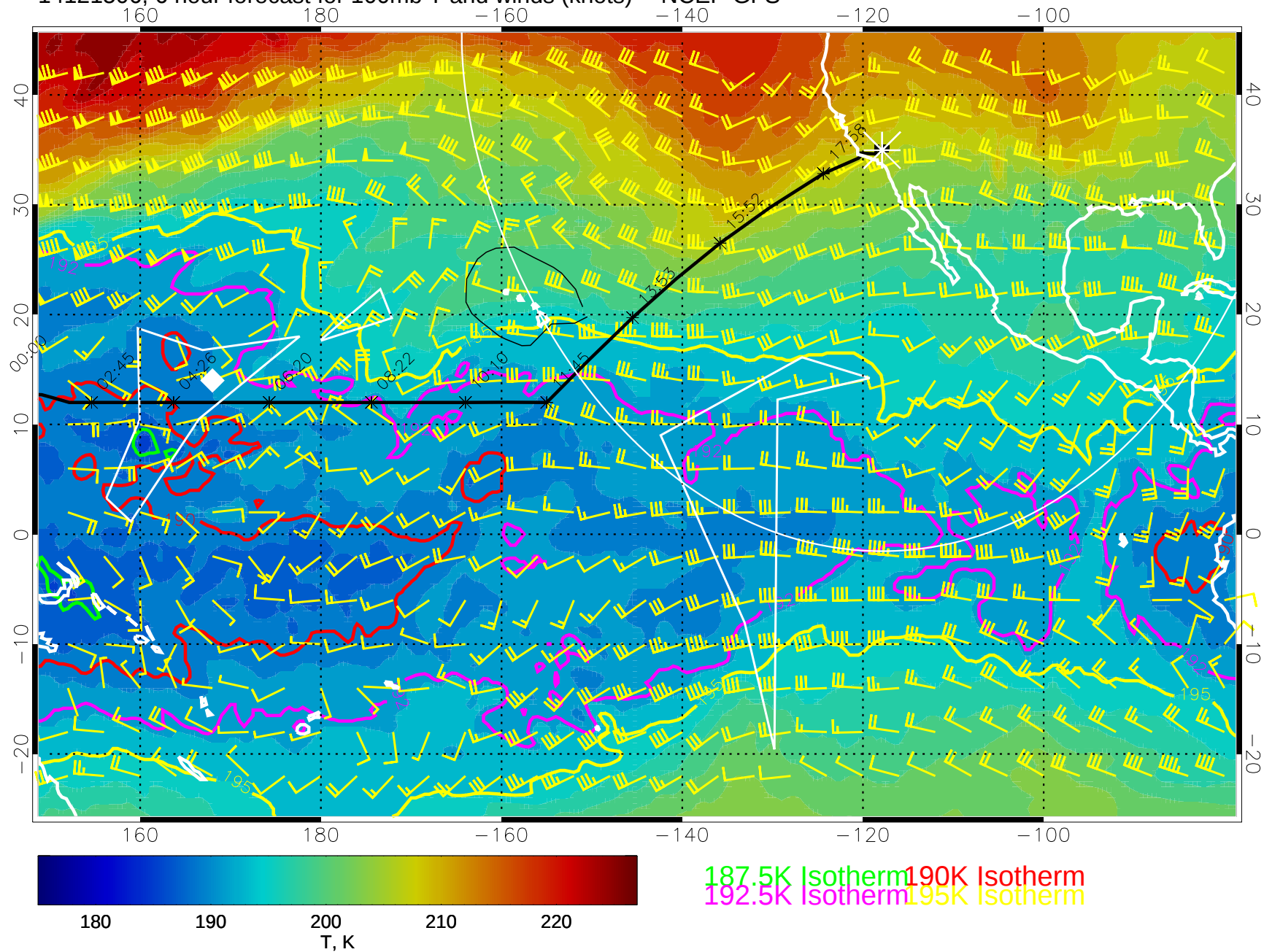
14121506, 6 hour forecast for 100mb T and winds (knots) -- NCEP GFS
