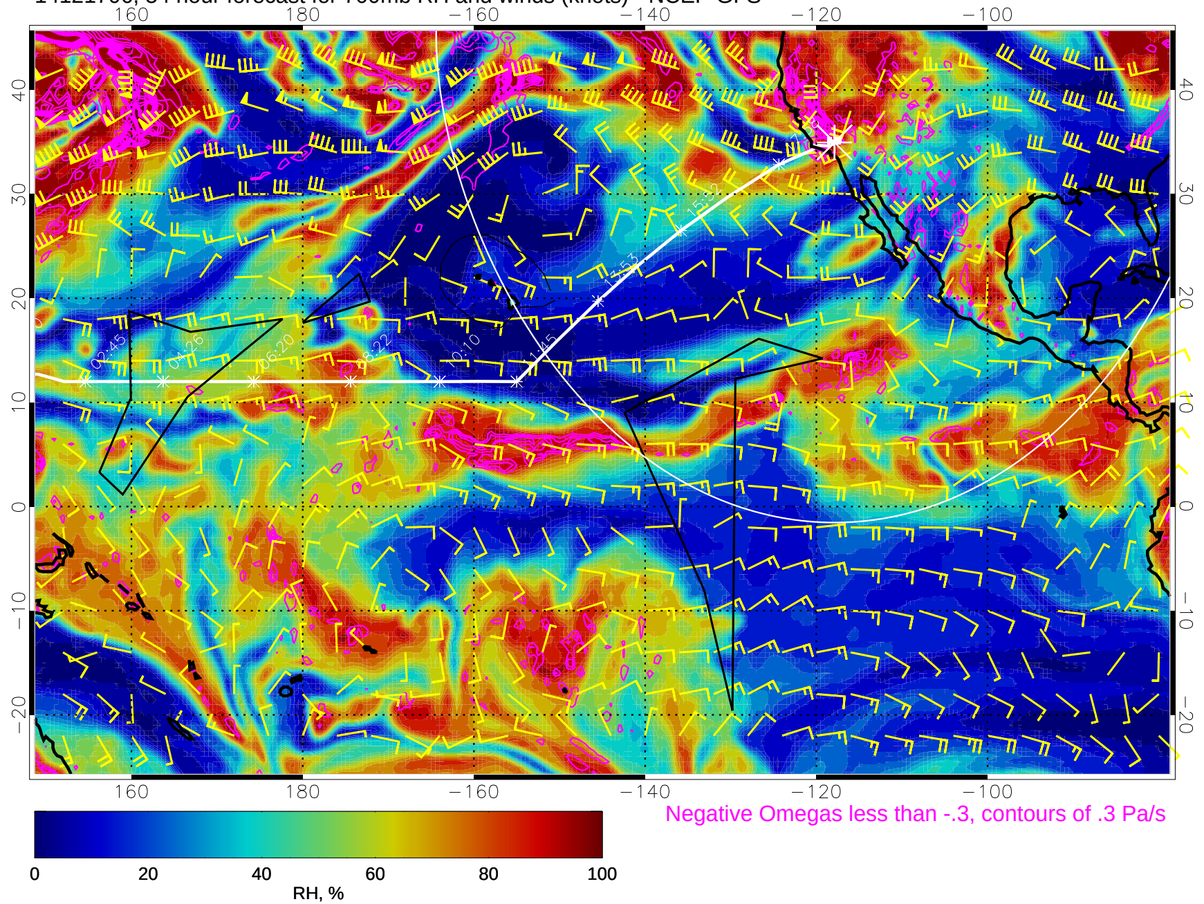
14121706, 54 hour forecast for 700mb RH and winds (knots) - NCEP GFS
