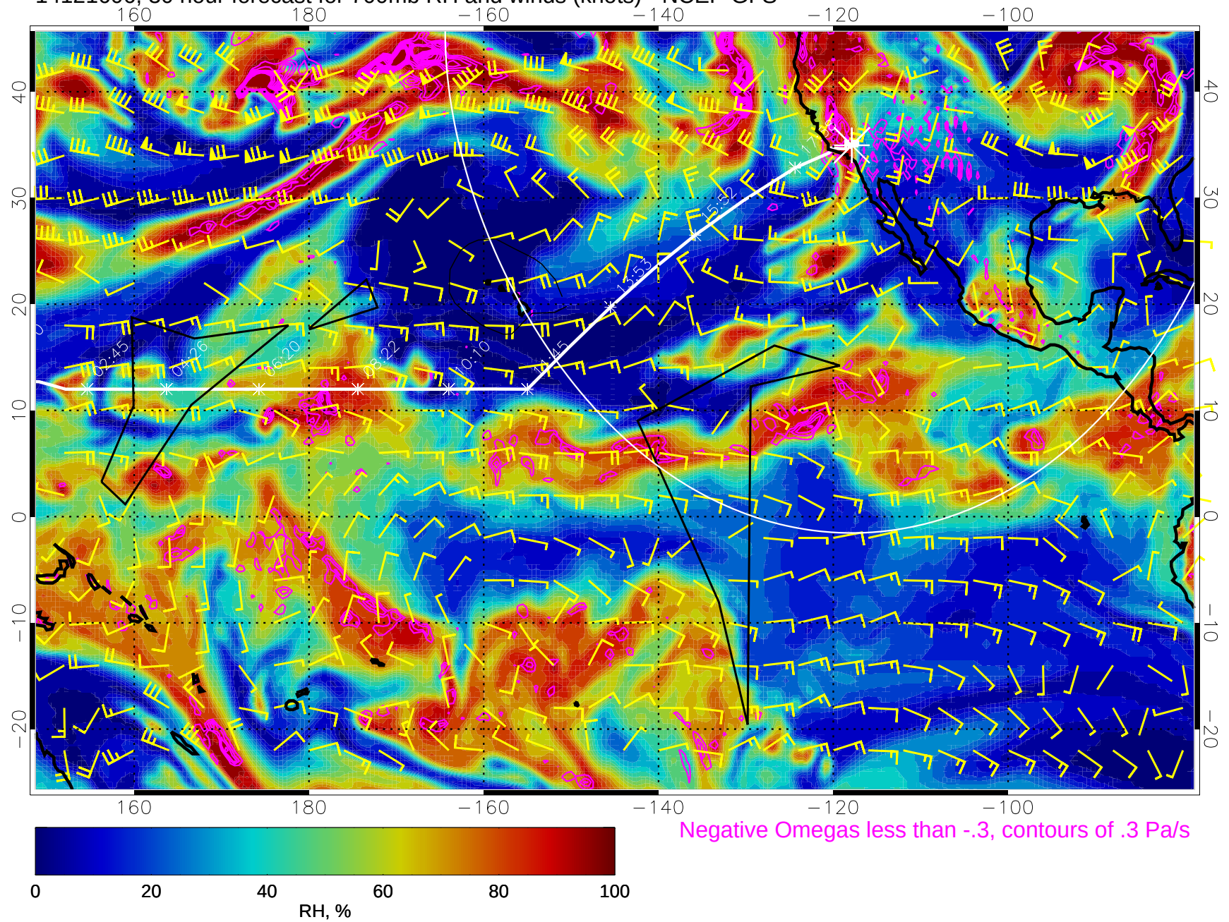
14121606, 30 hour forecast for 700mb RH and winds (knots) - NCEP GFS
