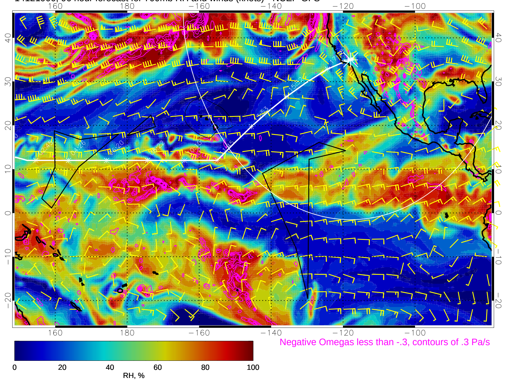
14121900, 96 hour forecast for 700mb RH and winds (knots) - NCEP GFS
