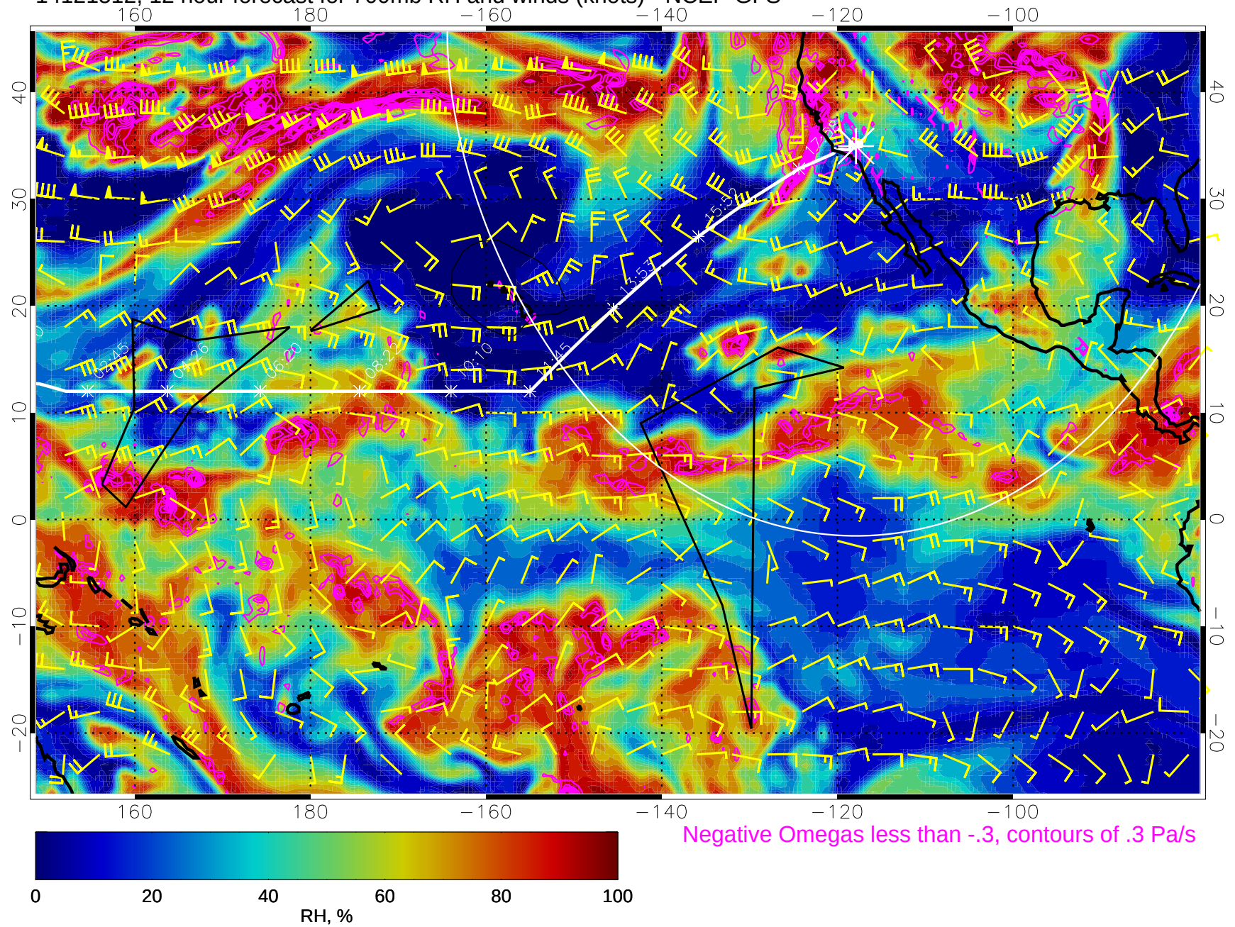
14121512, 12 hour forecast for 700mb RH and winds (knots) - NCEP GFS
