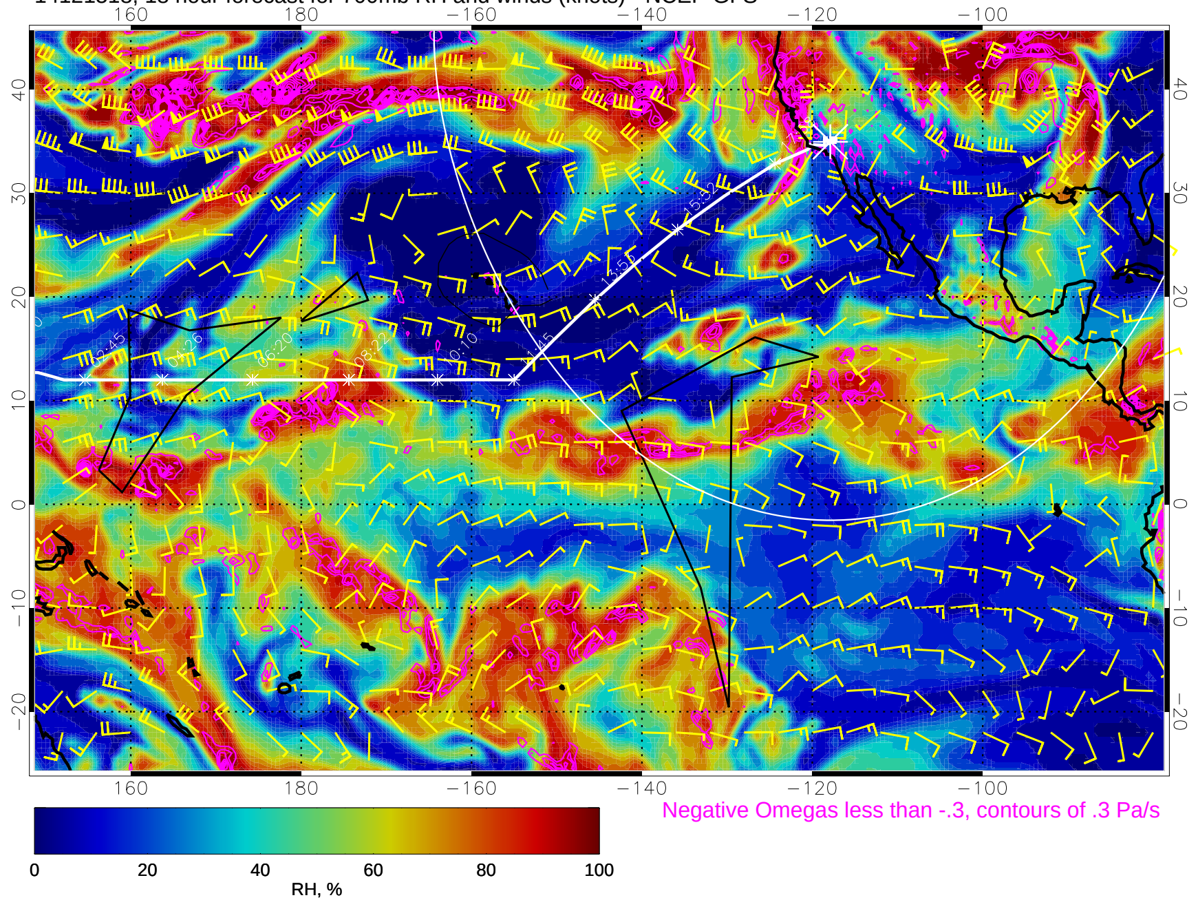
14121518, 18 hour forecast for 700mb RH and winds (knots) - NCEP GFS
