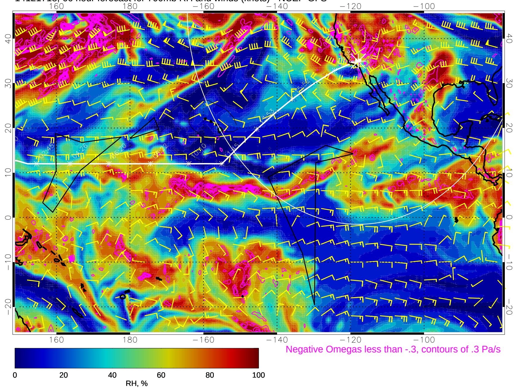
14121718, 66 hour forecast for 700mb RH and winds (knots) - NCEP GFS
