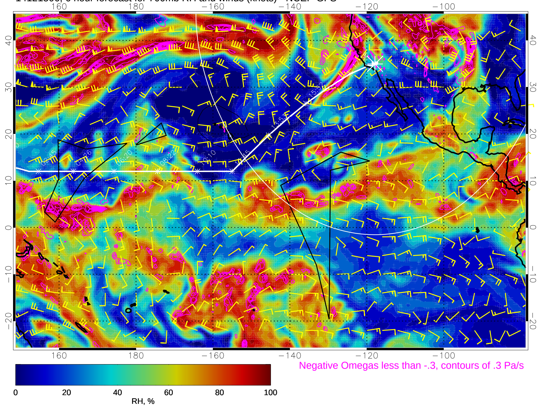
14121506, 6 hour forecast for 700mb RH and winds (knots) - NCEP GFS
