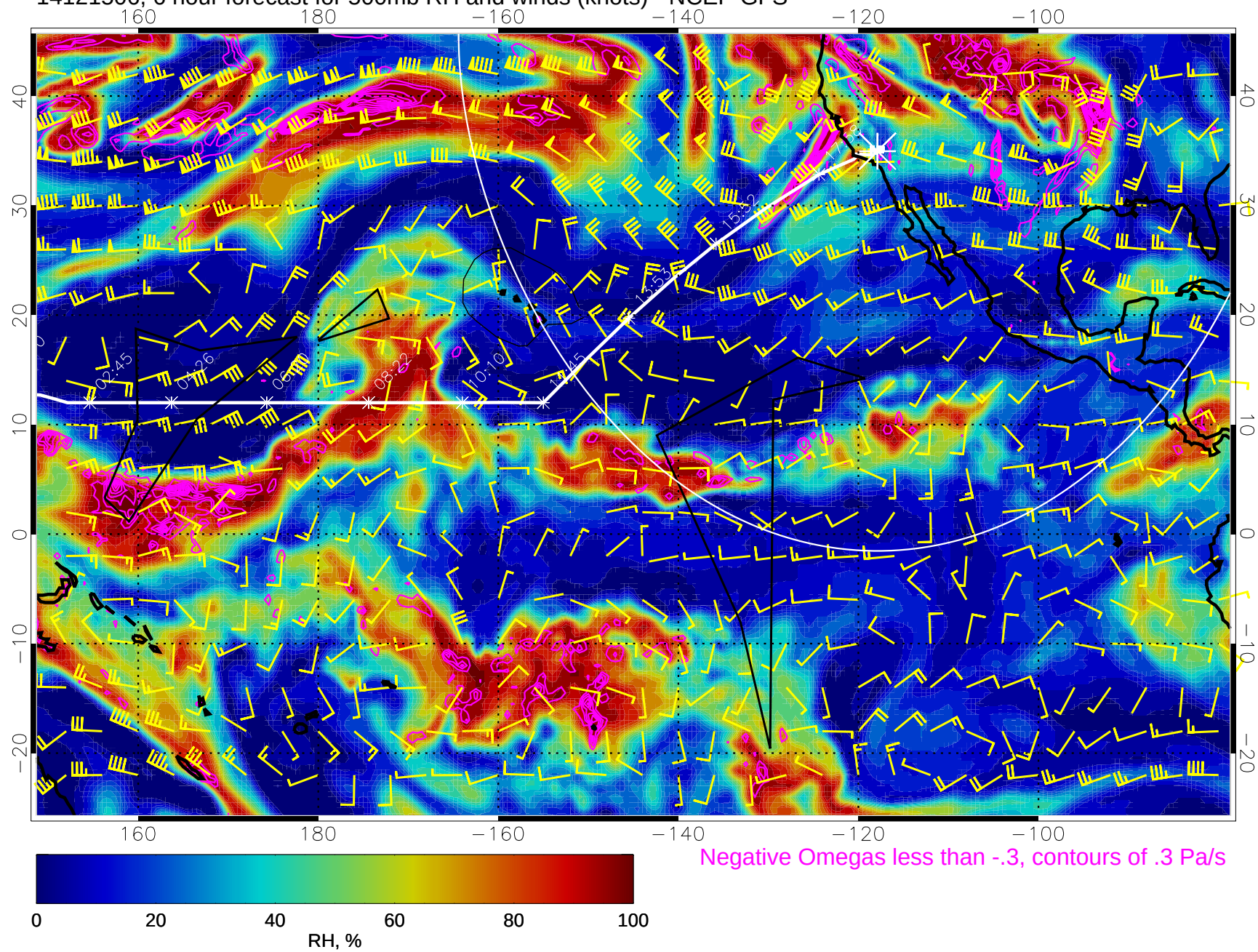
14121506, 6 hour forecast for 500mb RH and winds (knots) - NCEP GFS
