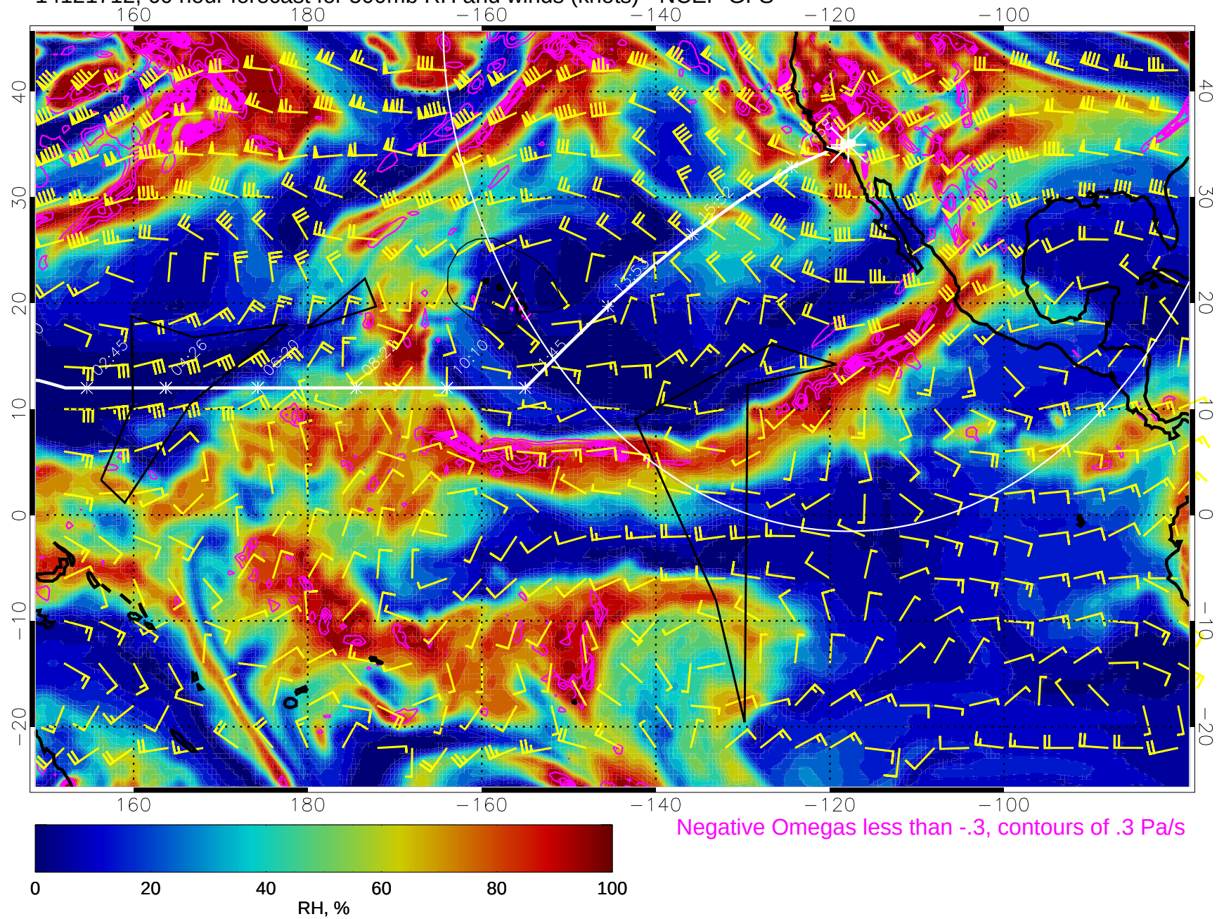
14121712, 60 hour forecast for 500mb RH and winds (knots) - NCEP GFS
