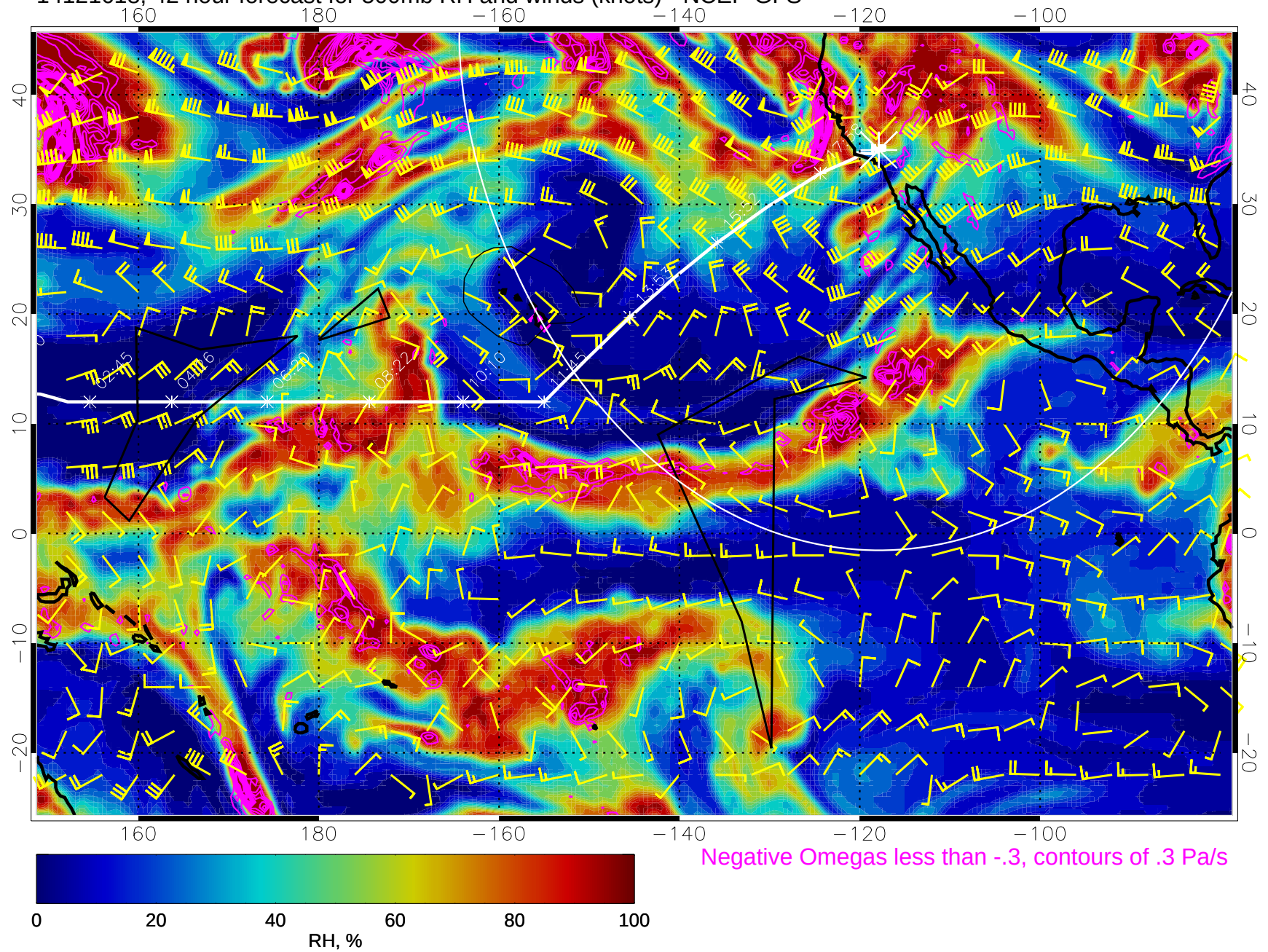
14121618, 42 hour forecast for 500mb RH and winds (knots) - NCEP GFS
