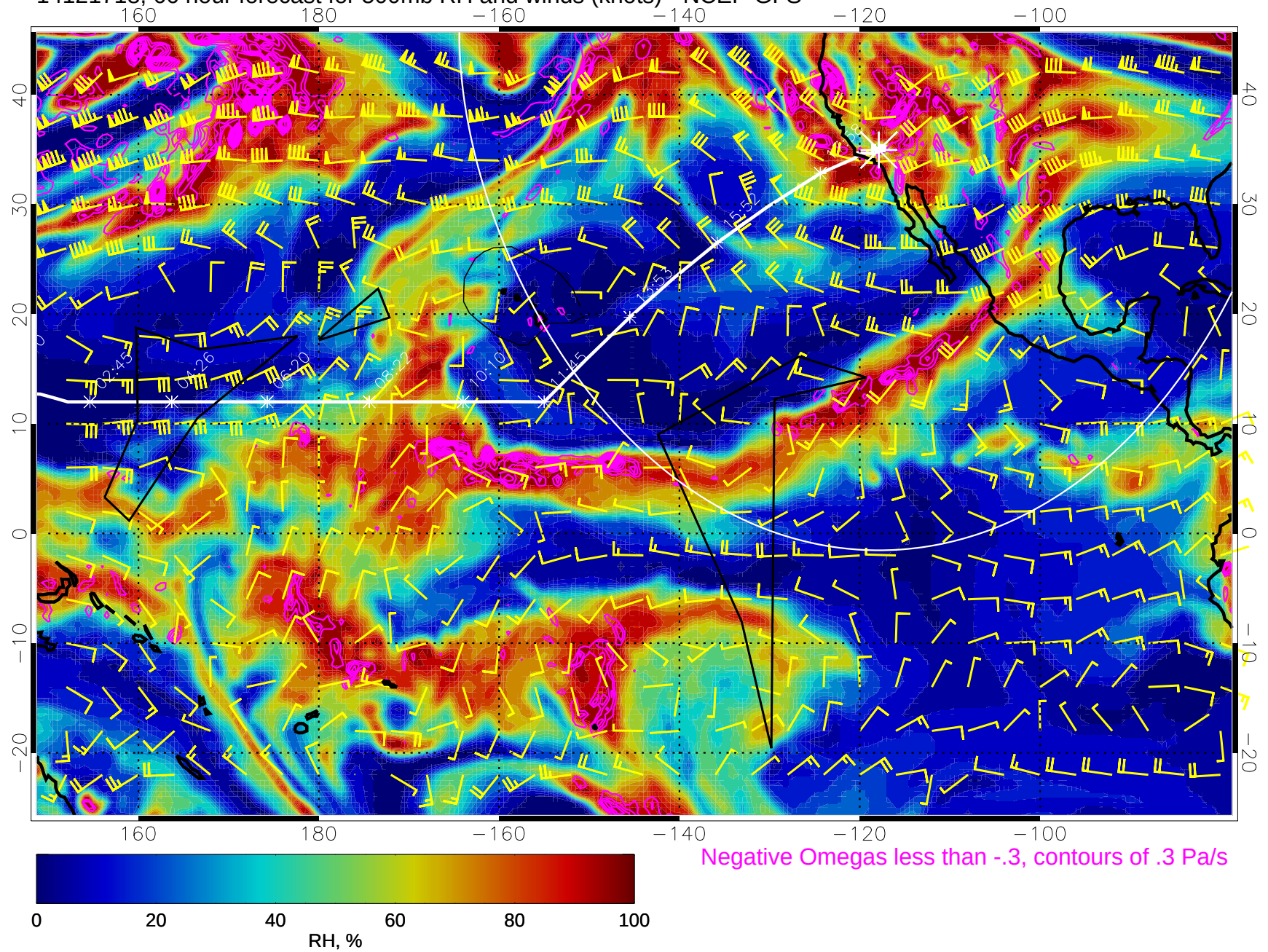
14121718, 66 hour forecast for 500mb RH and winds (knots) - NCEP GFS
