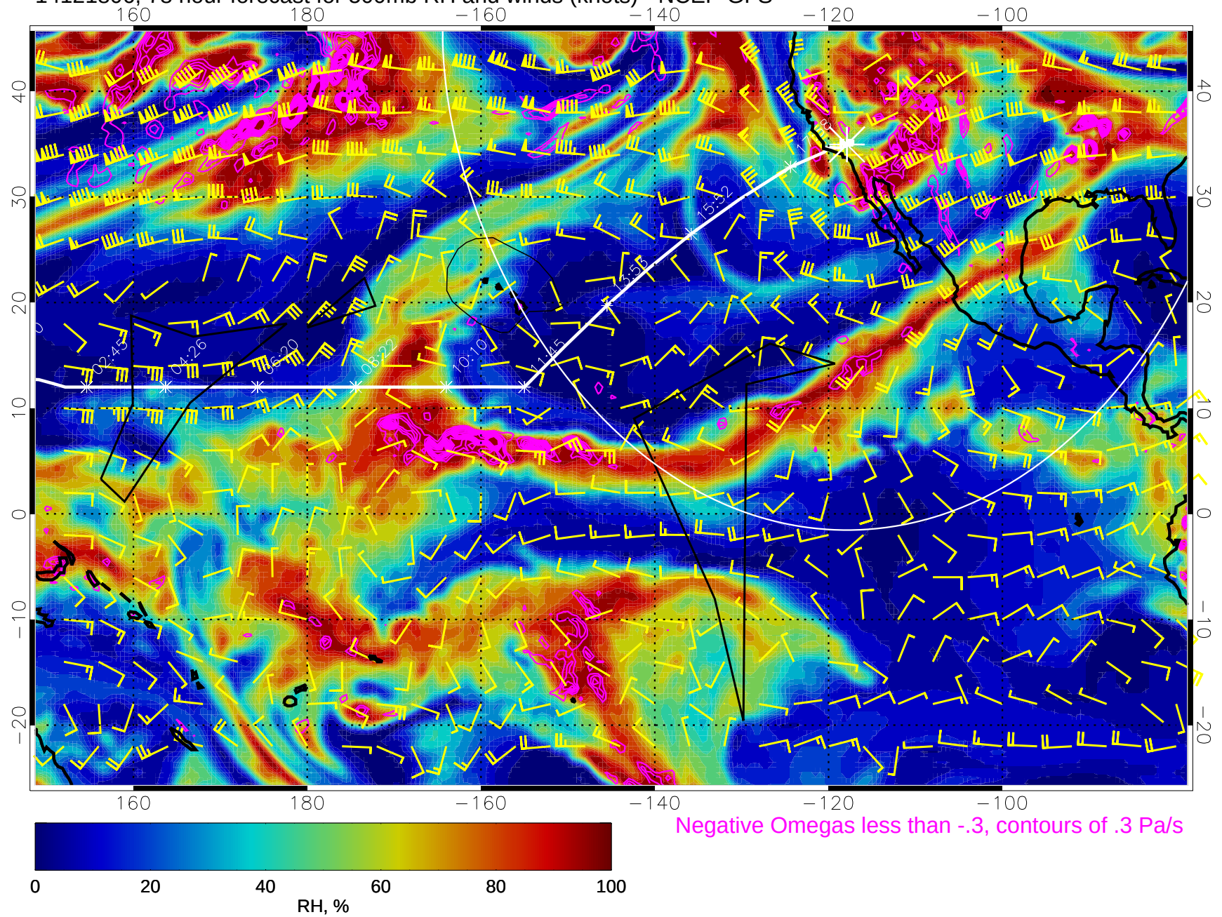
14121806, 78 hour forecast for 500mb RH and winds (knots) - NCEP GFS
