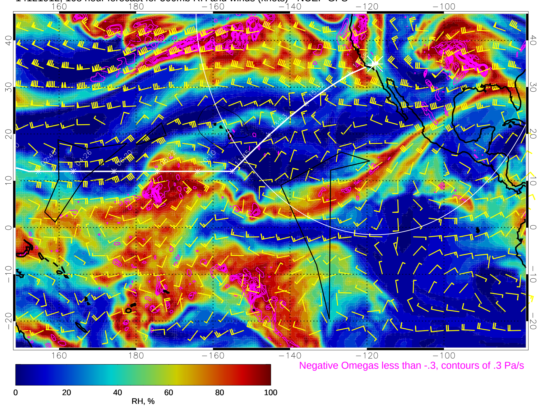
14121912, 108 hour forecast for 500mb RH and winds (knots) - NCEP GFS
