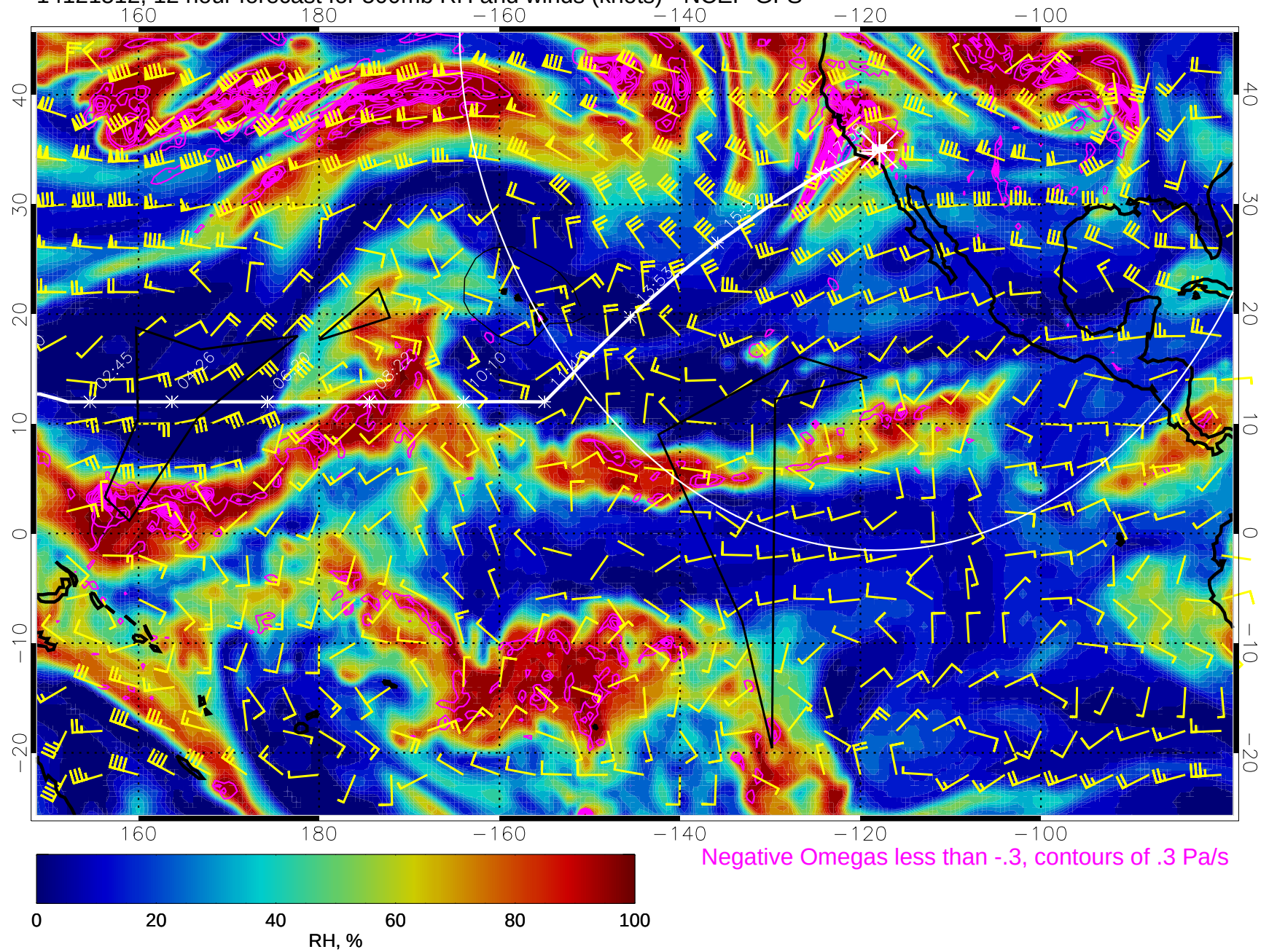
14121512, 12 hour forecast for 500mb RH and winds (knots) - NCEP GFS
