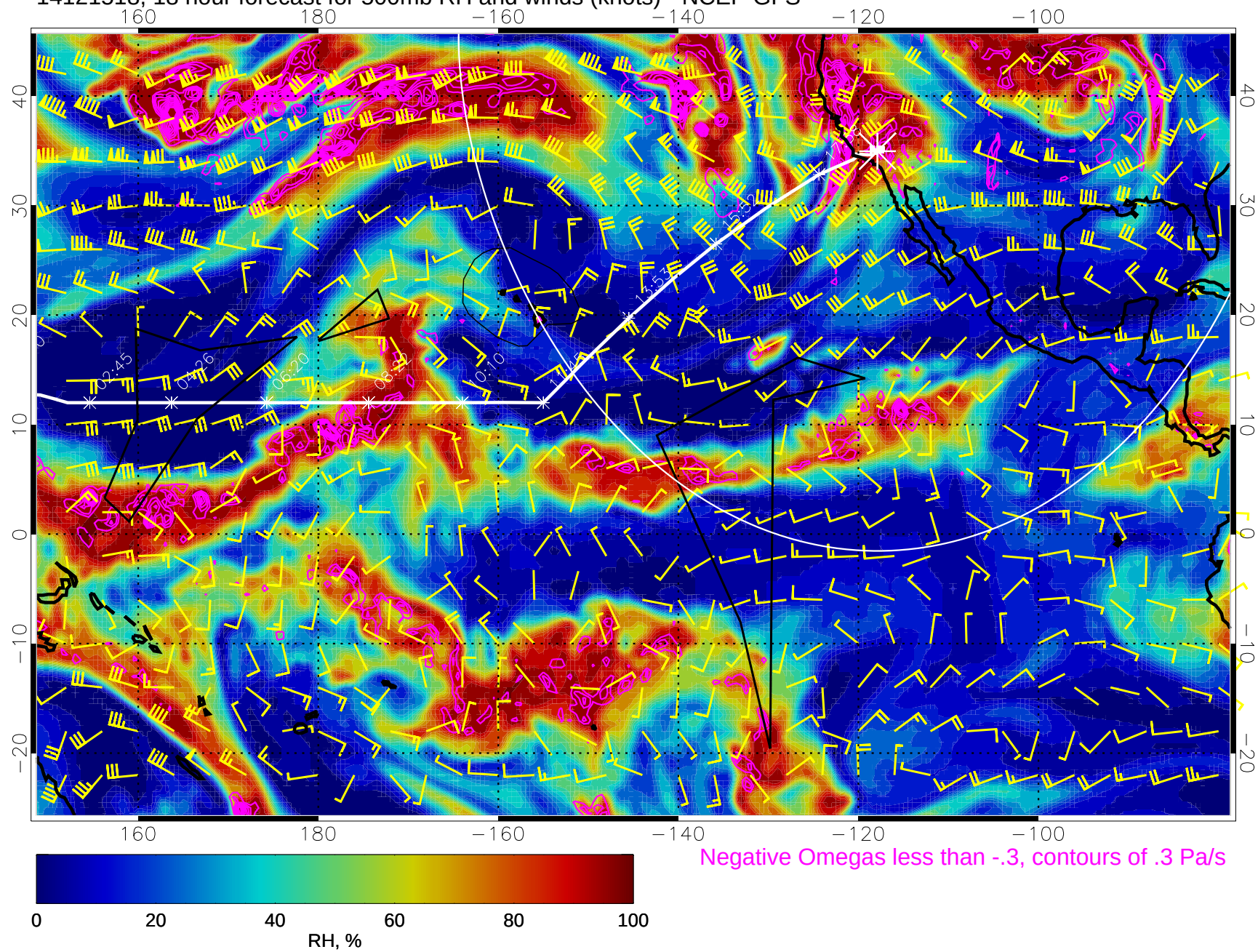
14121518, 18 hour forecast for 500mb RH and winds (knots) - NCEP GFS
