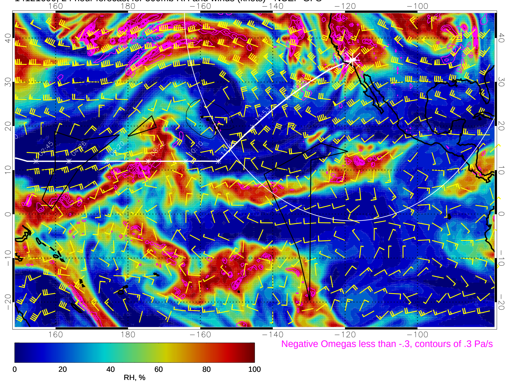
14121600, 24 hour forecast for 500mb RH and winds (knots) - NCEP GFS
