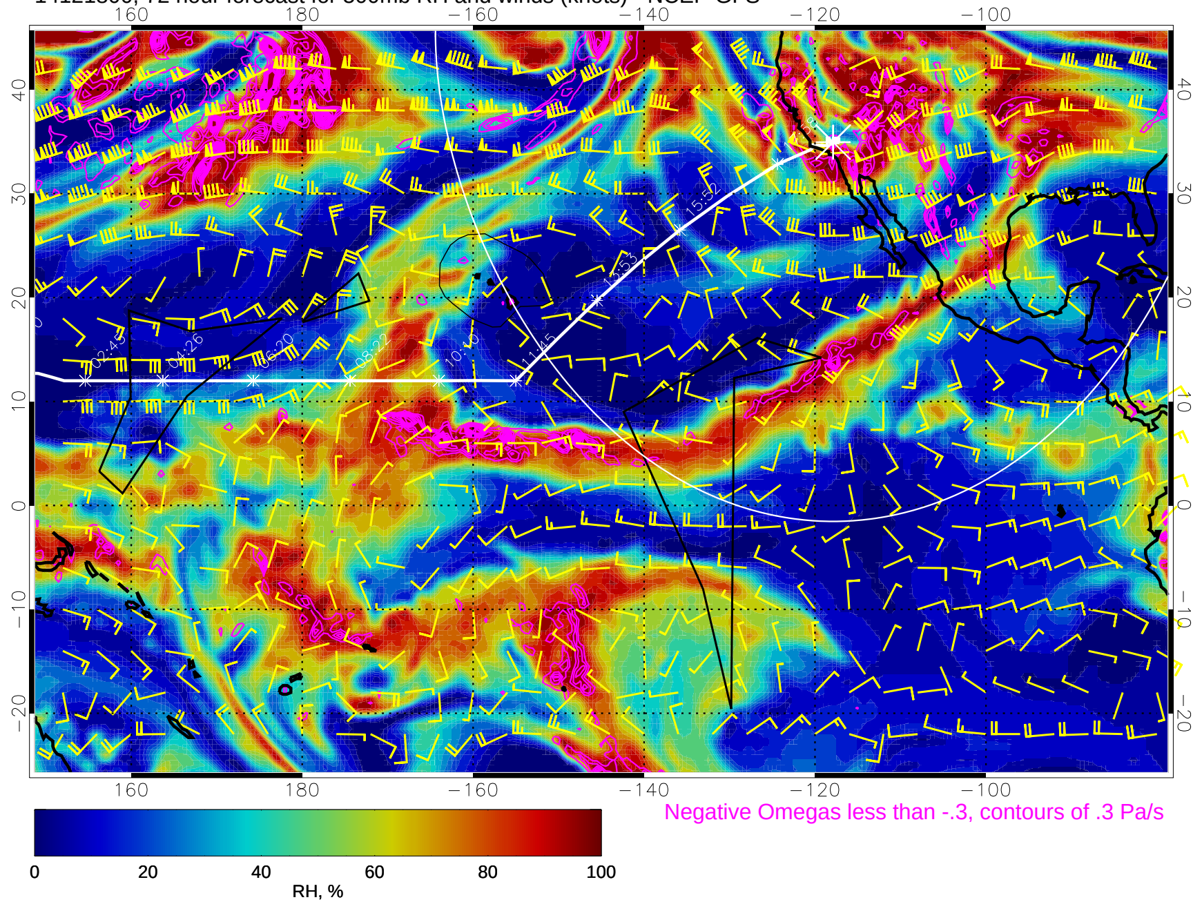
14121800, 72 hour forecast for 500mb RH and winds (knots) - NCEP GFS
