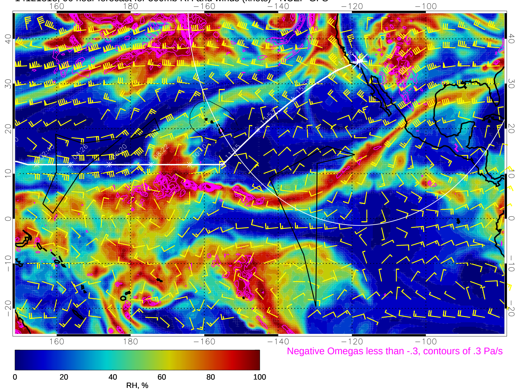
14121818, 90 hour forecast for 500mb RH and winds (knots) - NCEP GFS
