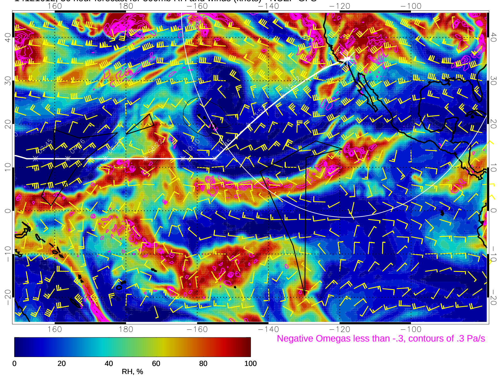
14121612, 36 hour forecast for 500mb RH and winds (knots) - NCEP GFS
