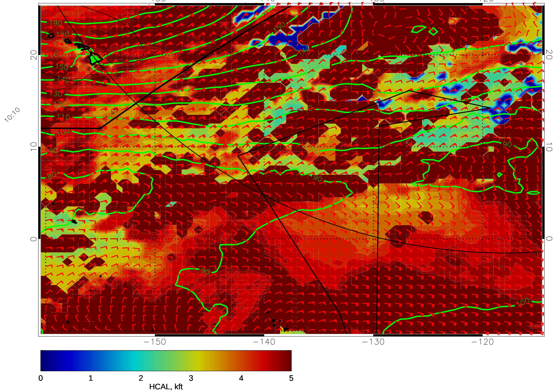
14121512, 12 hour forecast for HCAL, 1000mb Z, and winds (knots) -- NCEP GFS
