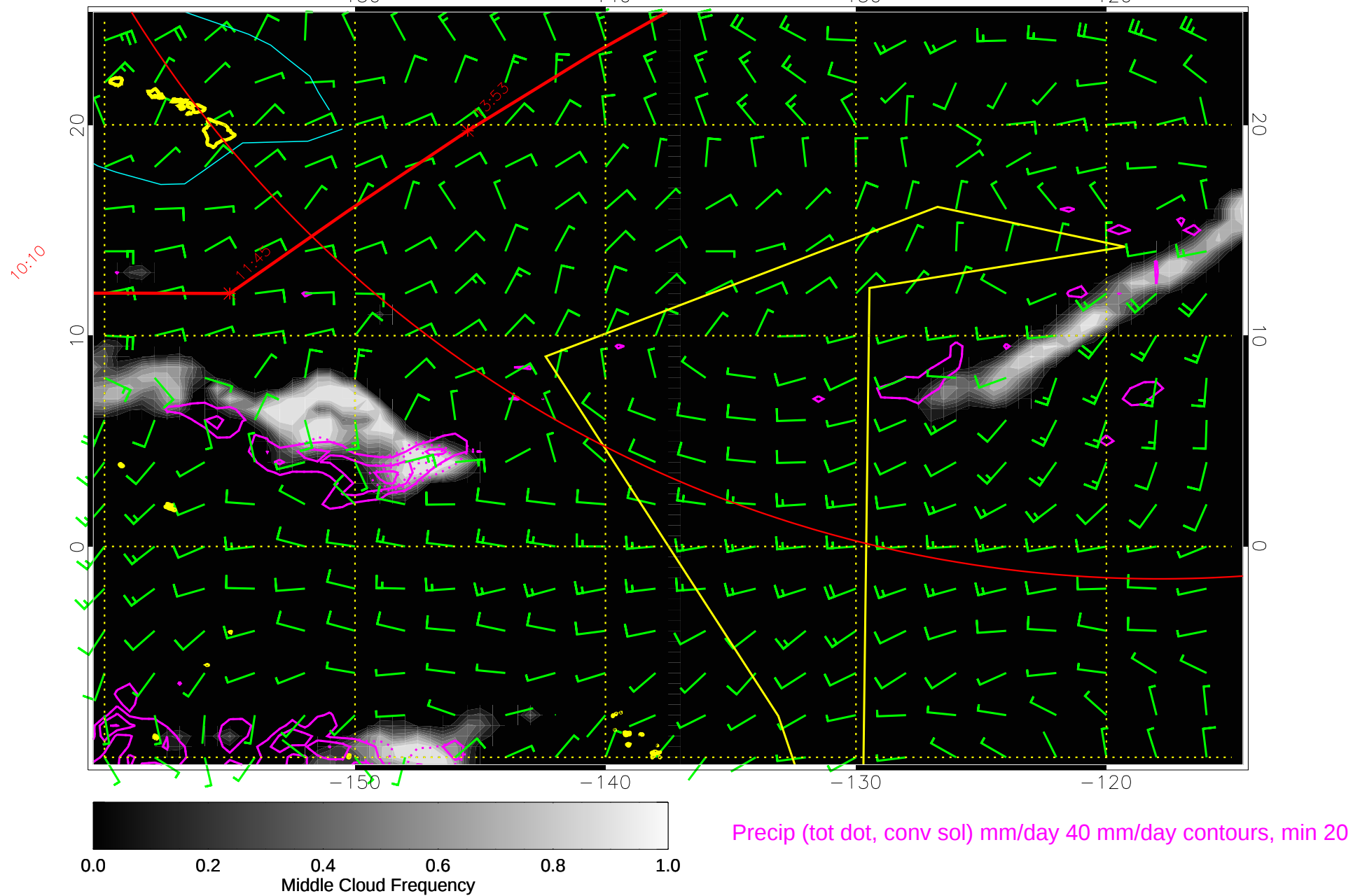
14121906, 102 hour forecast for 500mb winds (knots) and Middle Cloud Frequency -- NCEP GFS
