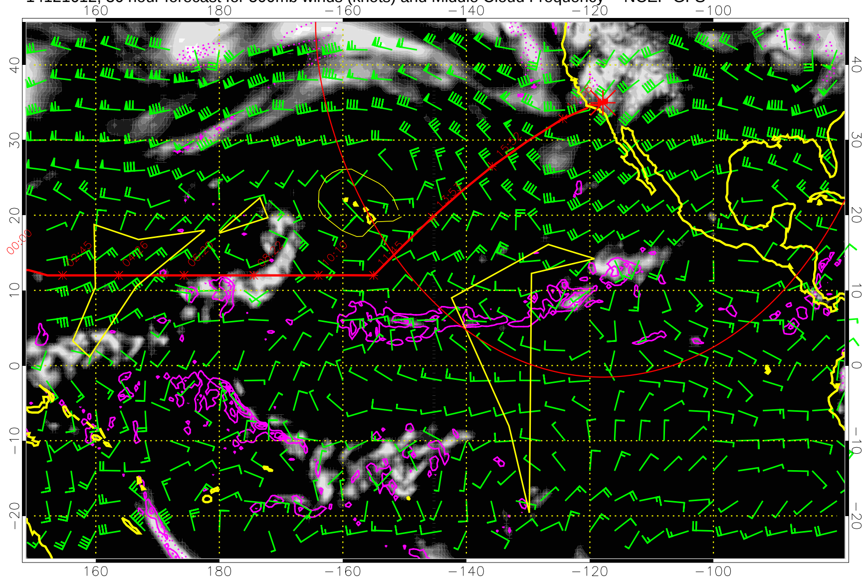
14121612, 36 hour forecast for 500mb winds (knots) and Middle Cloud Frequency -- NCEP GFS
