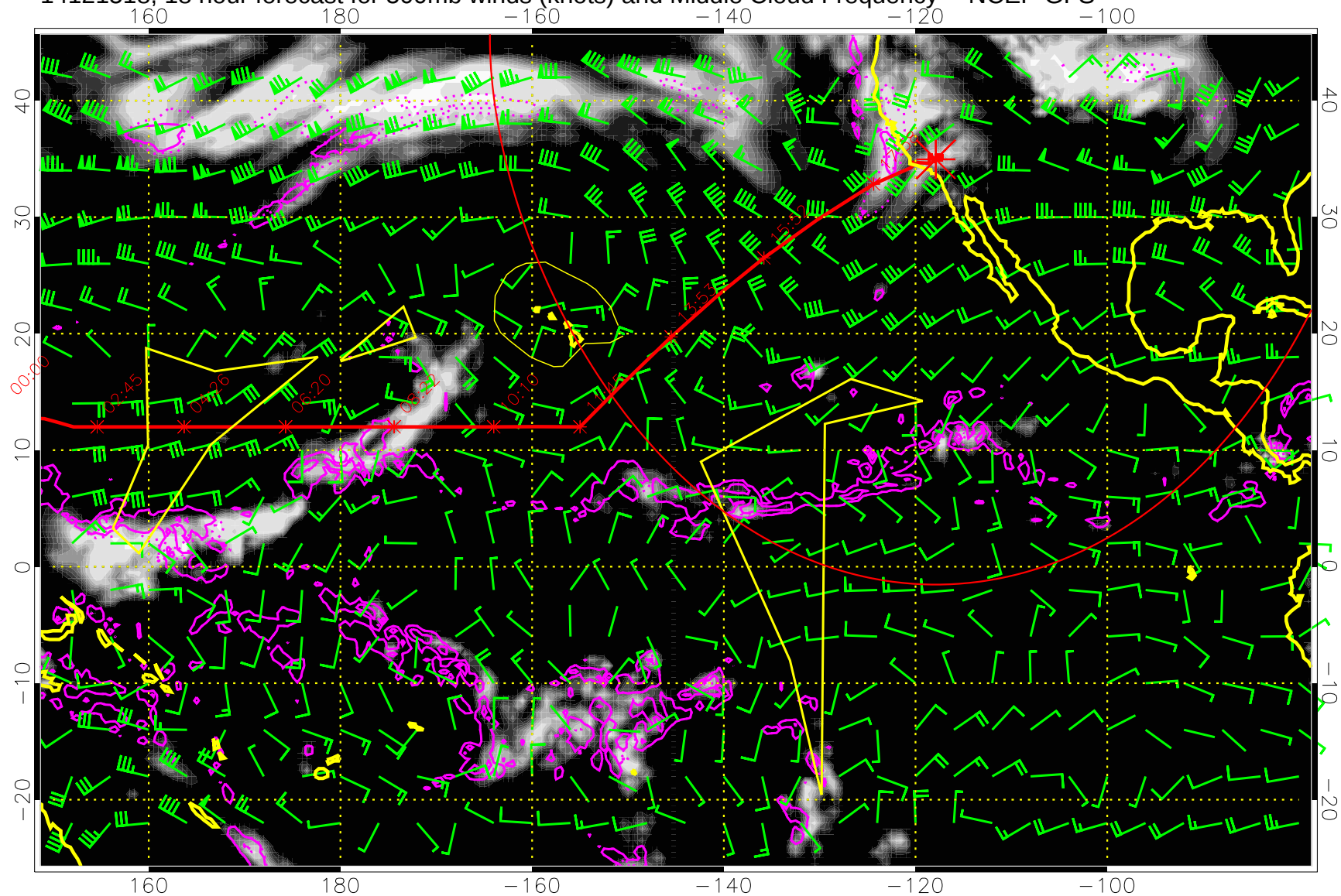
14121518, 18 hour forecast for 500mb winds (knots) and Middle Cloud Frequency -- NCEP GFS
