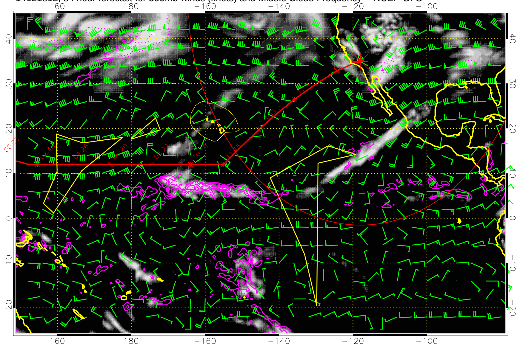
14121812, 84 hour forecast for 500mb winds (knots) and Middle Cloud Frequency -- NCEP GFS
