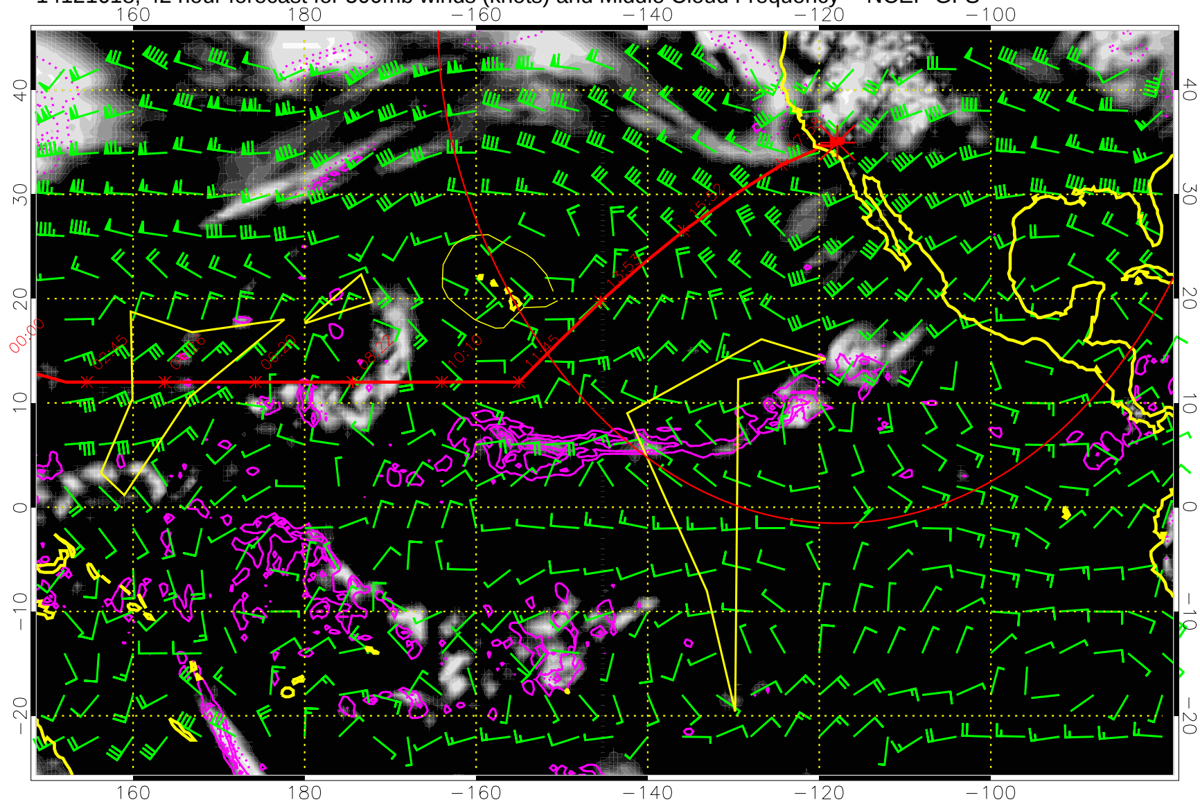
14121618, 42 hour forecast for 500mb winds (knots) and Middle Cloud Frequency -- NCEP GFS
