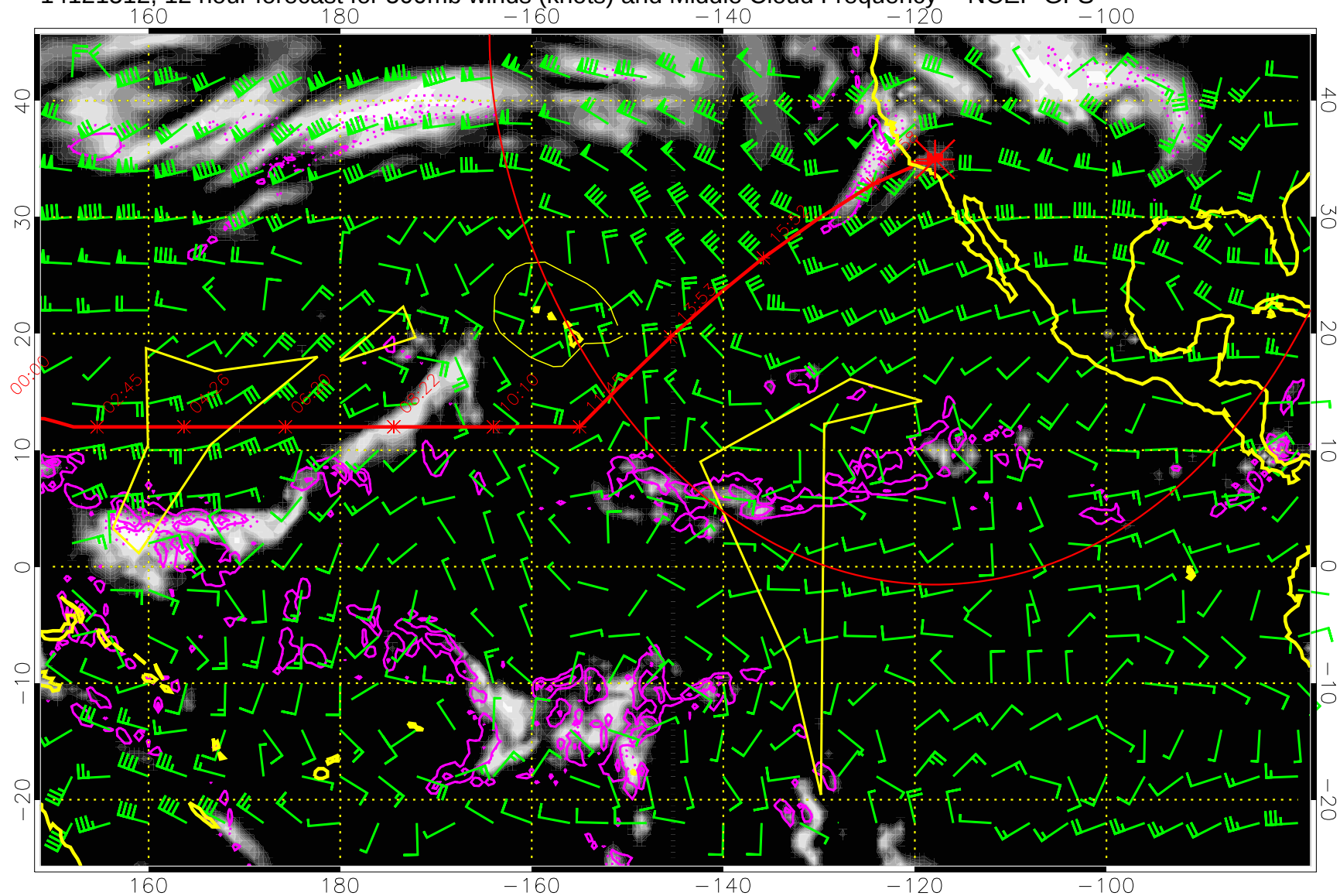
14121512, 12 hour forecast for 500mb winds (knots) and Middle Cloud Frequency -- NCEP GFS
