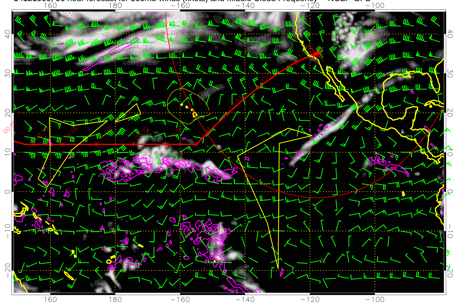
14121900, 96 hour forecast for 500mb winds (knots) and Middle Cloud Frequency -- NCEP GFS
