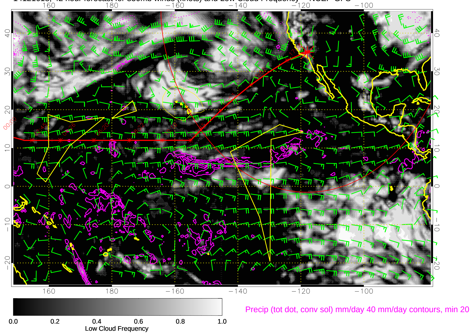
14121618, 42 hour forecast for 850mb winds (knots) and Low Cloud Frequency -- NCEP GFS
