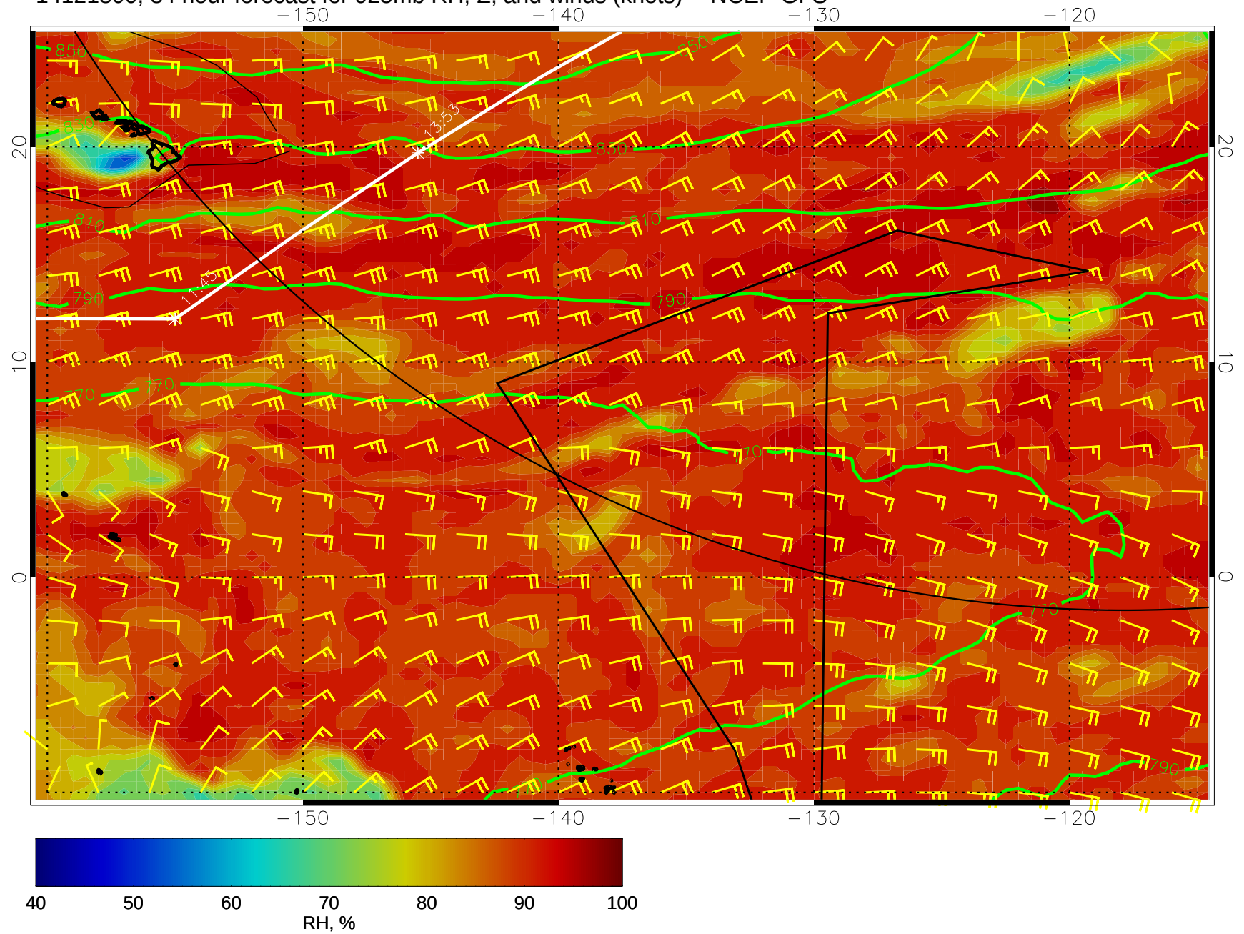
14121800, 84 hour forecast for 925mb RH, Z, and winds (knots) -- NCEP GFS
