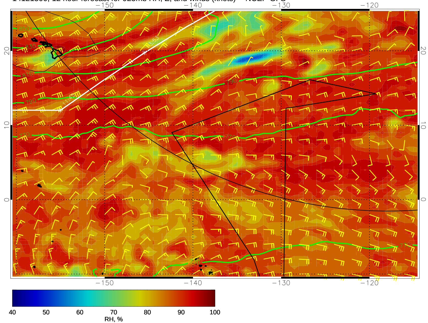
14121500, 12 hour forecast for 925mb RH, Z, and winds (knots) -- NCEP GFS
