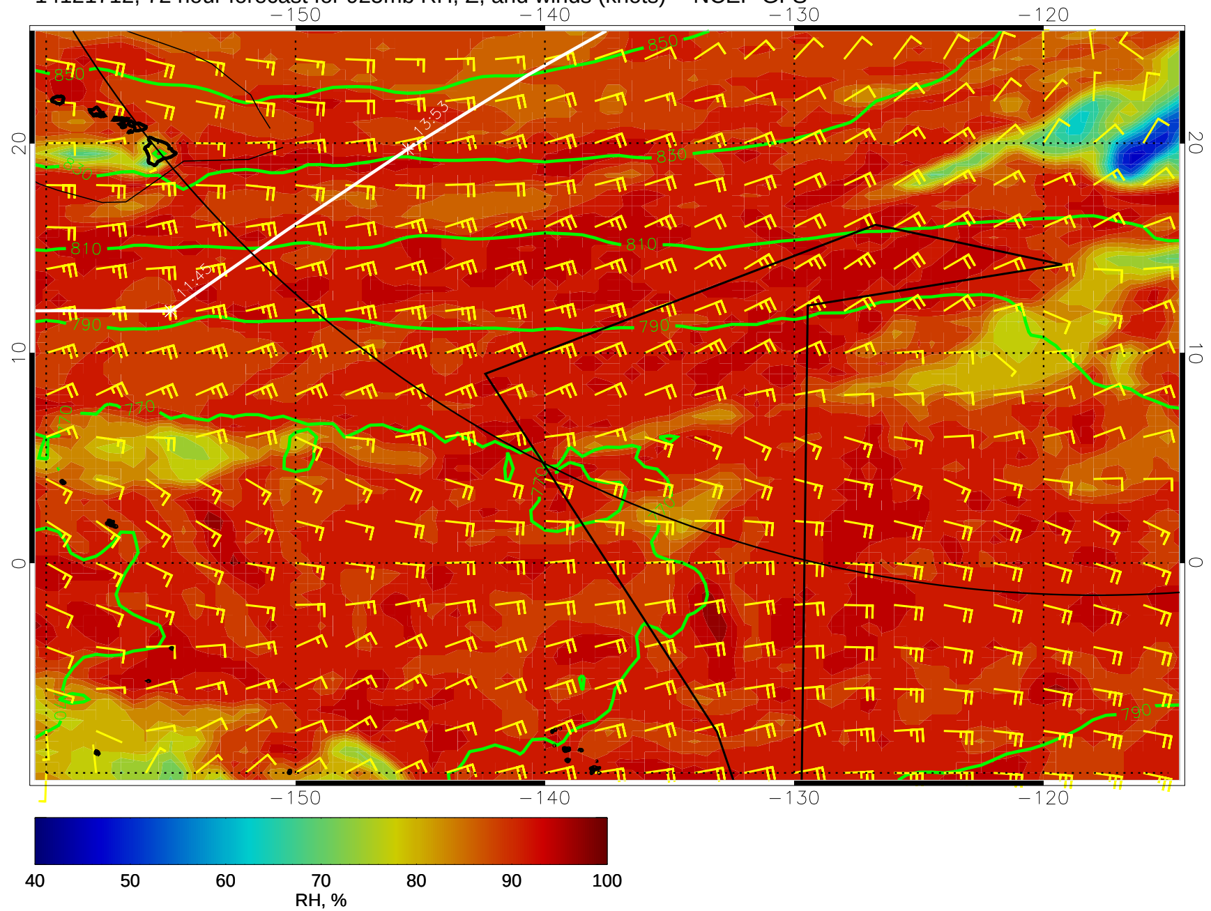
14121712, 72 hour forecast for 925mb RH, Z, and winds (knots) -- NCEP GFS
