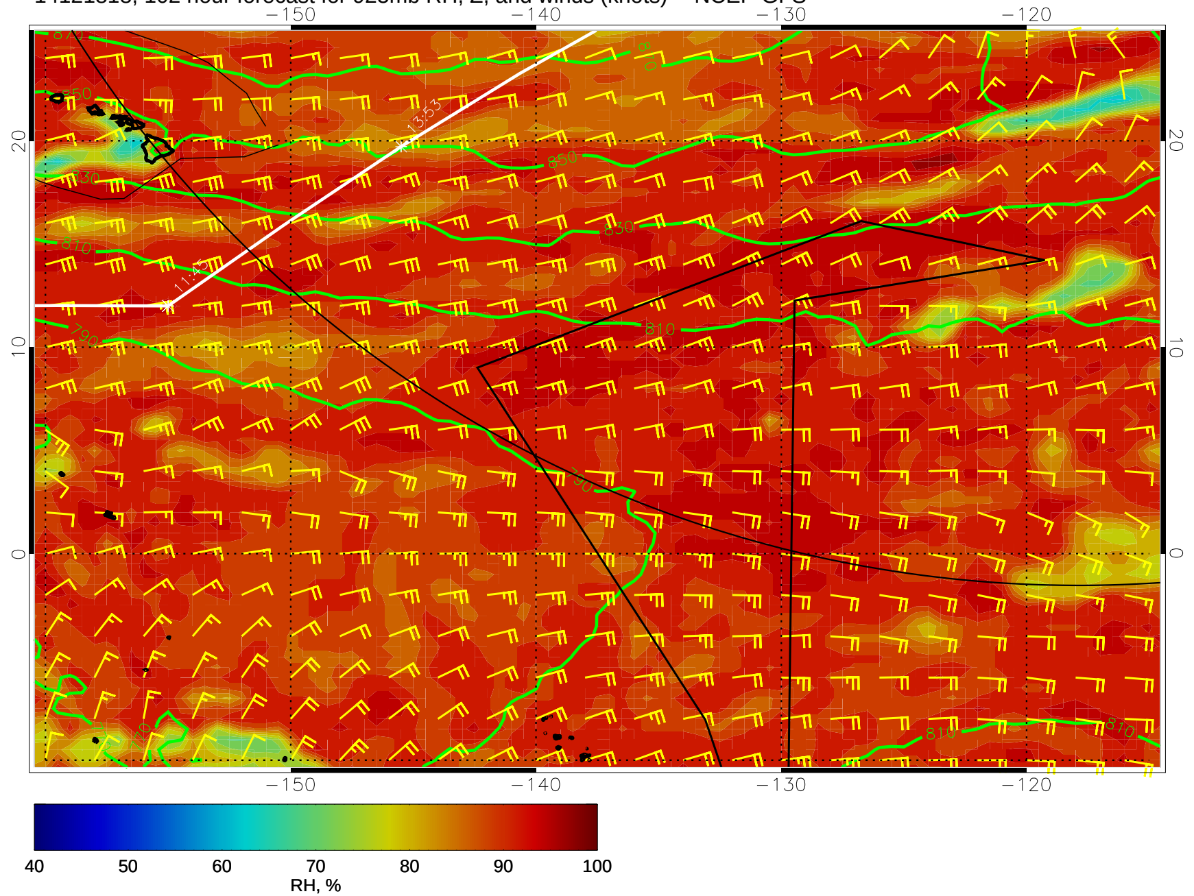
14121818, 102 hour forecast for 925mb RH, Z, and winds (knots) -- NCEP GFS
