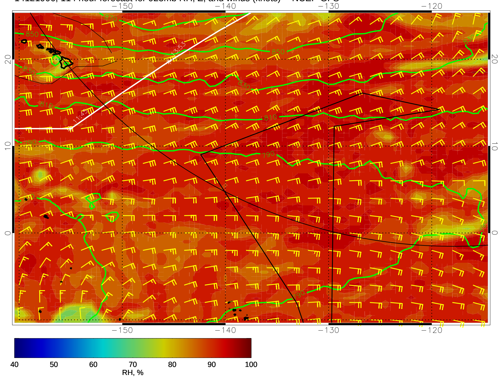
14121906, 114 hour forecast for 925mb RH, Z, and winds (knots) -- NCEP GFS
