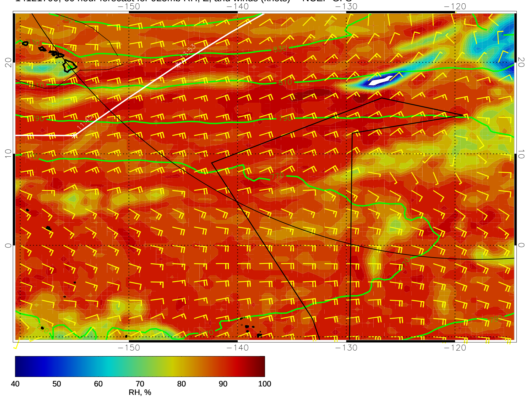
14121700, 60 hour forecast for 925mb RH, Z, and winds (knots) -- NCEP GFS
