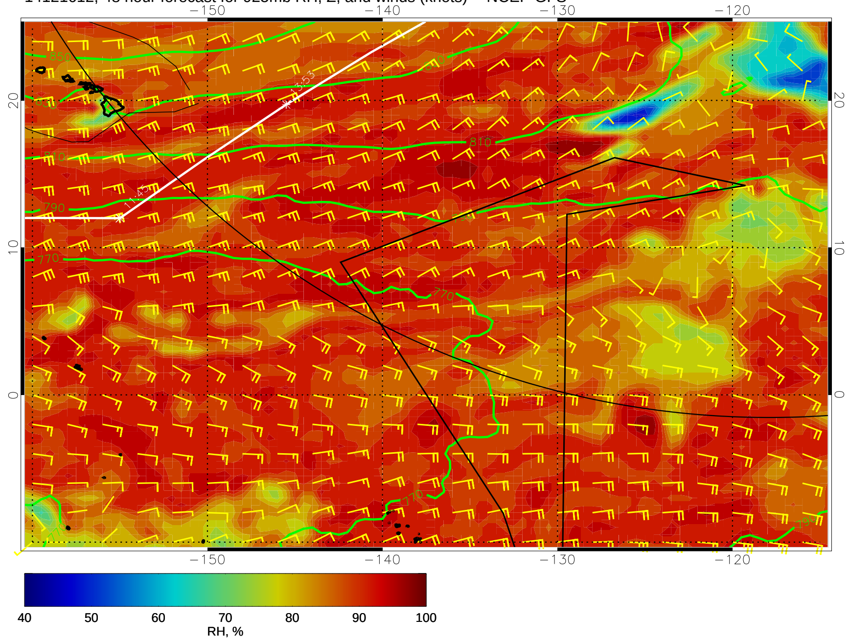
14121612, 48 hour forecast for 925mb RH, Z, and winds (knots) -- NCEP GFS
