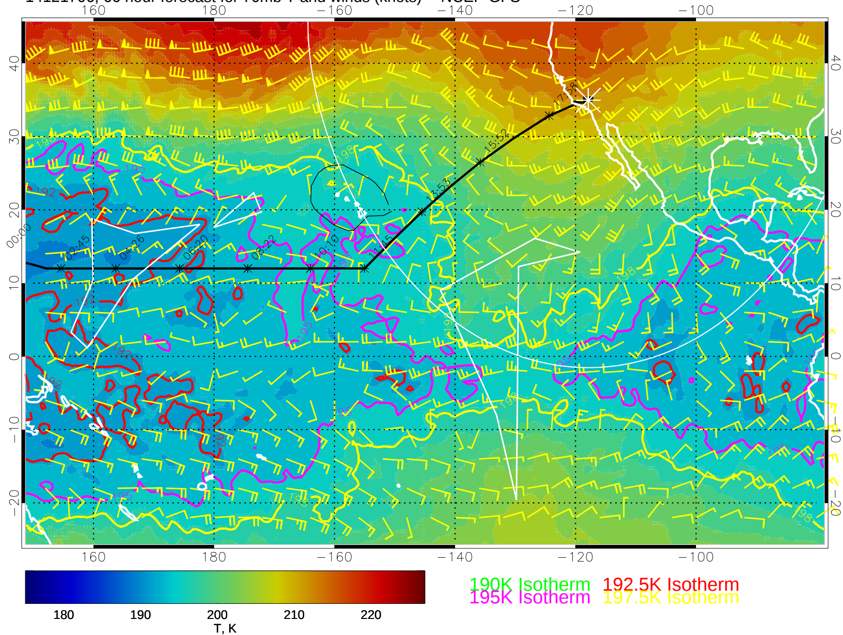
14121706, 66 hour forecast for 70mb T and winds (knots) -- NCEP GFS
