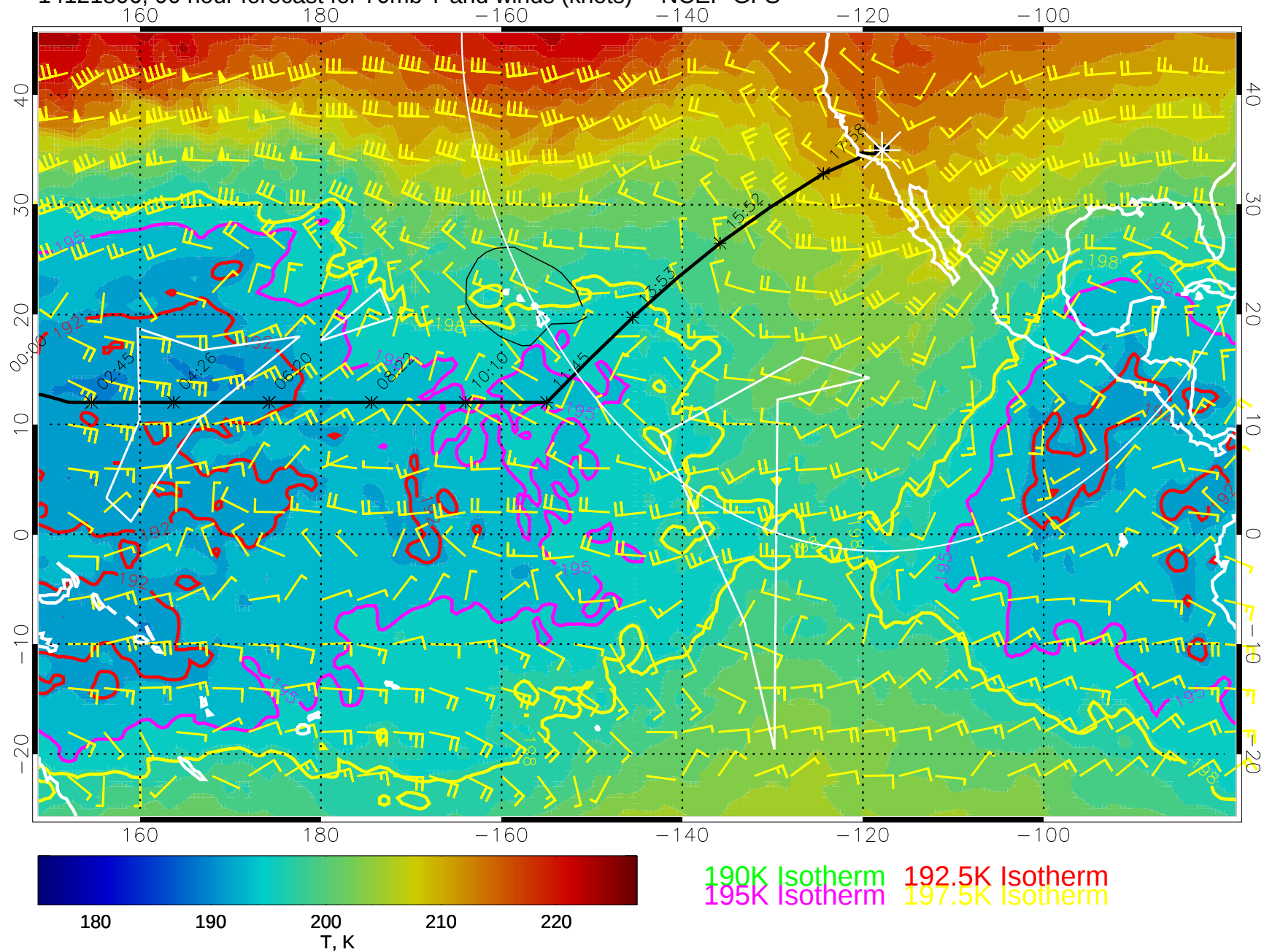
14121806, 90 hour forecast for 70mb T and winds (knots) -- NCEP GFS
