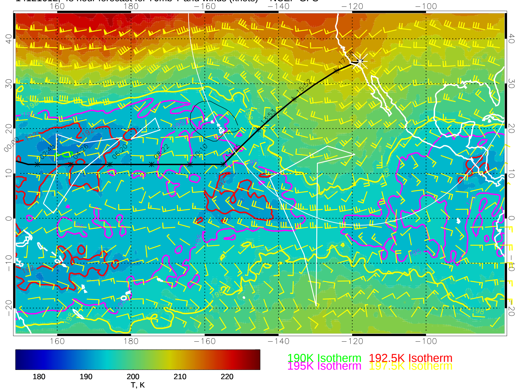
14121612, 48 hour forecast for 70mb T and winds (knots) -- NCEP GFS
