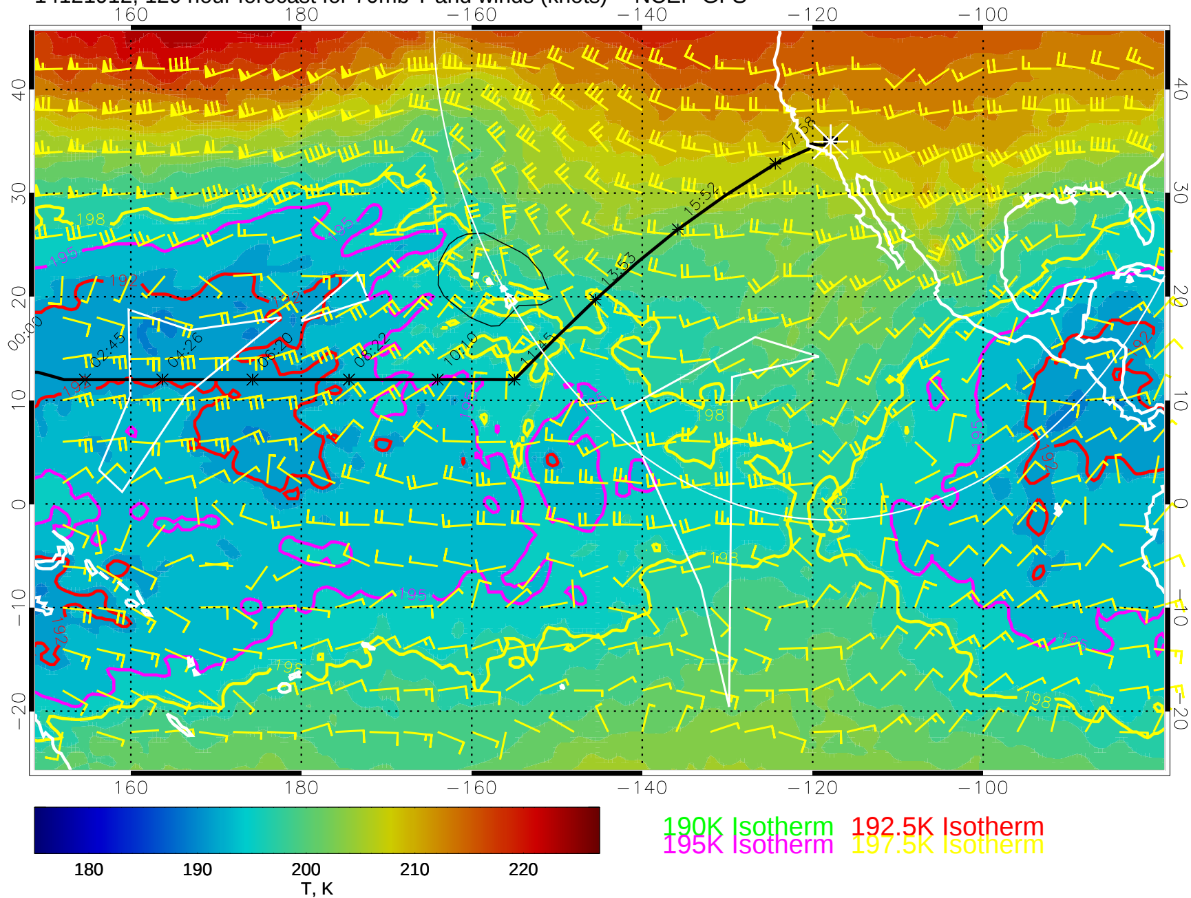
14121912, 120 hour forecast for 70mb T and winds (knots) -- NCEP GFS
