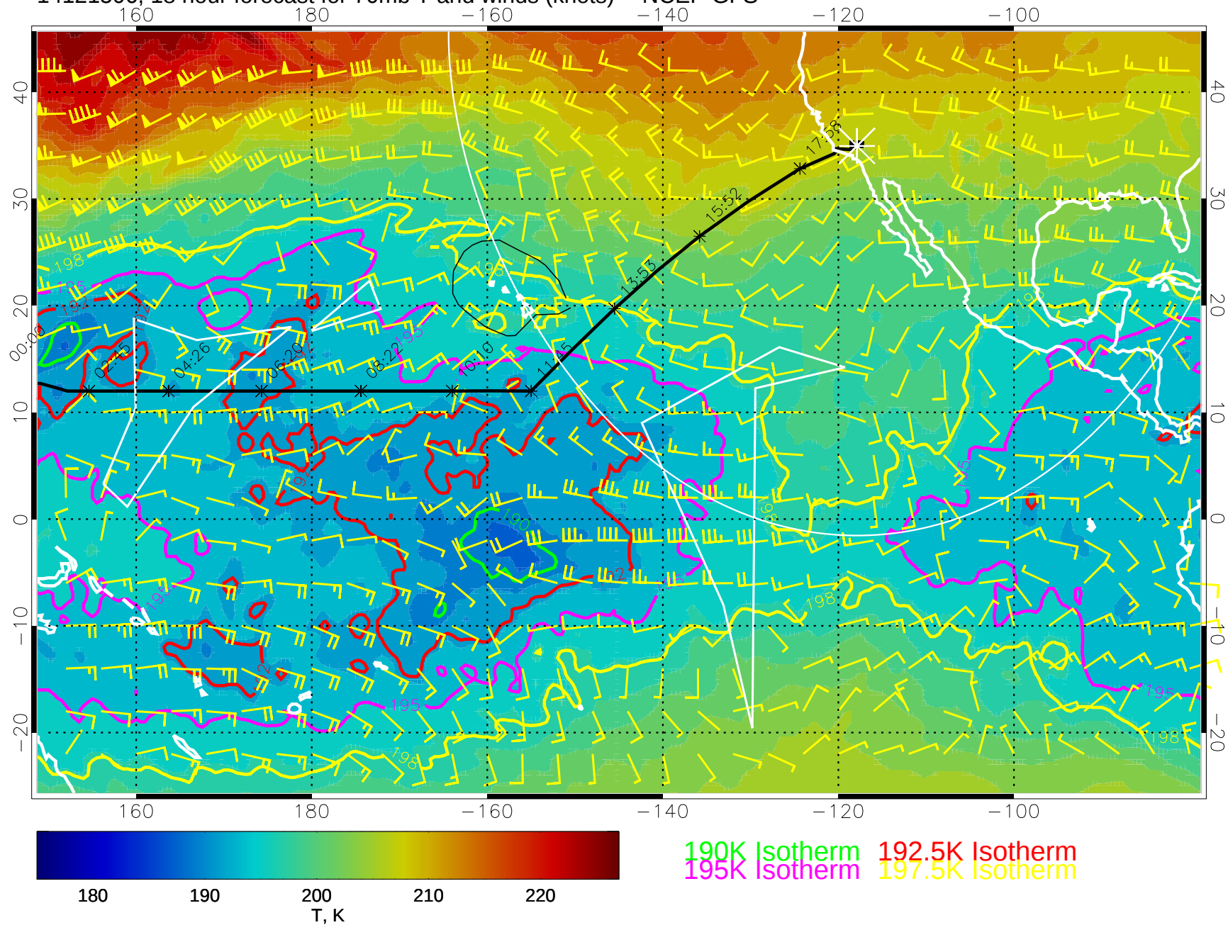
14121506, 18 hour forecast for 70mb T and winds (knots) -- NCEP GFS
