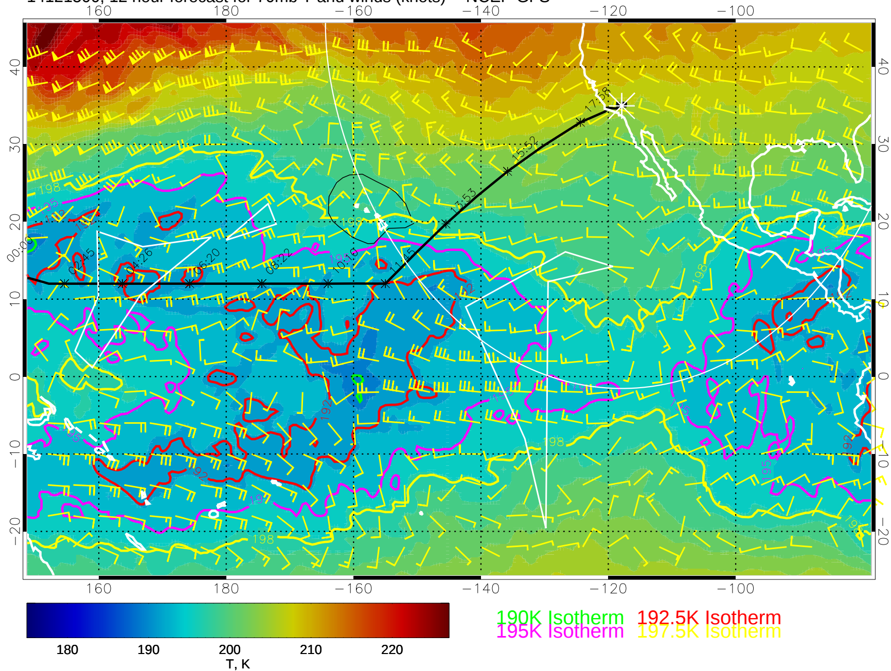
14121500, 12 hour forecast for 70mb T and winds (knots) -- NCEP GFS
