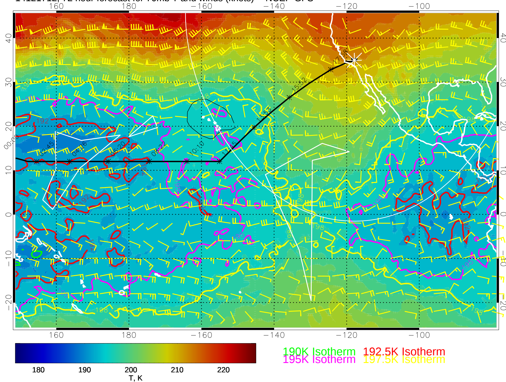
14121712, 72 hour forecast for 70mb T and winds (knots) -- NCEP GFS
