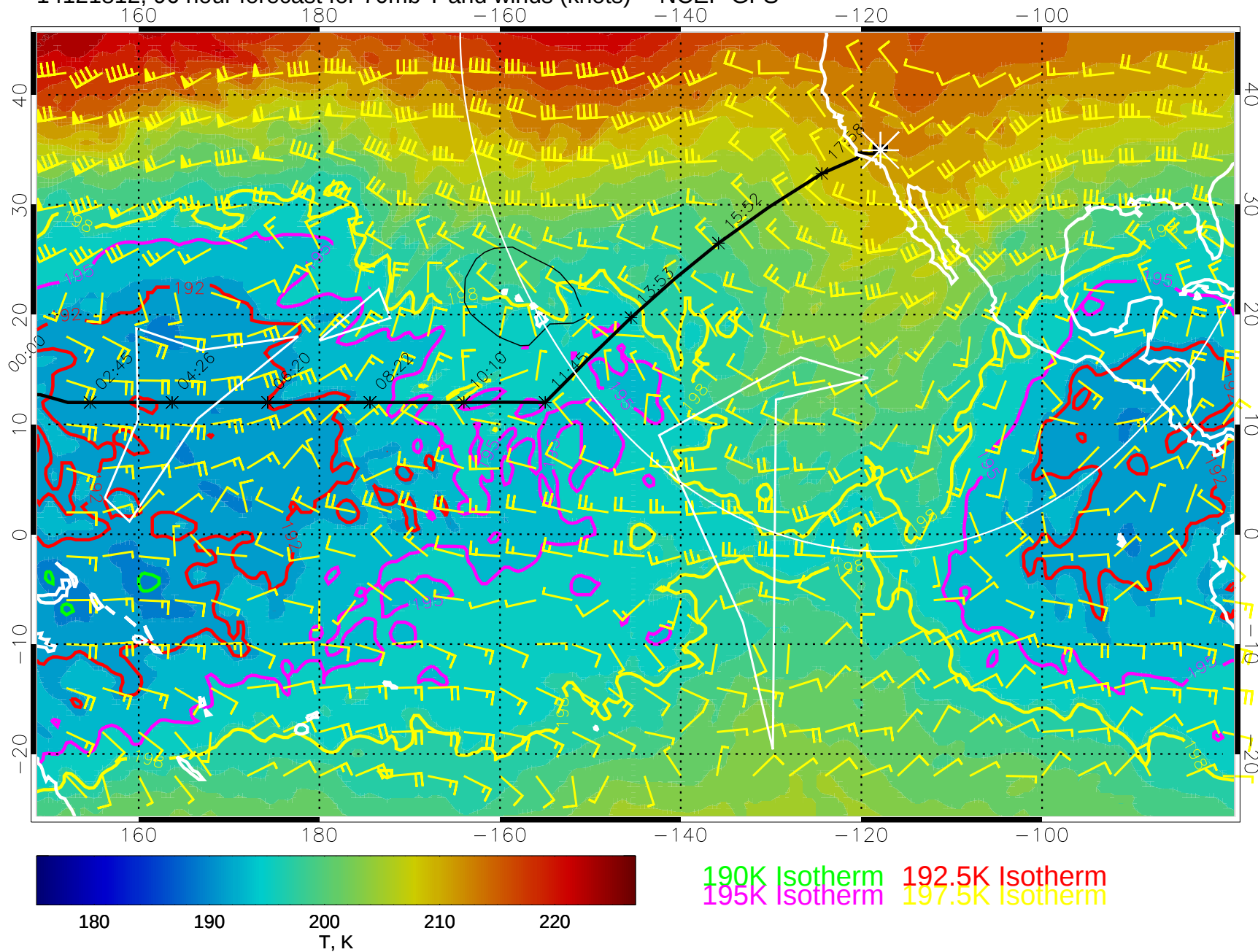
14121812, 96 hour forecast for 70mb T and winds (knots) -- NCEP GFS
