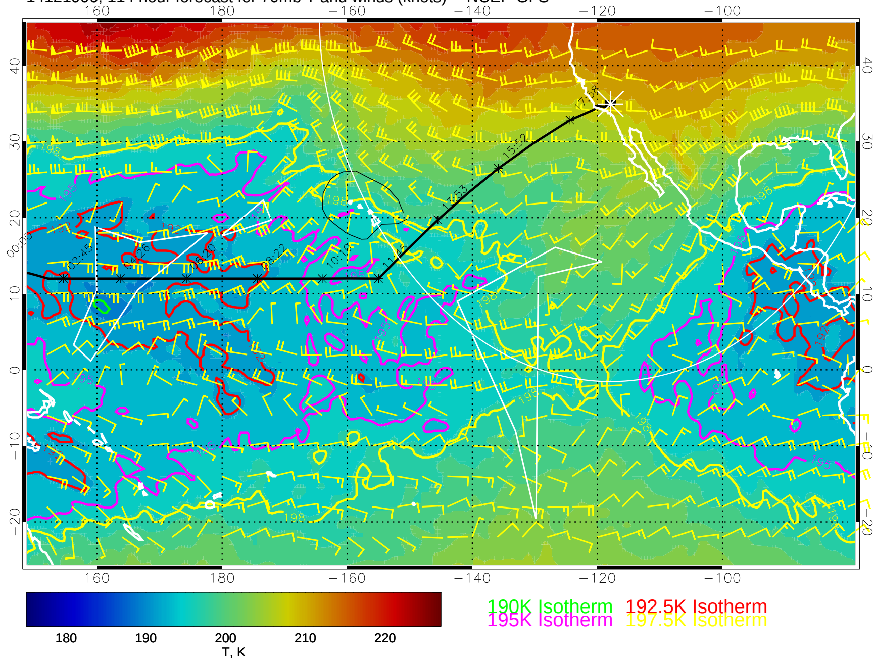
14121906, 114 hour forecast for 70mb T and winds (knots) -- NCEP GFS
