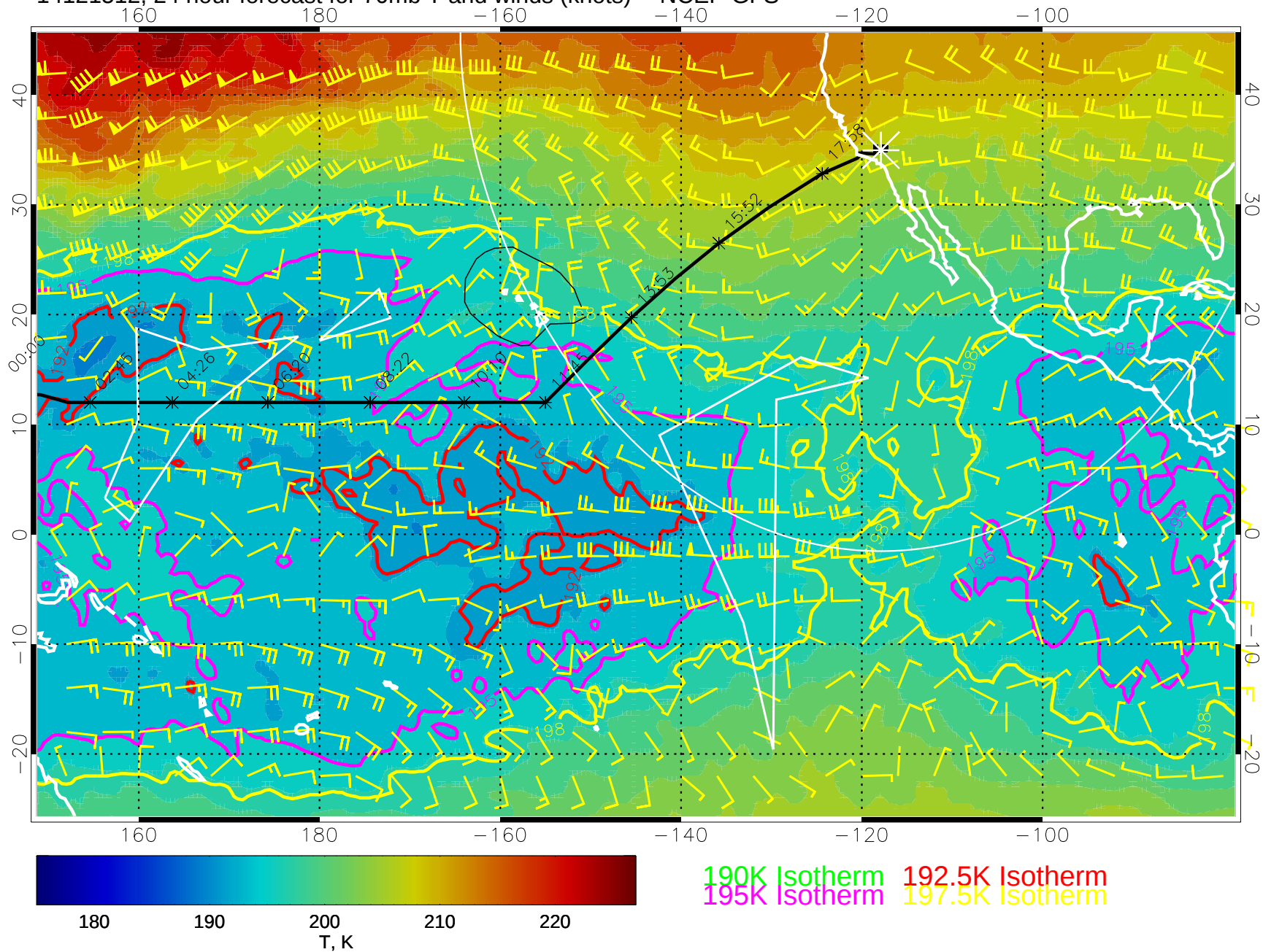
14121512, 24 hour forecast for 70mb T and winds (knots) -- NCEP GFS
