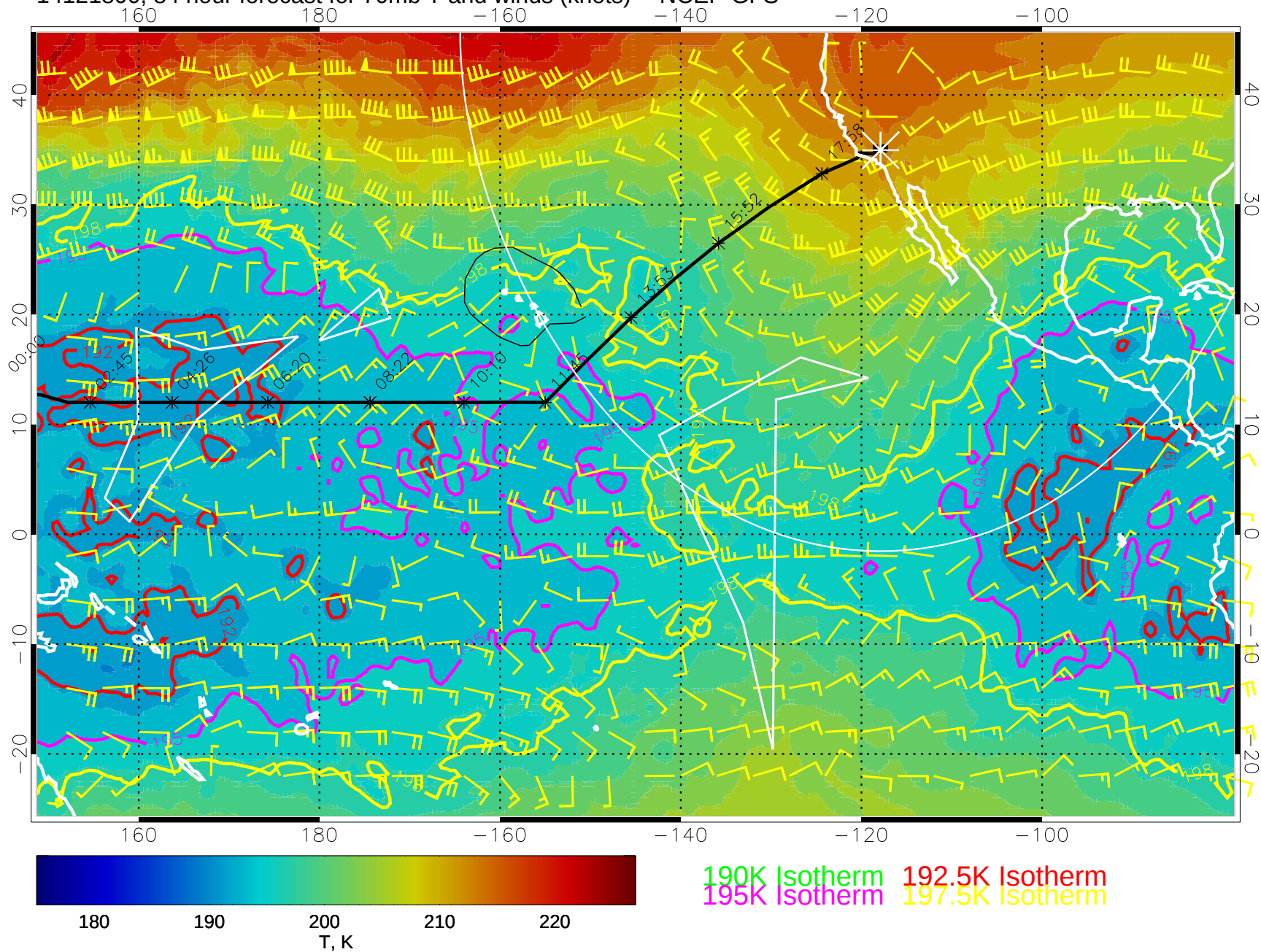
14121800, 84 hour forecast for 70mb T and winds (knots) -- NCEP GFS
