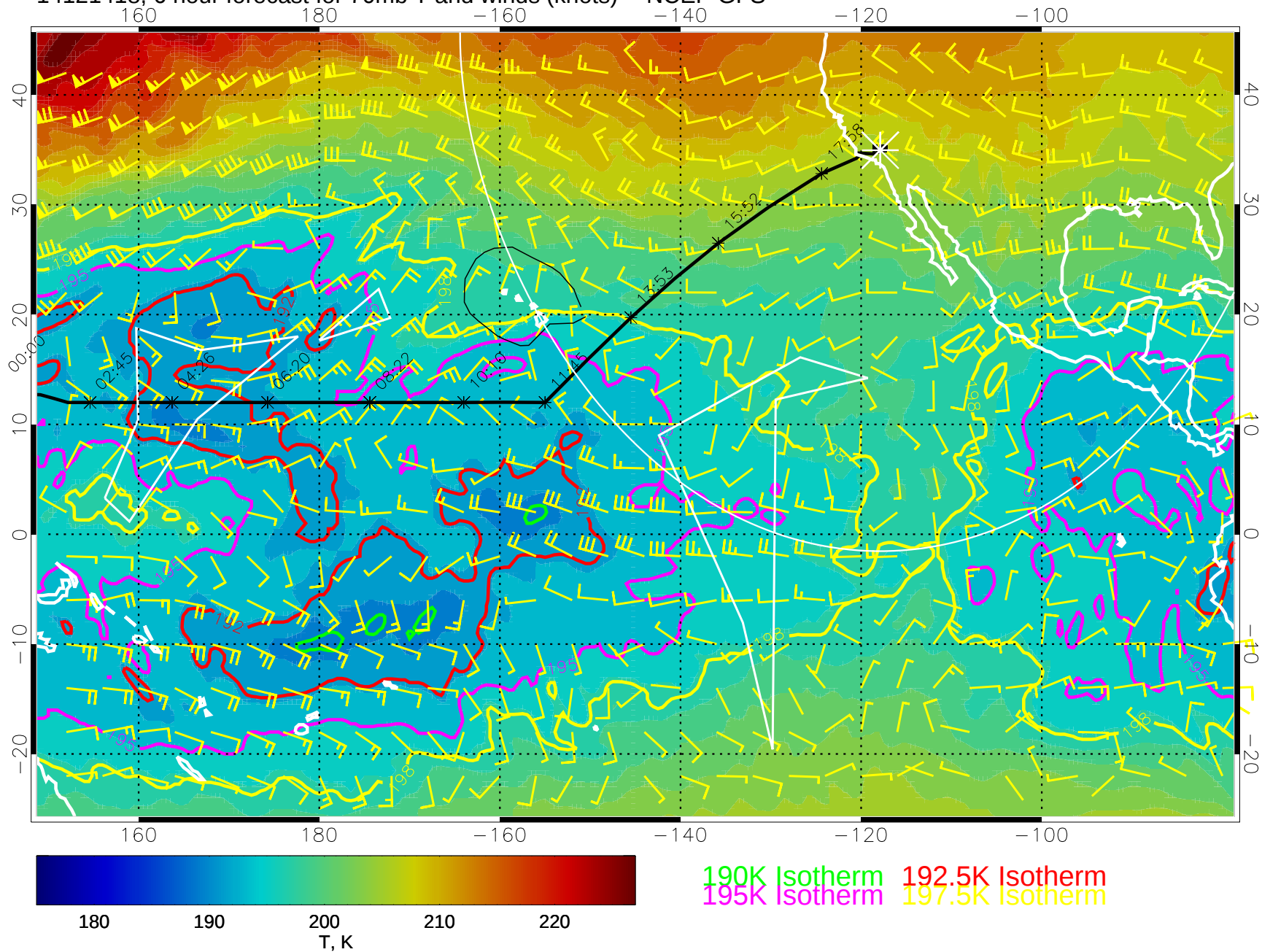
14121418, 6 hour forecast for 70mb T and winds (knots) -- NCEP GFS
