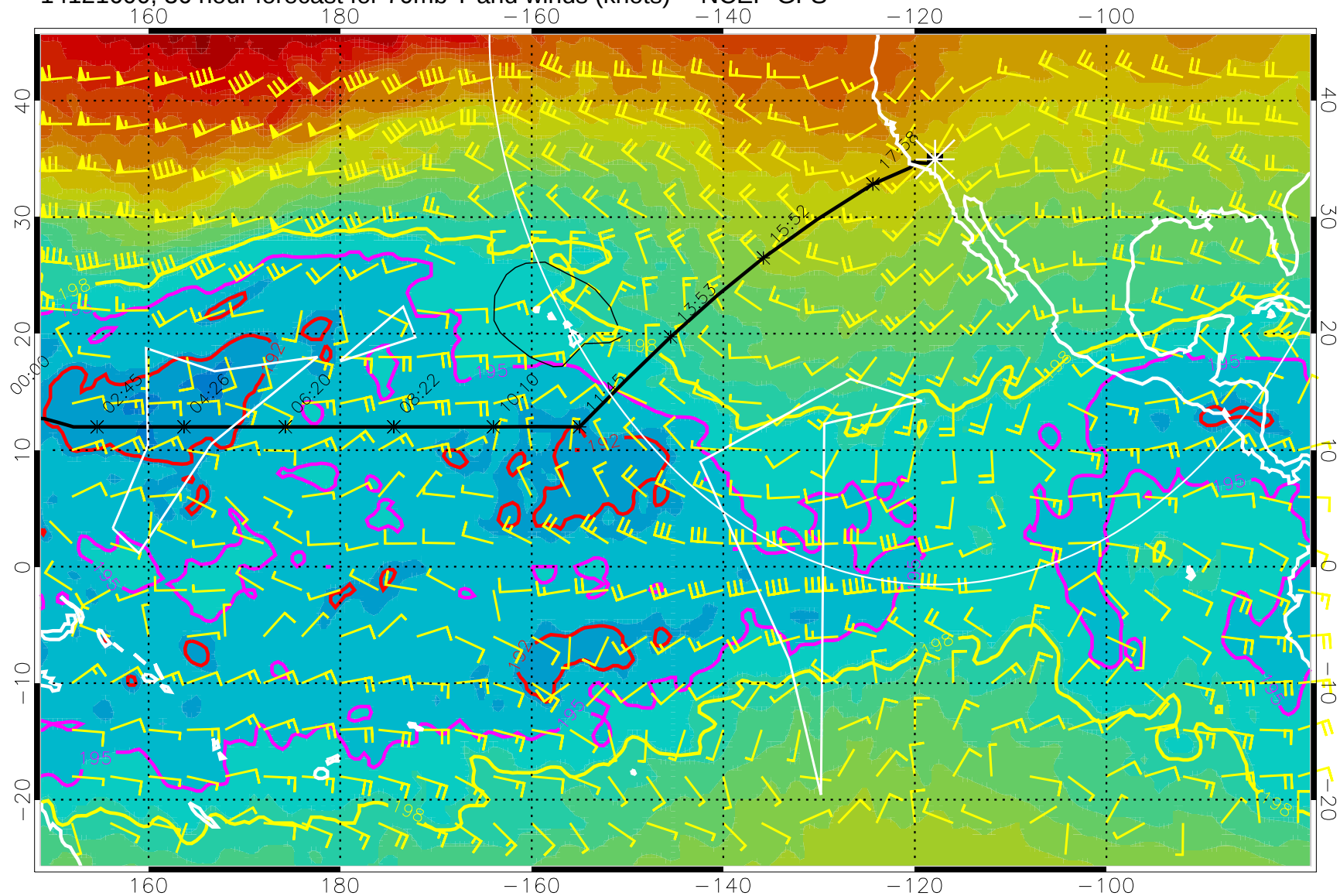
14121600, 36 hour forecast for 70mb T and winds (knots) -- NCEP GFS
