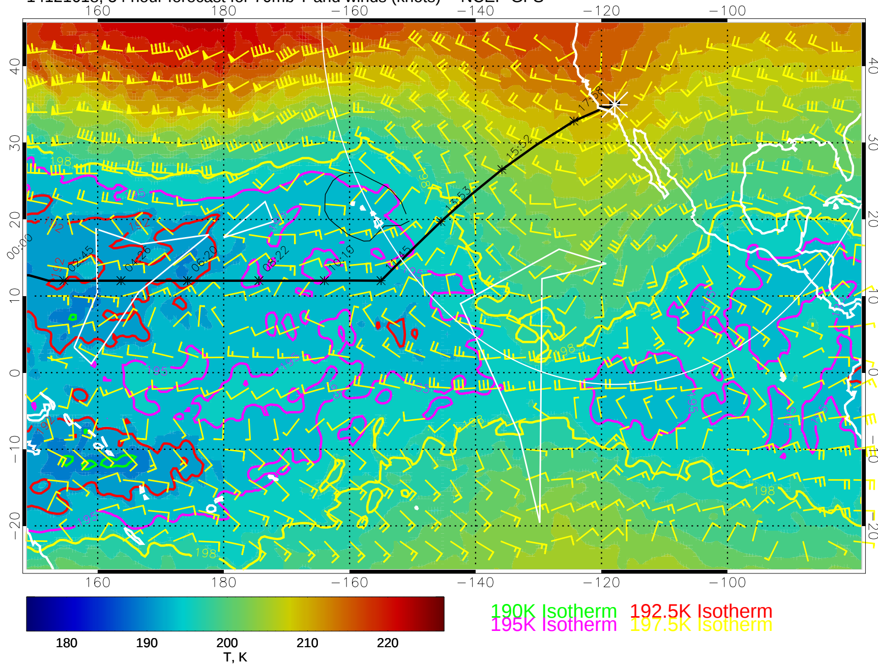
14121618, 54 hour forecast for 70mb T and winds (knots) -- NCEP GFS
