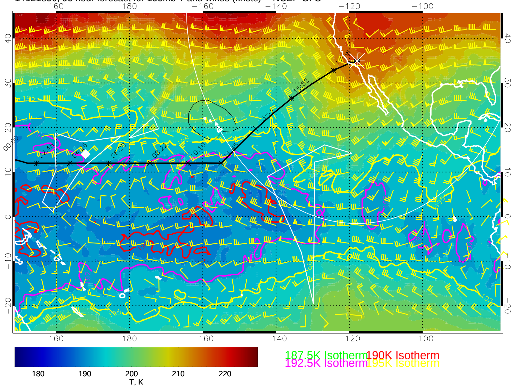
14121806, 90 hour forecast for 100mb T and winds (knots) -- NCEP GFS
