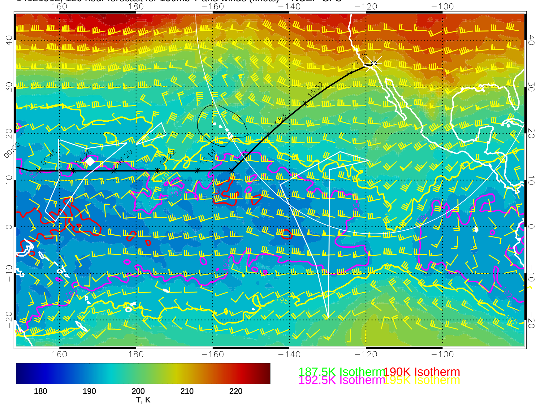
14121912, 120 hour forecast for 100mb T and winds (knots) -- NCEP GFS
