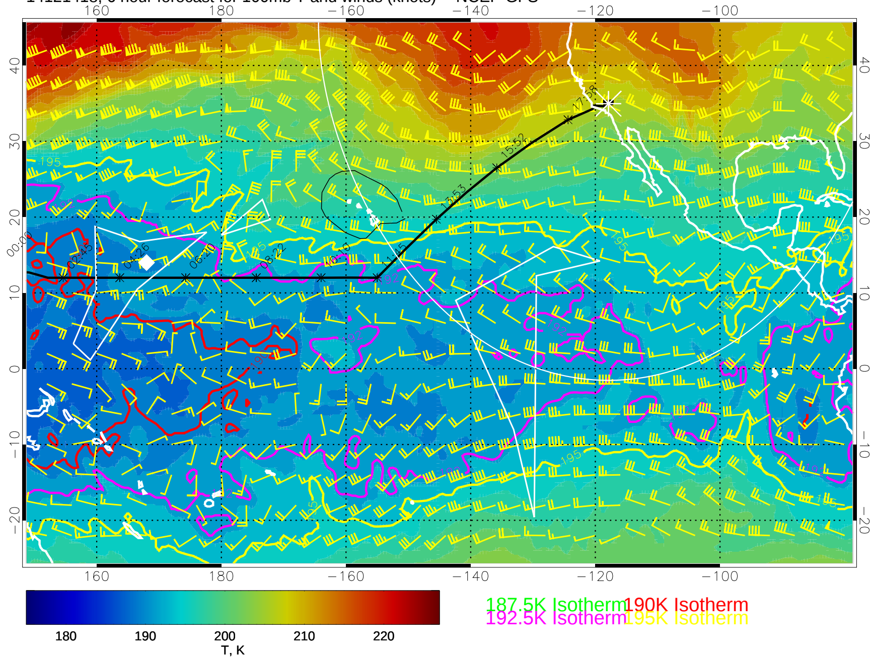
14121418, 6 hour forecast for 100mb T and winds (knots) -- NCEP GFS
