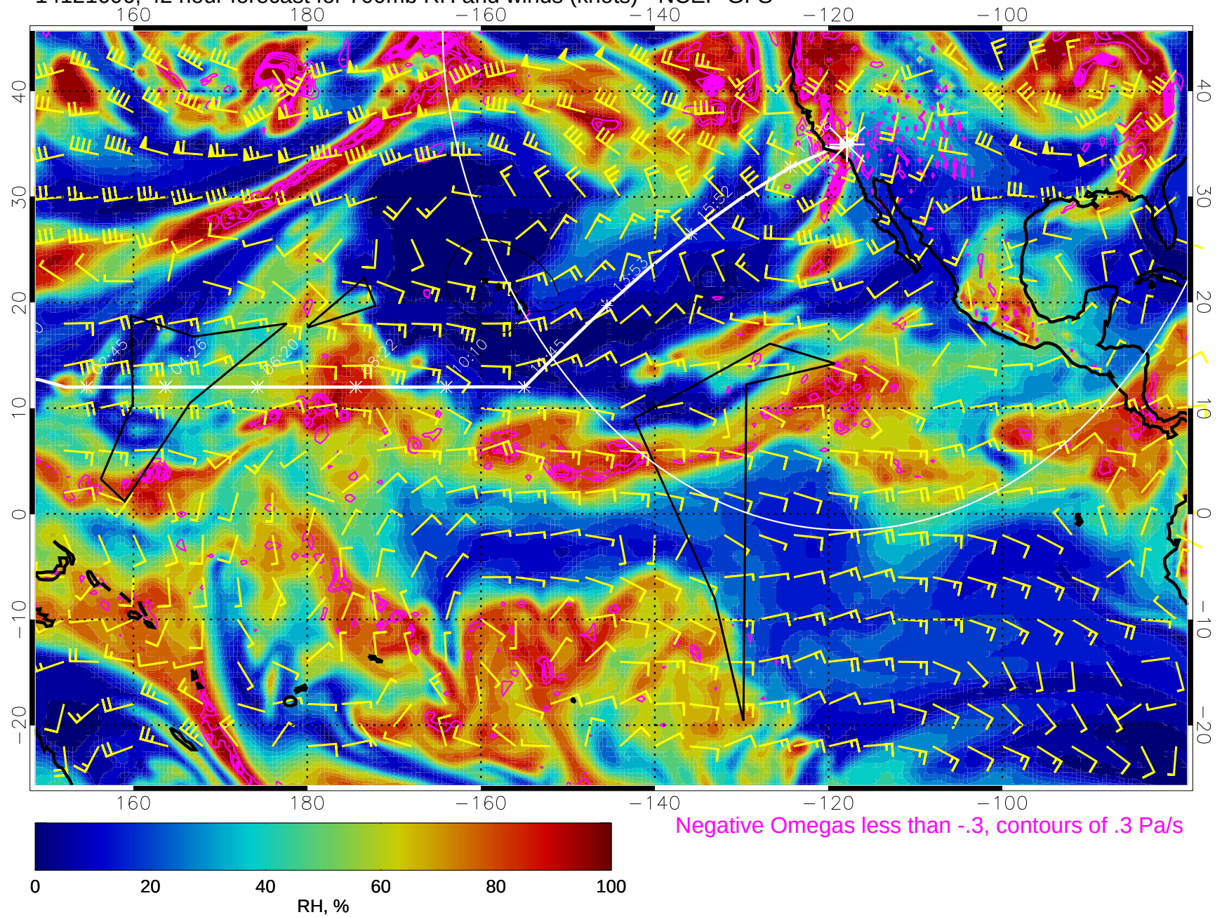
14121606, 42 hour forecast for 700mb RH and winds (knots) - NCEP GFS
