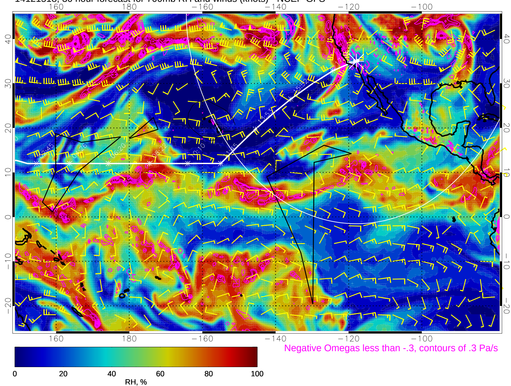
14121518, 30 hour forecast for 700mb RH and winds (knots) - NCEP GFS
