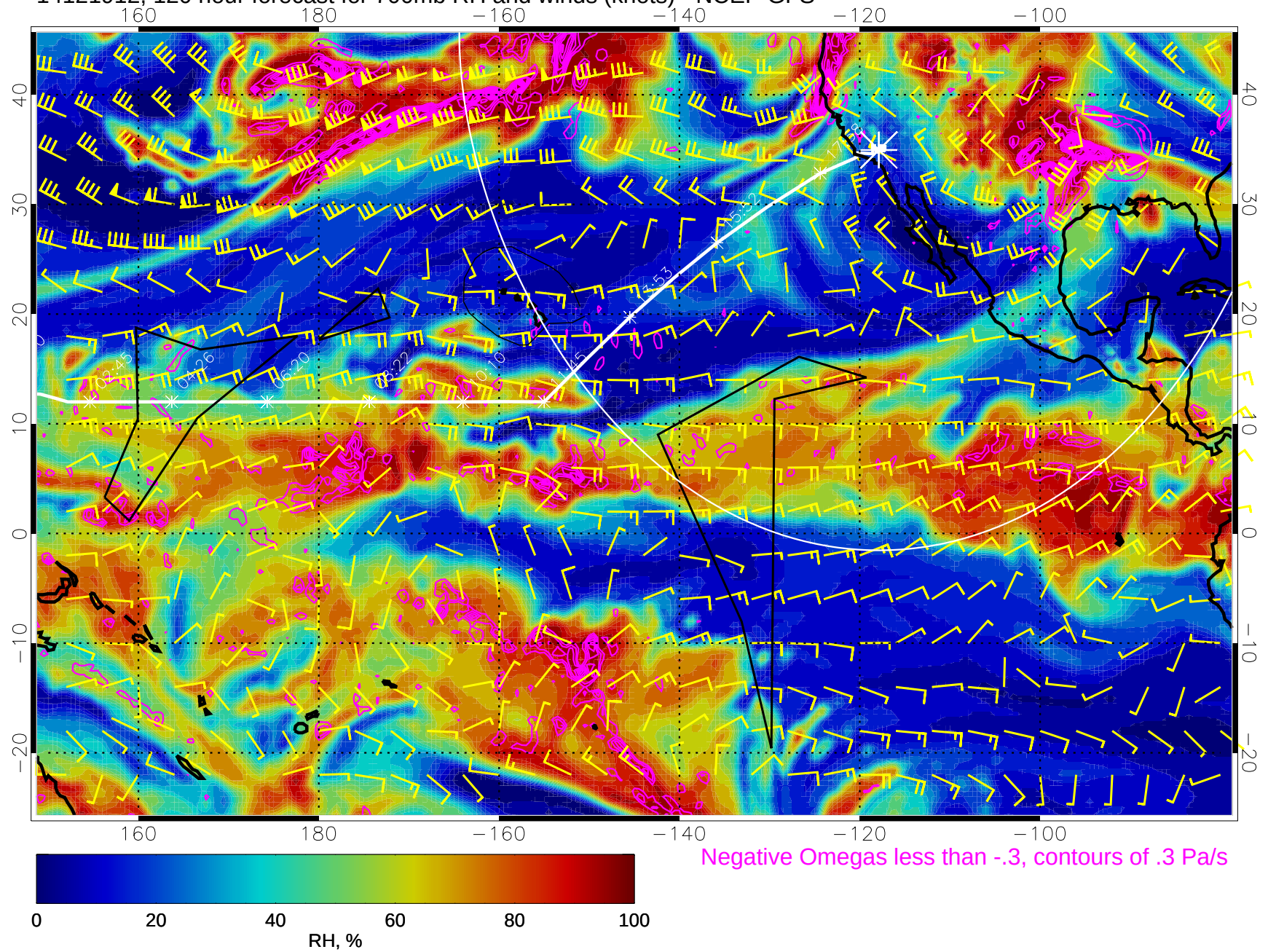
14121912, 120 hour forecast for 700mb RH and winds (knots) - NCEP GFS
