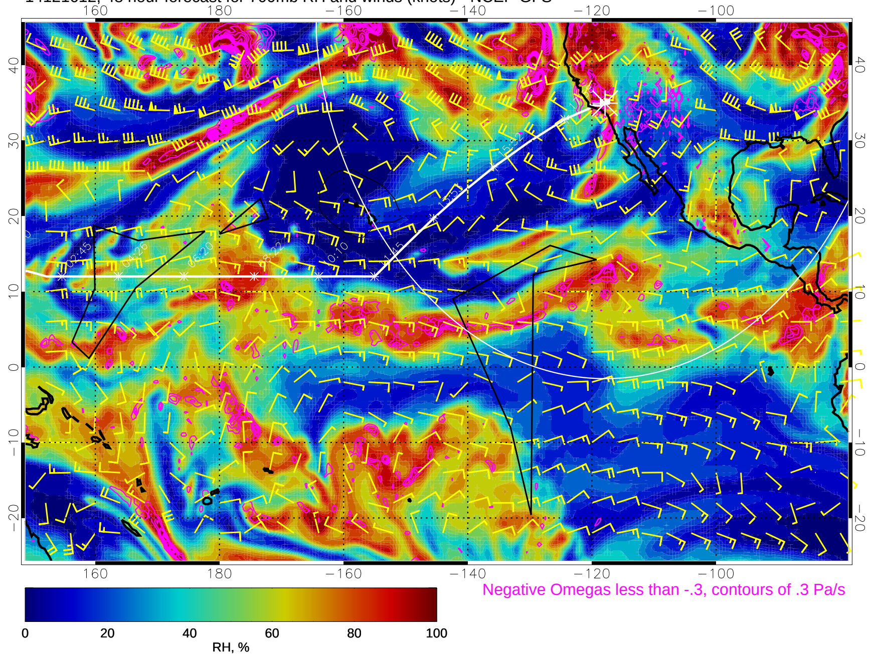
14121612, 48 hour forecast for 700mb RH and winds (knots) - NCEP GFS
