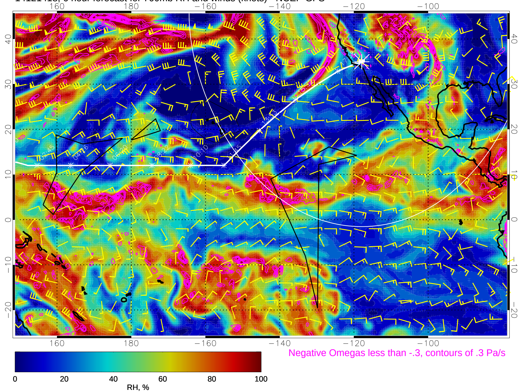
14121418, 6 hour forecast for 700mb RH and winds (knots) - NCEP GFS
