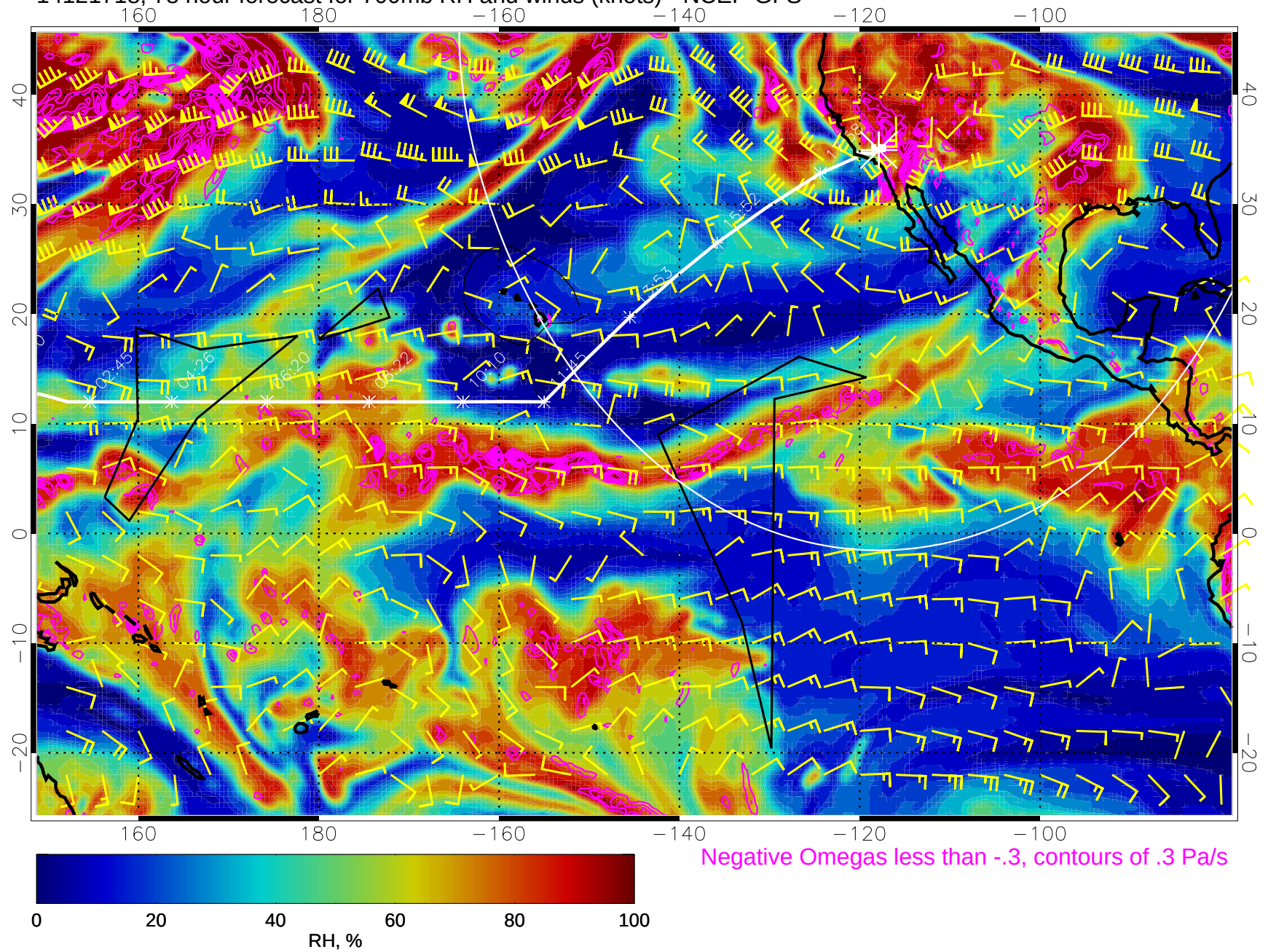
14121718, 78 hour forecast for 700mb RH and winds (knots) - NCEP GFS
