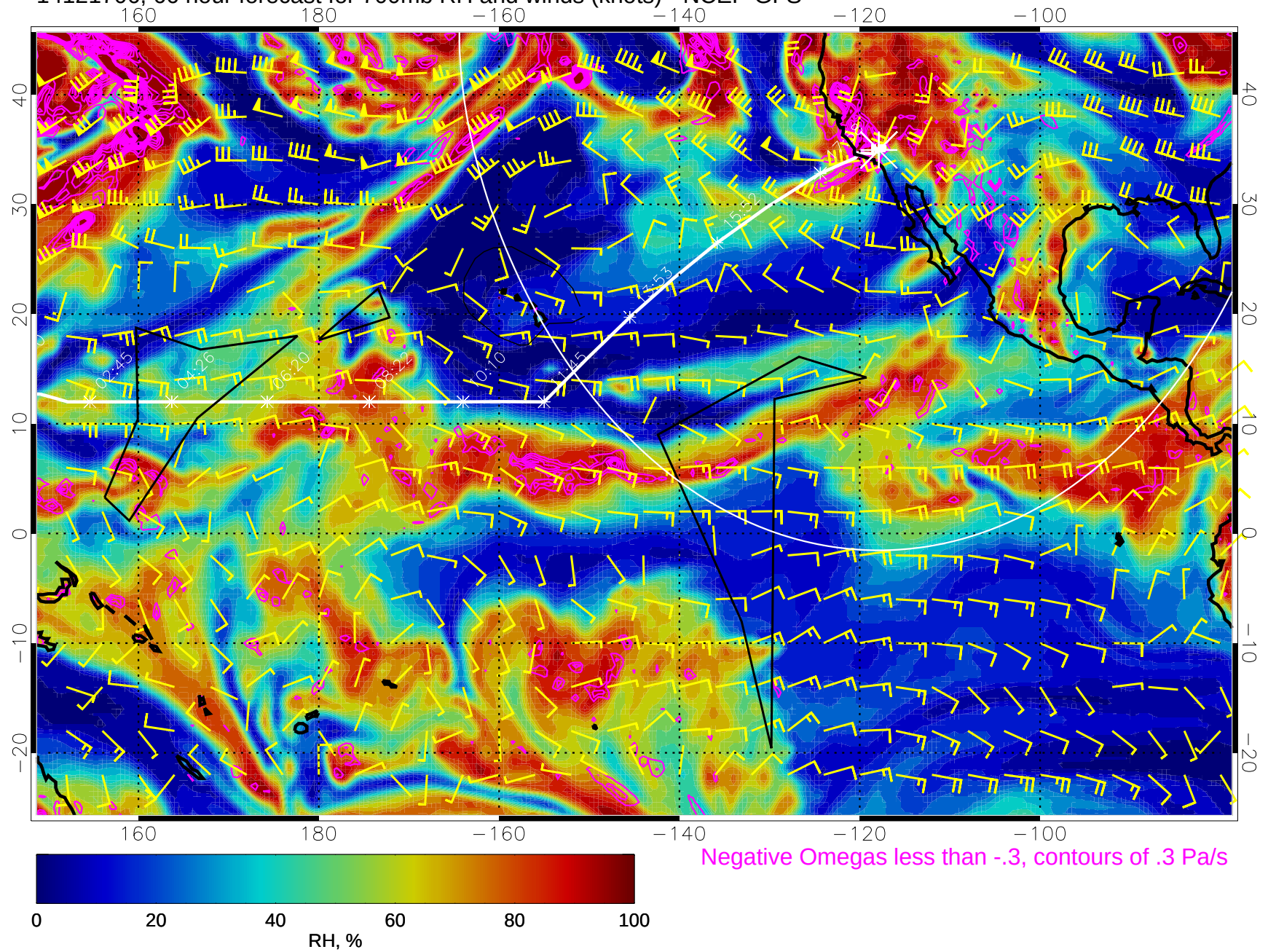
14121706, 66 hour forecast for 700mb RH and winds (knots) - NCEP GFS
