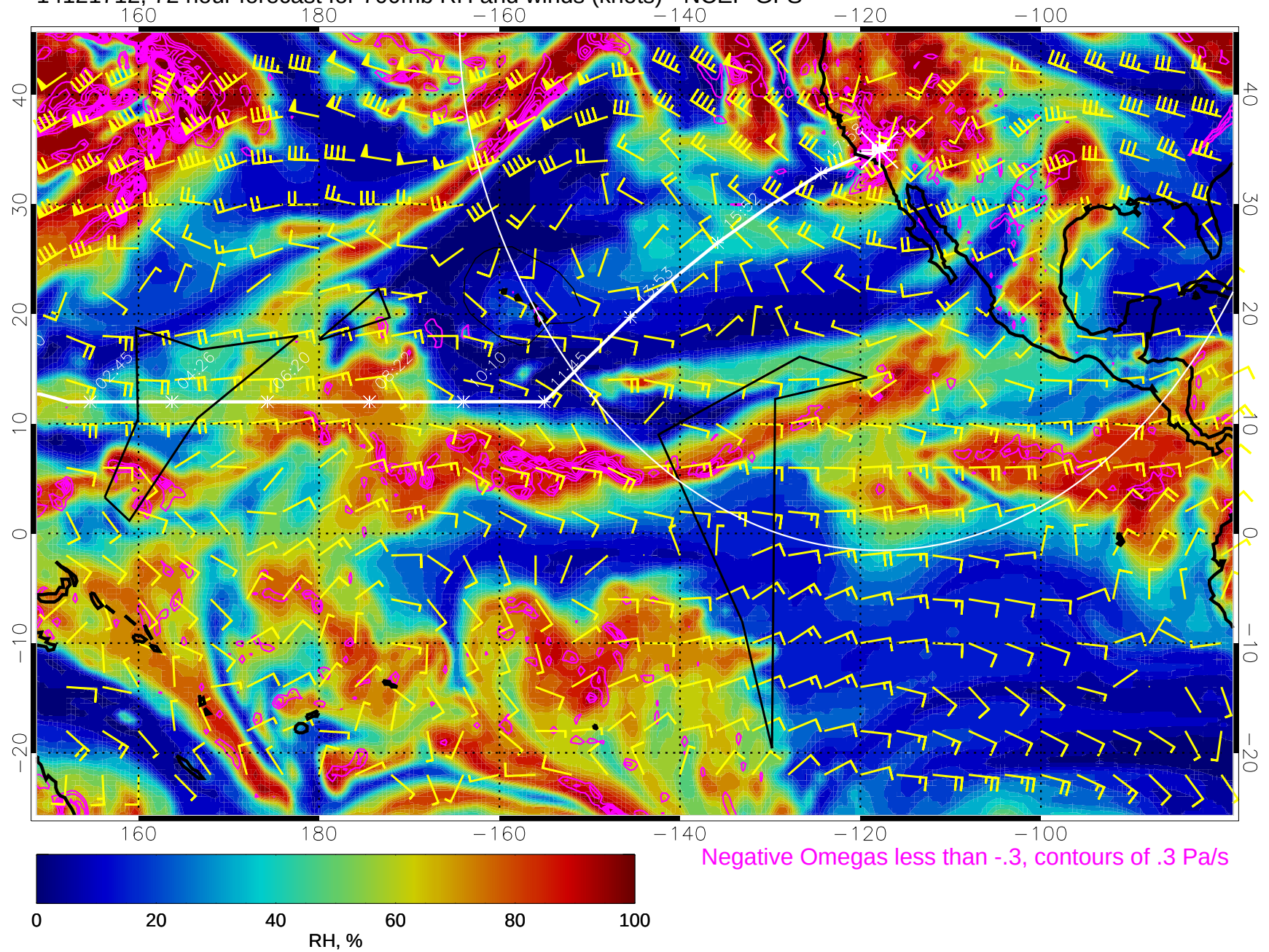
14121712, 72 hour forecast for 700mb RH and winds (knots) - NCEP GFS
