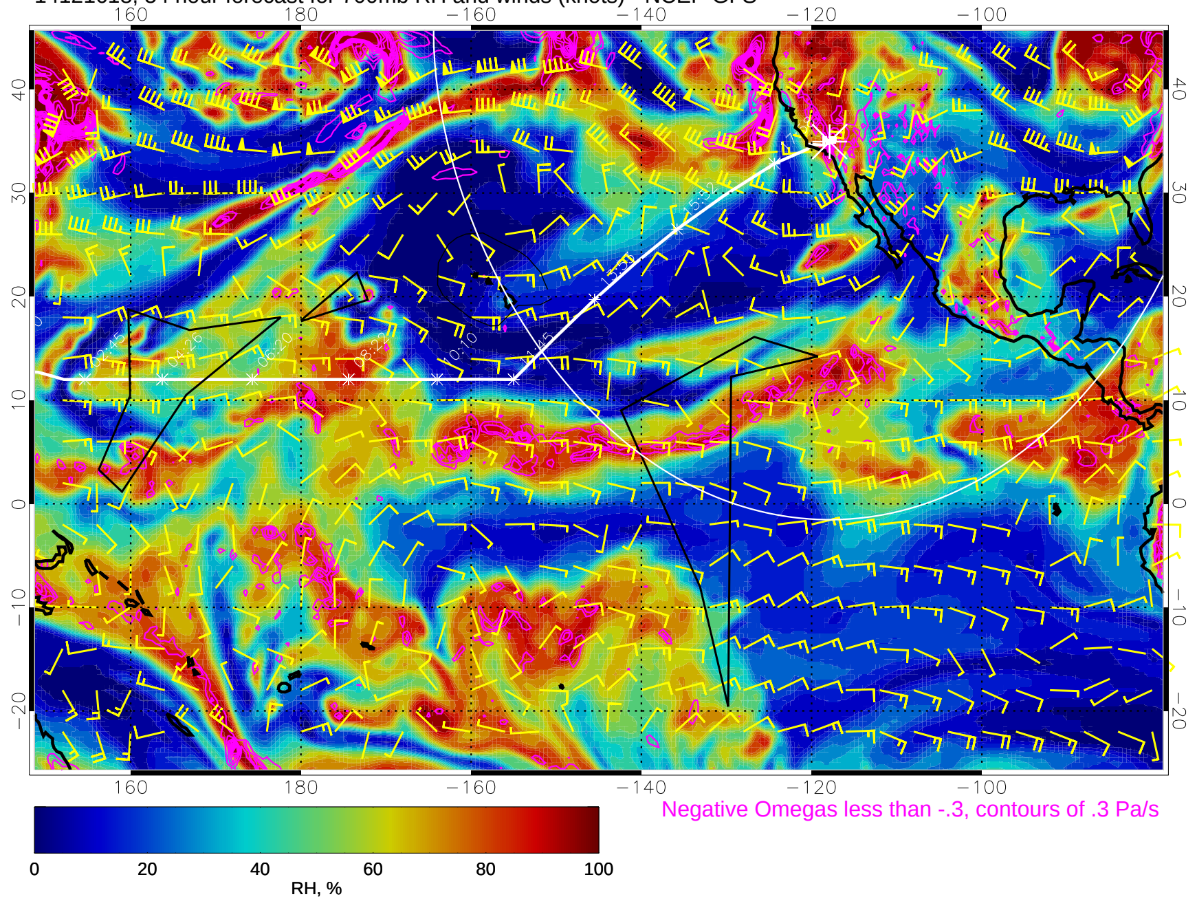
14121618, 54 hour forecast for 700mb RH and winds (knots) - NCEP GFS
