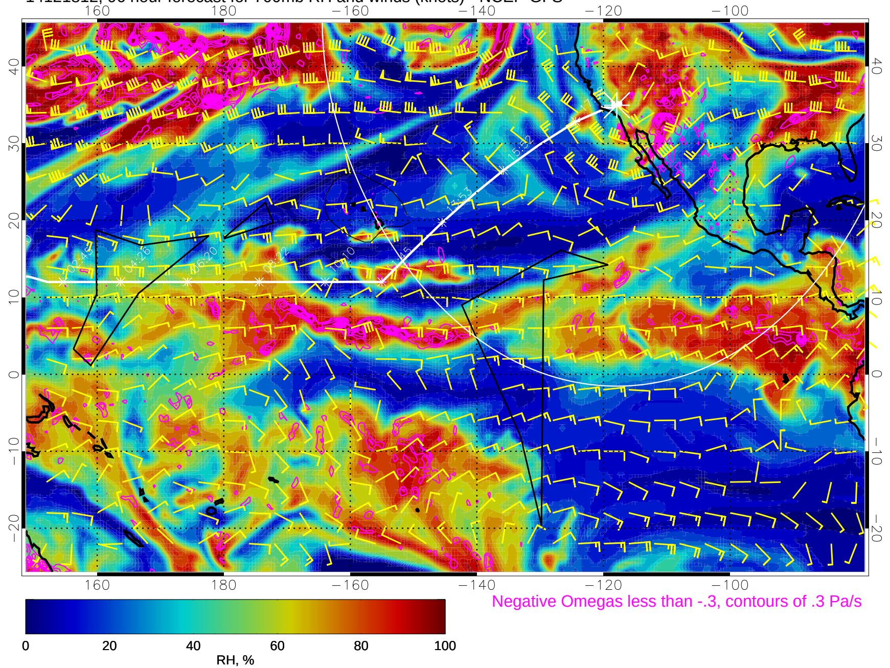
14121812, 96 hour forecast for 700mb RH and winds (knots) - NCEP GFS
