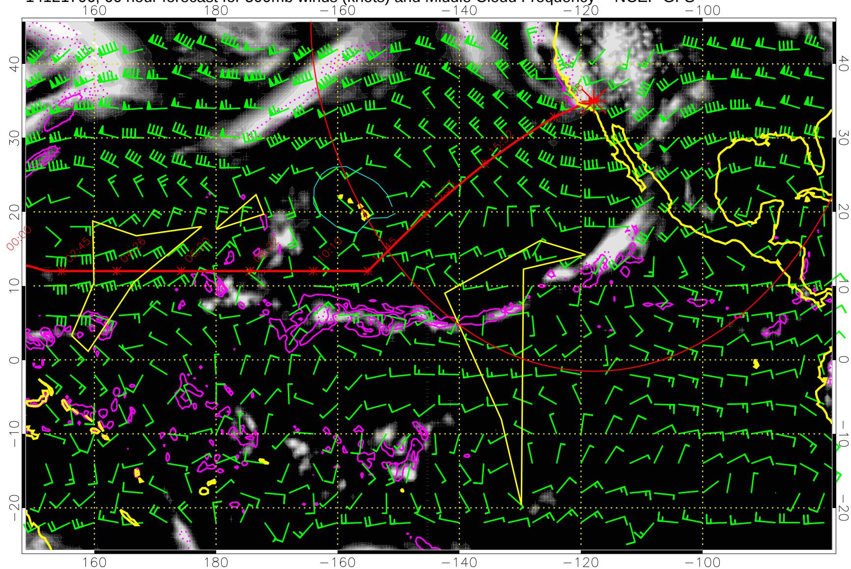
14121706, 66 hour forecast for 500mb winds (knots) and Middle Cloud Frequency -- NCEP GFS
