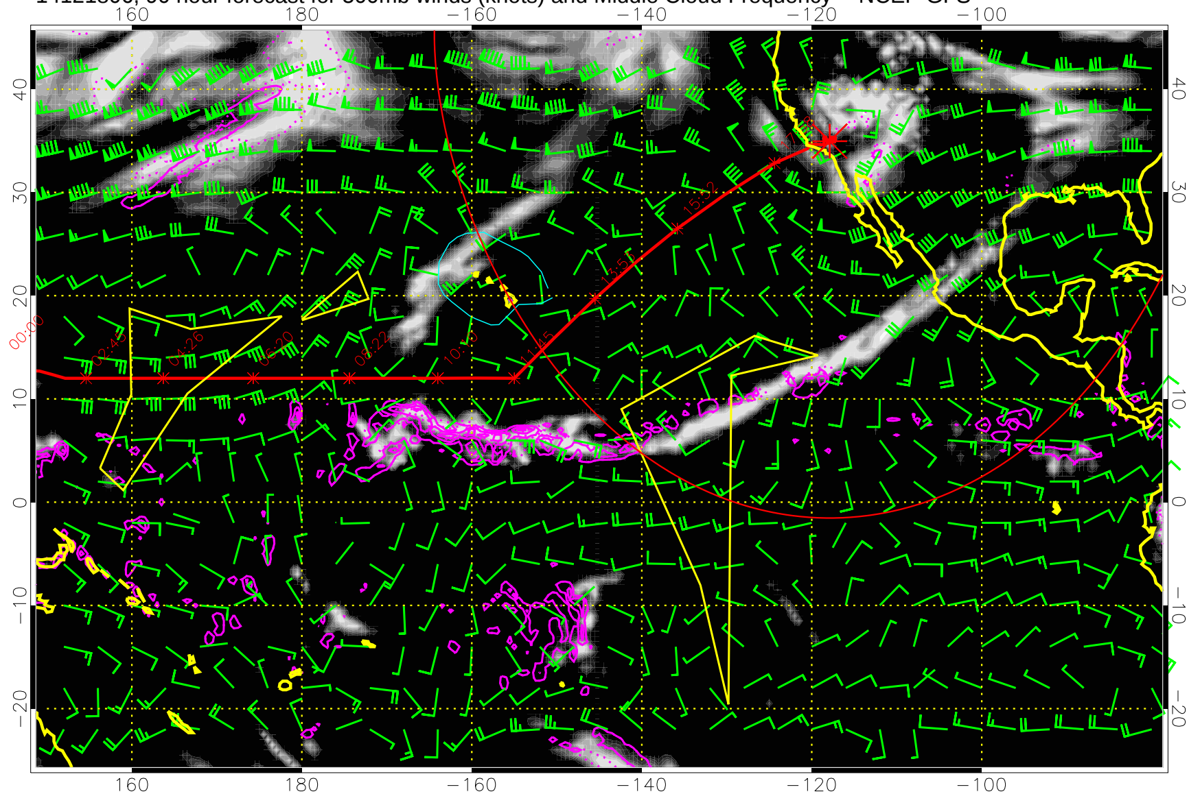
14121806, 90 hour forecast for 500mb winds (knots) and Middle Cloud Frequency -- NCEP GFS
