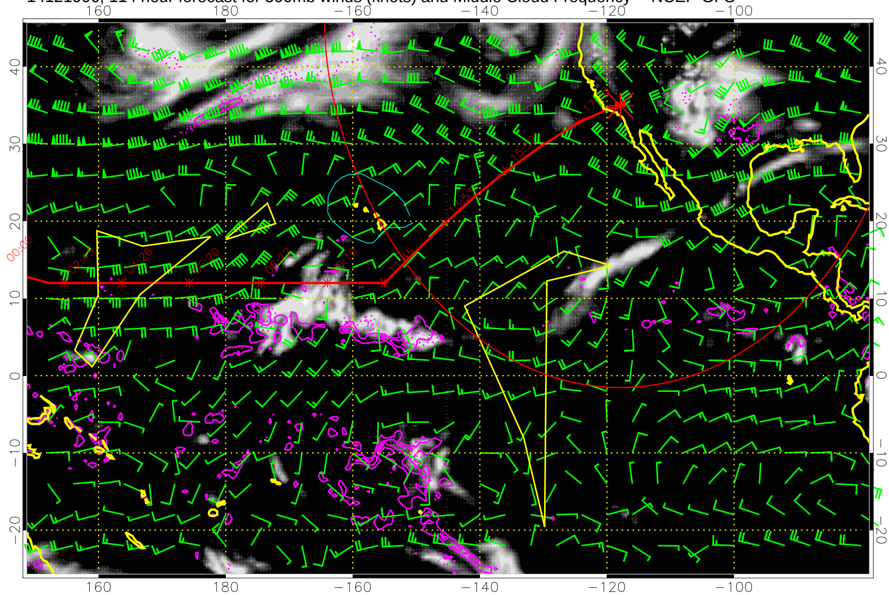
14121906, 114 hour forecast for 500mb winds (knots) and Middle Cloud Frequency -- NCEP GFS
