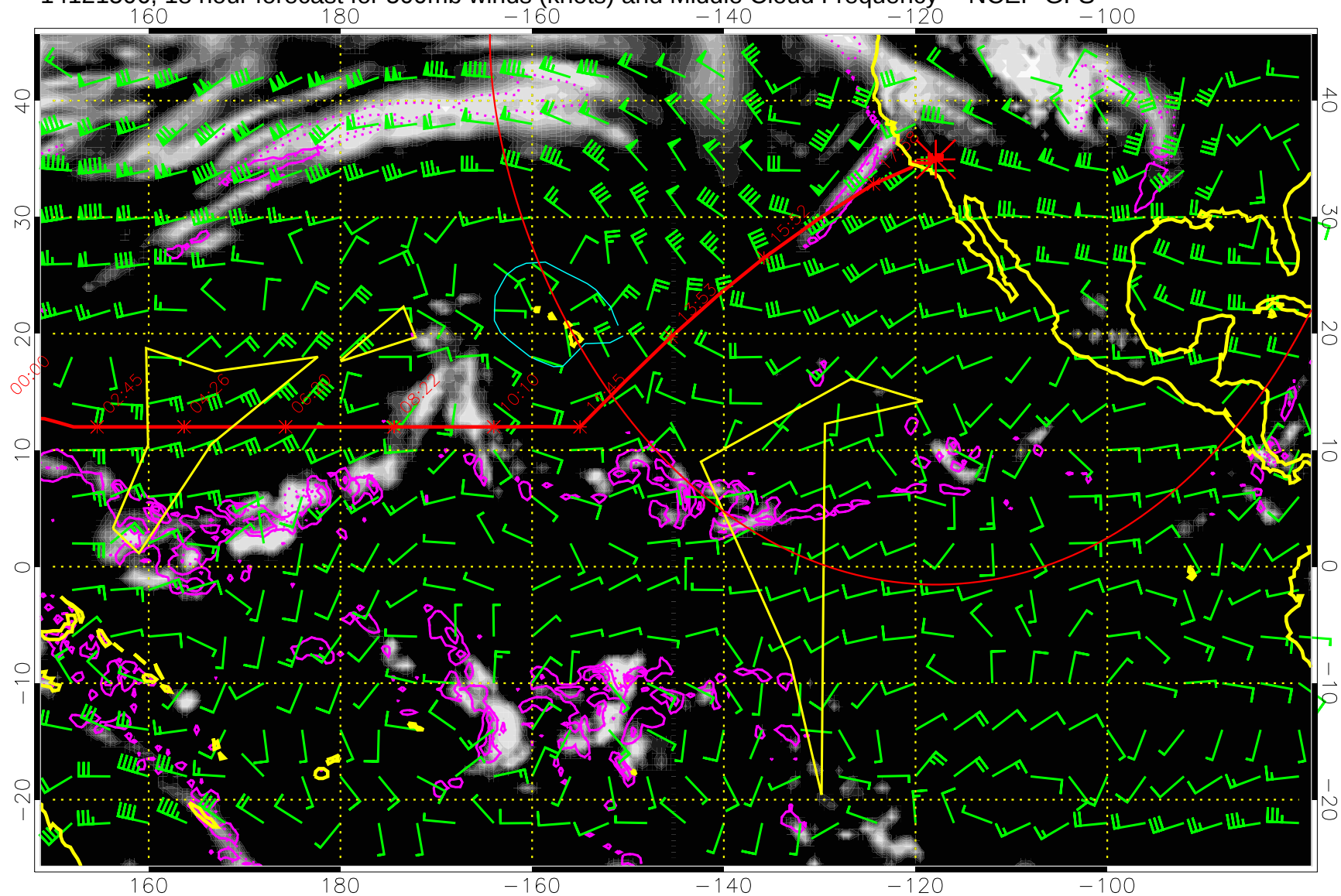
14121506, 18 hour forecast for 500mb winds (knots) and Middle Cloud Frequency -- NCEP GFS
