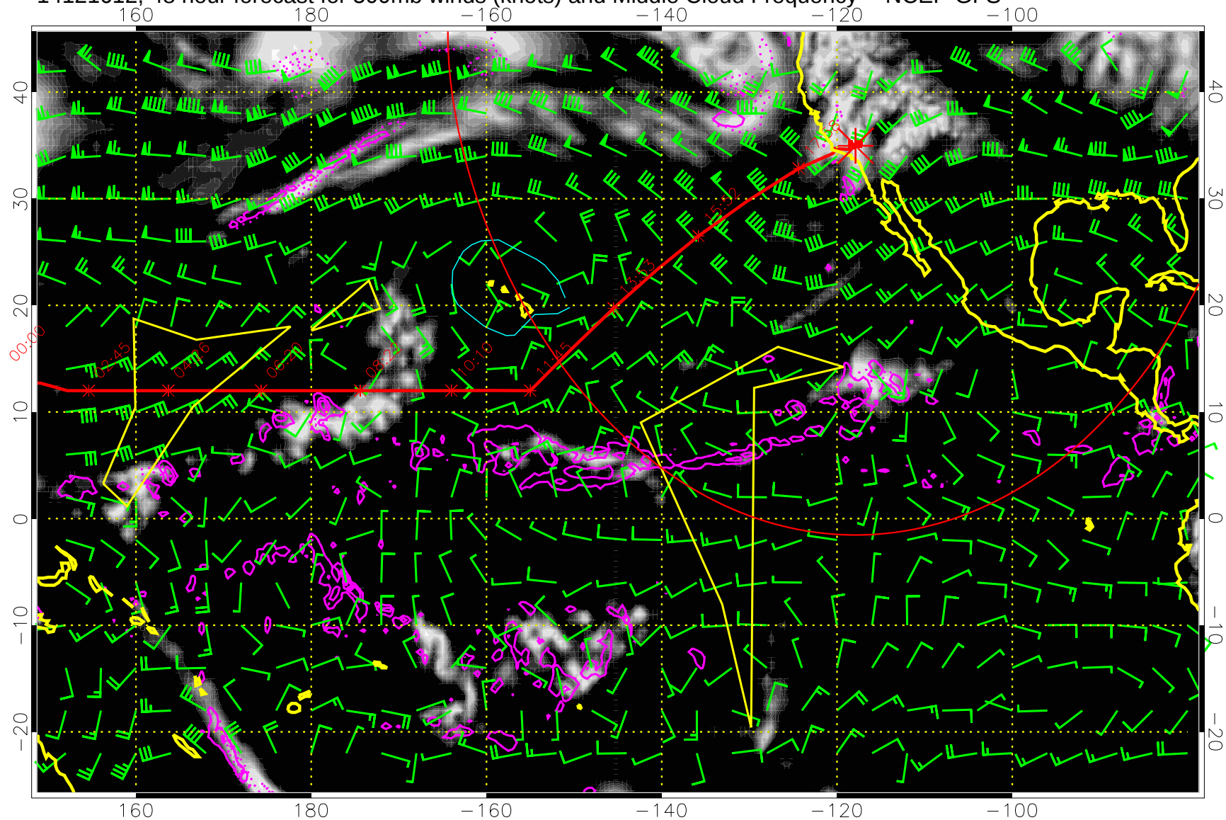
14121612, 48 hour forecast for 500mb winds (knots) and Middle Cloud Frequency -- NCEP GFS
