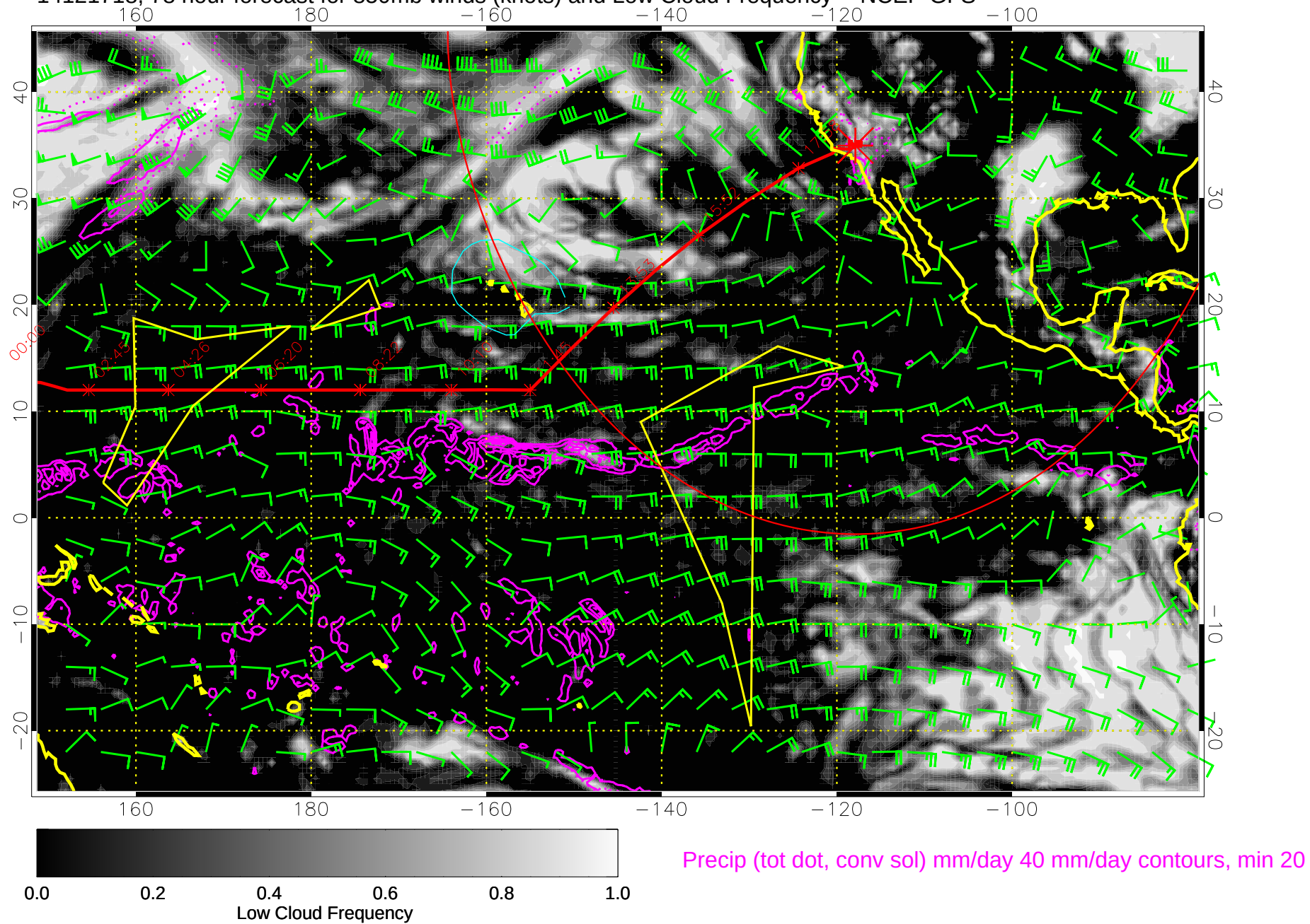
14121718, 78 hour forecast for 850mb winds (knots) and Low Cloud Frequency -- NCEP GFS
