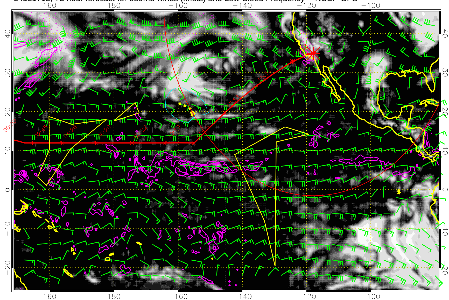
14121712, 72 hour forecast for 850mb winds (knots) and Low Cloud Frequency -- NCEP GFS
