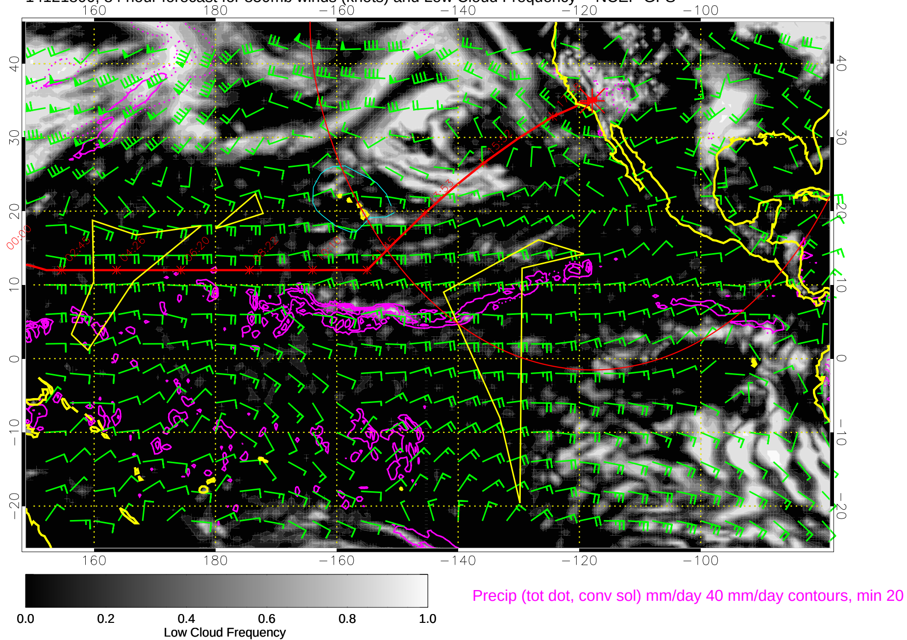
14121800, 84 hour forecast for 850mb winds (knots) and Low Cloud Frequency -- NCEP GFS
