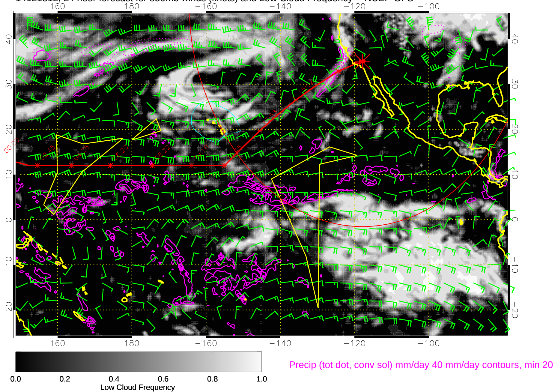
14121512, 24 hour forecast for 850mb winds (knots) and Low Cloud Frequency -- NCEP GFS
