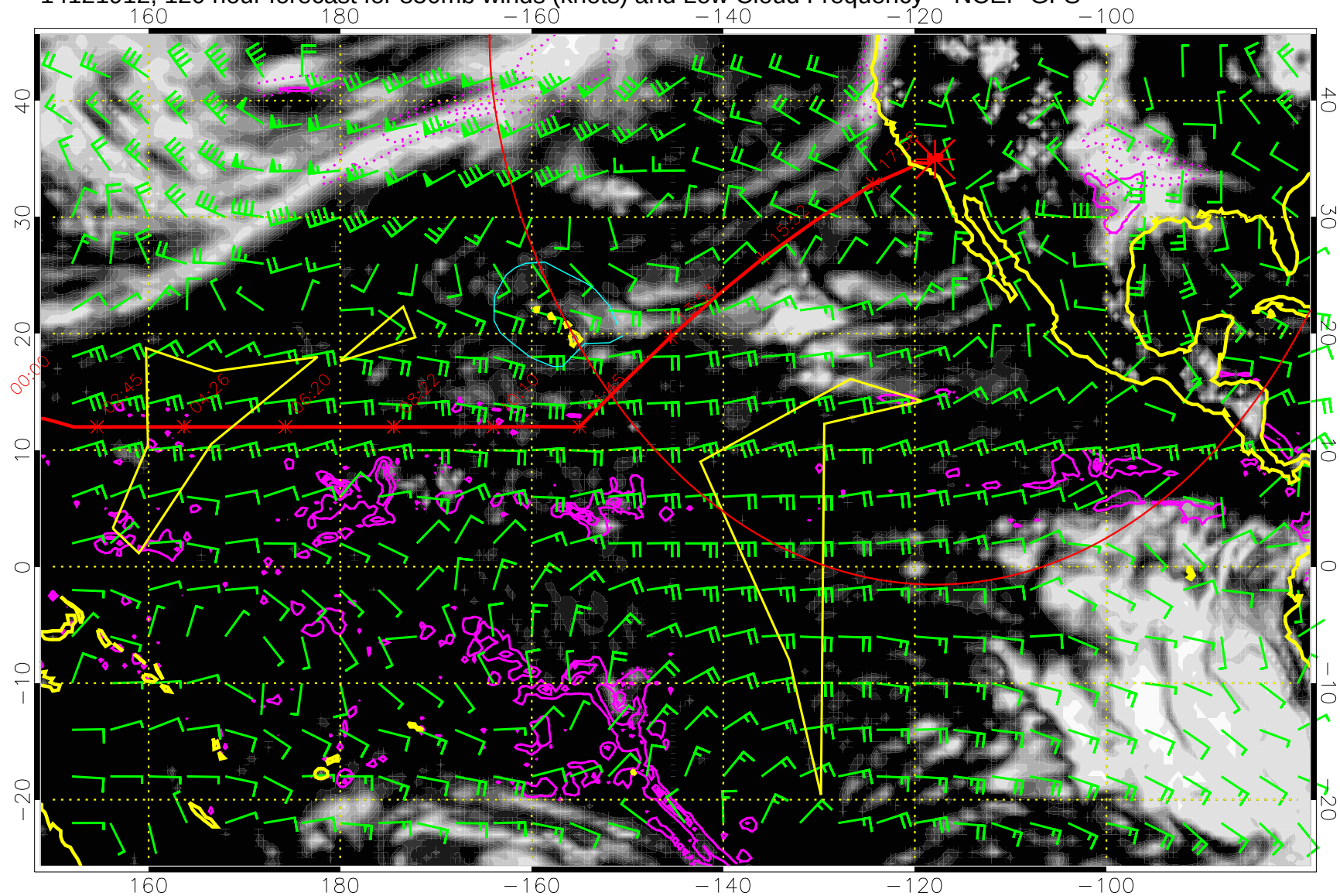
14121912, 120 hour forecast for 850mb winds (knots) and Low Cloud Frequency -- NCEP GFS
