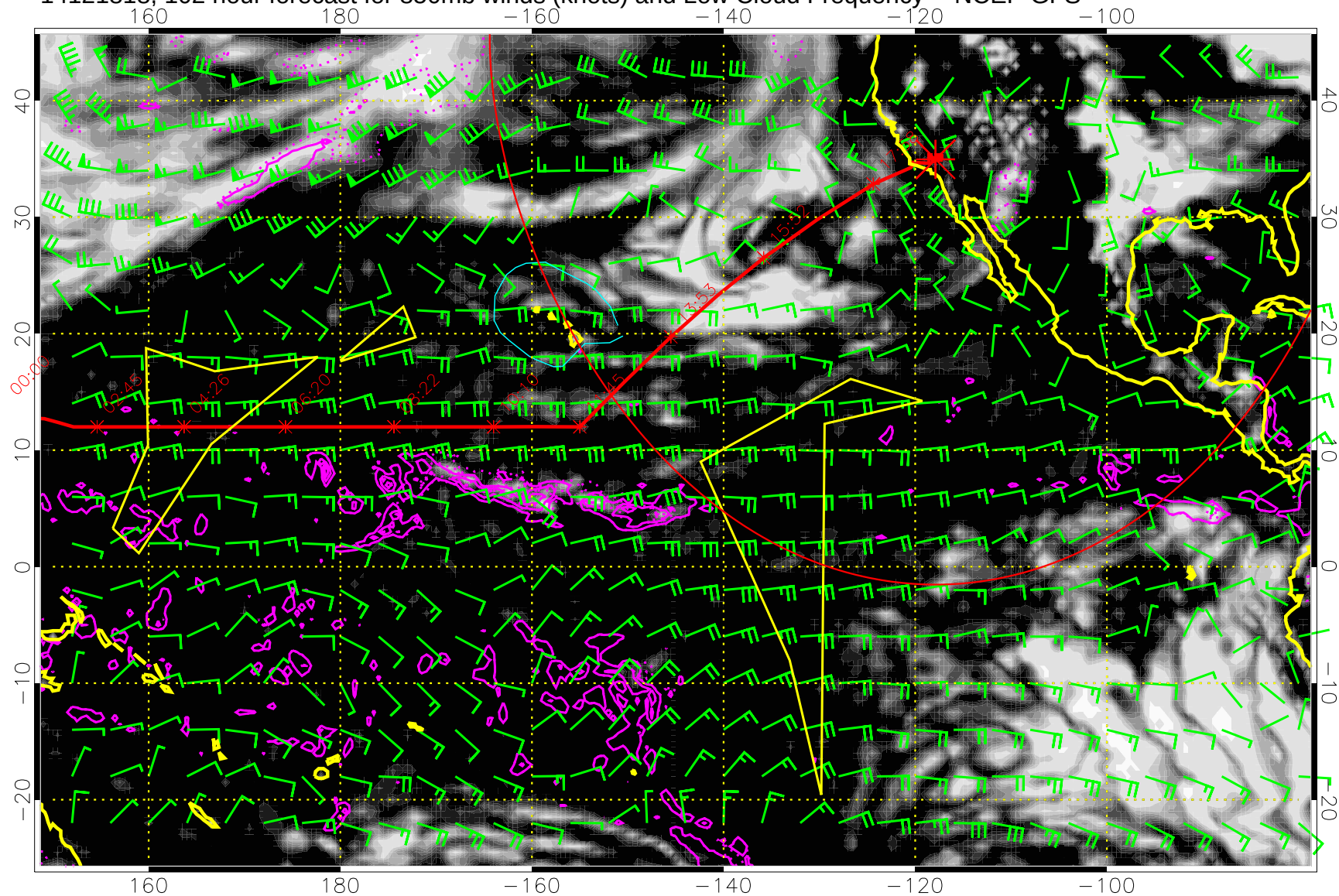
14121818, 102 hour forecast for 850mb winds (knots) and Low Cloud Frequency -- NCEP GFS
