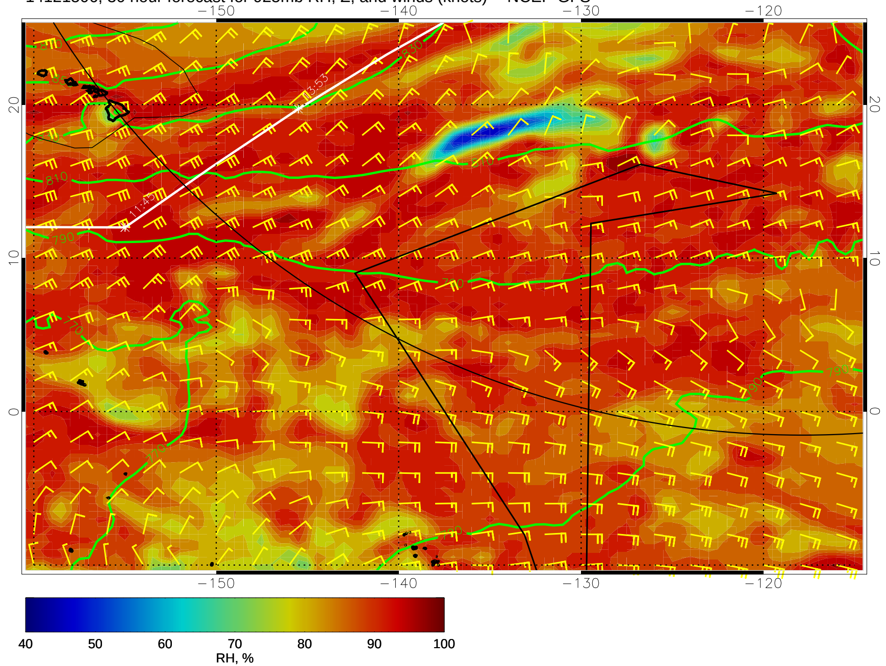
14121506, 30 hour forecast for 925mb RH, Z, and winds (knots) -- NCEP GFS
