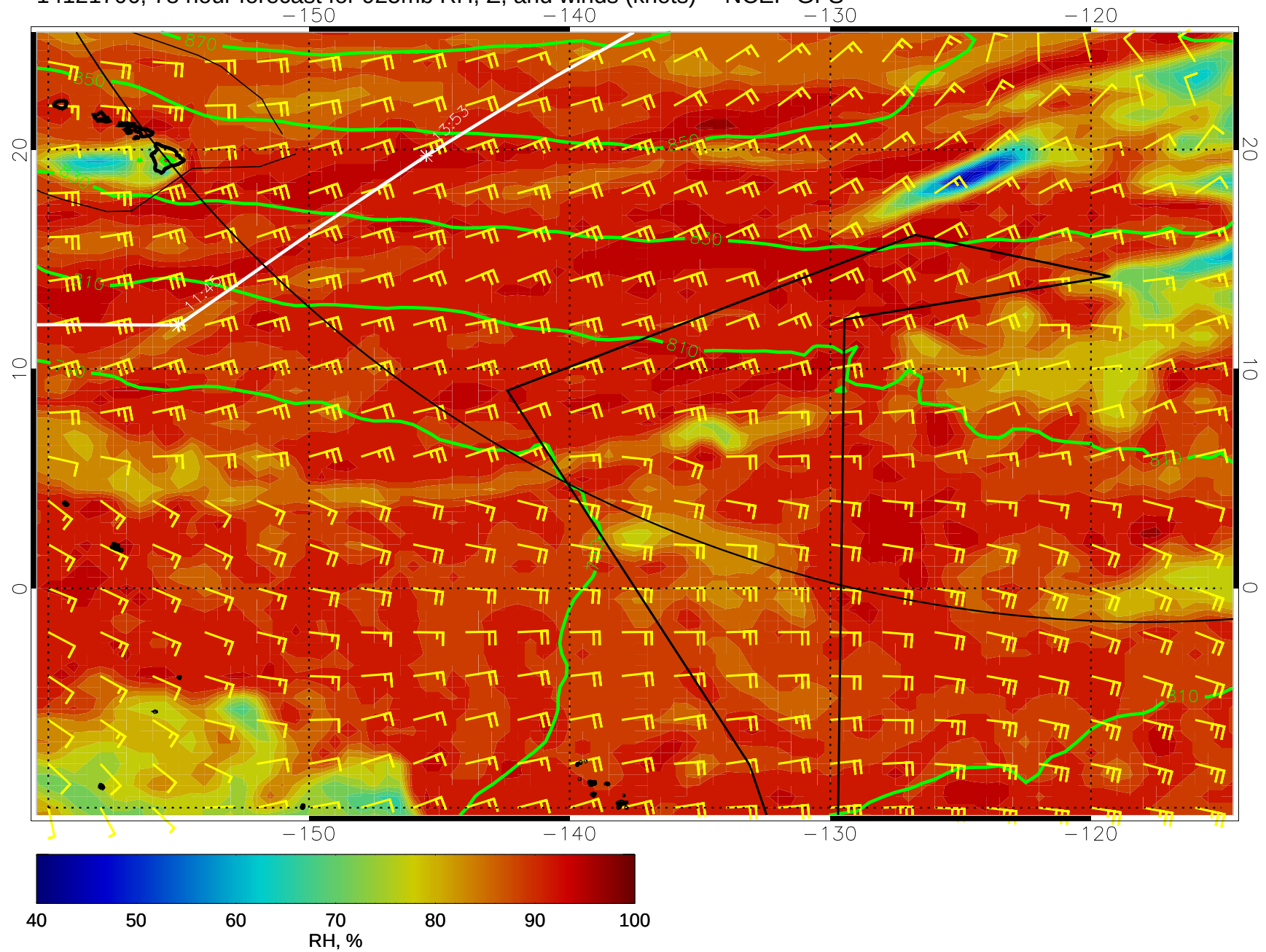
14121706, 78 hour forecast for 925mb RH, Z, and winds (knots) -- NCEP GFS
