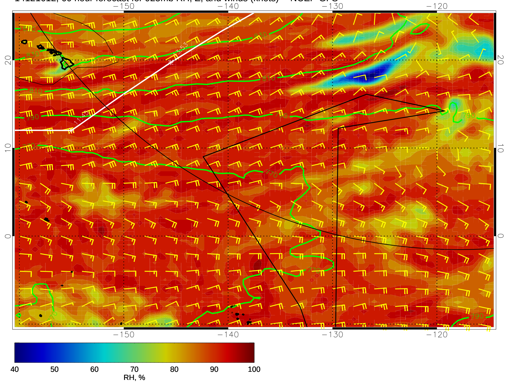
14121612, 60 hour forecast for 925mb RH, Z, and winds (knots) -- NCEP GFS
