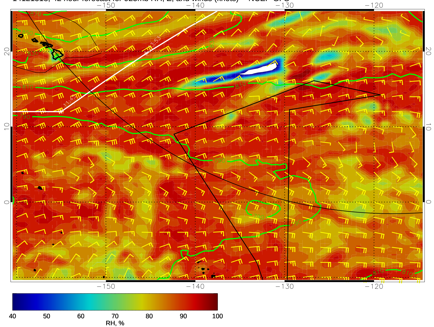
14121518, 42 hour forecast for 925mb RH, Z, and winds (knots) -- NCEP GFS
