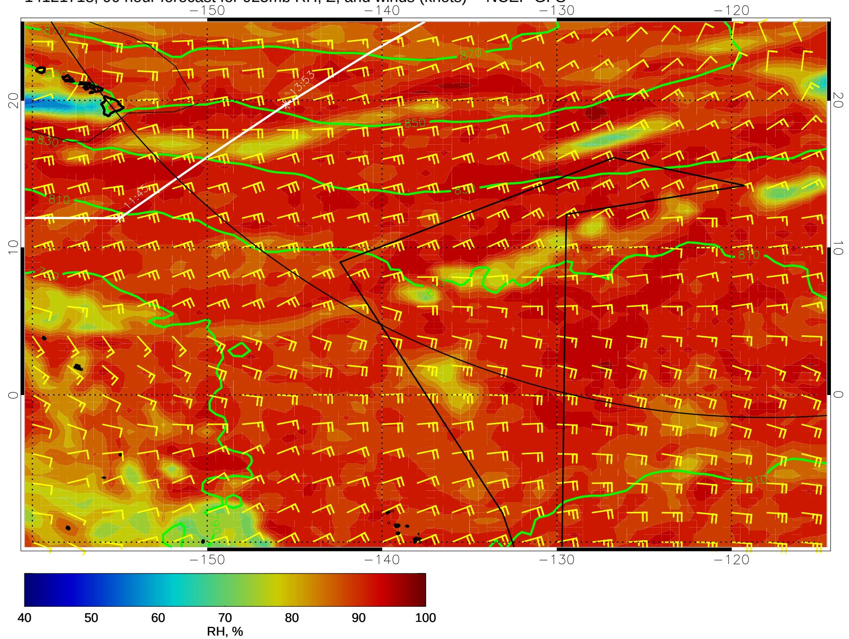
14121718, 90 hour forecast for 925mb RH, Z, and winds (knots) -- NCEP GFS
