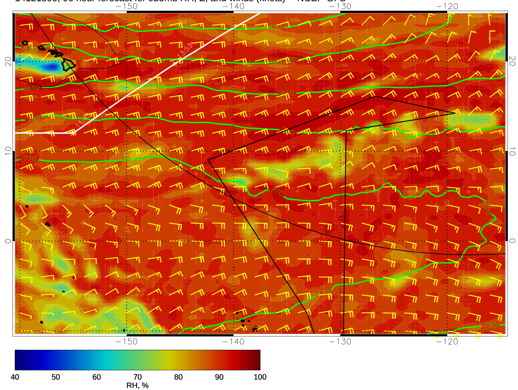
14121800, 96 hour forecast for 925mb RH, Z, and winds (knots) -- NCEP GFS
