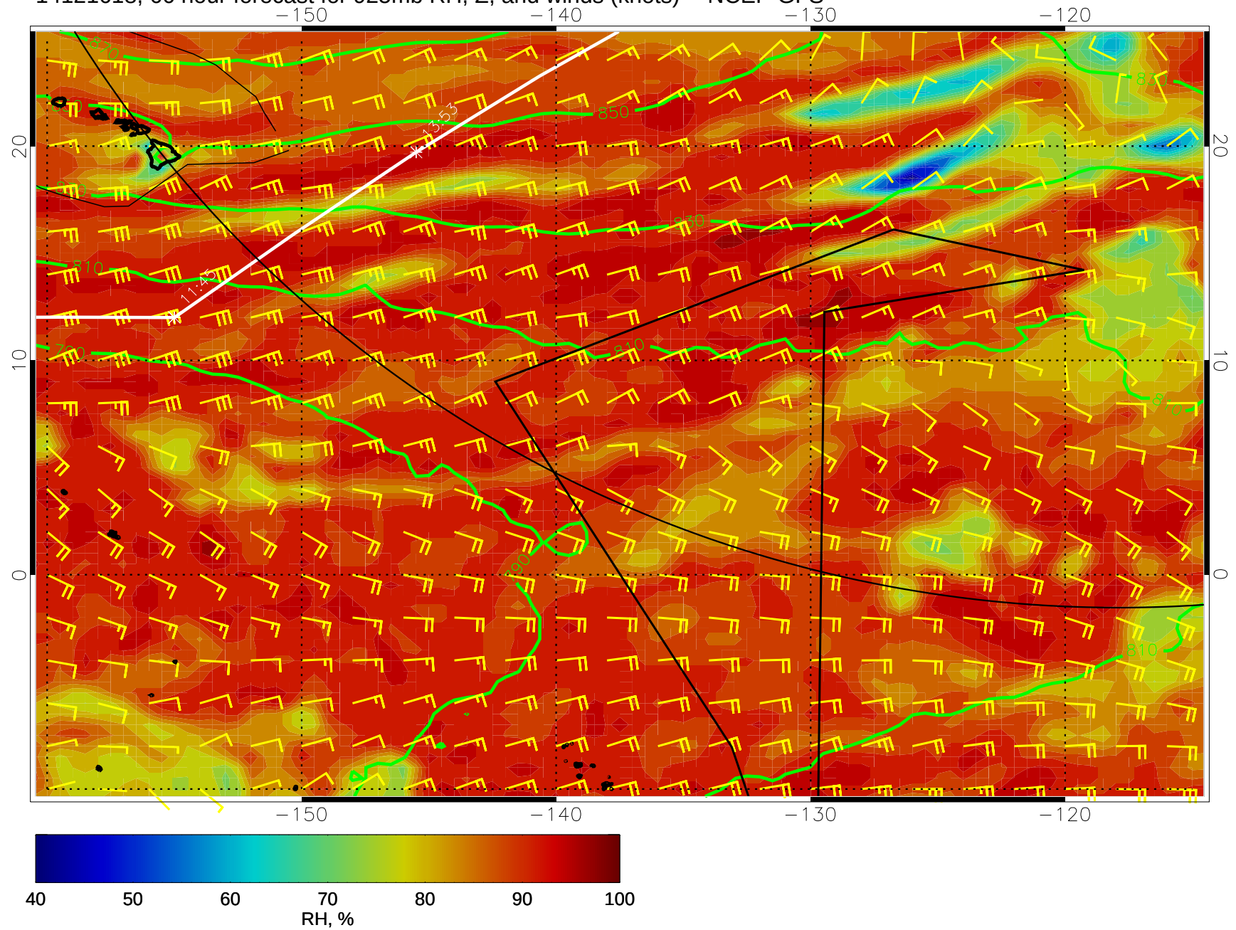
14121618, 66 hour forecast for 925mb RH, Z, and winds (knots) -- NCEP GFS
