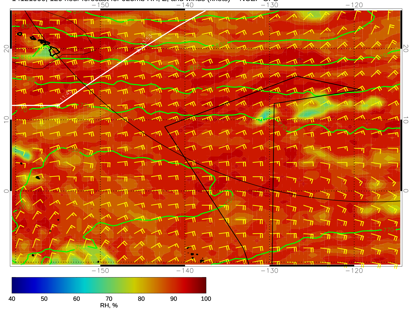
14121900, 120 hour forecast for 925mb RH, Z, and winds (knots) -- NCEP GFS
