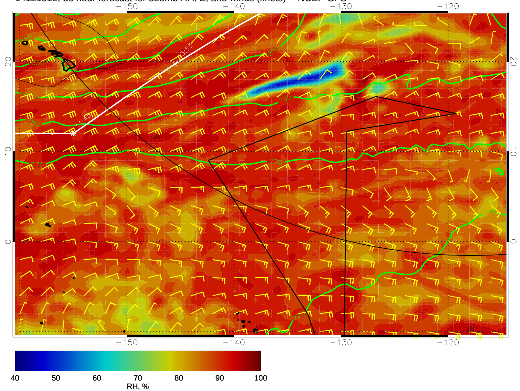
14121512, 36 hour forecast for 925mb RH, Z, and winds (knots) -- NCEP GFS
