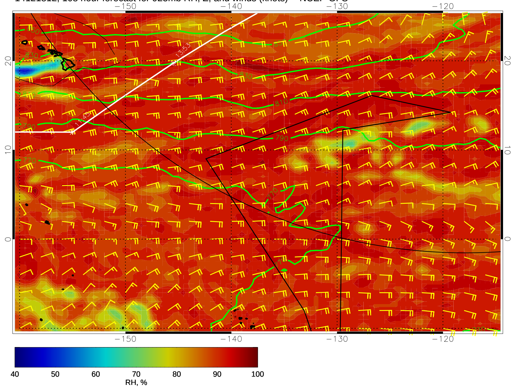
14121812, 108 hour forecast for 925mb RH, Z, and winds (knots) -- NCEP GFS
