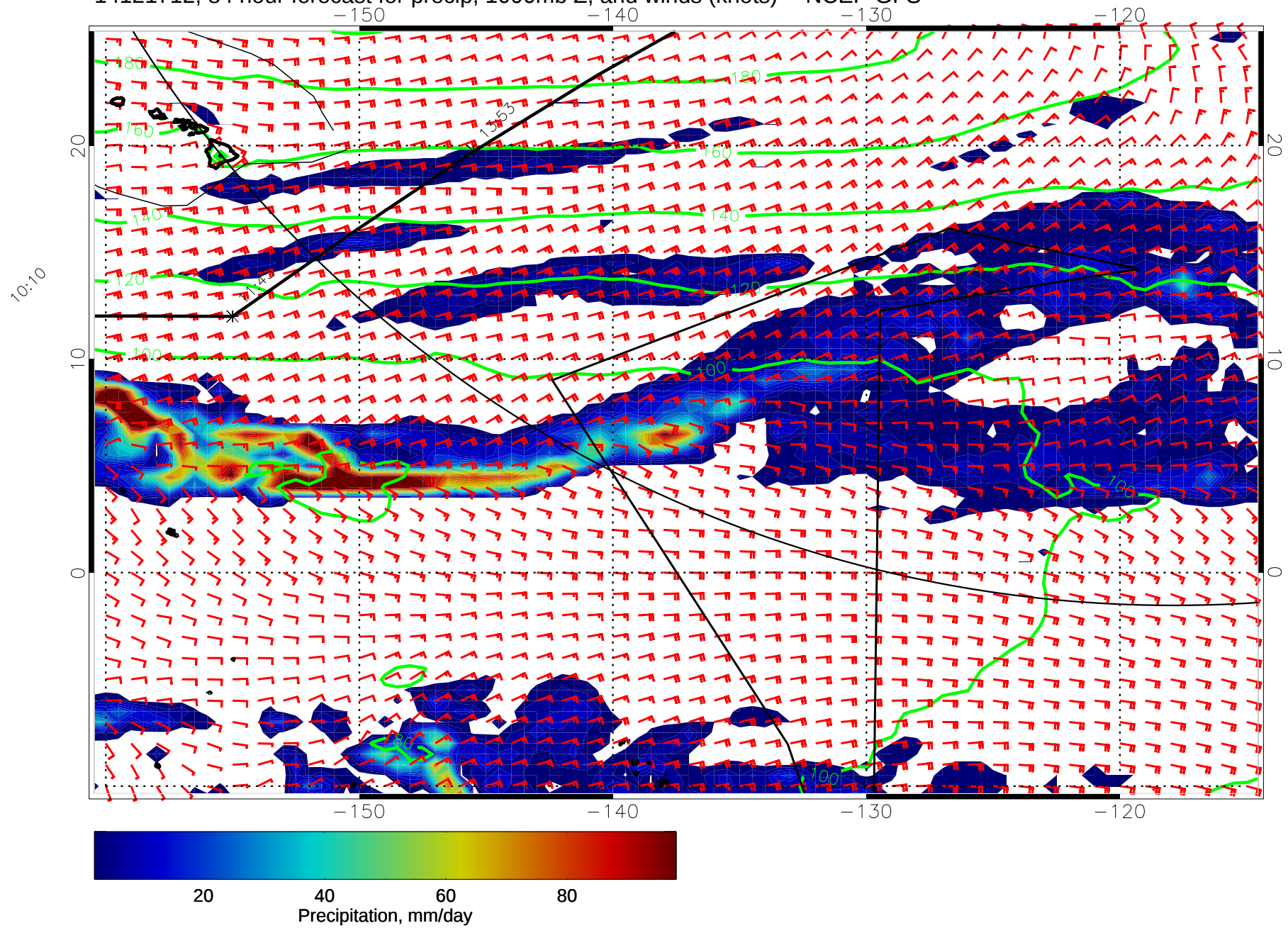
14121712, 84 hour forecast for precip, 1000mb Z, and winds (knots) -- NCEP GFS
