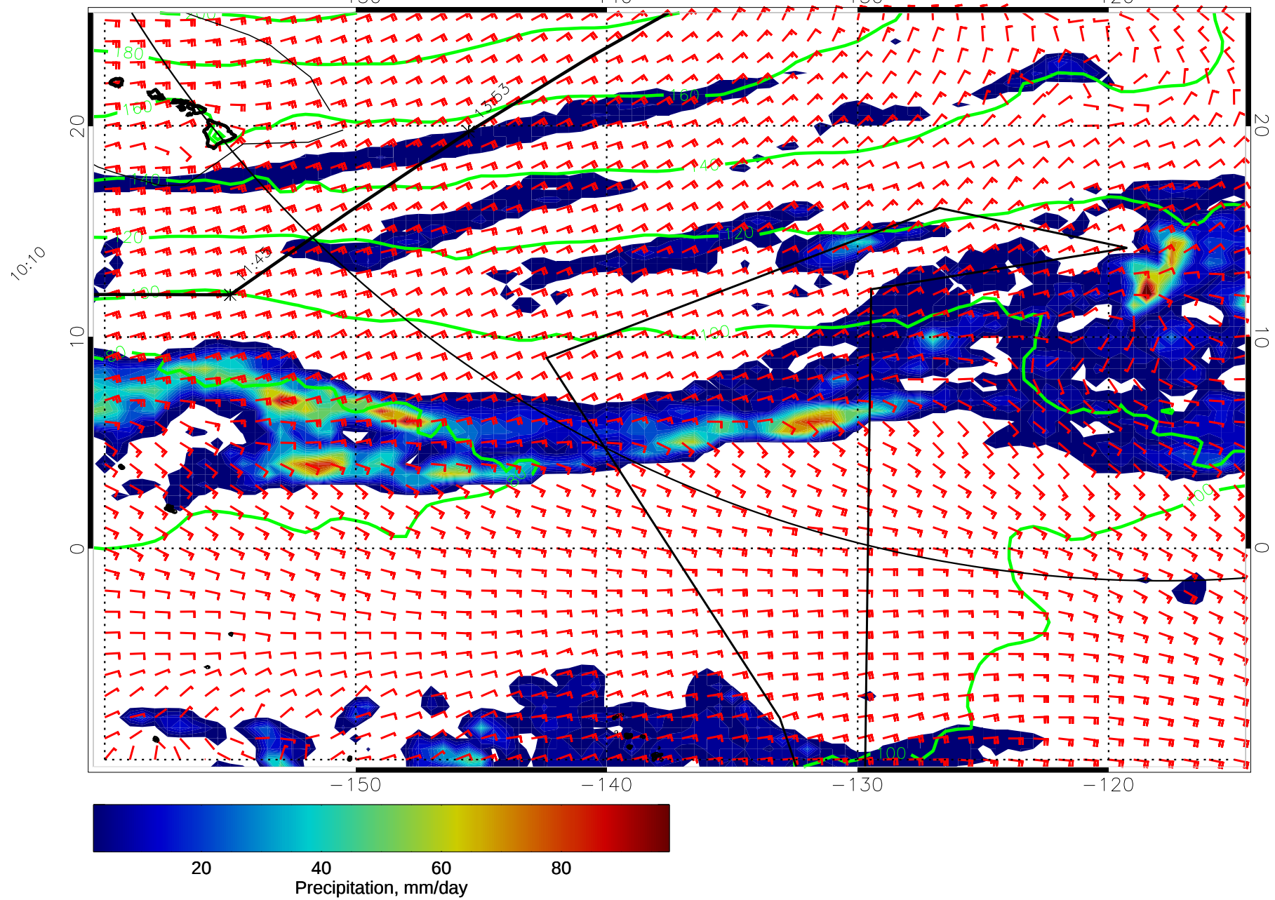
14121612, 60 hour forecast for precip, 1000mb Z, and winds (knots) -- NCEP GFS
