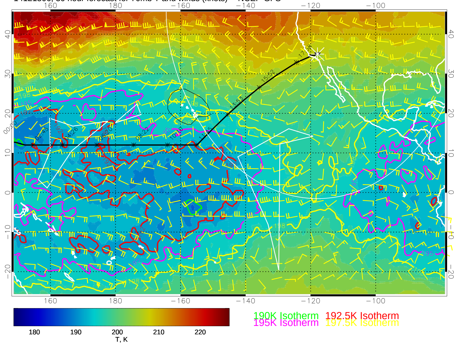
14121506, 30 hour forecast for 70mb T and winds (knots) -- NCEP GFS
