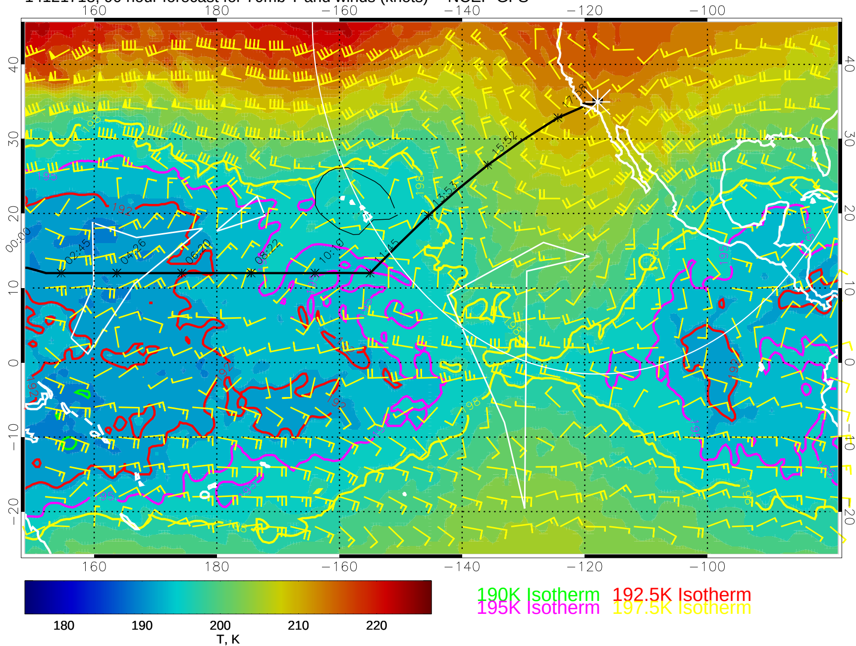
14121718, 90 hour forecast for 70mb T and winds (knots) -- NCEP GFS
