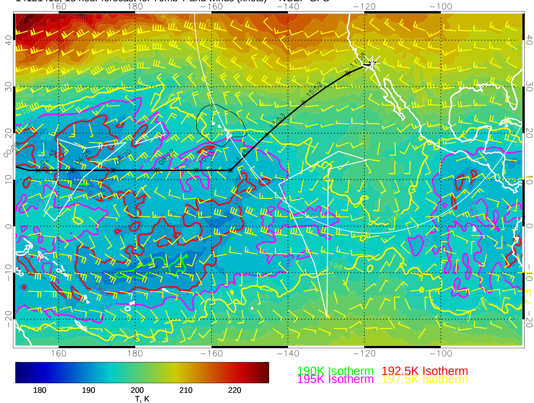
14121418, 18 hour forecast for 70mb T and winds (knots) -- NCEP GFS
