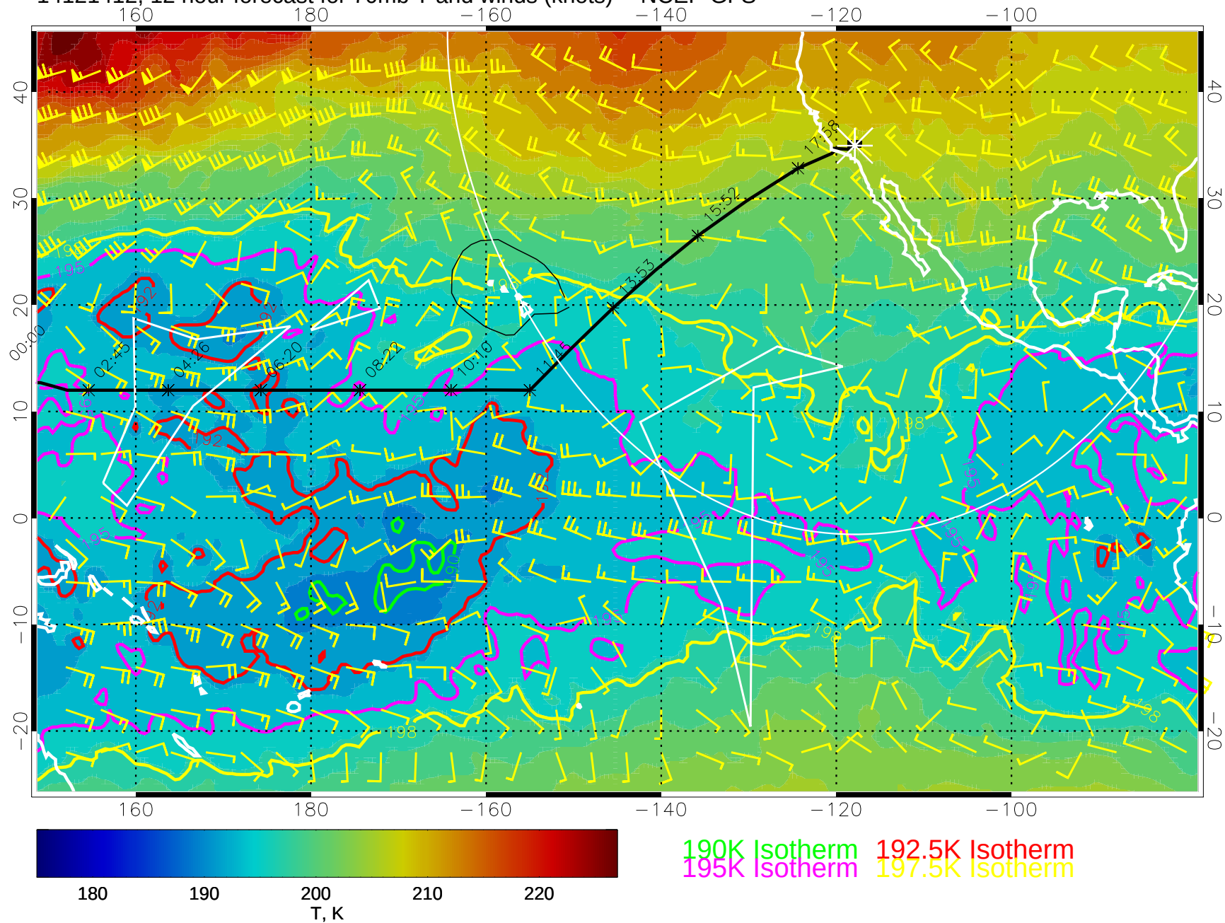
14121412, 12 hour forecast for 70mb T and winds (knots) -- NCEP GFS
