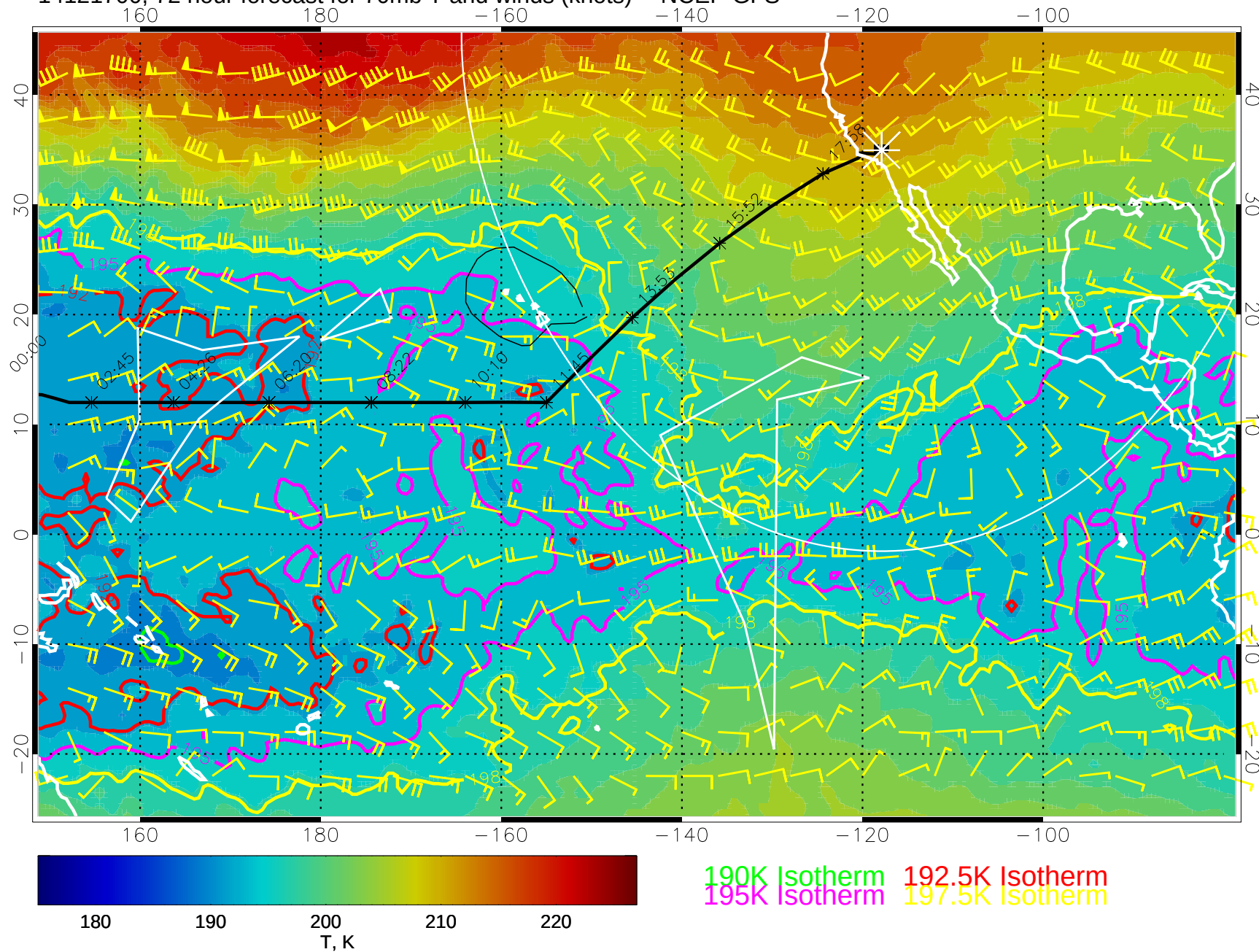
14121700, 72 hour forecast for 70mb T and winds (knots) -- NCEP GFS
