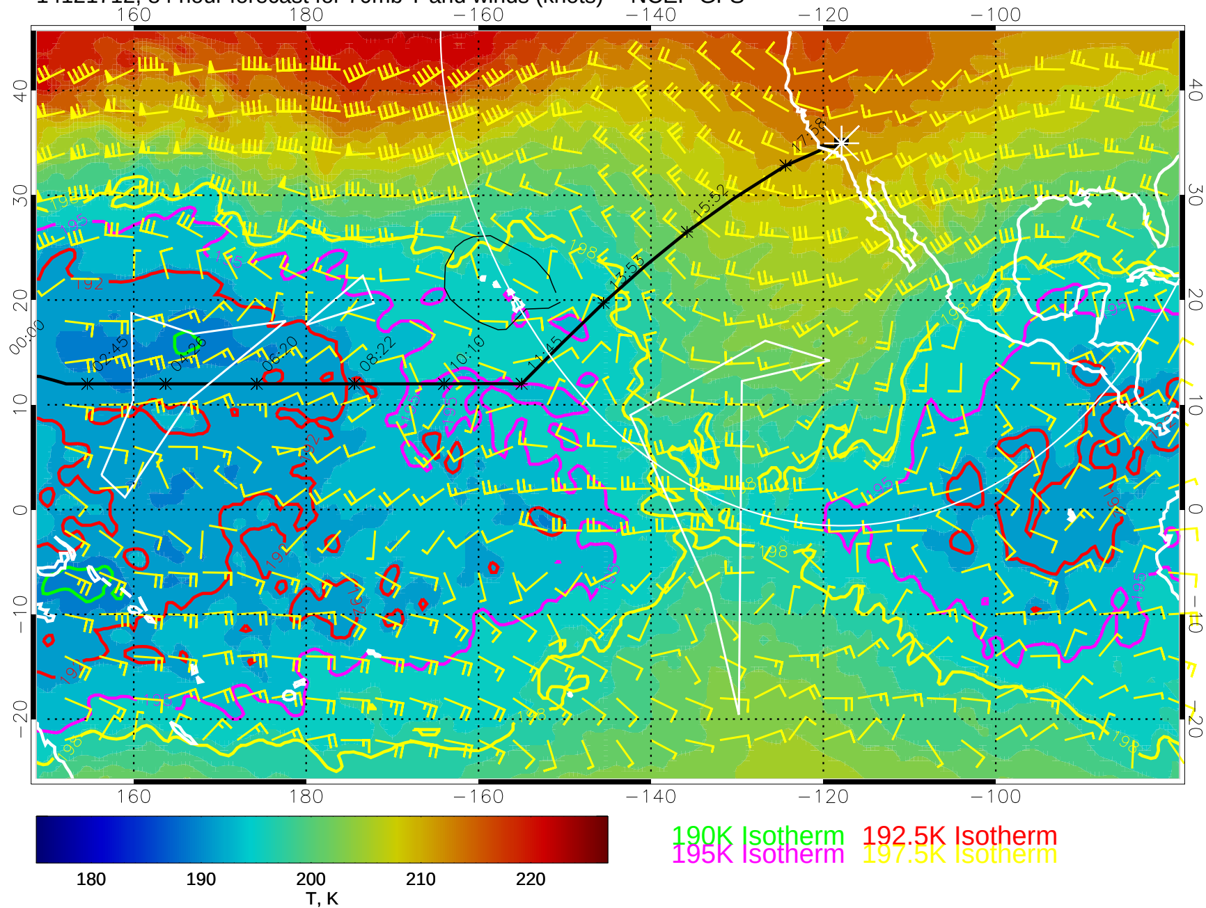
14121712, 84 hour forecast for 70mb T and winds (knots) -- NCEP GFS
