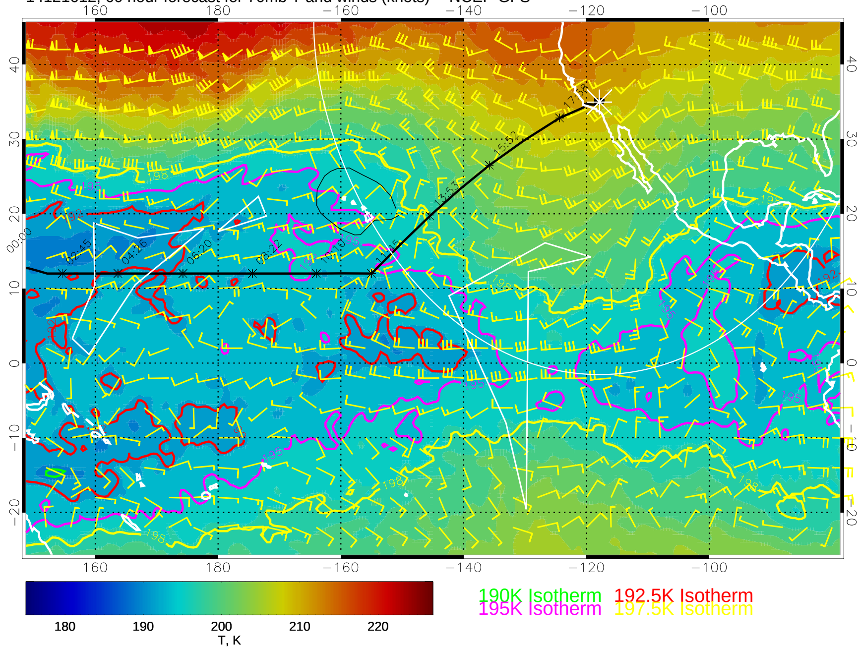
14121612, 60 hour forecast for 70mb T and winds (knots) -- NCEP GFS
