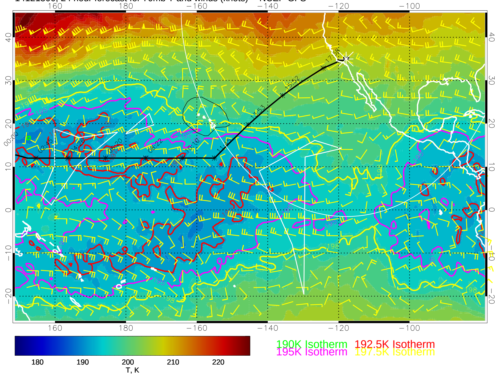
14121500, 24 hour forecast for 70mb T and winds (knots) -- NCEP GFS
