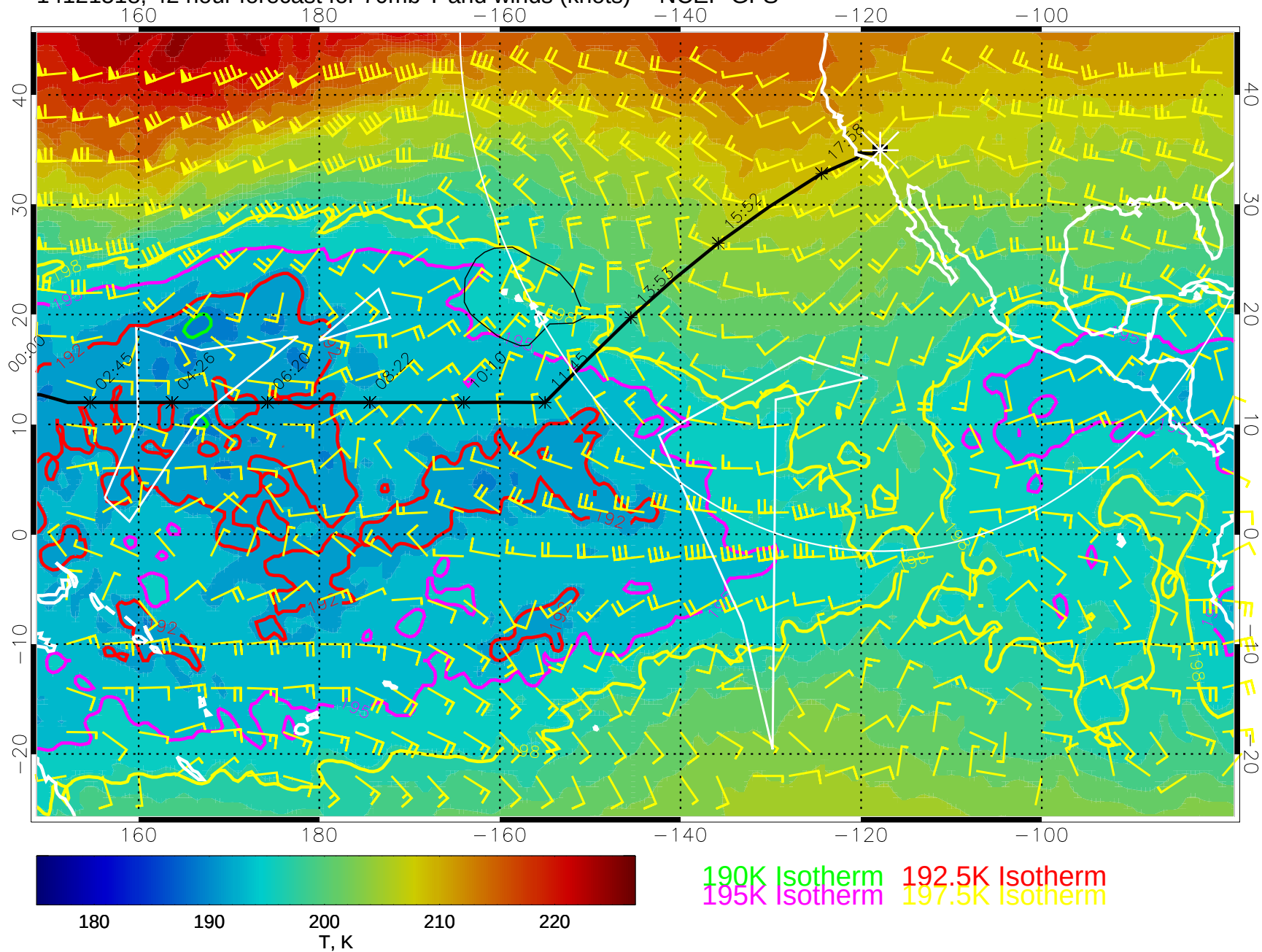
14121518, 42 hour forecast for 70mb T and winds (knots) -- NCEP GFS
