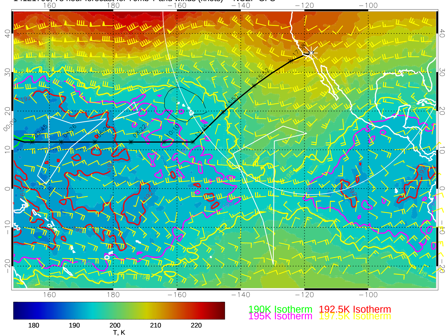
14121706, 78 hour forecast for 70mb T and winds (knots) -- NCEP GFS
