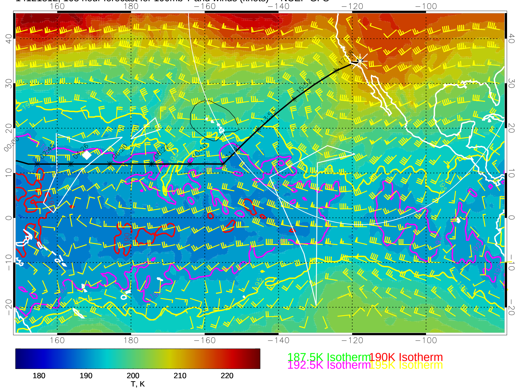
14121812, 108 hour forecast for 100mb T and winds (knots) -- NCEP GFS
