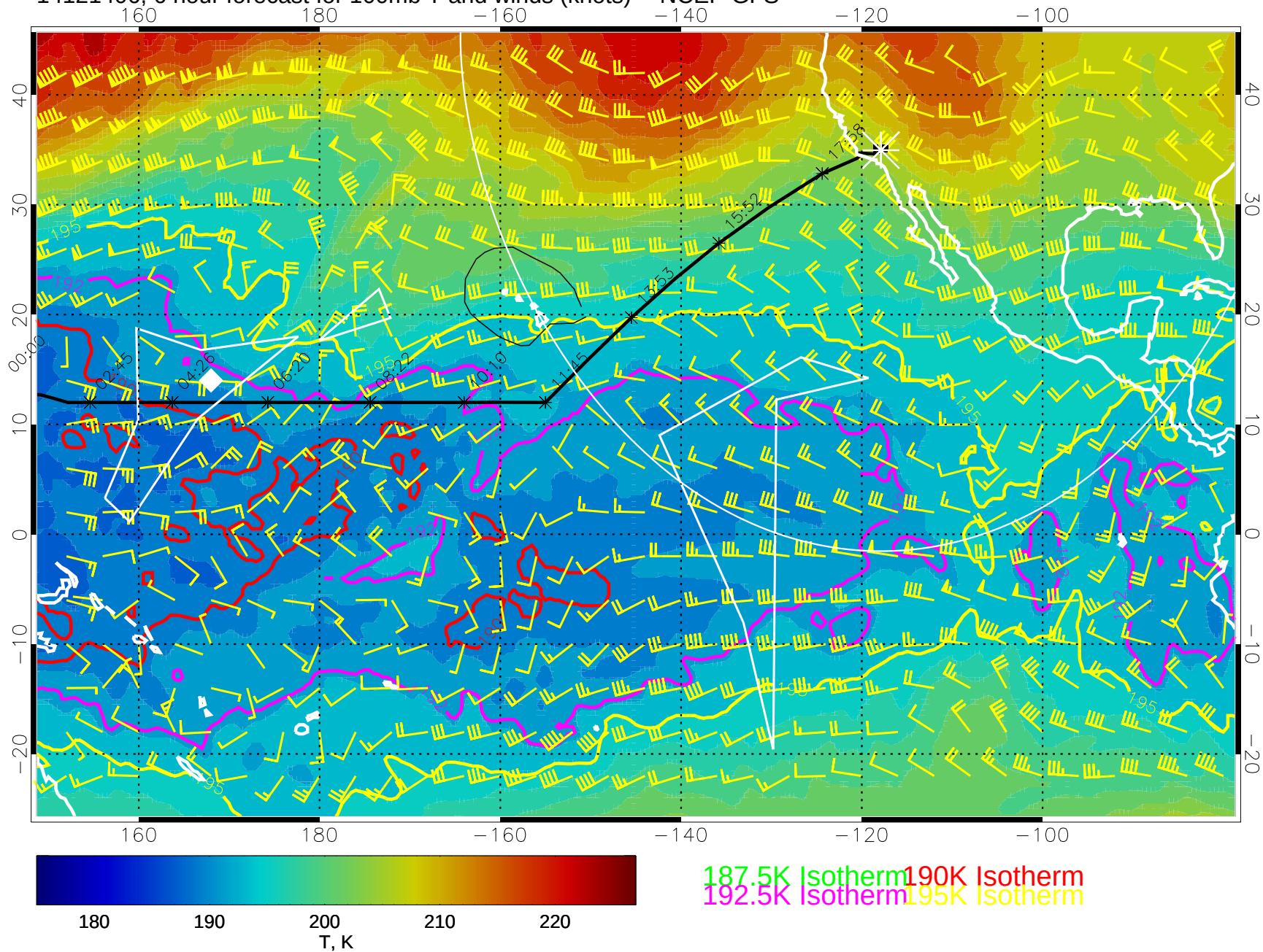
14121406, 6 hour forecast for 100mb T and winds (knots) -- NCEP GFS
