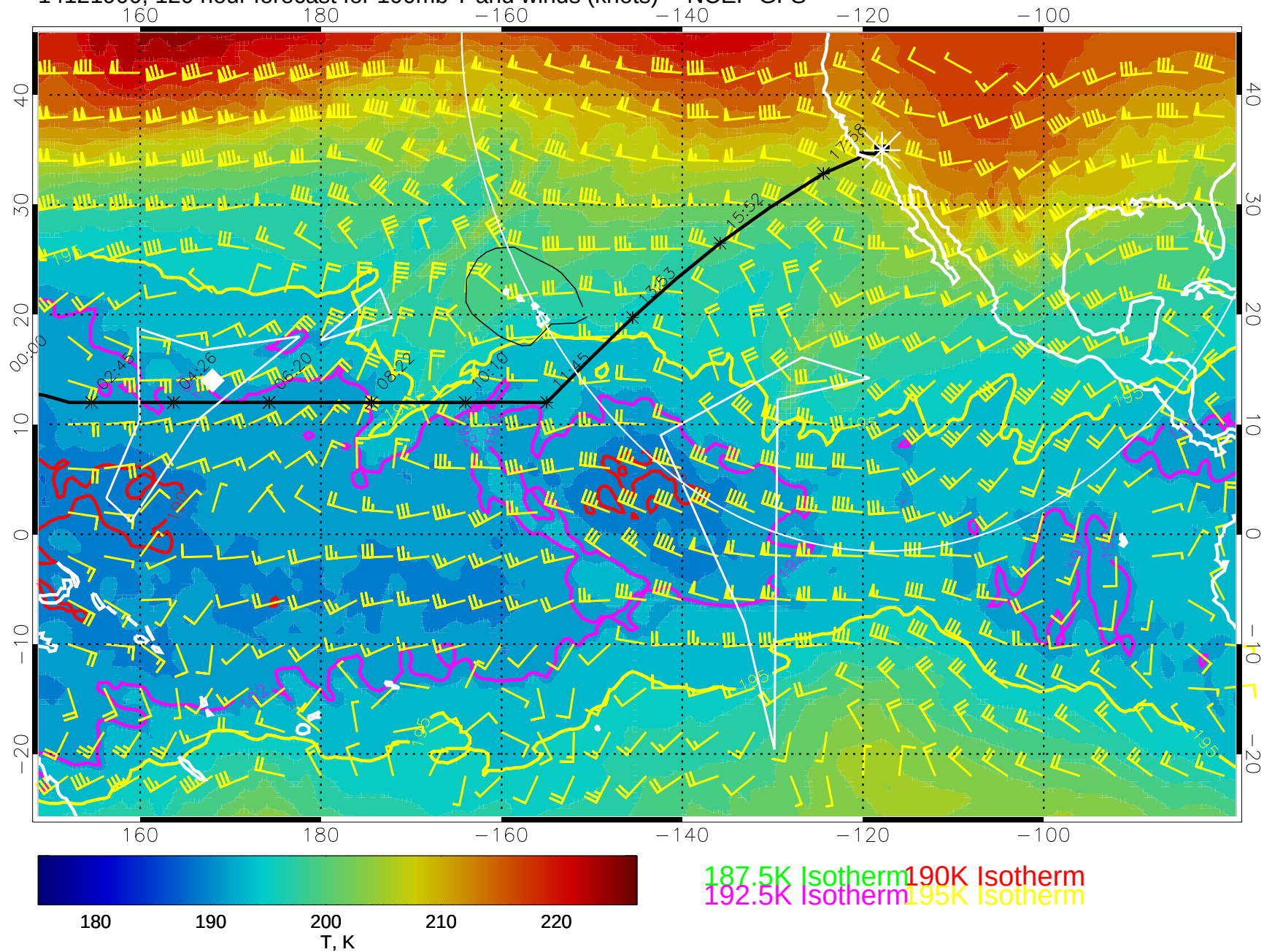
14121900, 120 hour forecast for 100mb T and winds (knots) -- NCEP GFS
