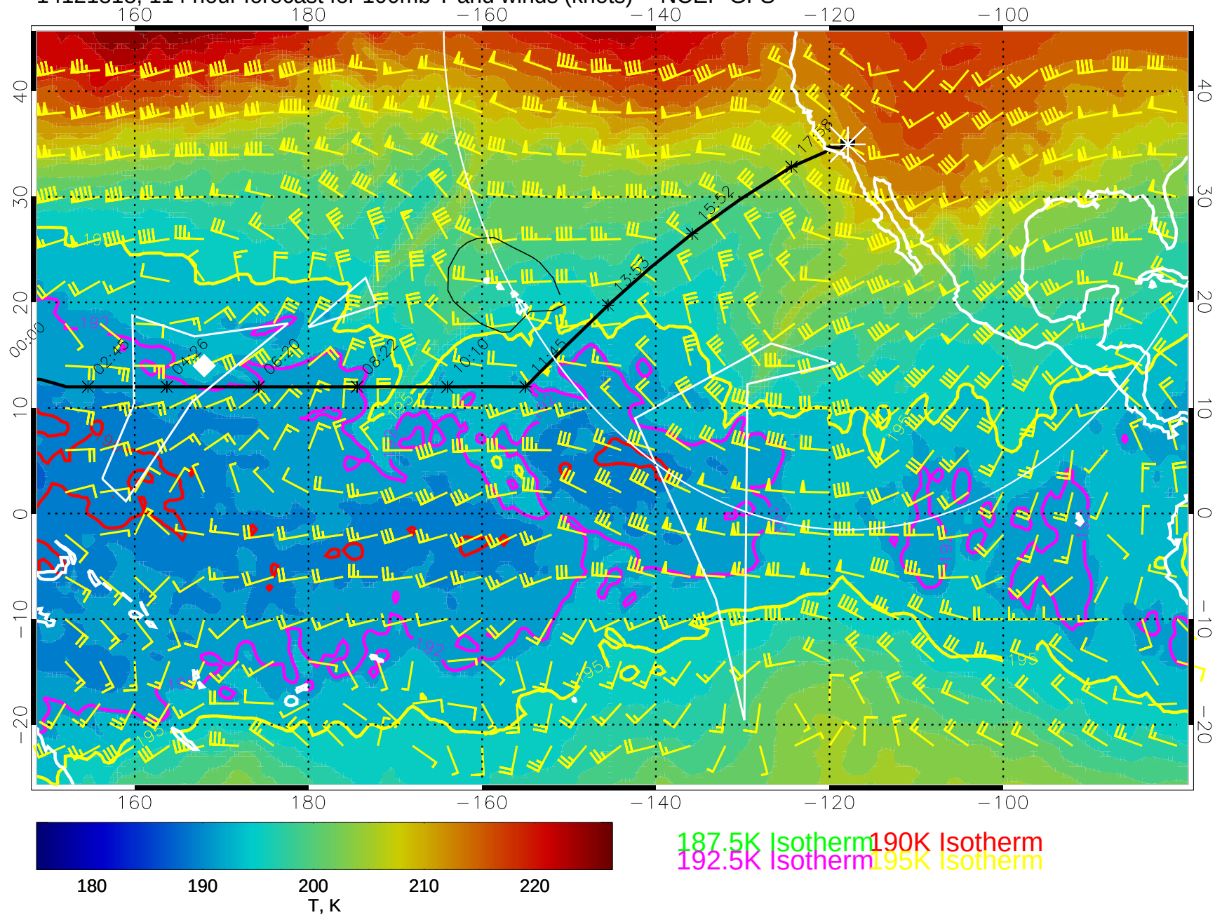
14121818, 114 hour forecast for 100mb T and winds (knots) -- NCEP GFS
