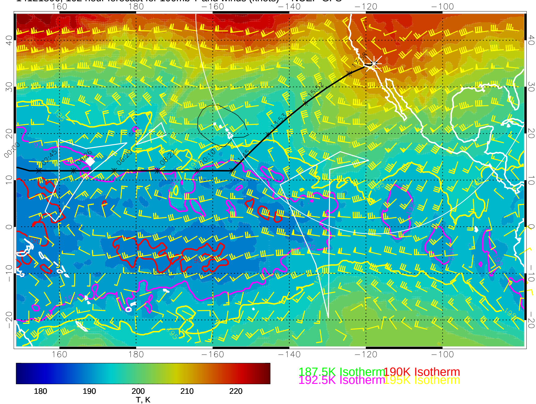
14121806, 102 hour forecast for 100mb T and winds (knots) -- NCEP GFS
