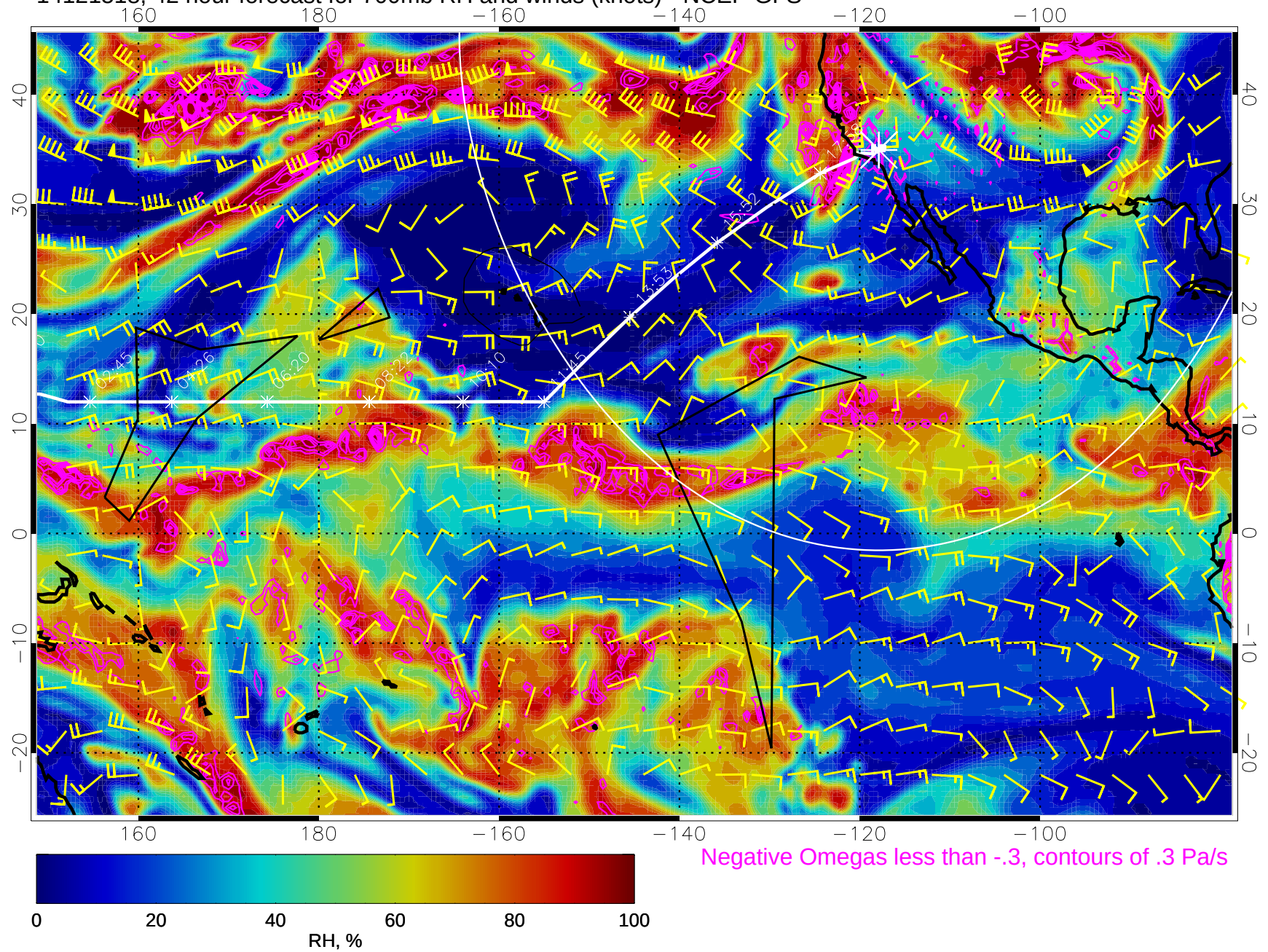
14121518, 42 hour forecast for 700mb RH and winds (knots) - NCEP GFS
