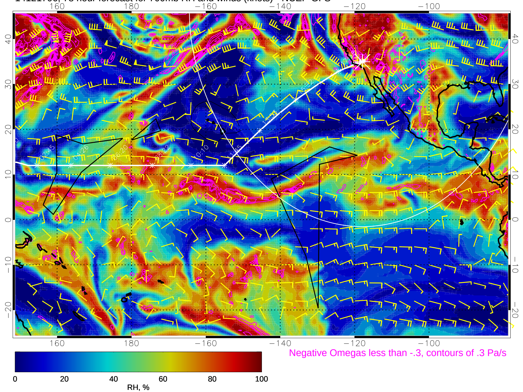
14121706, 78 hour forecast for 700mb RH and winds (knots) - NCEP GFS
