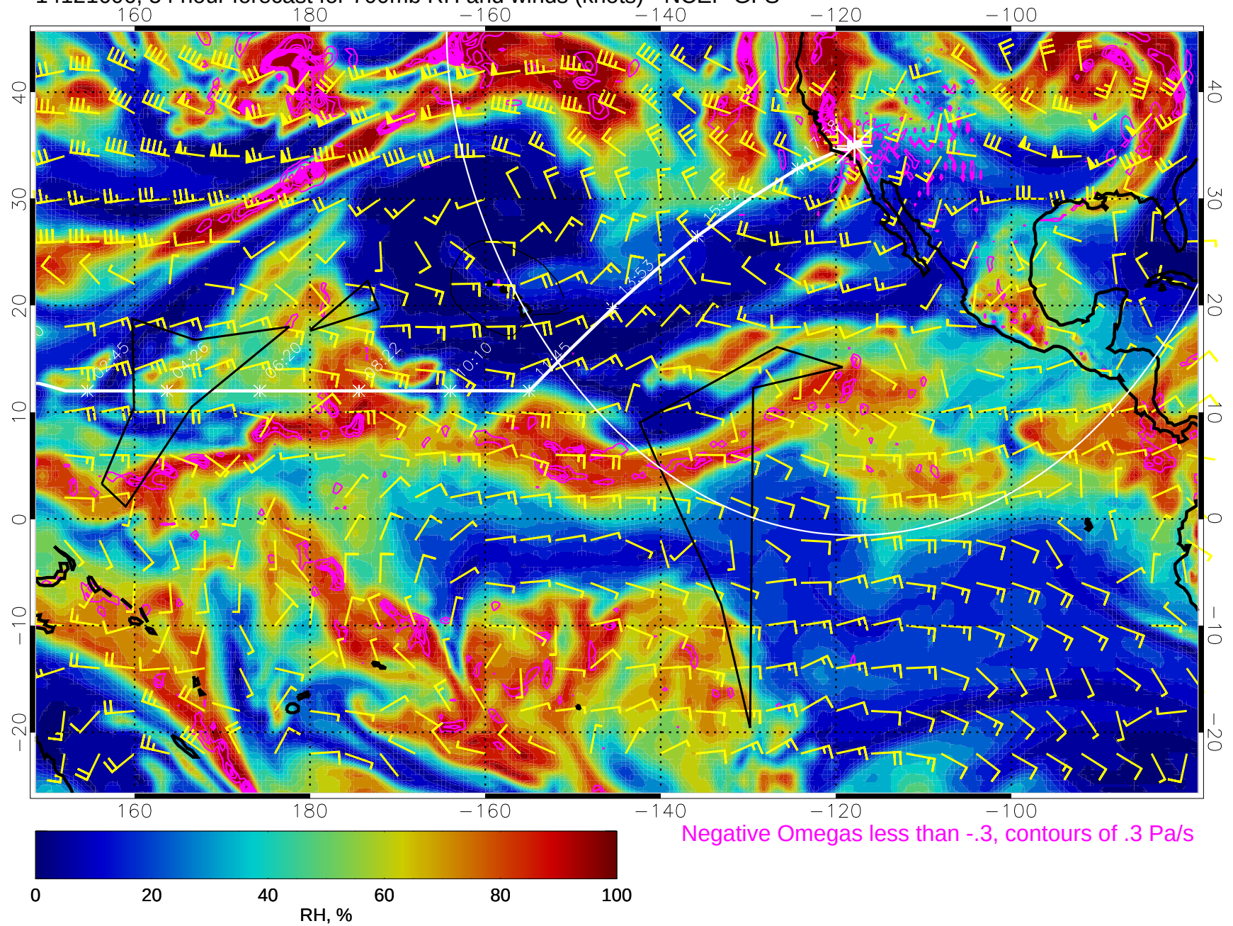
14121606, 54 hour forecast for 700mb RH and winds (knots) - NCEP GFS
