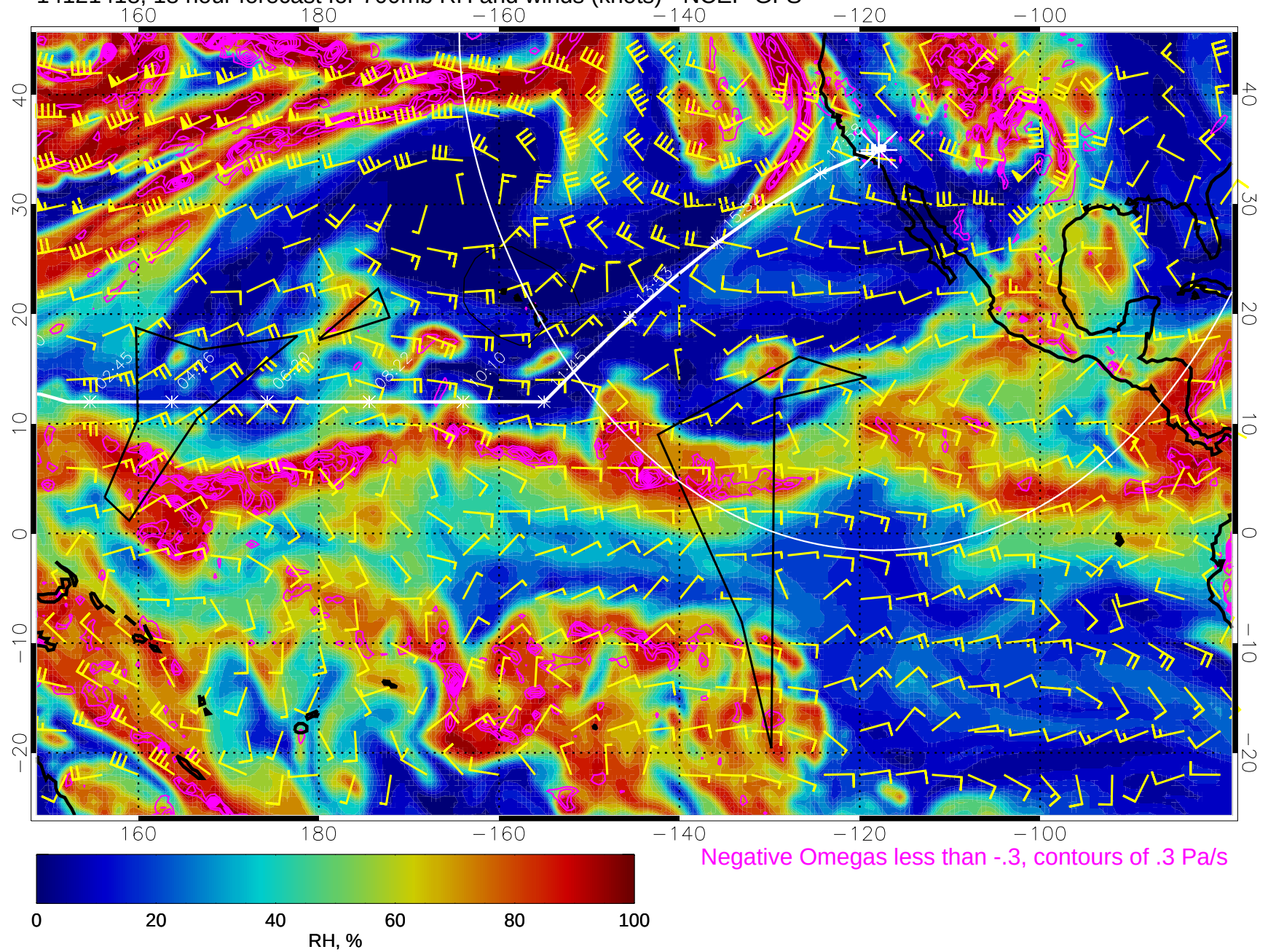
14121418, 18 hour forecast for 700mb RH and winds (knots) - NCEP GFS
