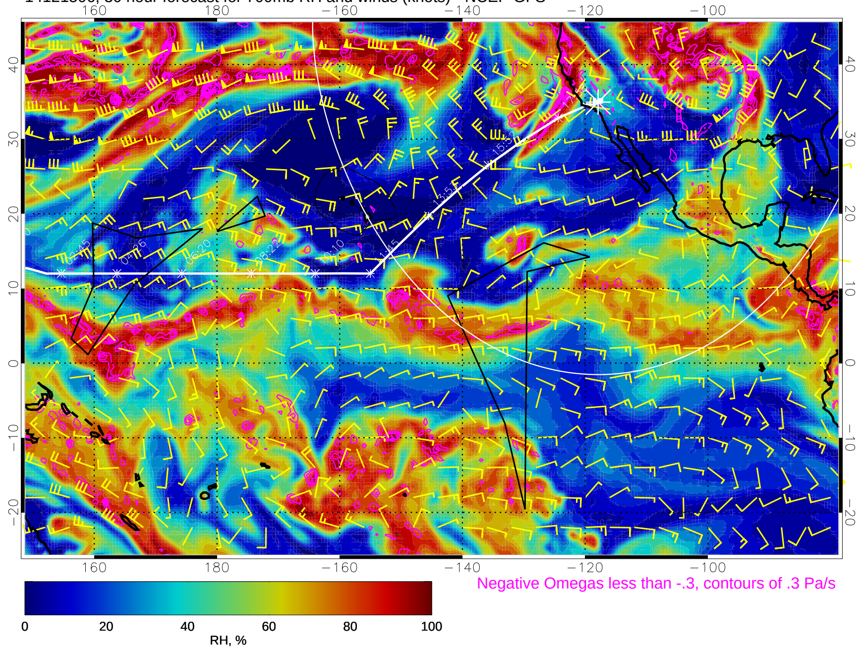
14121506, 30 hour forecast for 700mb RH and winds (knots) - NCEP GFS
