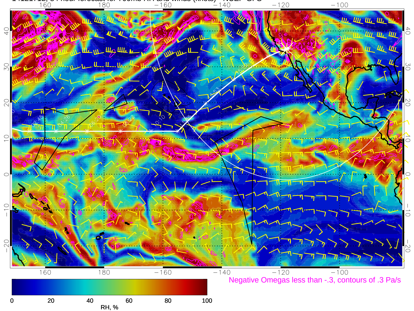
14121712, 84 hour forecast for 700mb RH and winds (knots) - NCEP GFS
