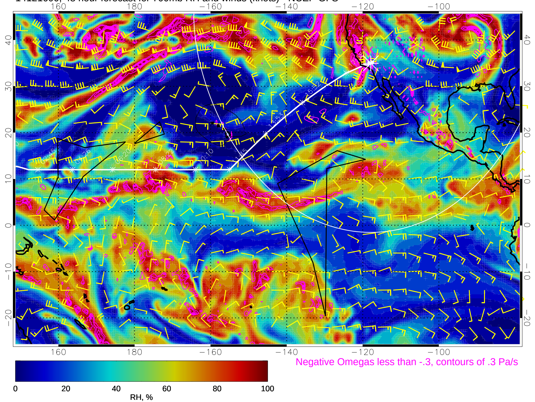
14121600, 48 hour forecast for 700mb RH and winds (knots) - NCEP GFS
