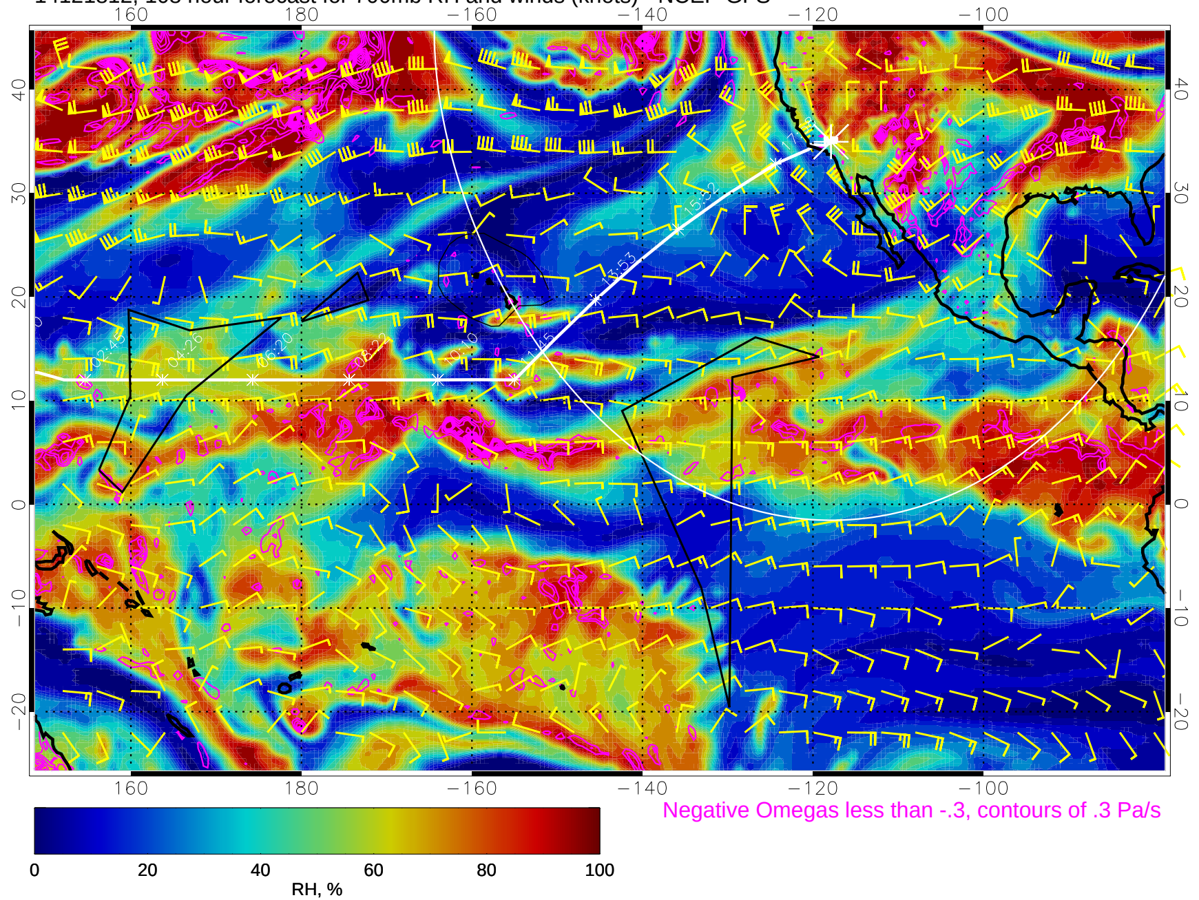
14121812, 108 hour forecast for 700mb RH and winds (knots) - NCEP GFS
