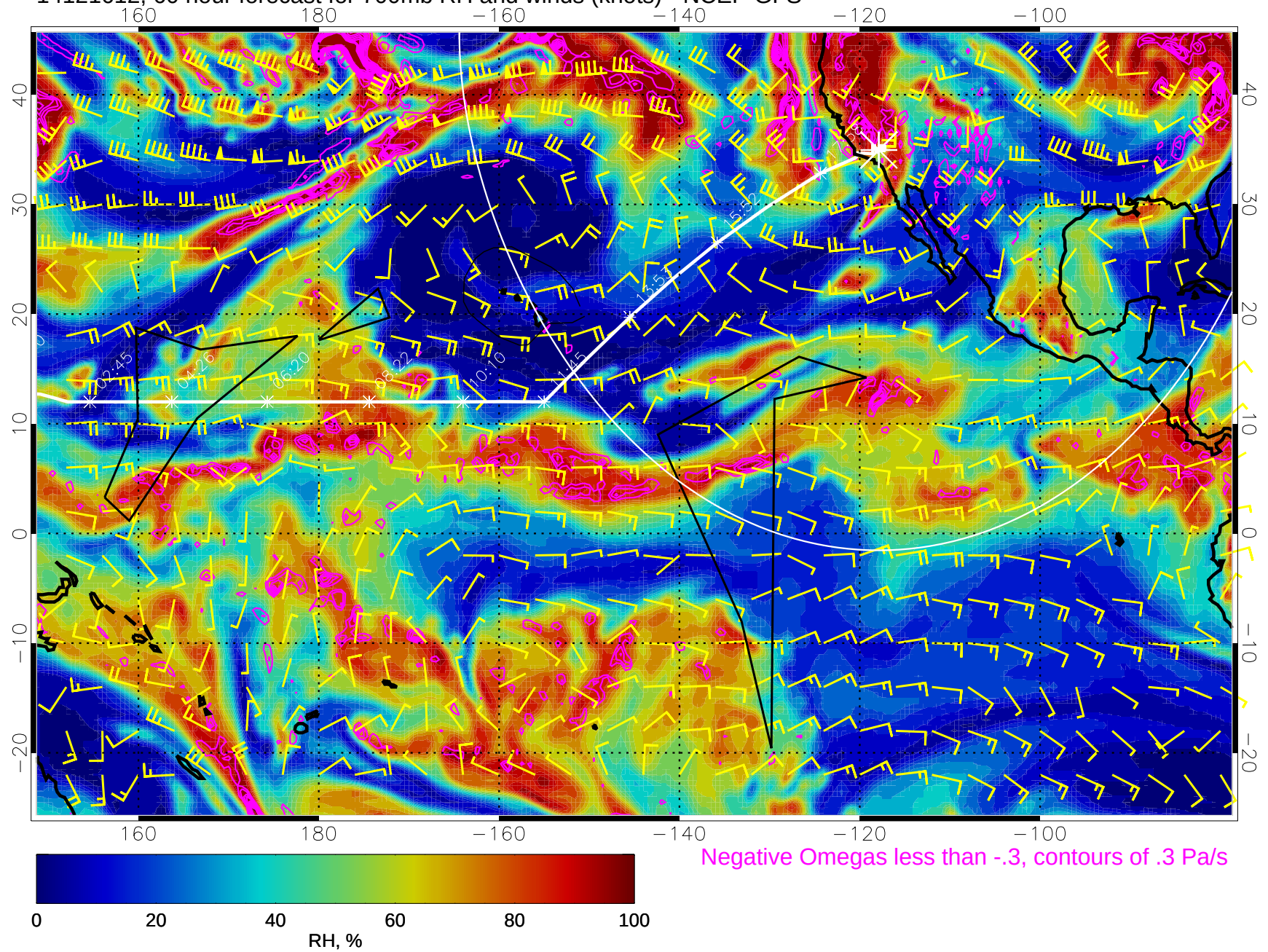
14121612, 60 hour forecast for 700mb RH and winds (knots) - NCEP GFS
