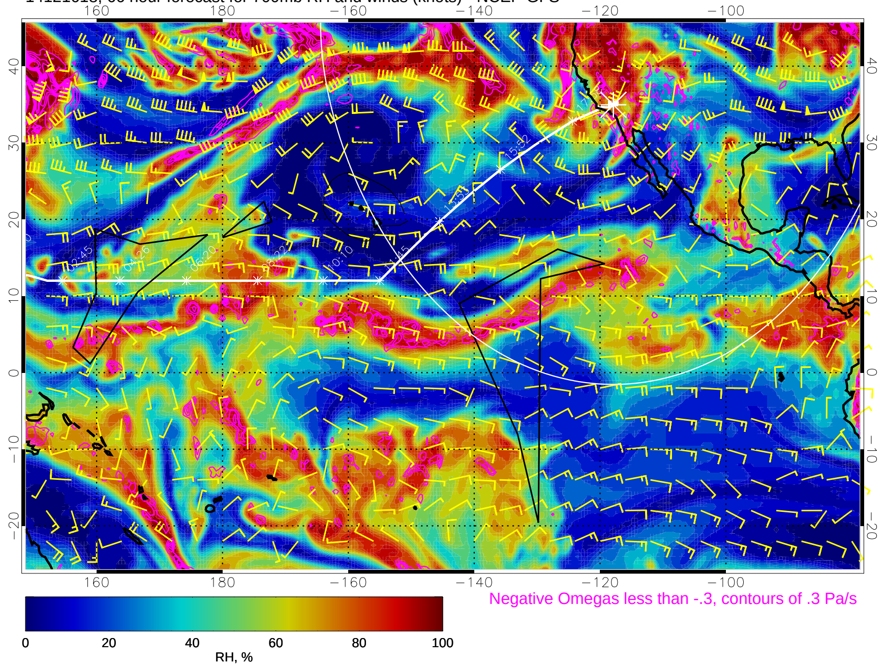
14121618, 66 hour forecast for 700mb RH and winds (knots) - NCEP GFS
