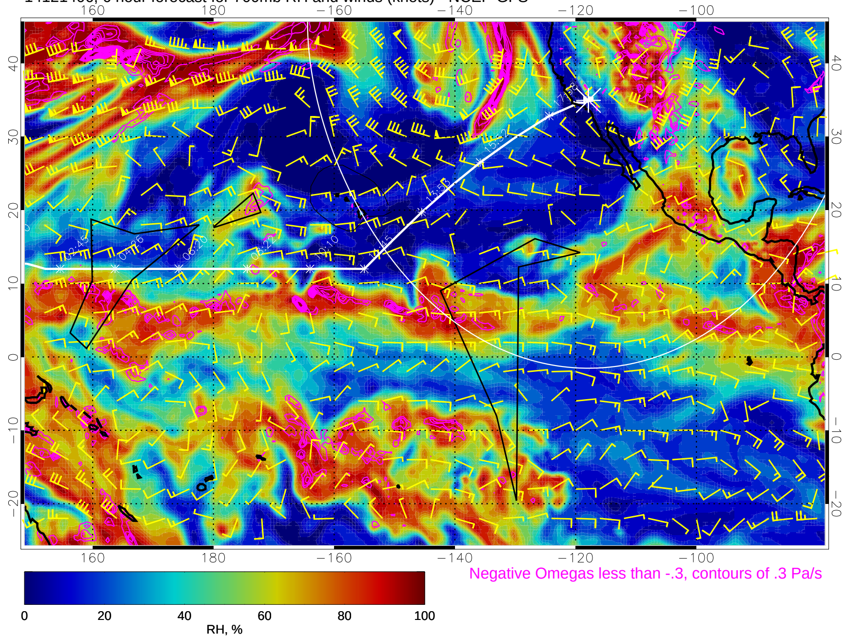
14121406, 6 hour forecast for 700mb RH and winds (knots) - NCEP GFS
