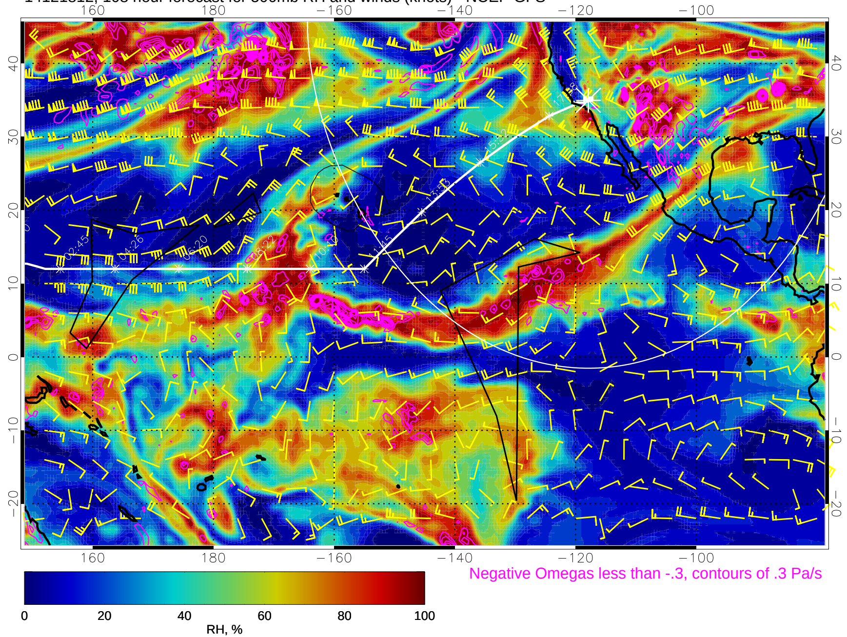
14121812, 108 hour forecast for 500mb RH and winds (knots) - NCEP GFS
