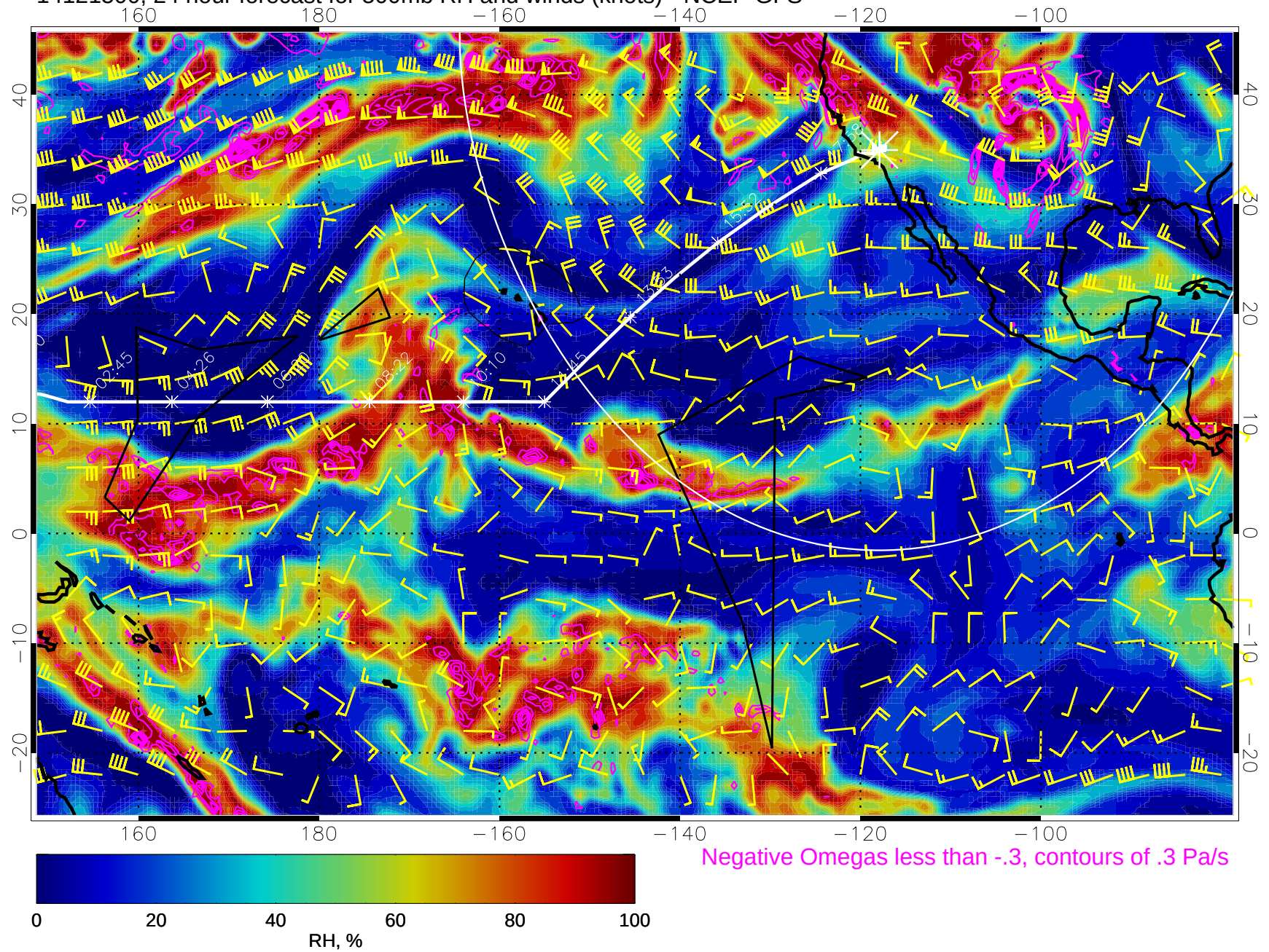
14121500, 24 hour forecast for 500mb RH and winds (knots) - NCEP GFS
