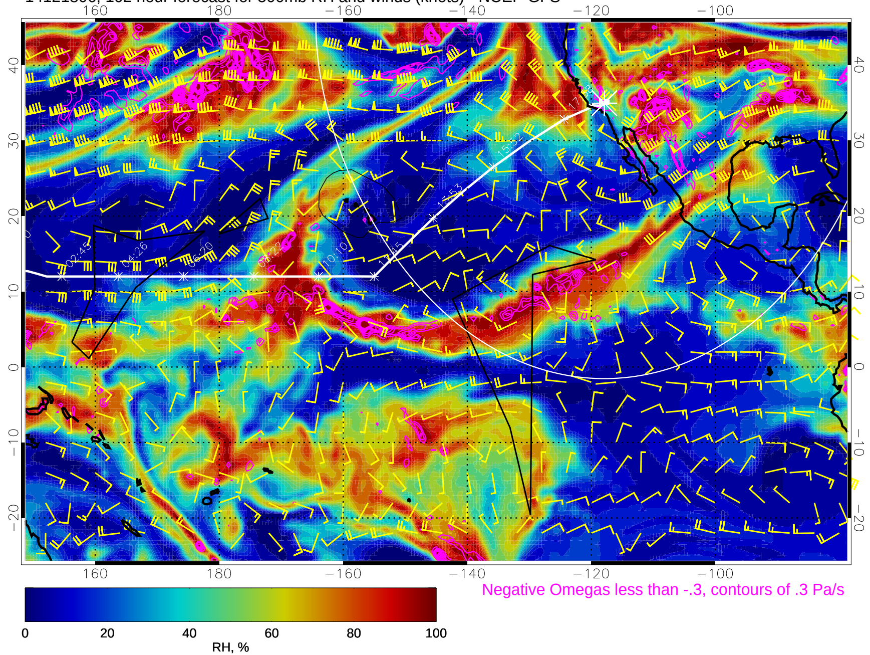
14121806, 102 hour forecast for 500mb RH and winds (knots) - NCEP GFS
