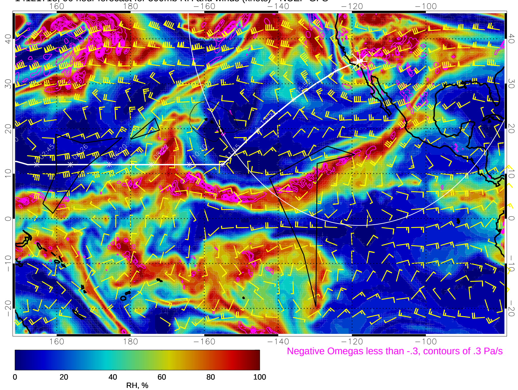
14121718, 90 hour forecast for 500mb RH and winds (knots) - NCEP GFS
