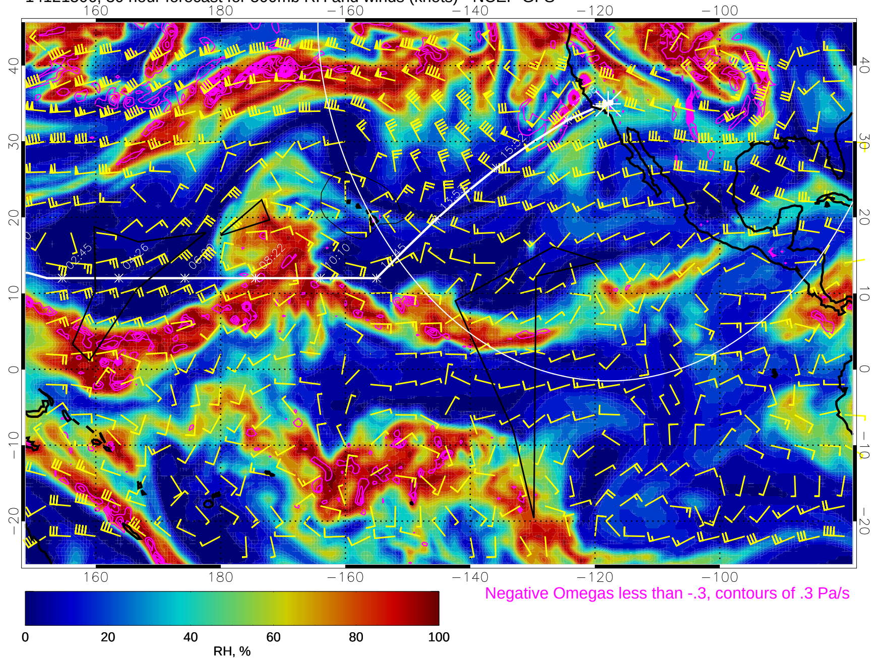
14121506, 30 hour forecast for 500mb RH and winds (knots) - NCEP GFS
