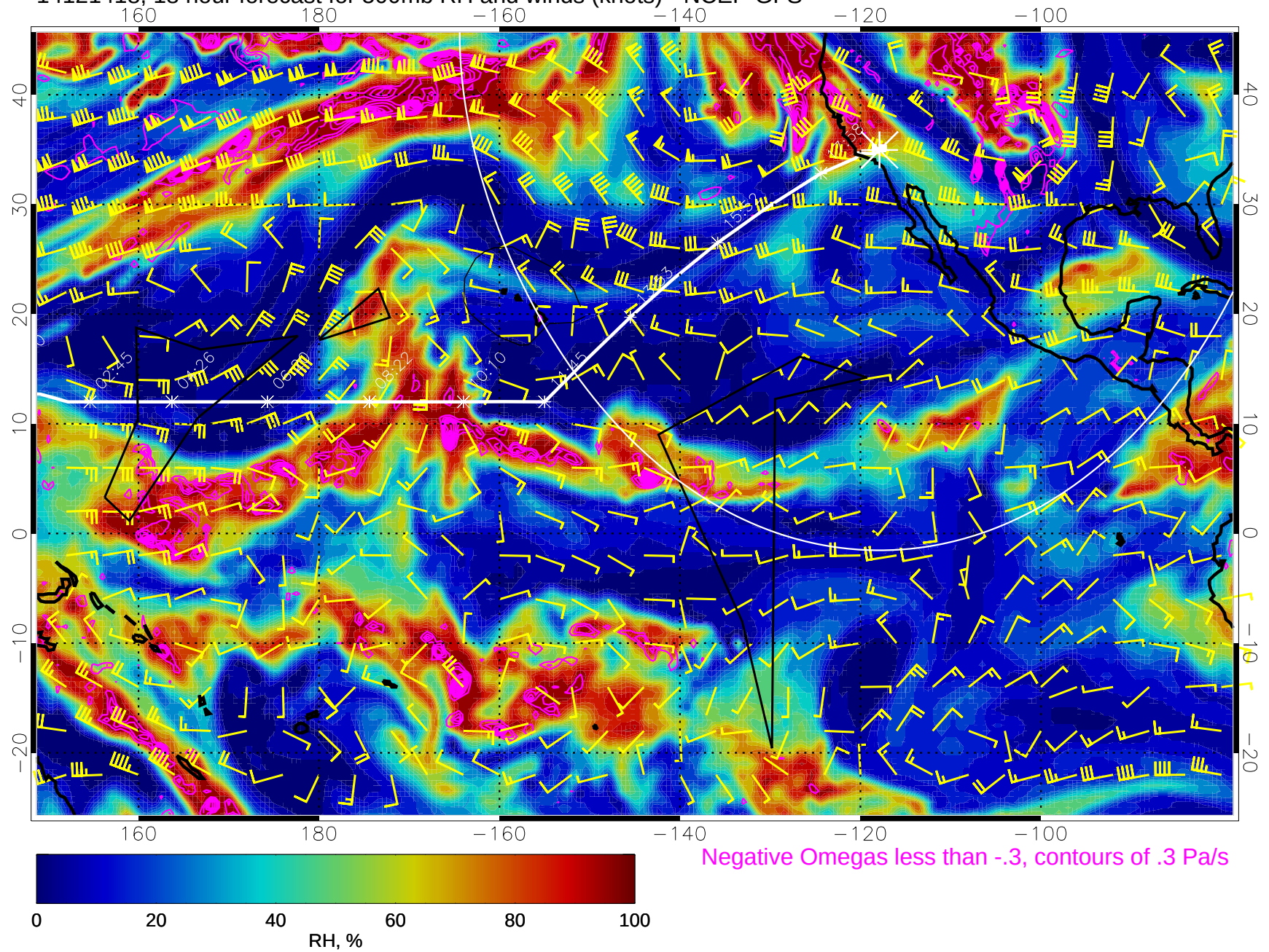
14121418, 18 hour forecast for 500mb RH and winds (knots) - NCEP GFS
