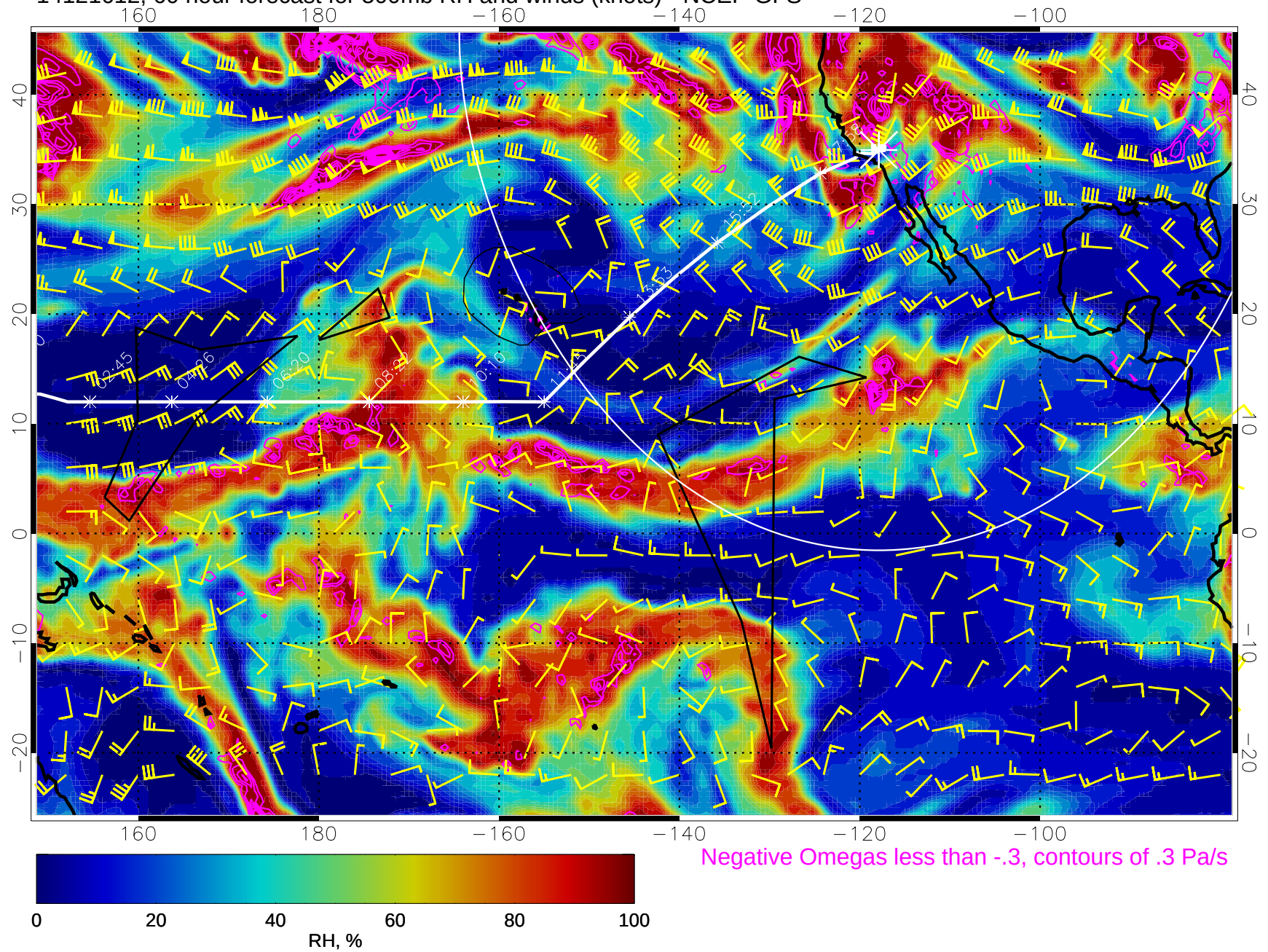
14121612, 60 hour forecast for 500mb RH and winds (knots) - NCEP GFS
