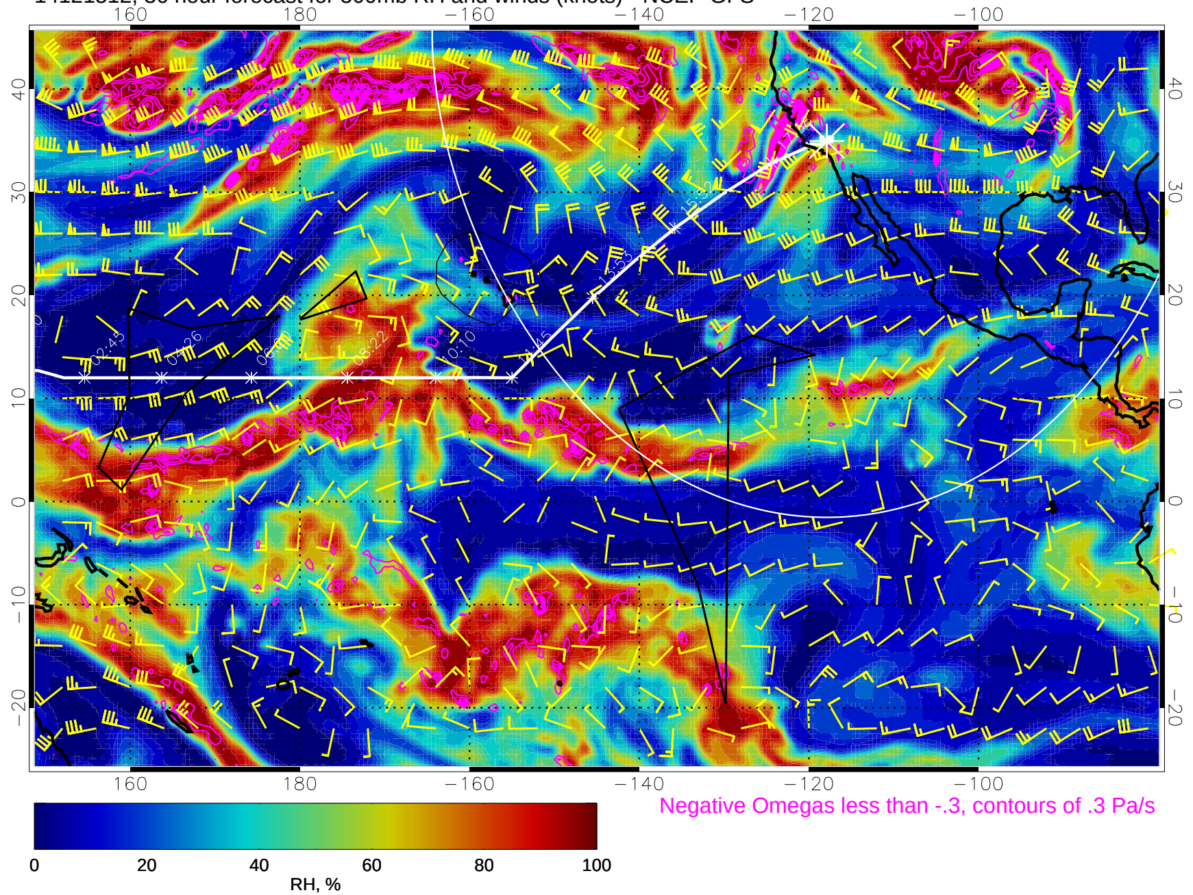
14121512, 36 hour forecast for 500mb RH and winds (knots) - NCEP GFS
