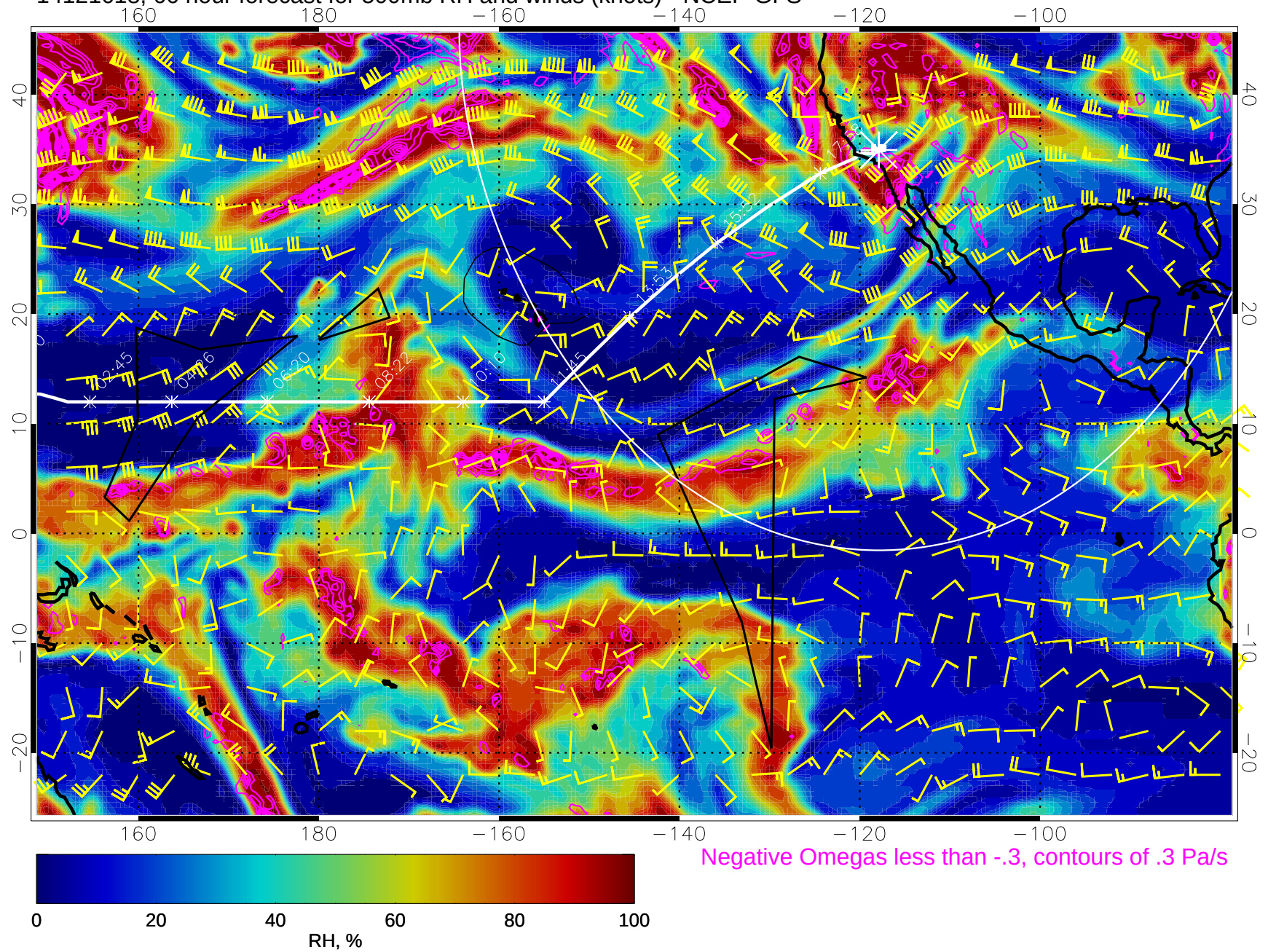
14121618, 66 hour forecast for 500mb RH and winds (knots) - NCEP GFS
