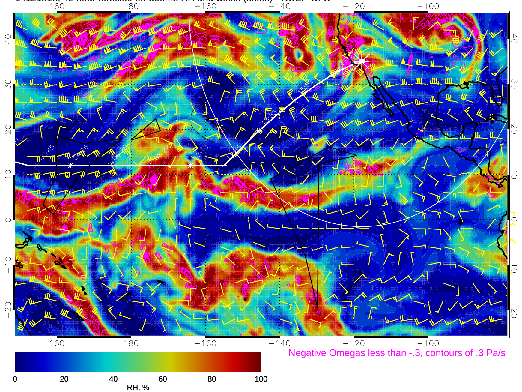
14121518, 42 hour forecast for 500mb RH and winds (knots) - NCEP GFS
