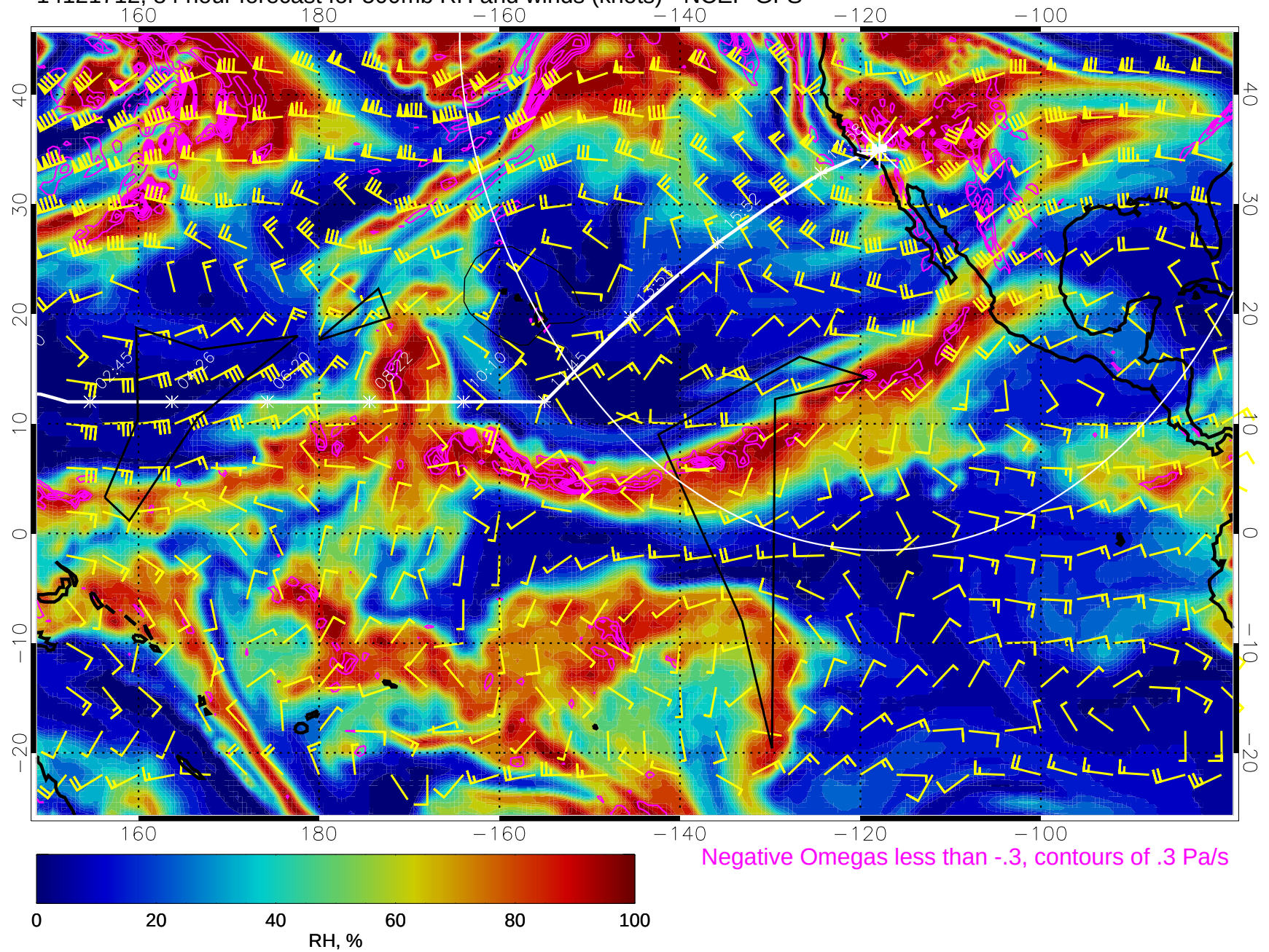
14121712, 84 hour forecast for 500mb RH and winds (knots) - NCEP GFS
