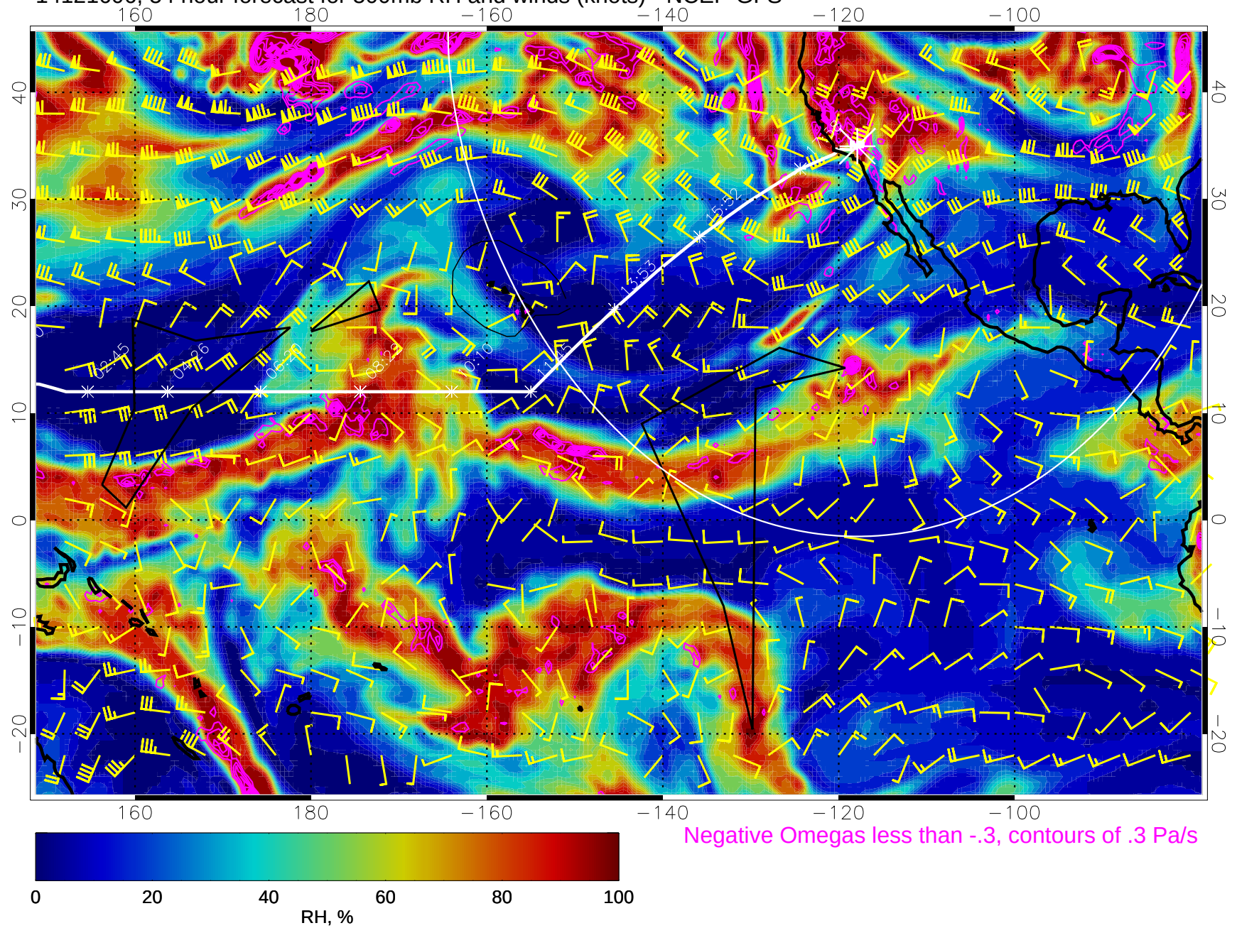
14121606, 54 hour forecast for 500mb RH and winds (knots) - NCEP GFS
