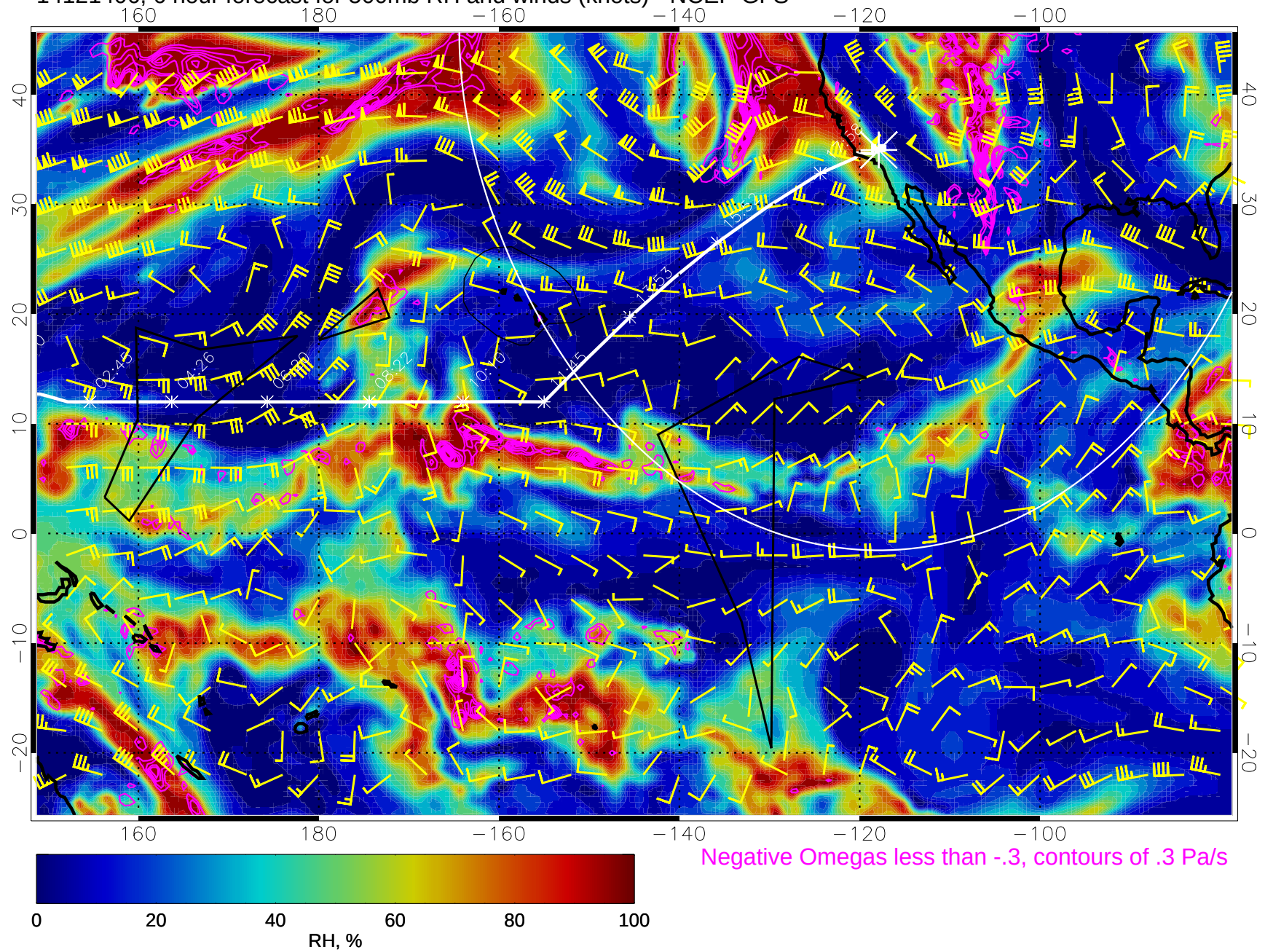
14121406, 6 hour forecast for 500mb RH and winds (knots) - NCEP GFS
