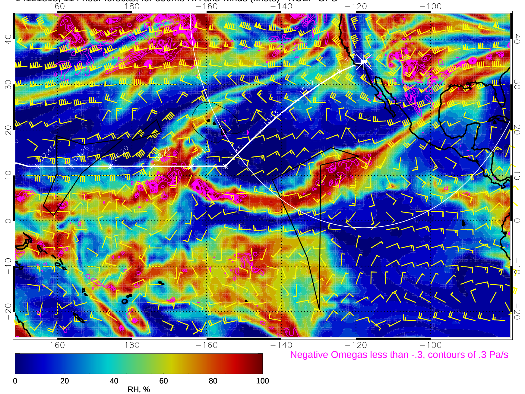
14121818, 114 hour forecast for 500mb RH and winds (knots) - NCEP GFS
