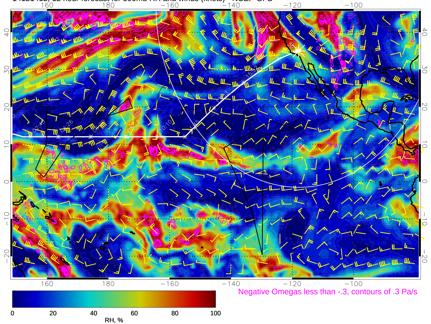
14121412, 12 hour forecast for 500mb RH and winds (knots) - NCEP GFS
