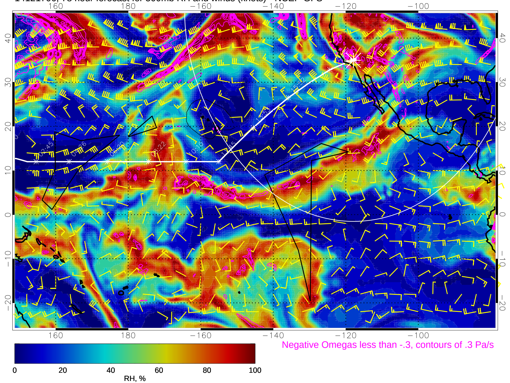
14121706, 78 hour forecast for 500mb RH and winds (knots) - NCEP GFS
