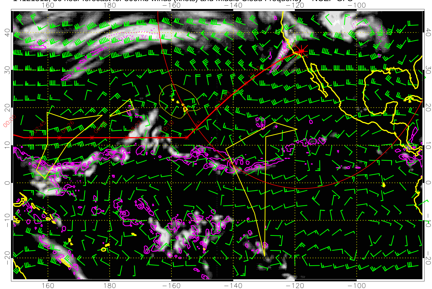
14121512, 36 hour forecast for 500mb winds (knots) and Middle Cloud Frequency -- NCEP GFS
