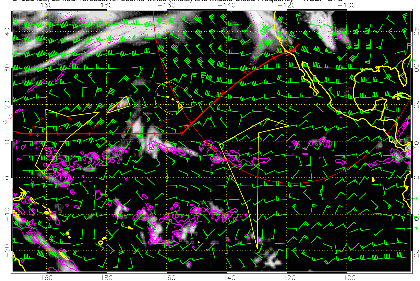
14121418, 18 hour forecast for 500mb winds (knots) and Middle Cloud Frequency -- NCEP GFS
