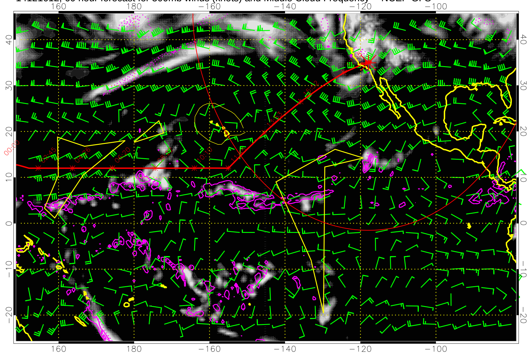
14121612, 60 hour forecast for 500mb winds (knots) and Middle Cloud Frequency -- NCEP GFS
