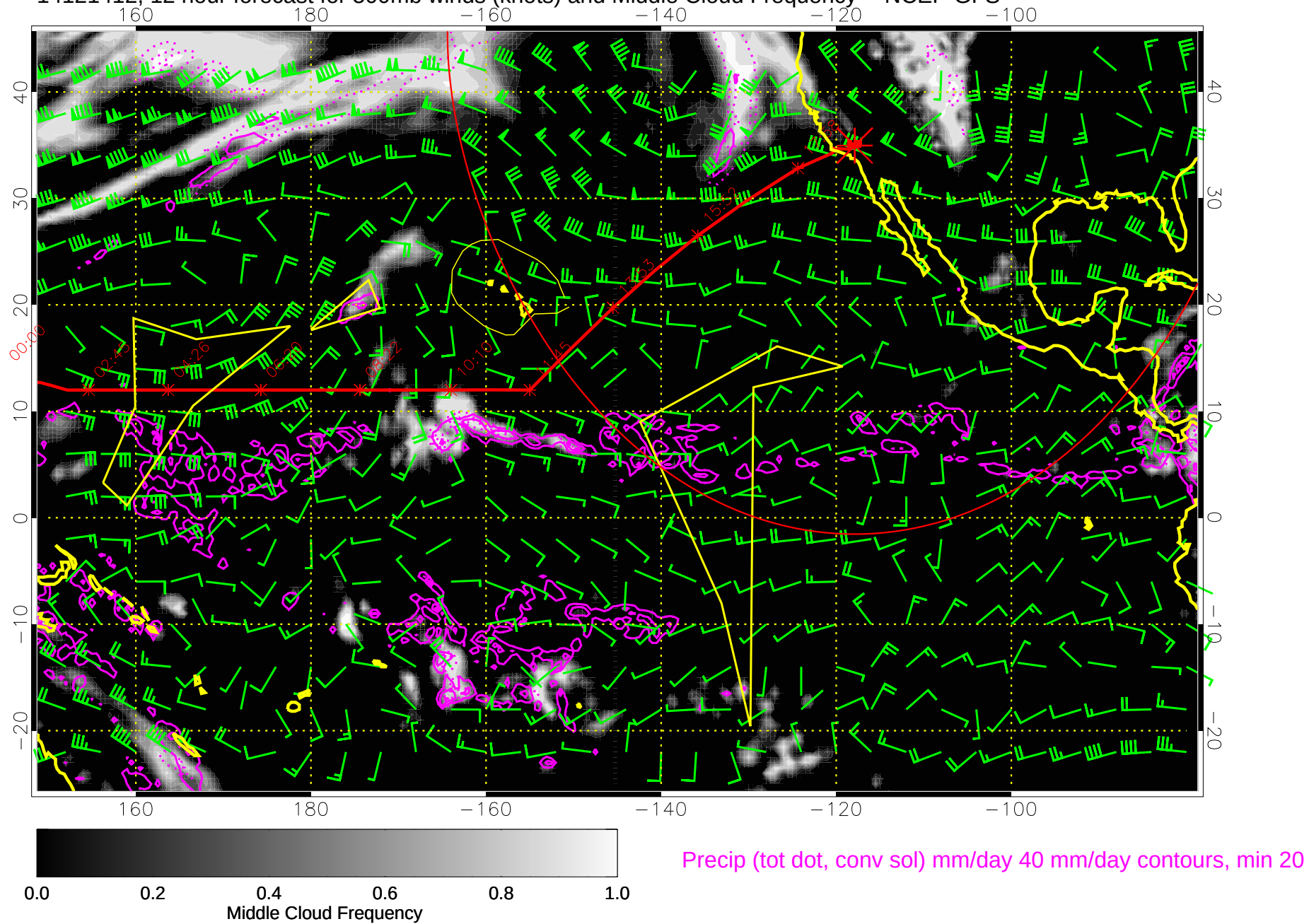
14121412, 12 hour forecast for 500mb winds (knots) and Middle Cloud Frequency -- NCEP GFS
