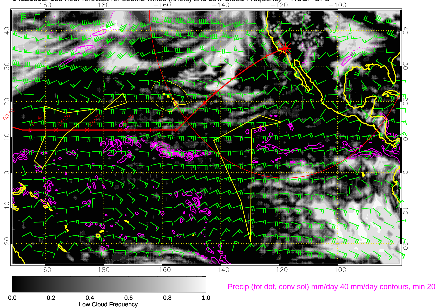
14121812, 108 hour forecast for 850mb winds (knots) and Low Cloud Frequency -- NCEP GFS
