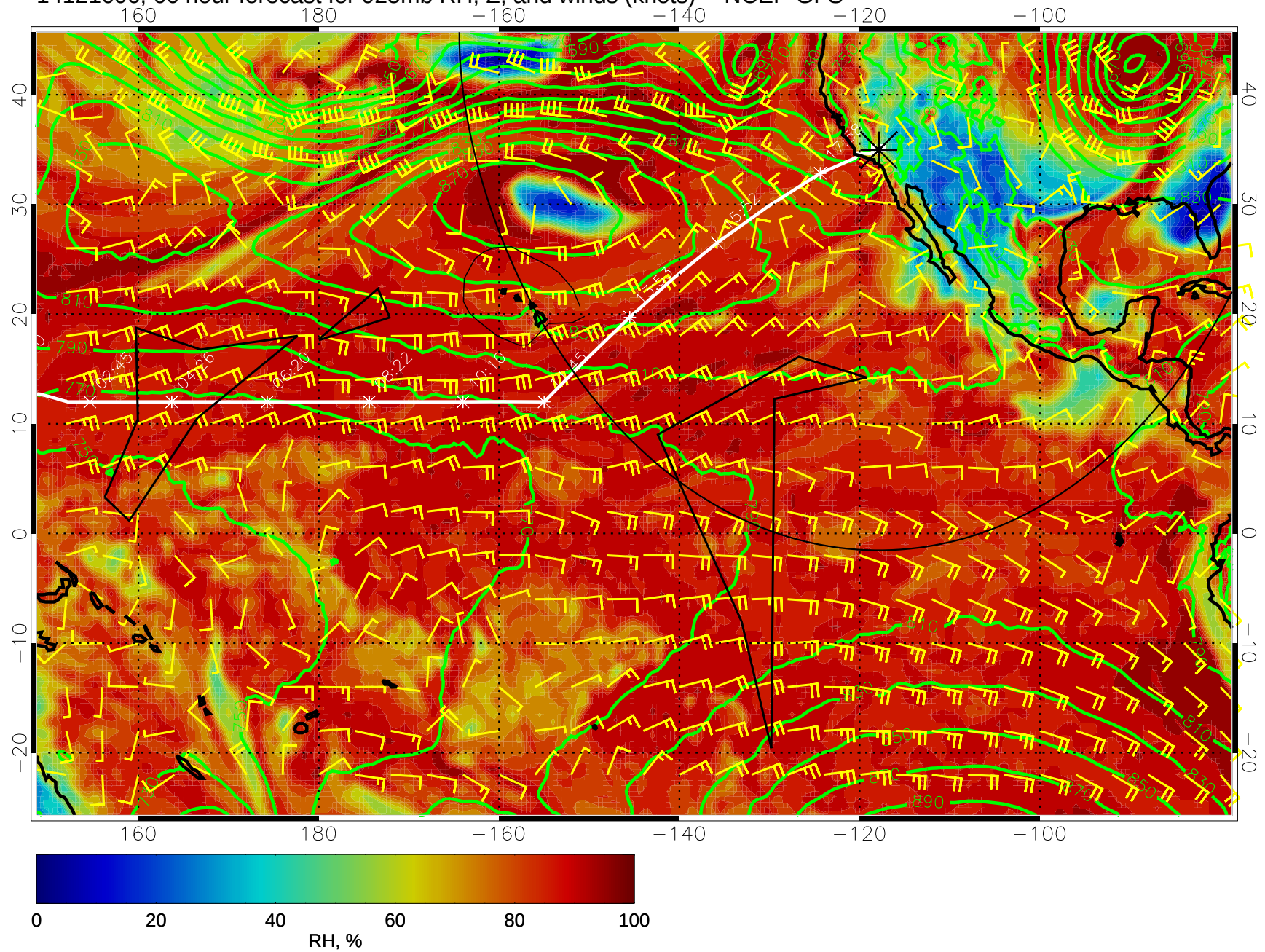
14121606, 66 hour forecast for 925mb RH, Z, and winds (knots) -- NCEP GFS
