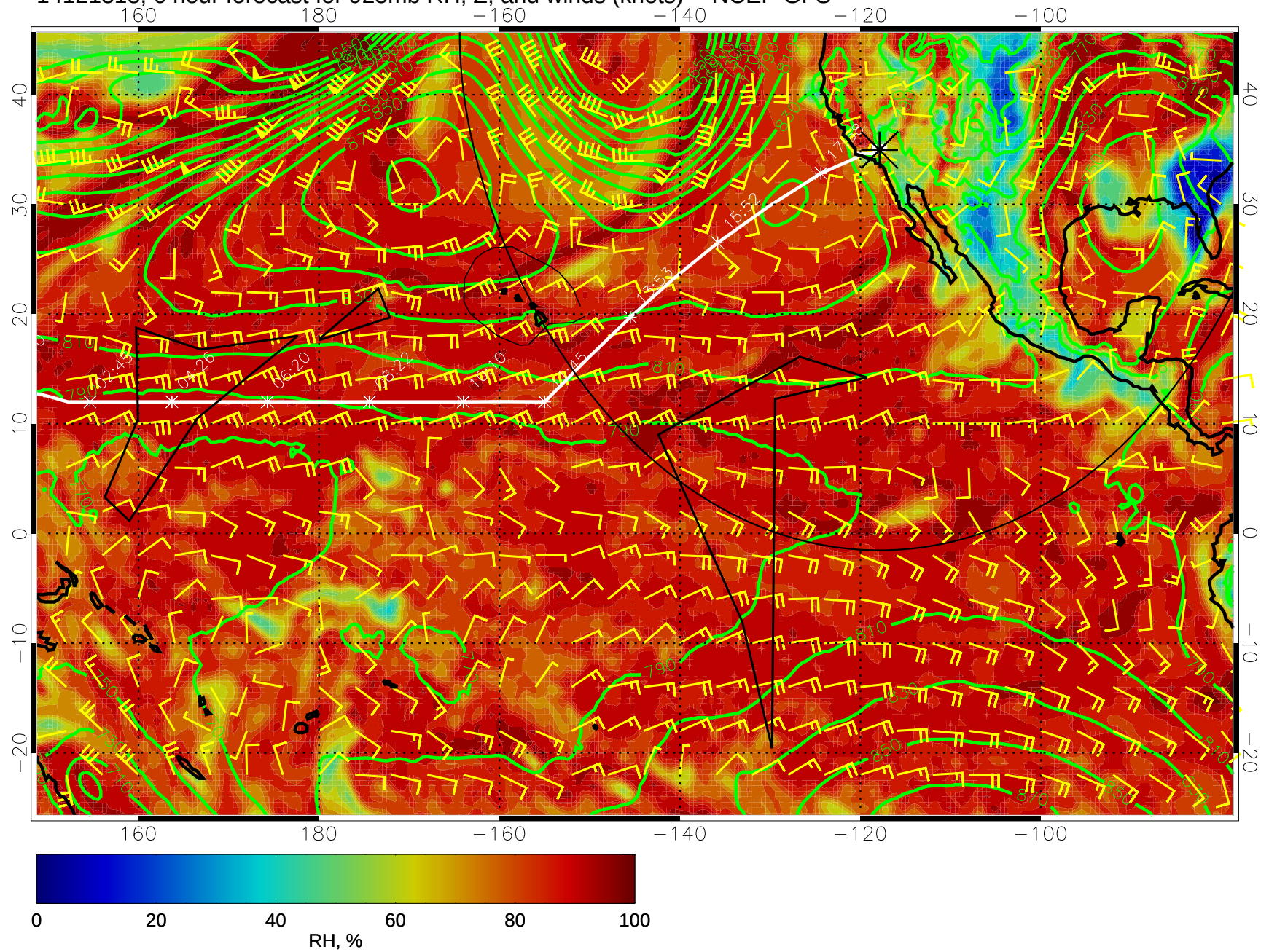
14121318, 6 hour forecast for 925mb RH, Z, and winds (knots) -- NCEP GFS
