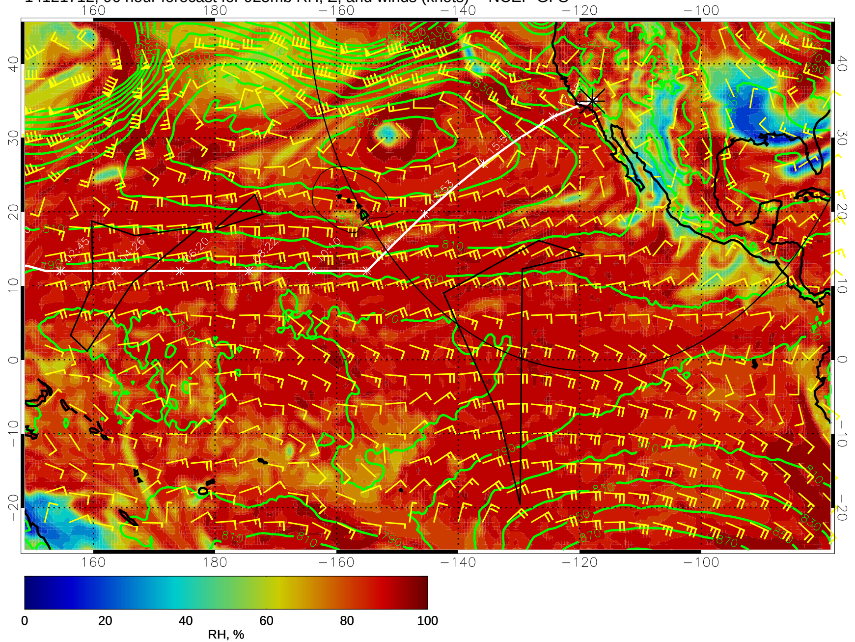
14121712, 96 hour forecast for 925mb RH, Z, and winds (knots) -- NCEP GFS
