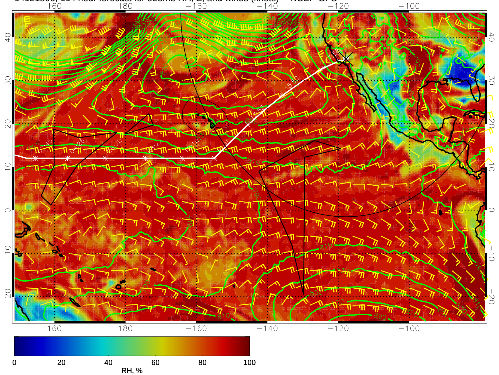
14121806, 114 hour forecast for 925mb RH, Z, and winds (knots) -- NCEP GFS
