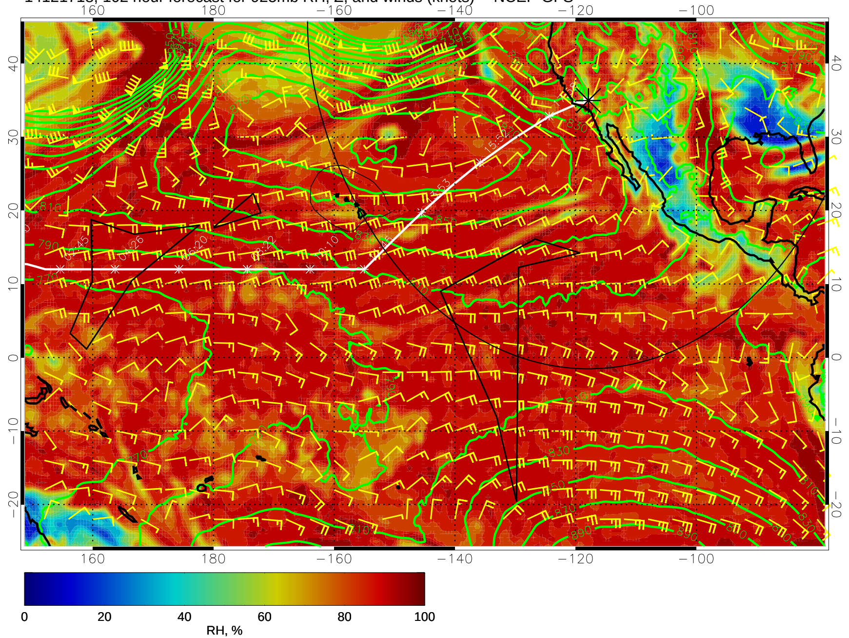
14121718, 102 hour forecast for 925mb RH, Z, and winds (knots) -- NCEP GFS
