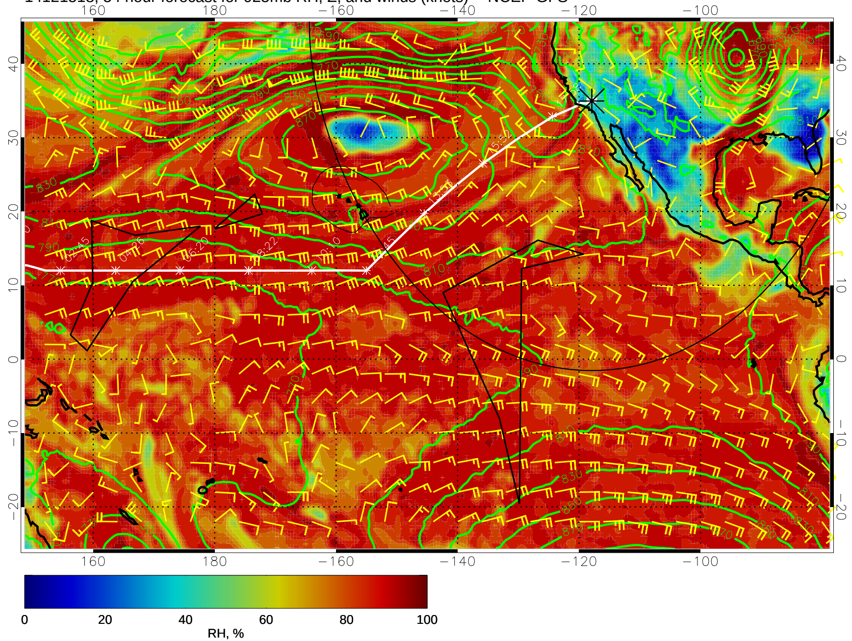
14121518, 54 hour forecast for 925mb RH, Z, and winds (knots) -- NCEP GFS
