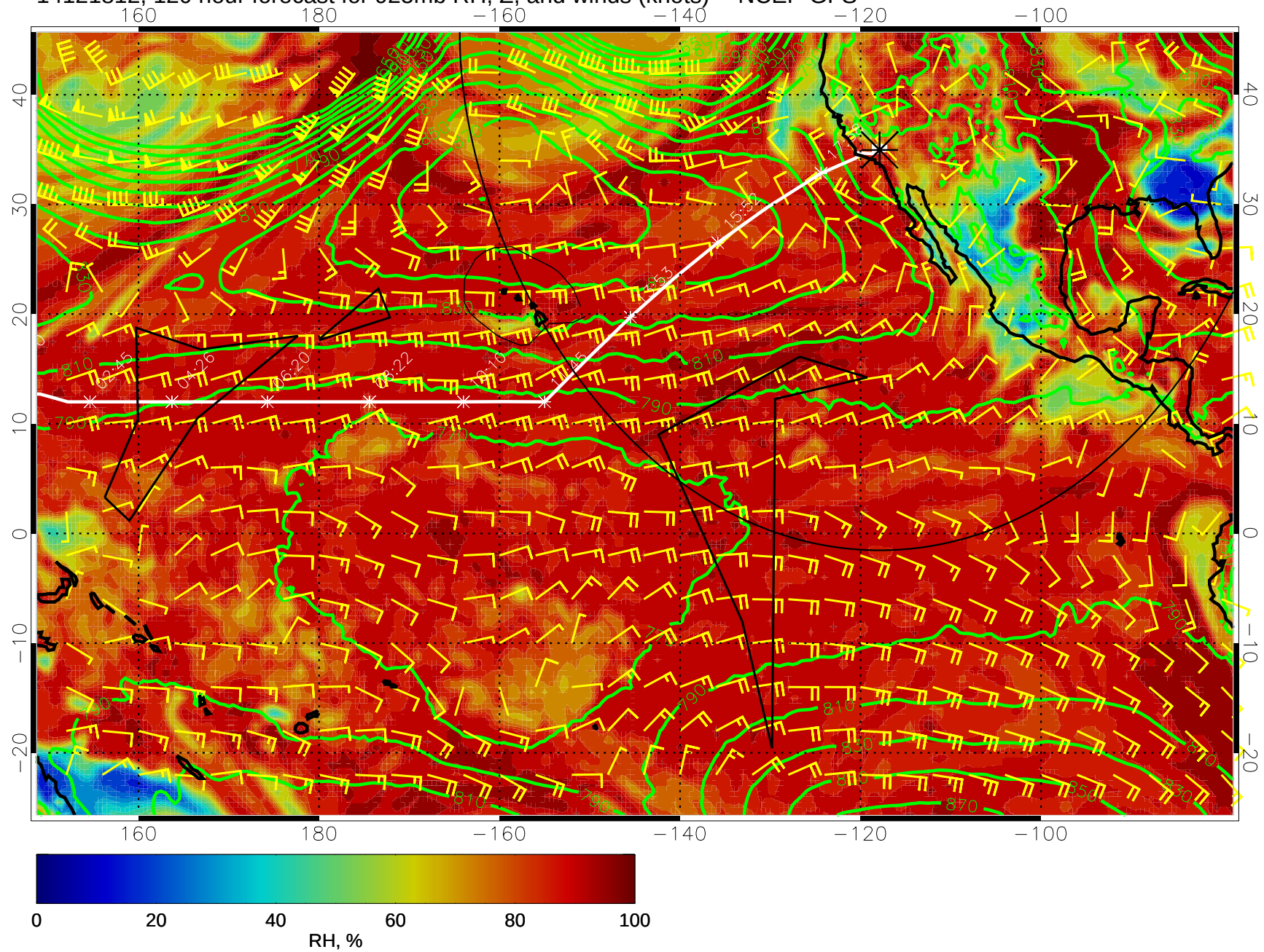
14121812, 120 hour forecast for 925mb RH, Z, and winds (knots) -- NCEP GFS
