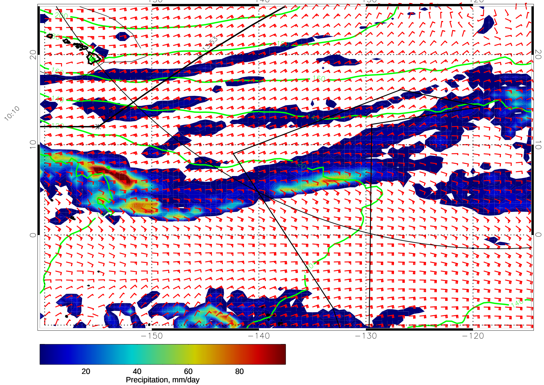
14121618, 78 hour forecast for precip, 1000mb Z, and winds (knots) -- NCEP GFS
