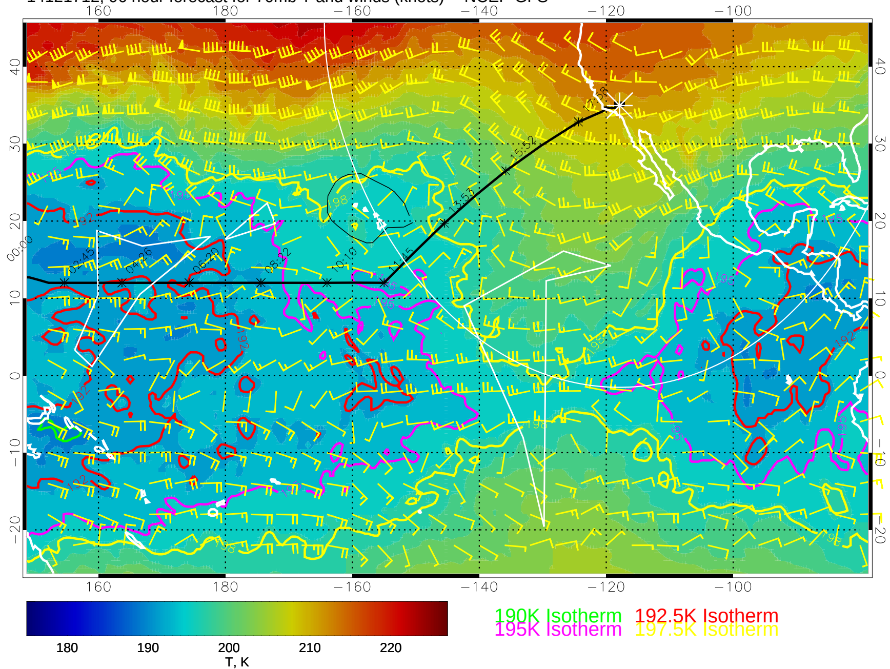
14121712, 96 hour forecast for 70mb T and winds (knots) -- NCEP GFS
