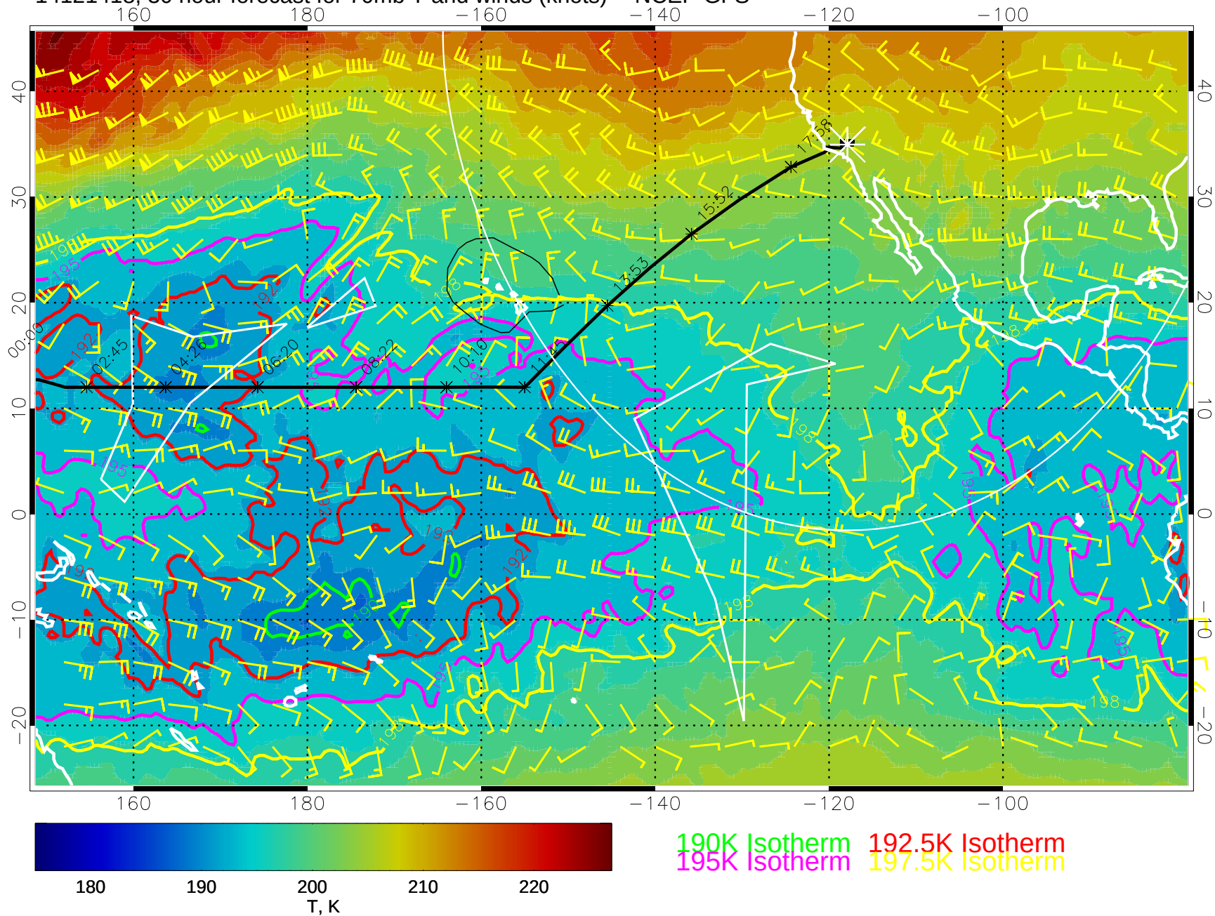
14121418, 30 hour forecast for 70mb T and winds (knots) -- NCEP GFS
