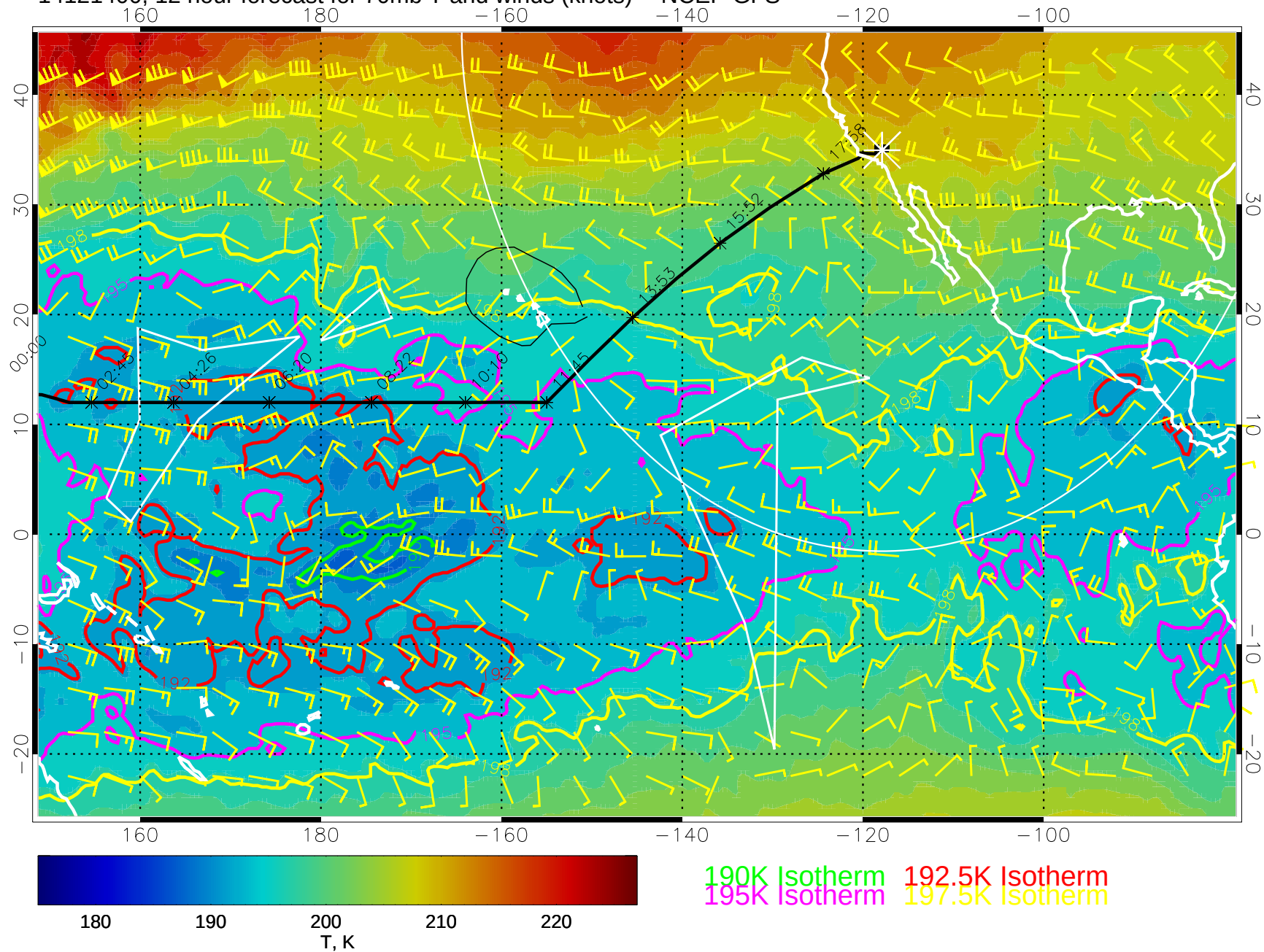
14121400, 12 hour forecast for 70mb T and winds (knots) -- NCEP GFS
