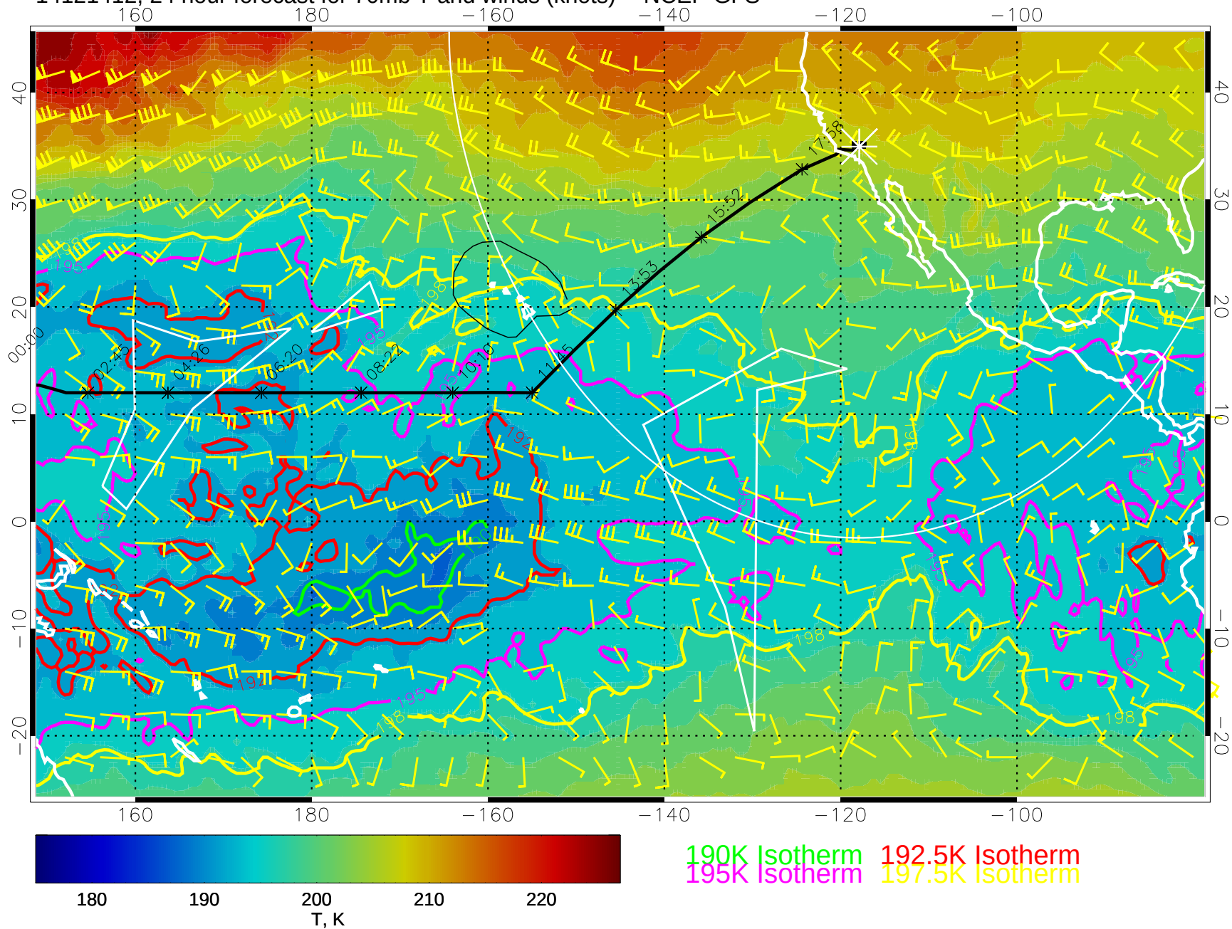
14121412, 24 hour forecast for 70mb T and winds (knots) -- NCEP GFS
