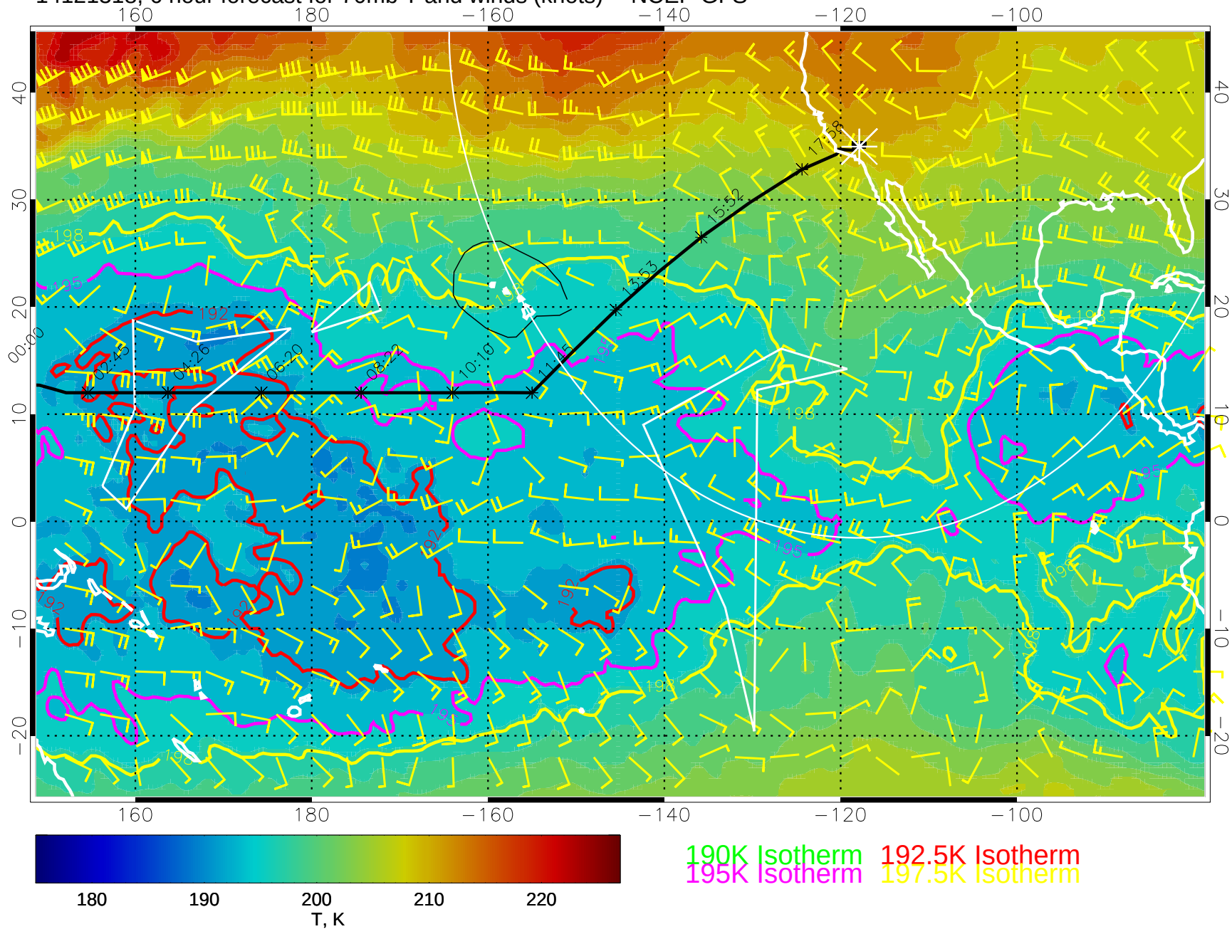
14121318, 6 hour forecast for 70mb T and winds (knots) -- NCEP GFS
