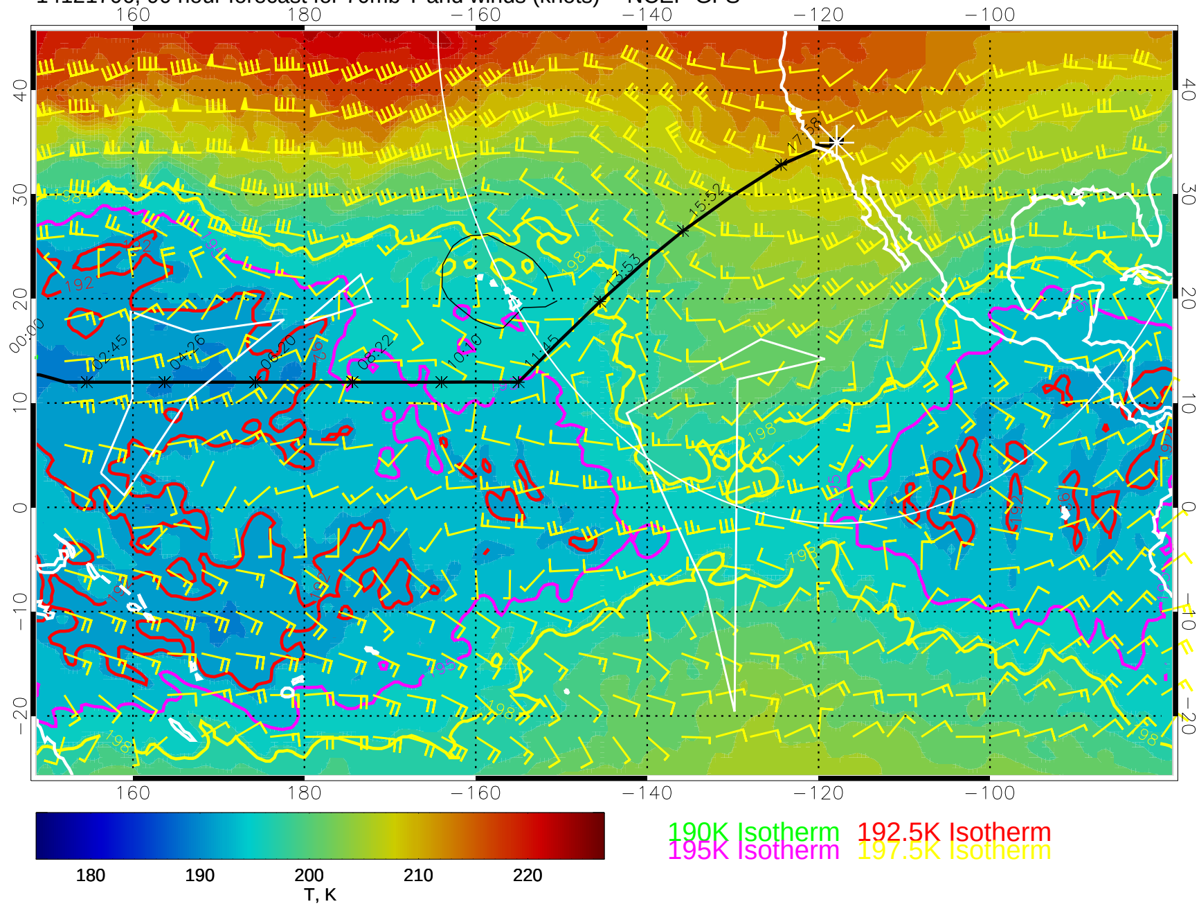
14121706, 90 hour forecast for 70mb T and winds (knots) -- NCEP GFS
