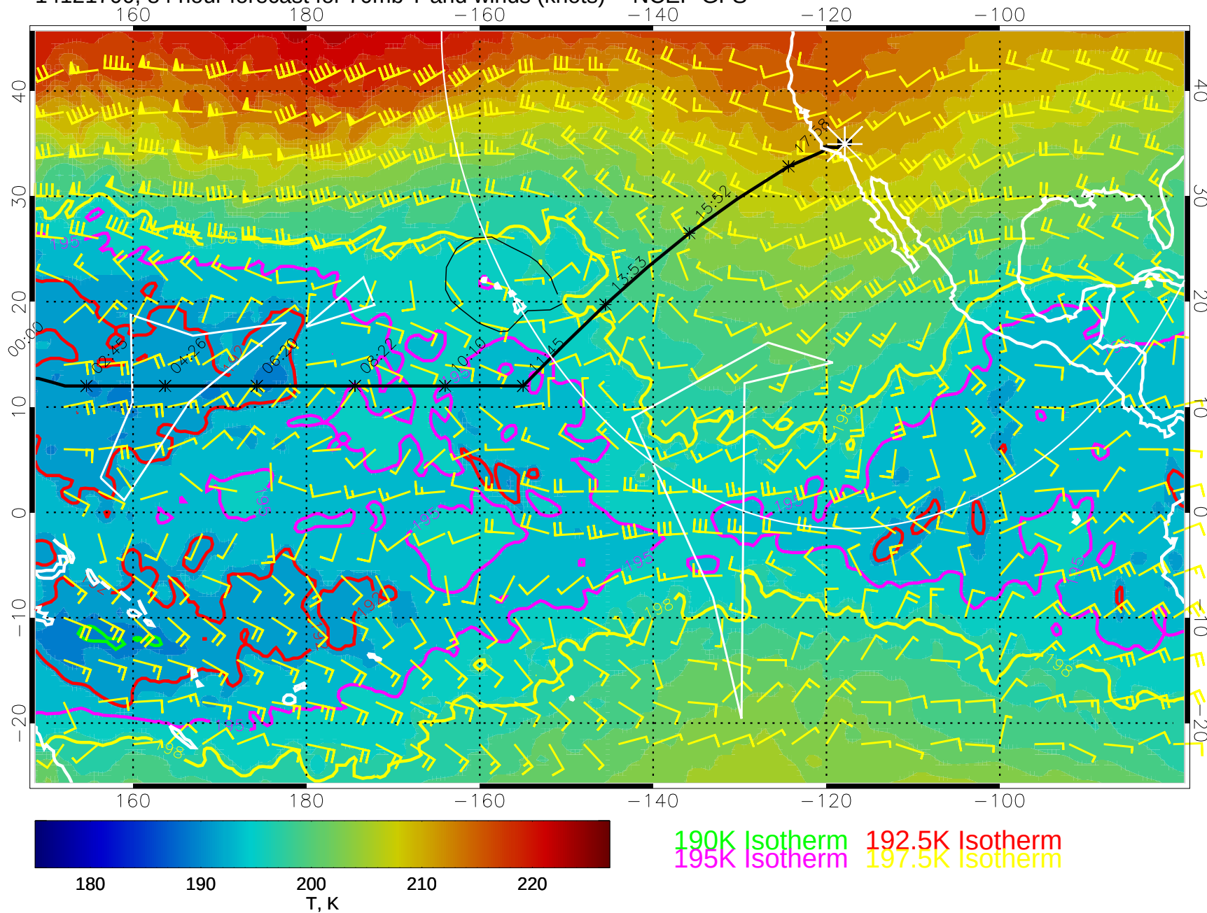
14121700, 84 hour forecast for 70mb T and winds (knots) -- NCEP GFS
