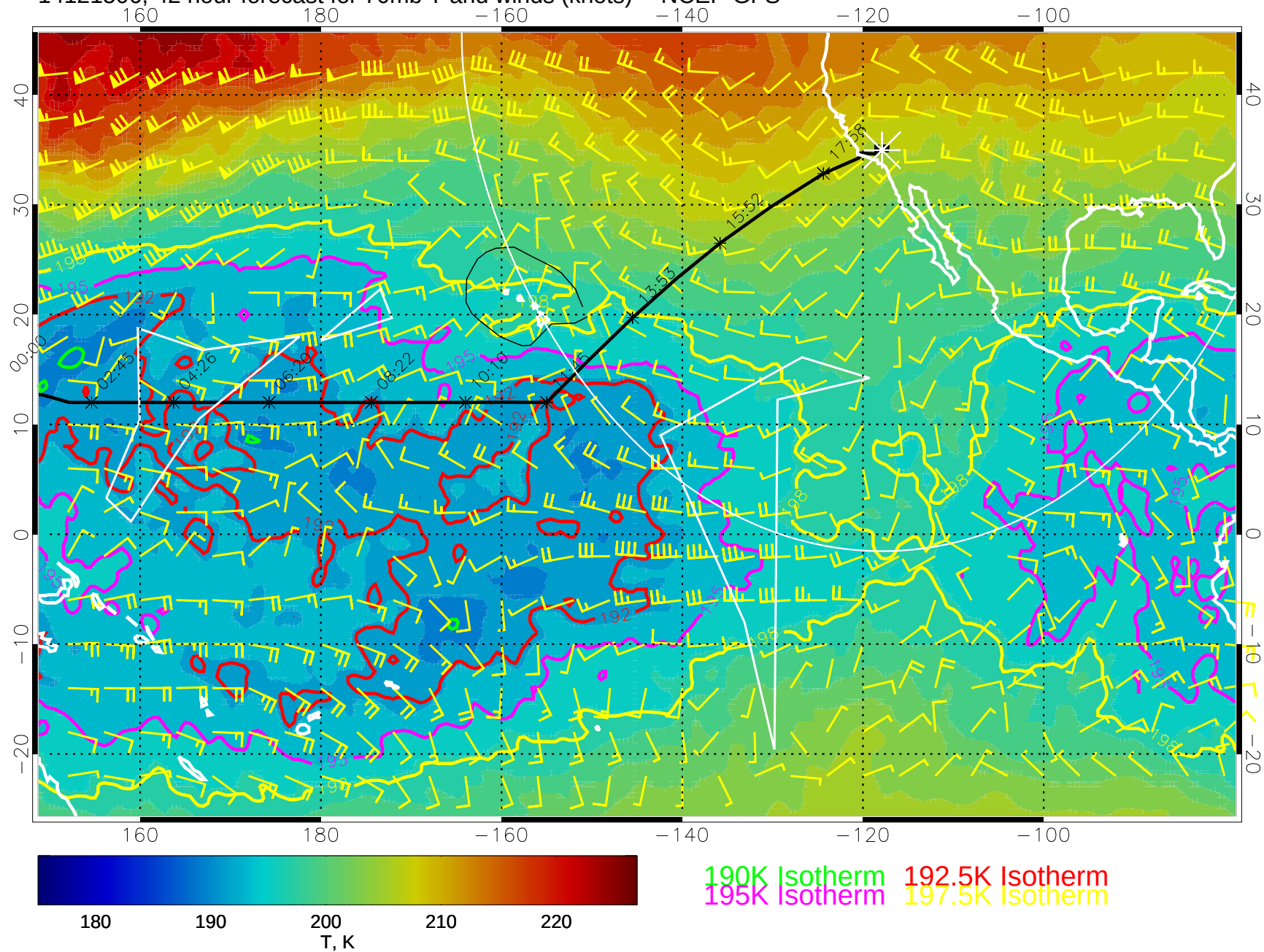
14121506, 42 hour forecast for 70mb T and winds (knots) -- NCEP GFS
