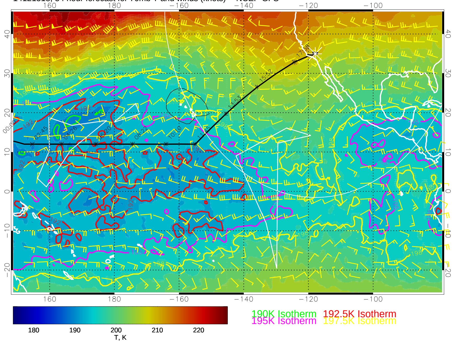
14121518, 54 hour forecast for 70mb T and winds (knots) -- NCEP GFS
