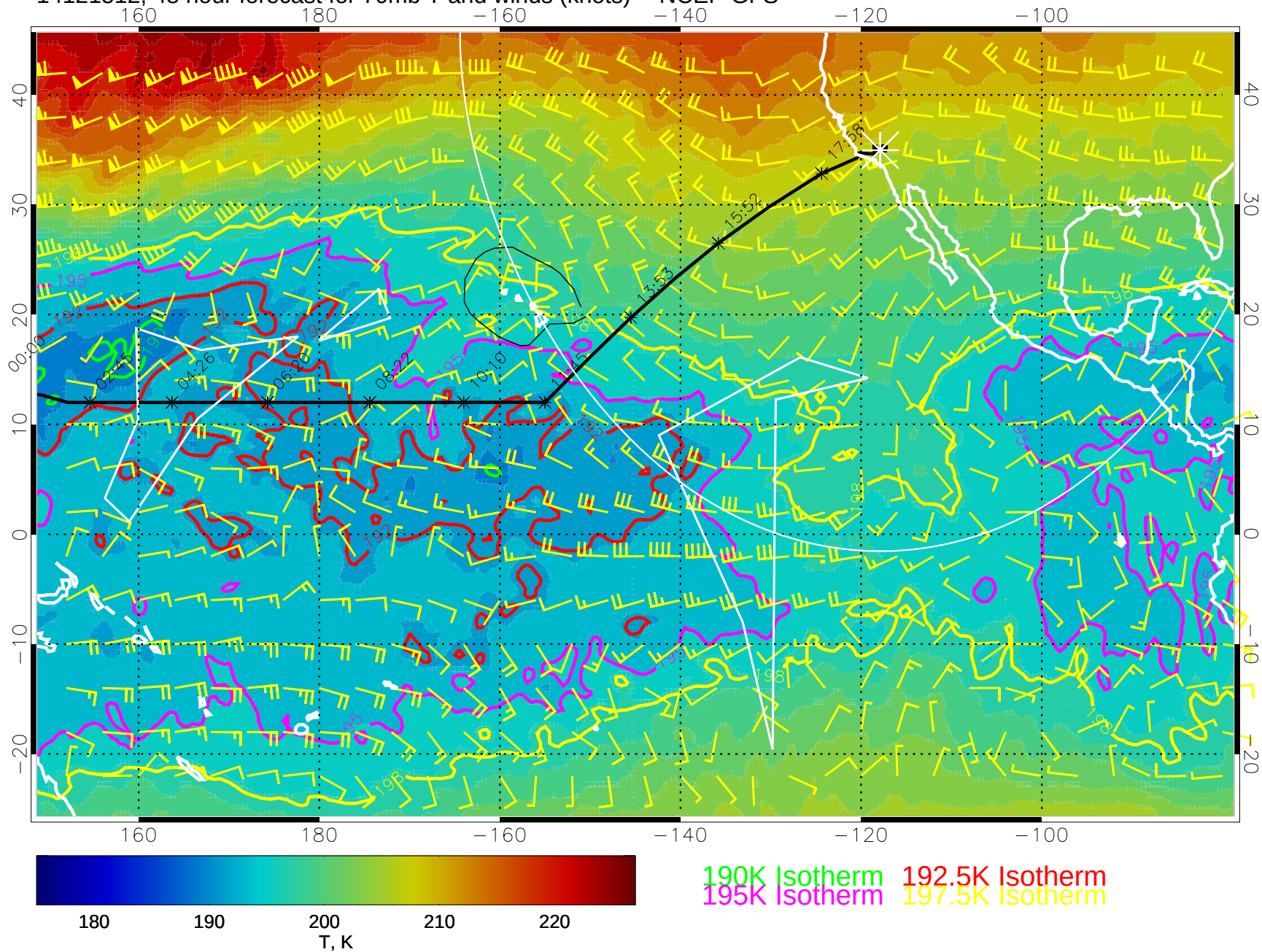
14121512, 48 hour forecast for 70mb T and winds (knots) -- NCEP GFS
