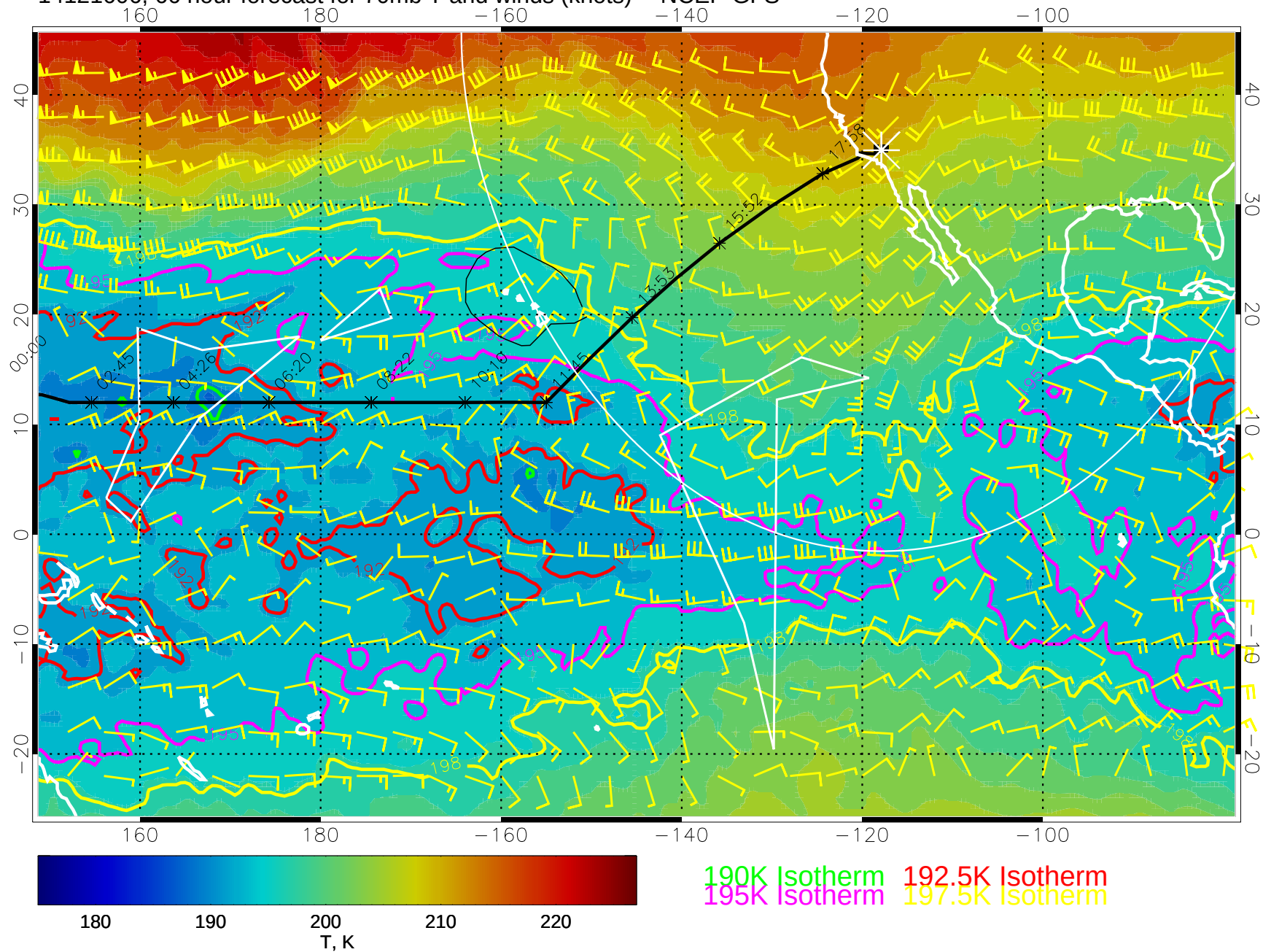
14121606, 66 hour forecast for 70mb T and winds (knots) -- NCEP GFS
