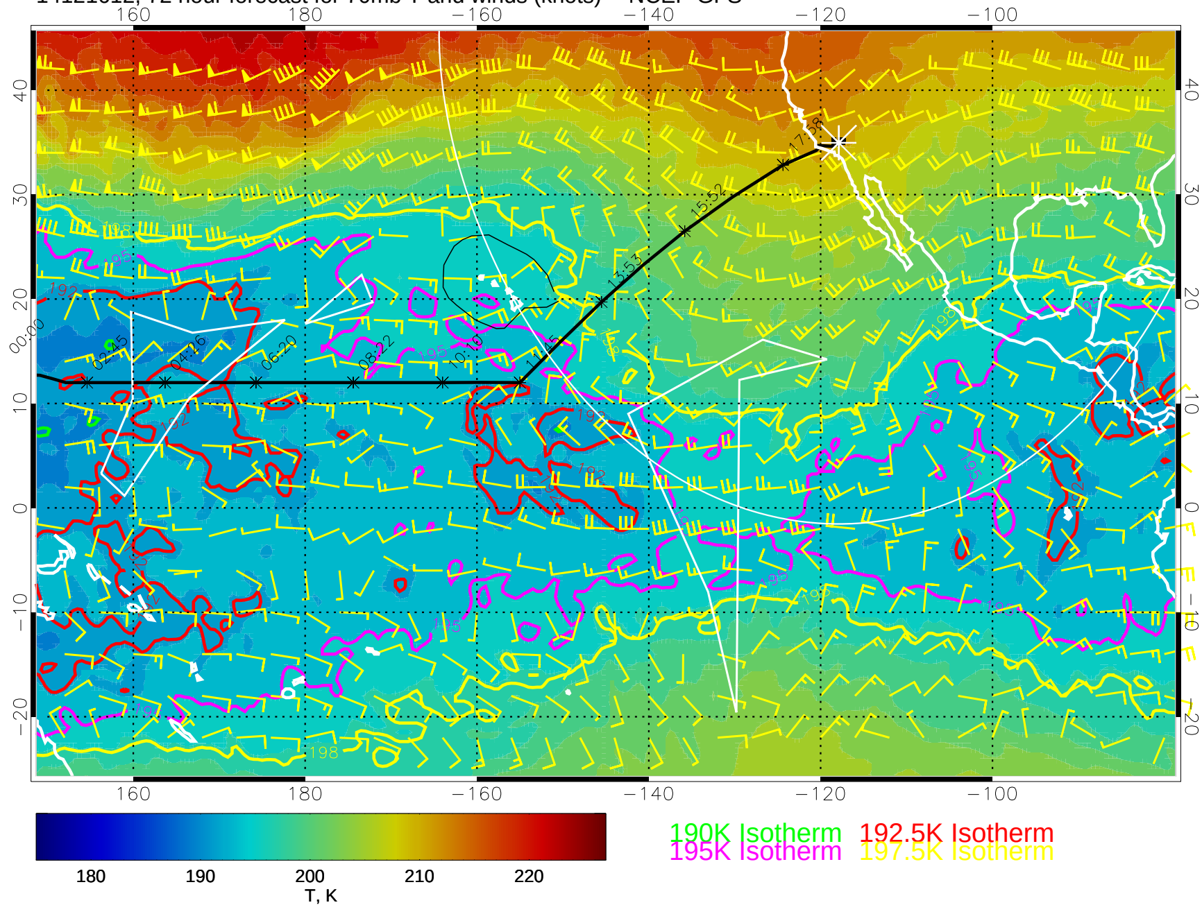
14121612, 72 hour forecast for 70mb T and winds (knots) -- NCEP GFS
