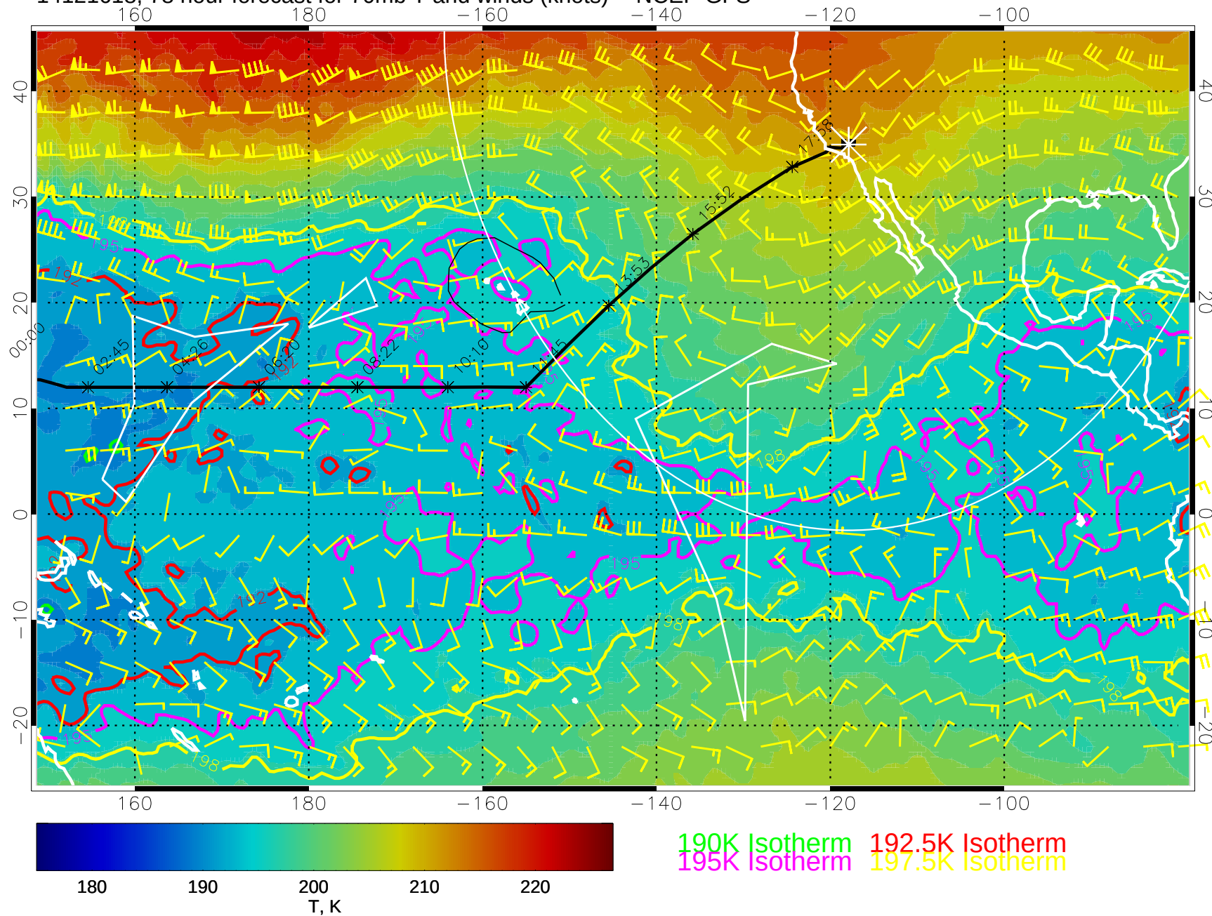
14121618, 78 hour forecast for 70mb T and winds (knots) -- NCEP GFS
