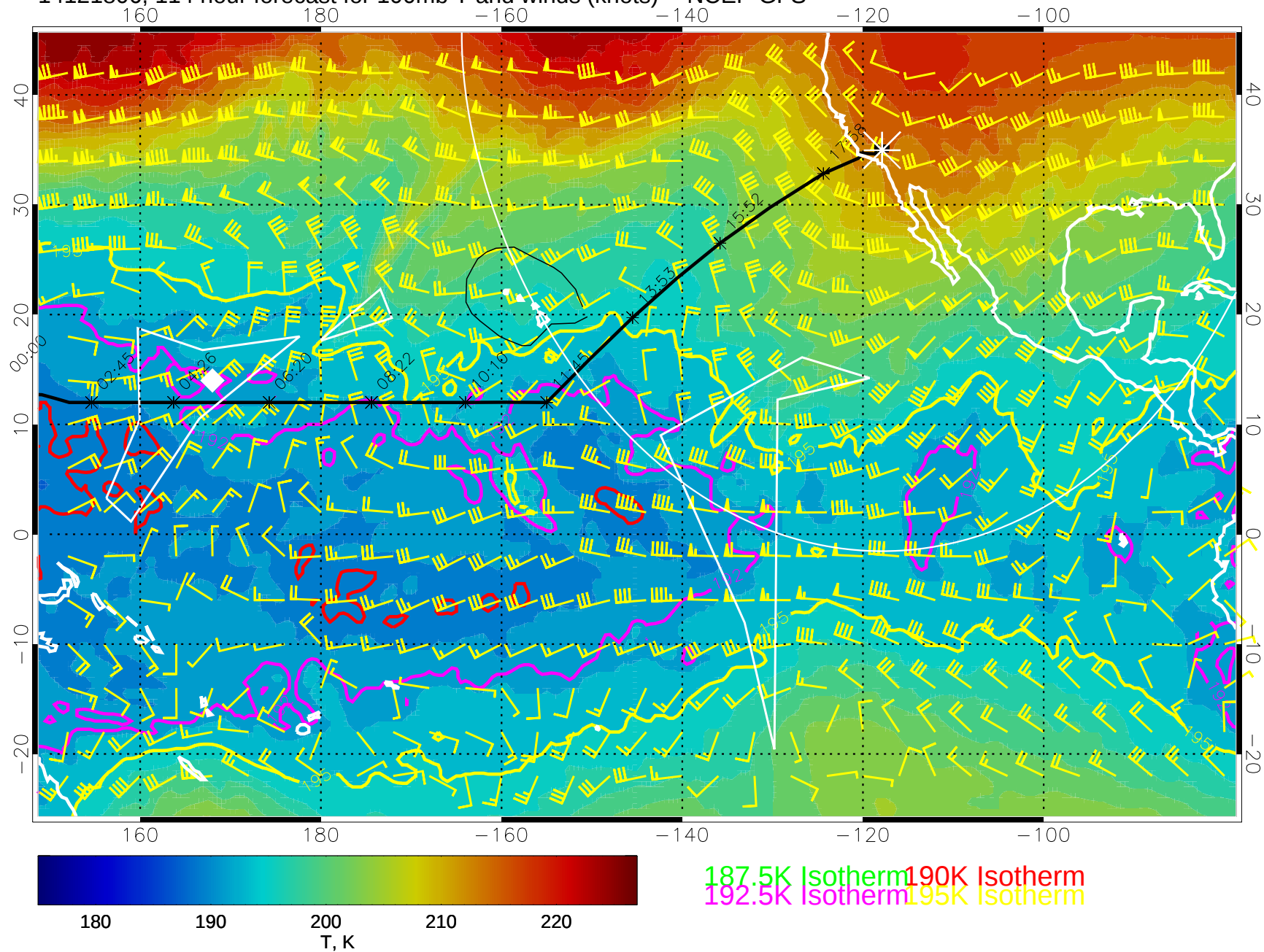
14121806, 114 hour forecast for 100mb T and winds (knots) -- NCEP GFS
