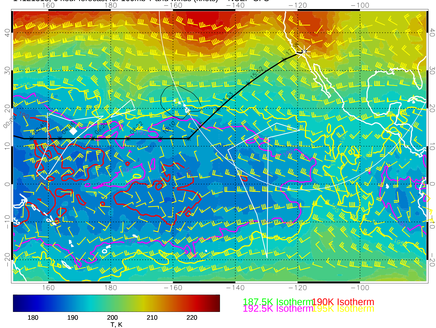
14121318, 6 hour forecast for 100mb T and winds (knots) -- NCEP GFS
