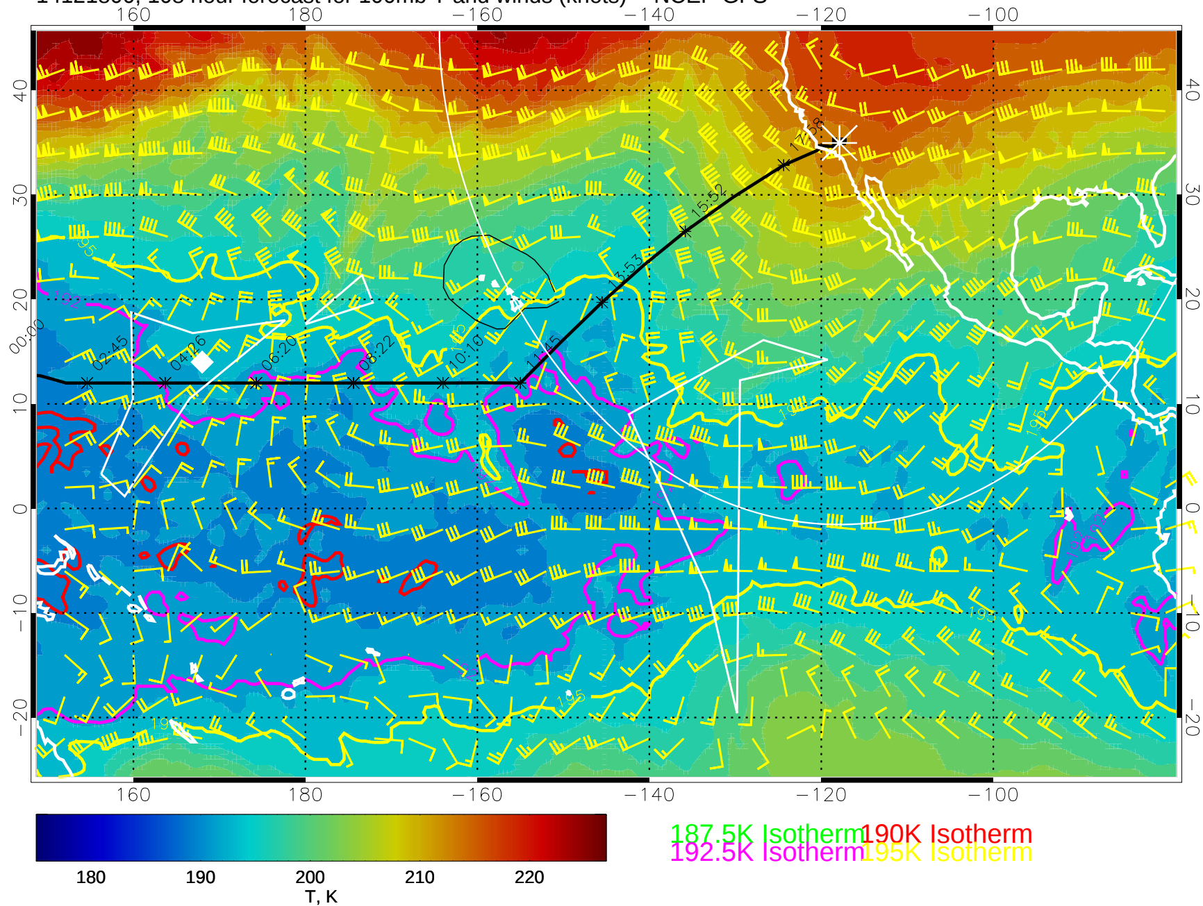
14121800, 108 hour forecast for 100mb T and winds (knots) -- NCEP GFS
