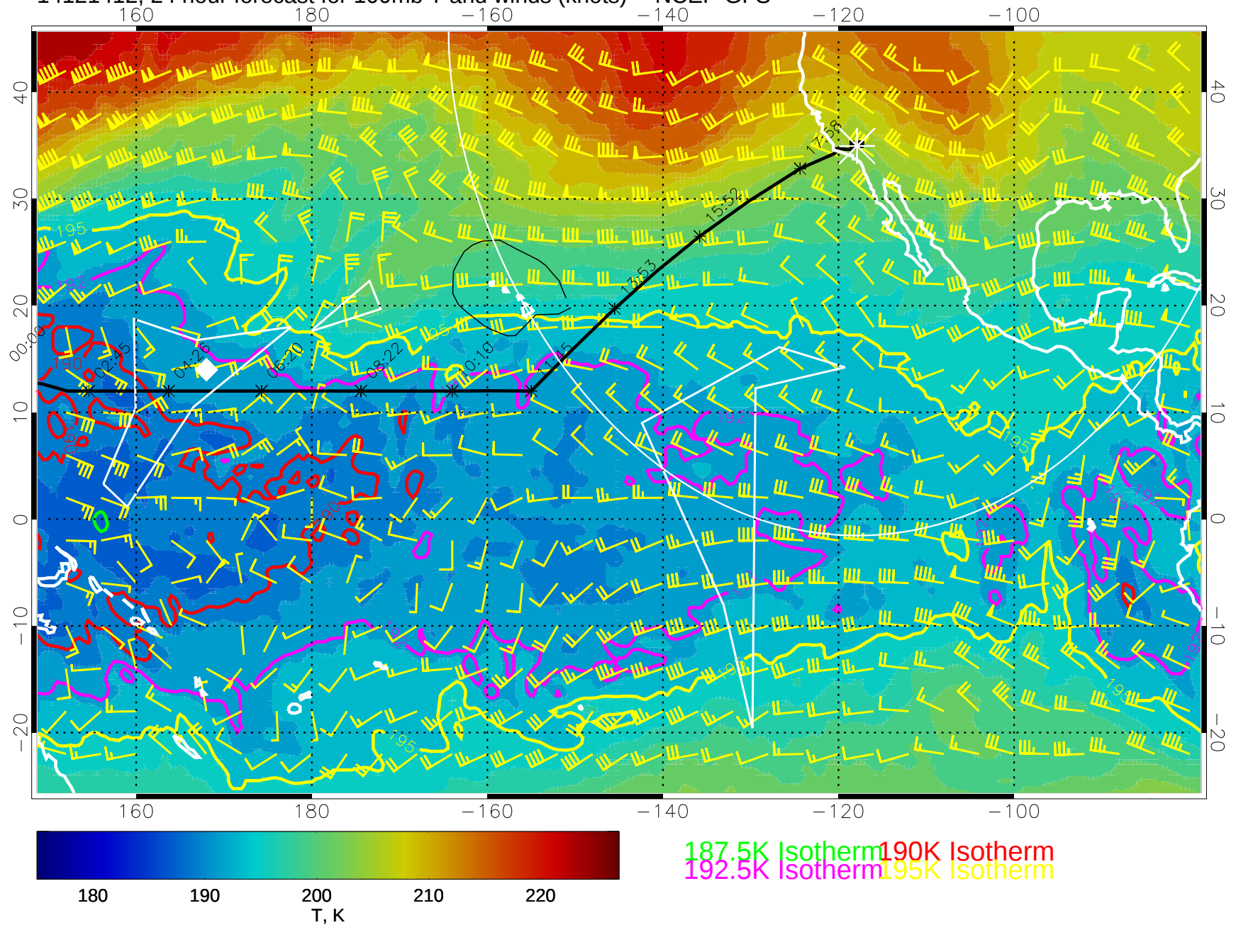
14121412, 24 hour forecast for 100mb T and winds (knots) -- NCEP GFS
