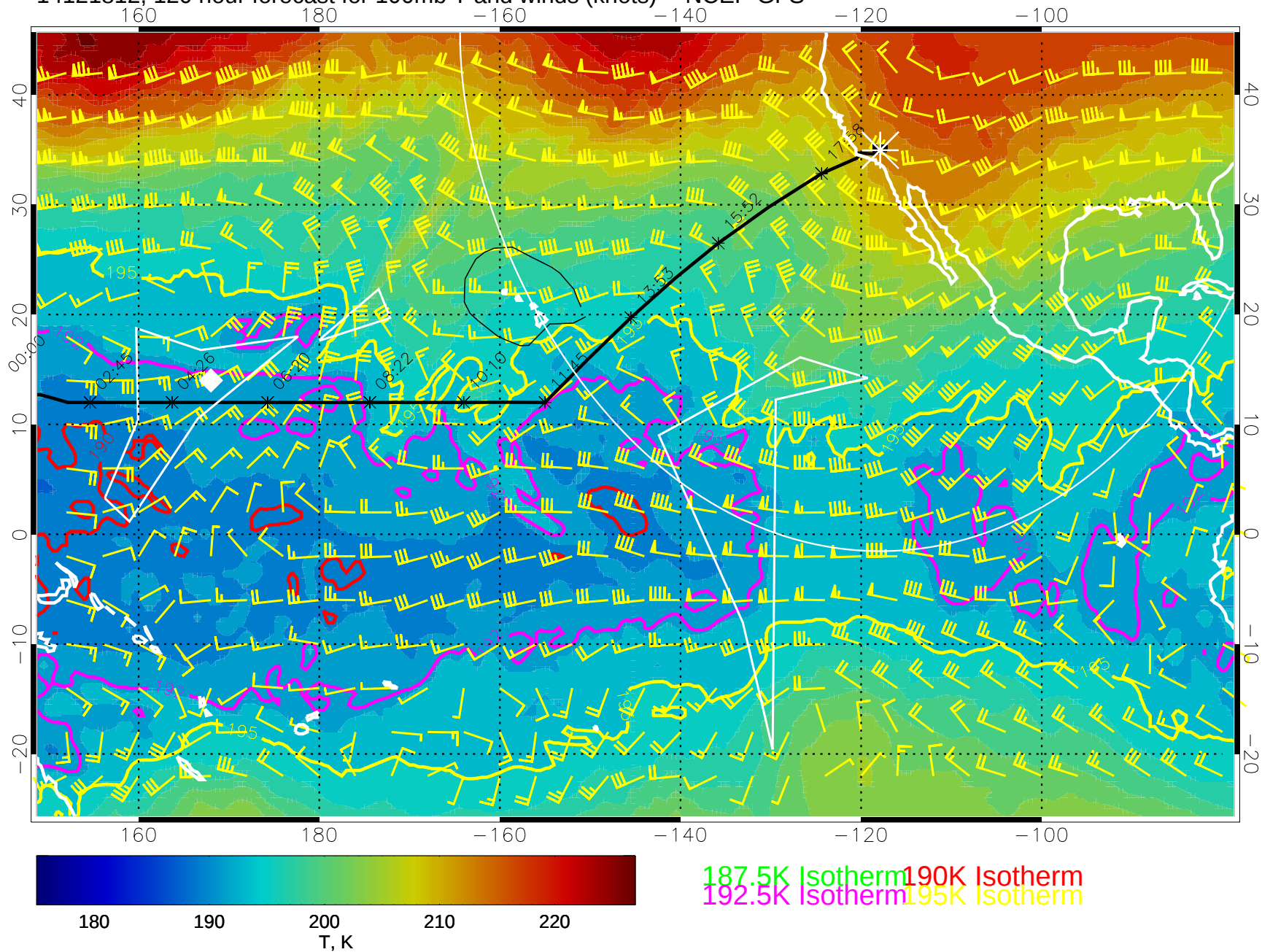
14121812, 120 hour forecast for 100mb T and winds (knots) -- NCEP GFS
