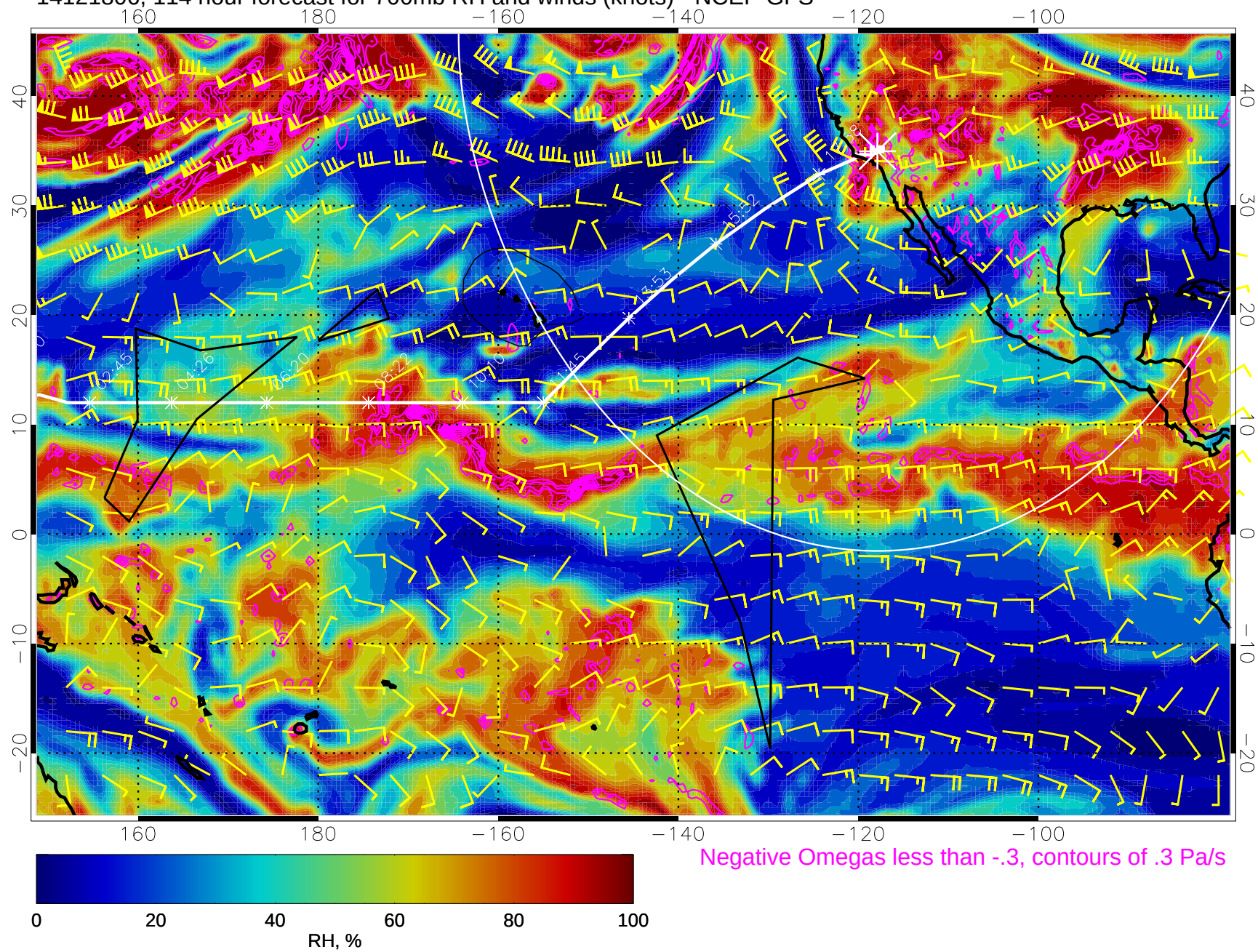
14121806, 114 hour forecast for 700mb RH and winds (knots) - NCEP GFS
