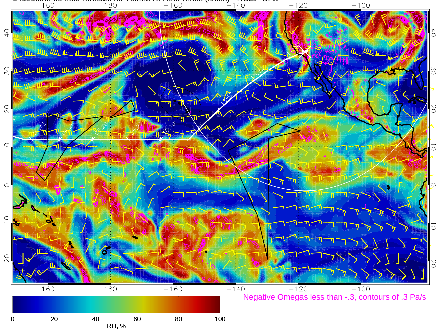
14121606, 66 hour forecast for 700mb RH and winds (knots) - NCEP GFS
