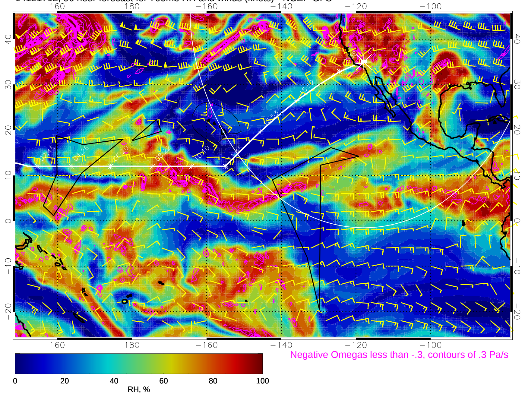
14121712, 96 hour forecast for 700mb RH and winds (knots) - NCEP GFS
