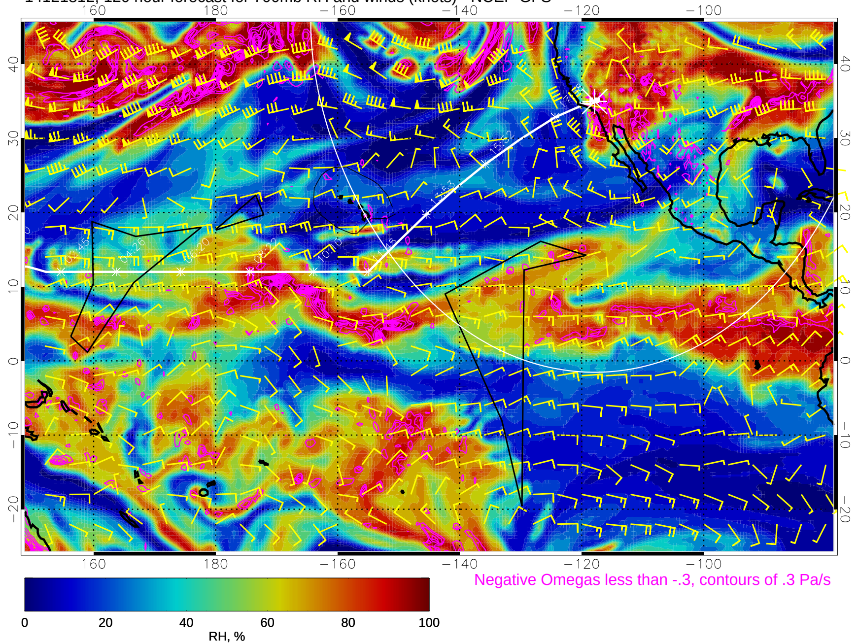
14121812, 120 hour forecast for 700mb RH and winds (knots) - NCEP GFS
