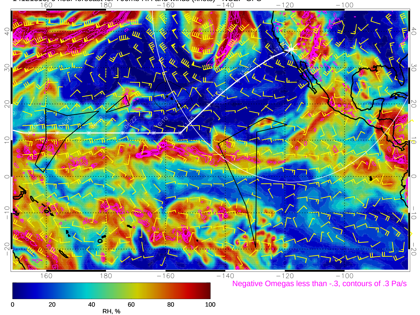
14121318, 6 hour forecast for 700mb RH and winds (knots) - NCEP GFS
