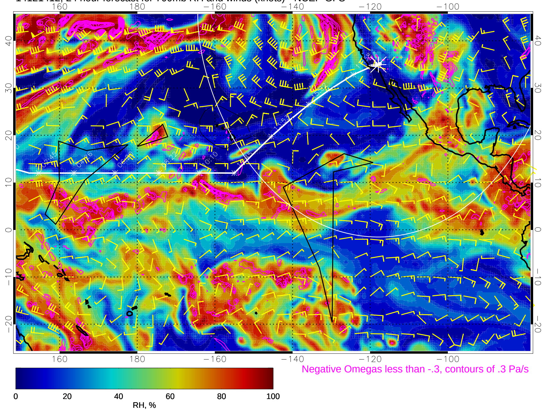
14121412, 24 hour forecast for 700mb RH and winds (knots) - NCEP GFS
