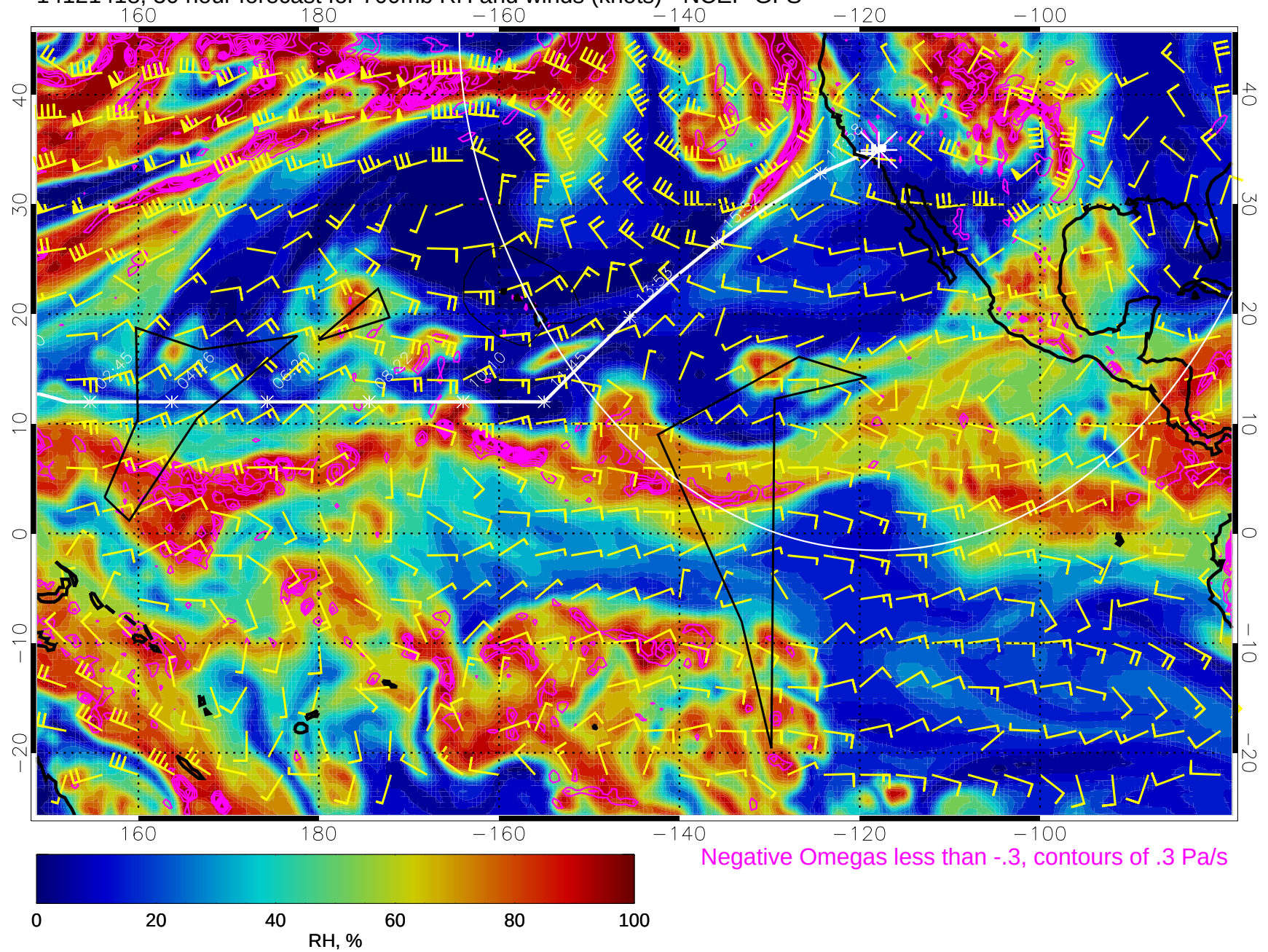
14121418, 30 hour forecast for 700mb RH and winds (knots) - NCEP GFS
