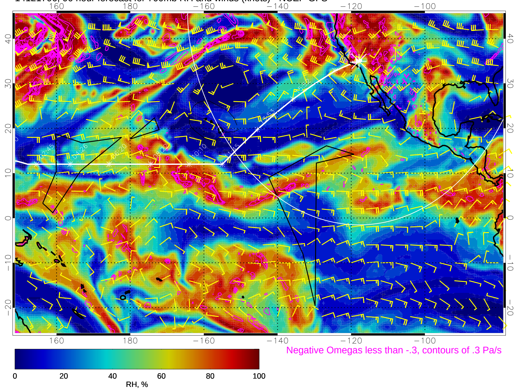
14121706, 90 hour forecast for 700mb RH and winds (knots) - NCEP GFS
