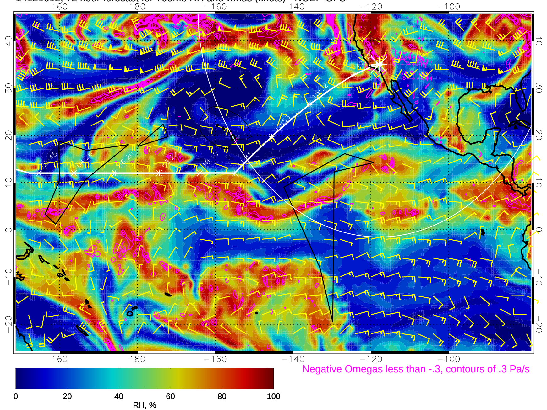
14121612, 72 hour forecast for 700mb RH and winds (knots) - NCEP GFS
