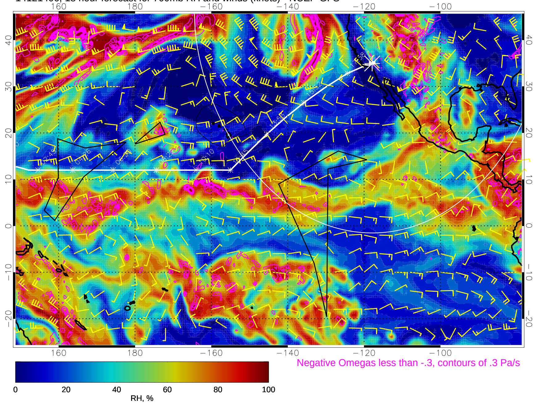
14121406, 18 hour forecast for 700mb RH and winds (knots) - NCEP GFS
