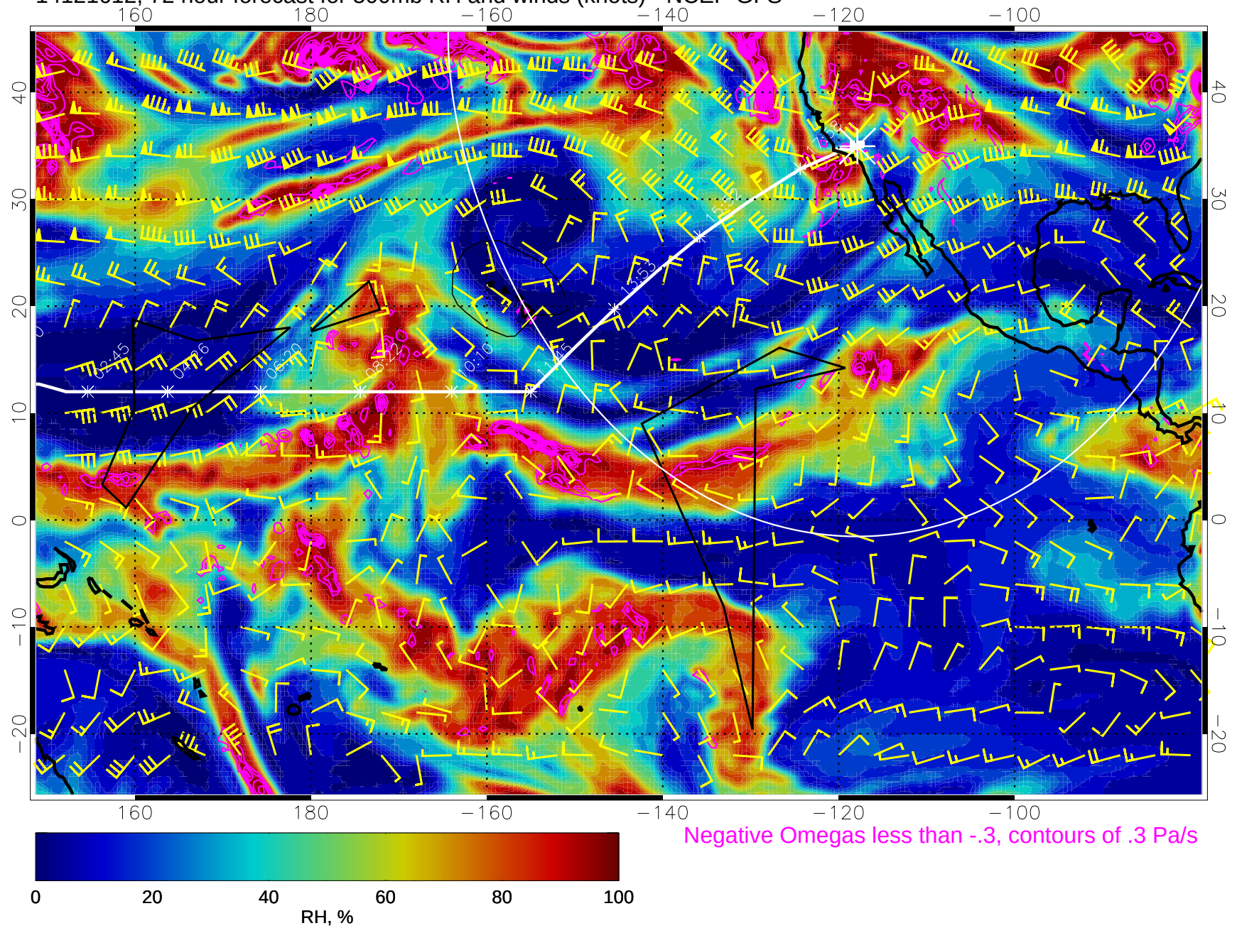
14121612, 72 hour forecast for 500mb RH and winds (knots) - NCEP GFS
