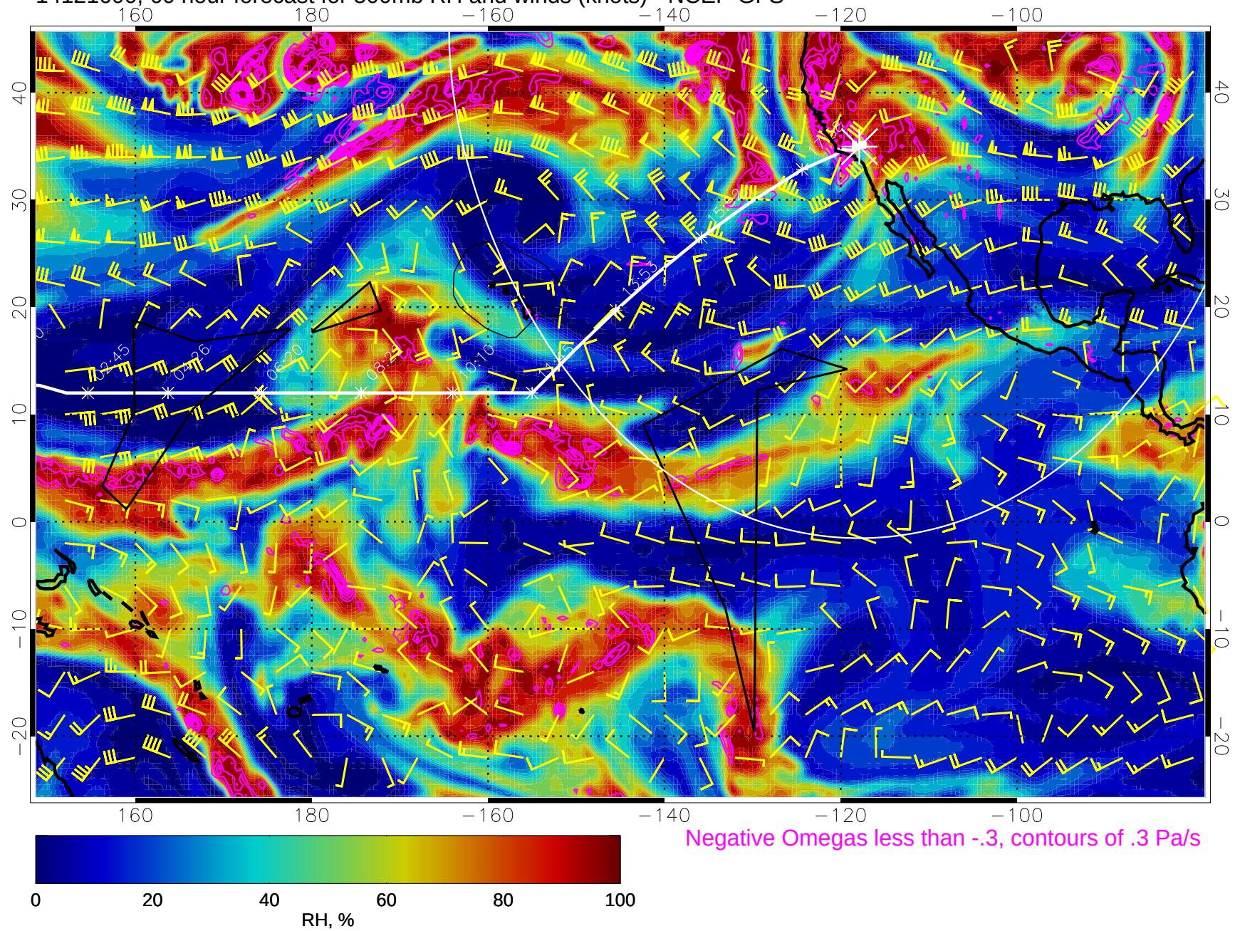
14121600, 60 hour forecast for 500mb RH and winds (knots) - NCEP GFS
