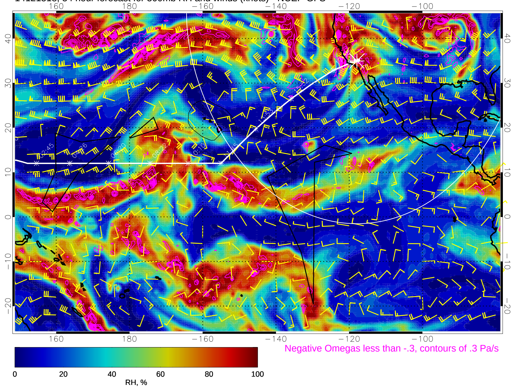
14121518, 54 hour forecast for 500mb RH and winds (knots) - NCEP GFS
