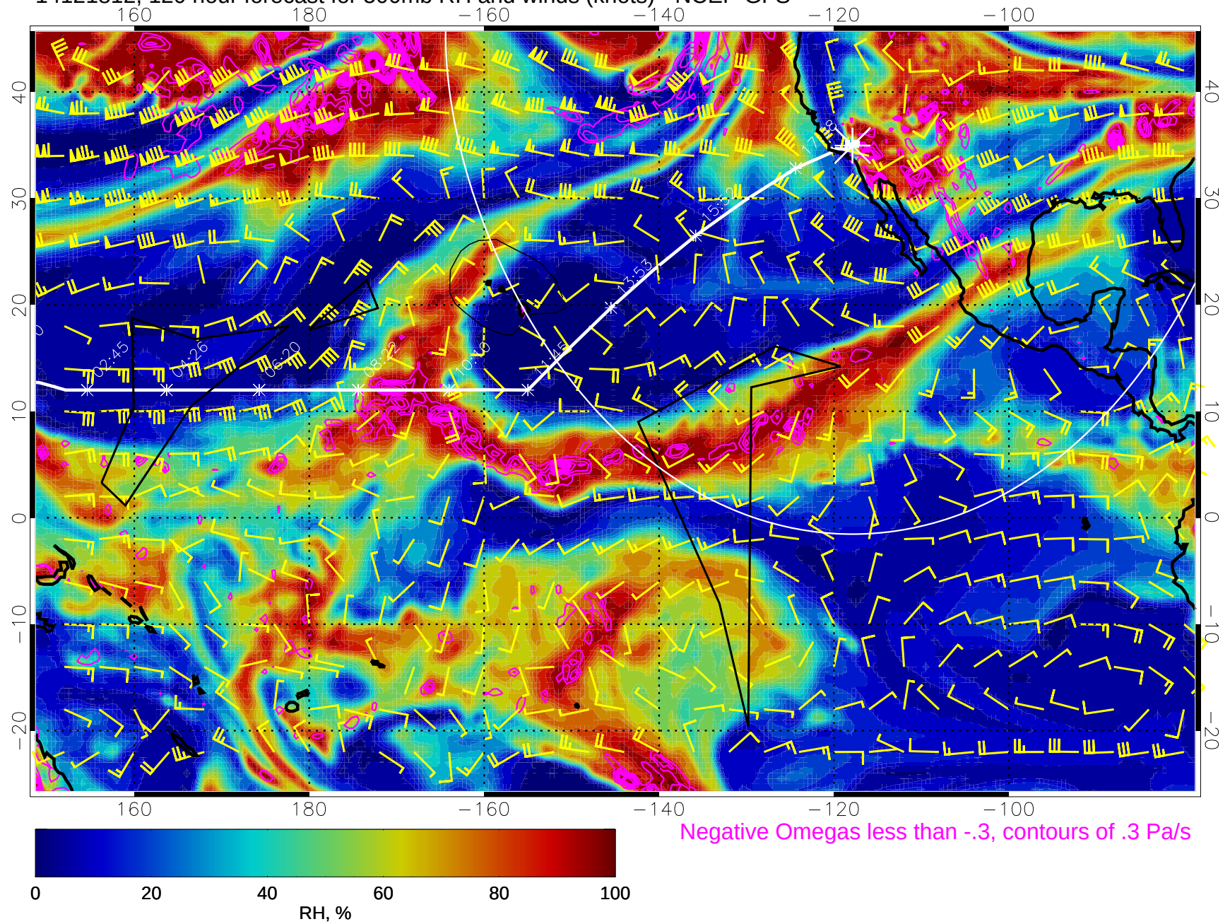
14121812, 120 hour forecast for 500mb RH and winds (knots) - NCEP GFS
