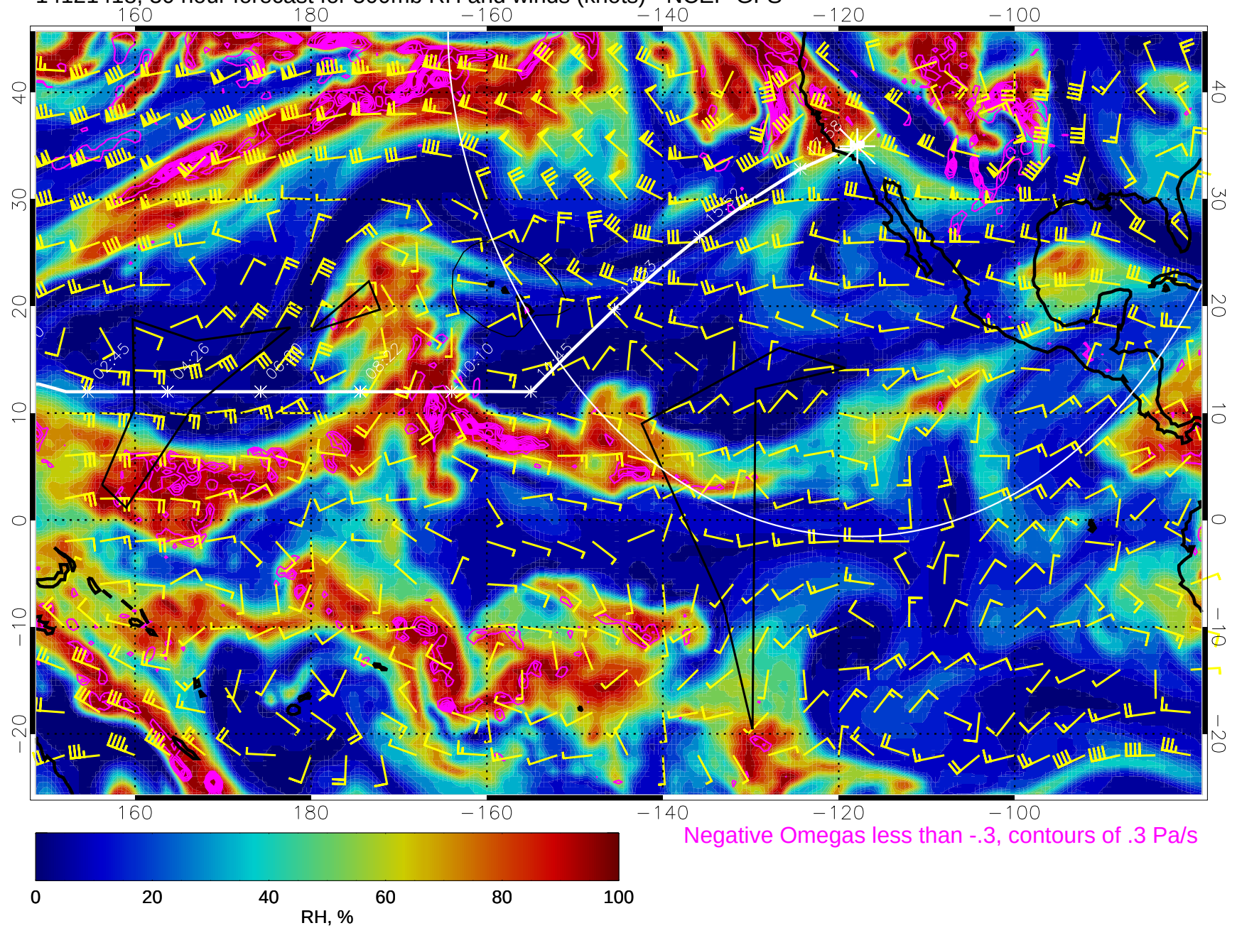
14121418, 30 hour forecast for 500mb RH and winds (knots) - NCEP GFS
