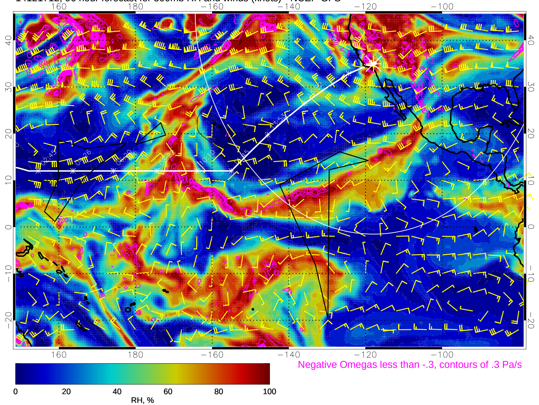
14121712, 96 hour forecast for 500mb RH and winds (knots) - NCEP GFS
