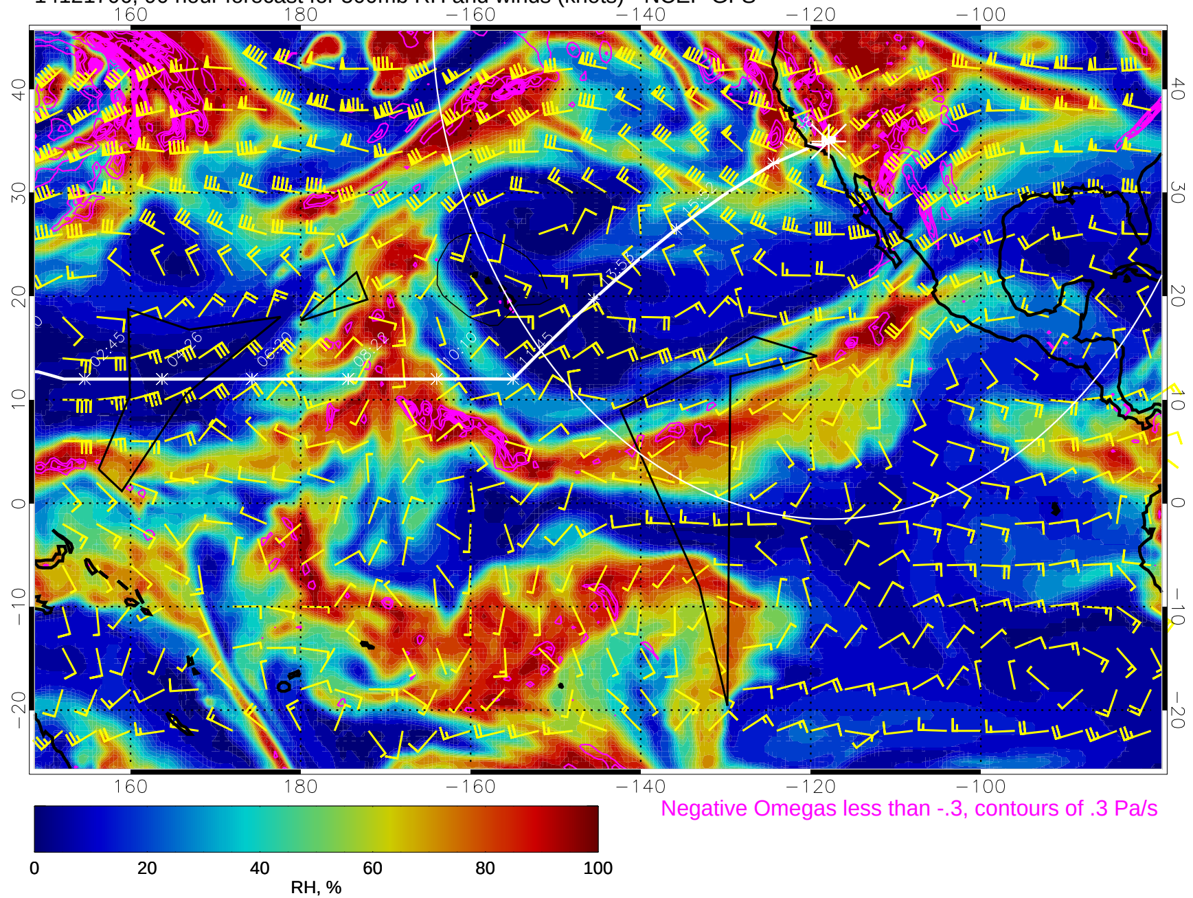
14121706, 90 hour forecast for 500mb RH and winds (knots) - NCEP GFS
