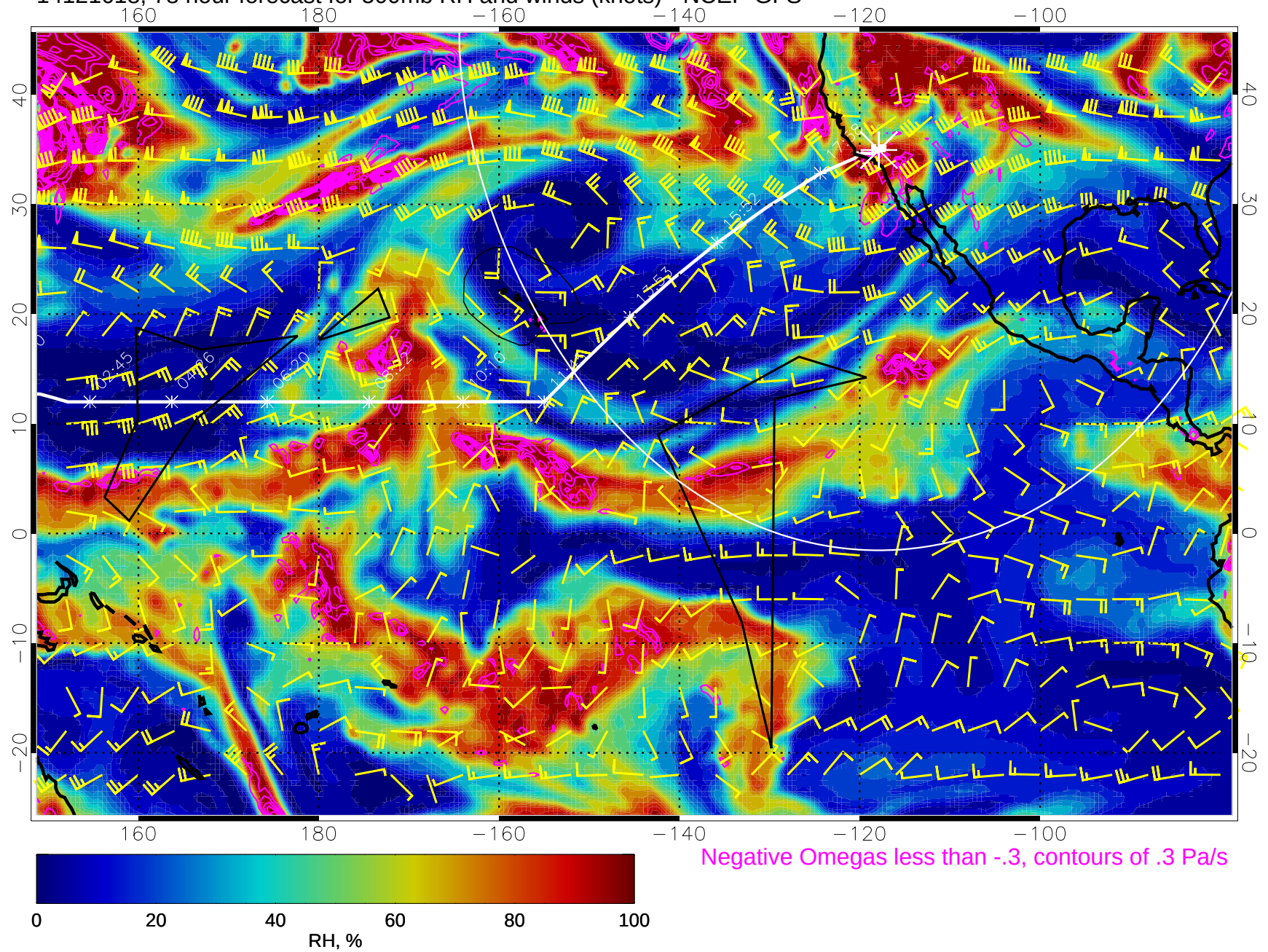
14121618, 78 hour forecast for 500mb RH and winds (knots) - NCEP GFS
