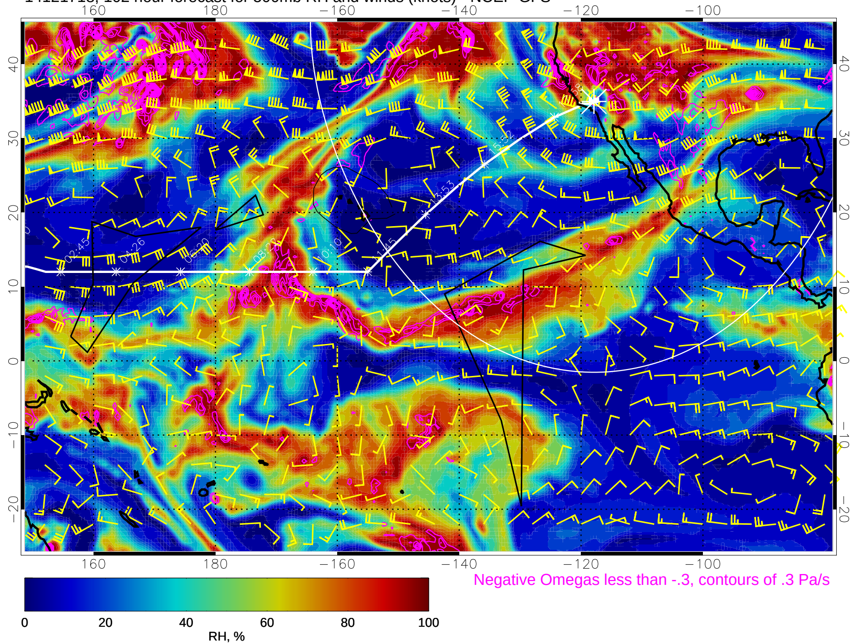
14121718, 102 hour forecast for 500mb RH and winds (knots) - NCEP GFS
