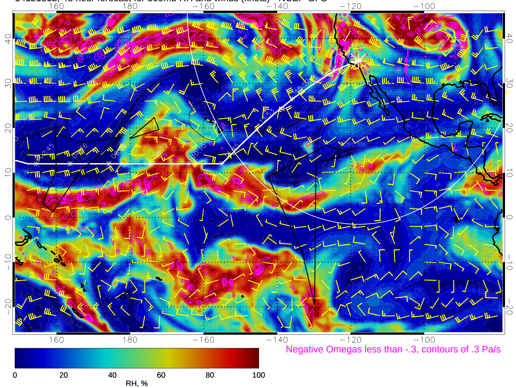
14121512, 48 hour forecast for 500mb RH and winds (knots) - NCEP GFS
