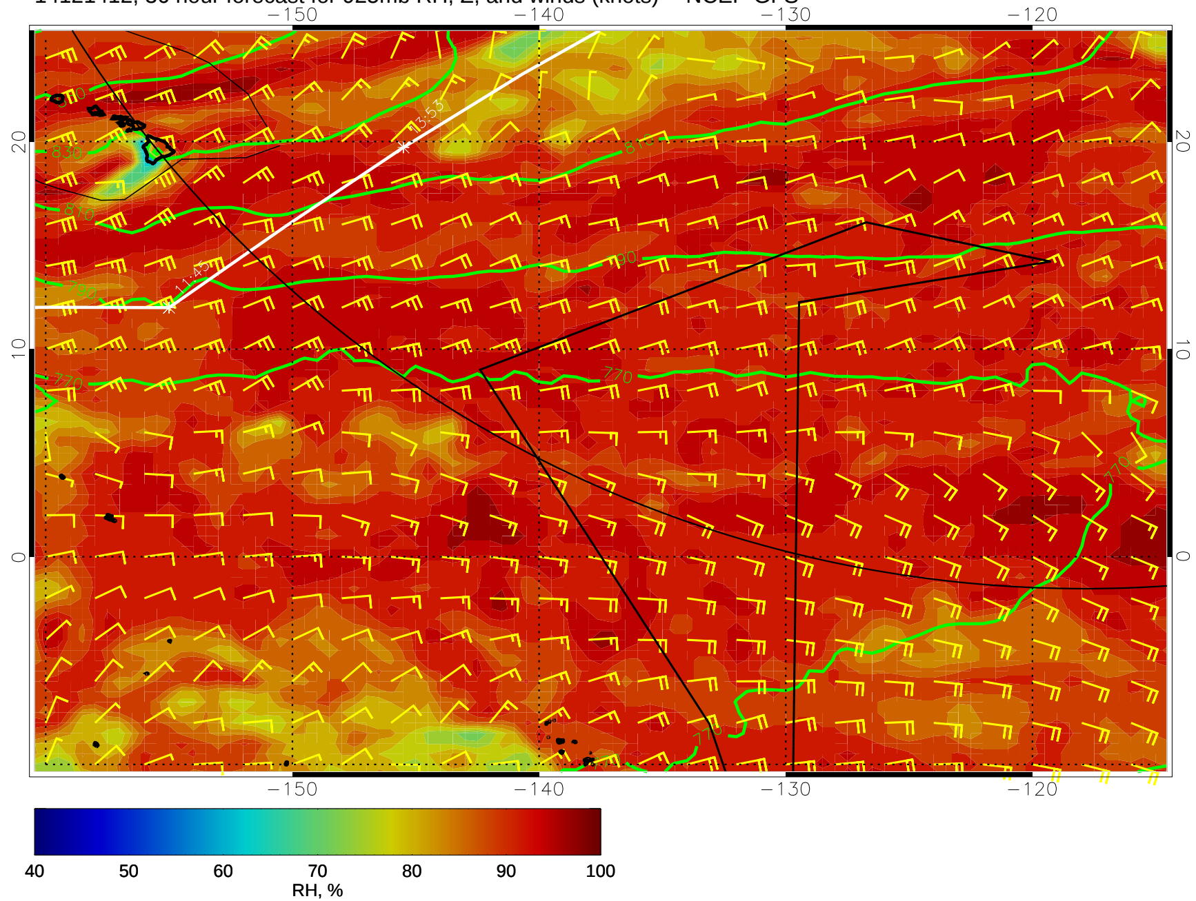
14121412, 36 hour forecast for 925mb RH, Z, and winds (knots) -- NCEP GFS
