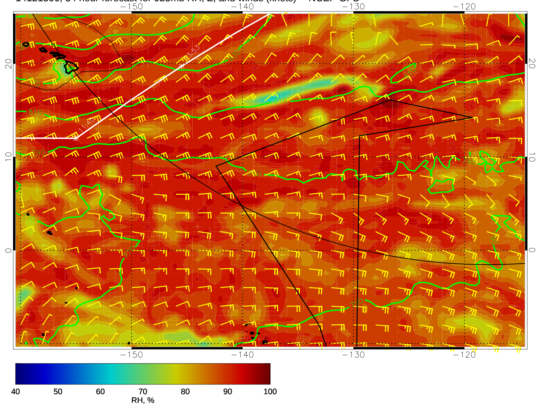
14121506, 54 hour forecast for 925mb RH, Z, and winds (knots) -- NCEP GFS
