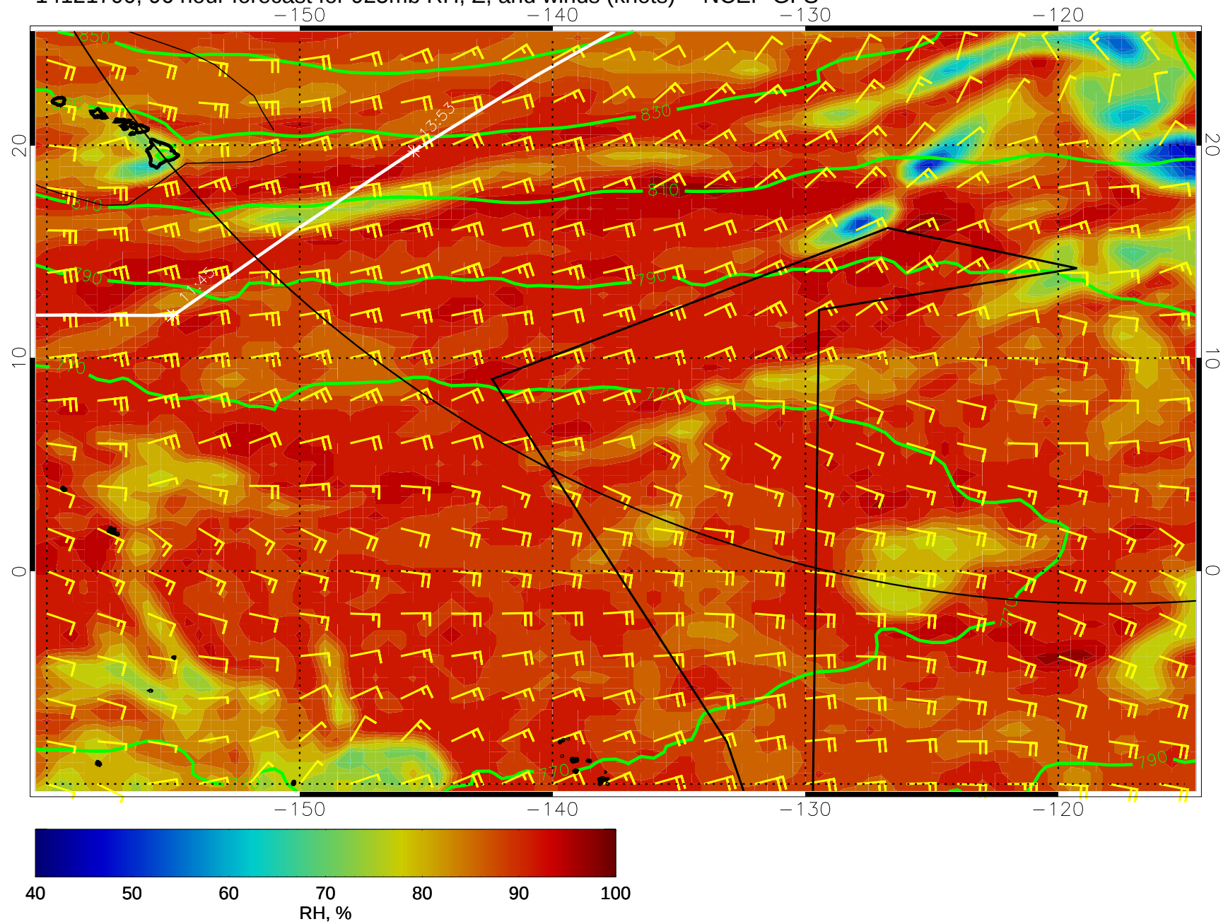
14121700, 96 hour forecast for 925mb RH, Z, and winds (knots) -- NCEP GFS
