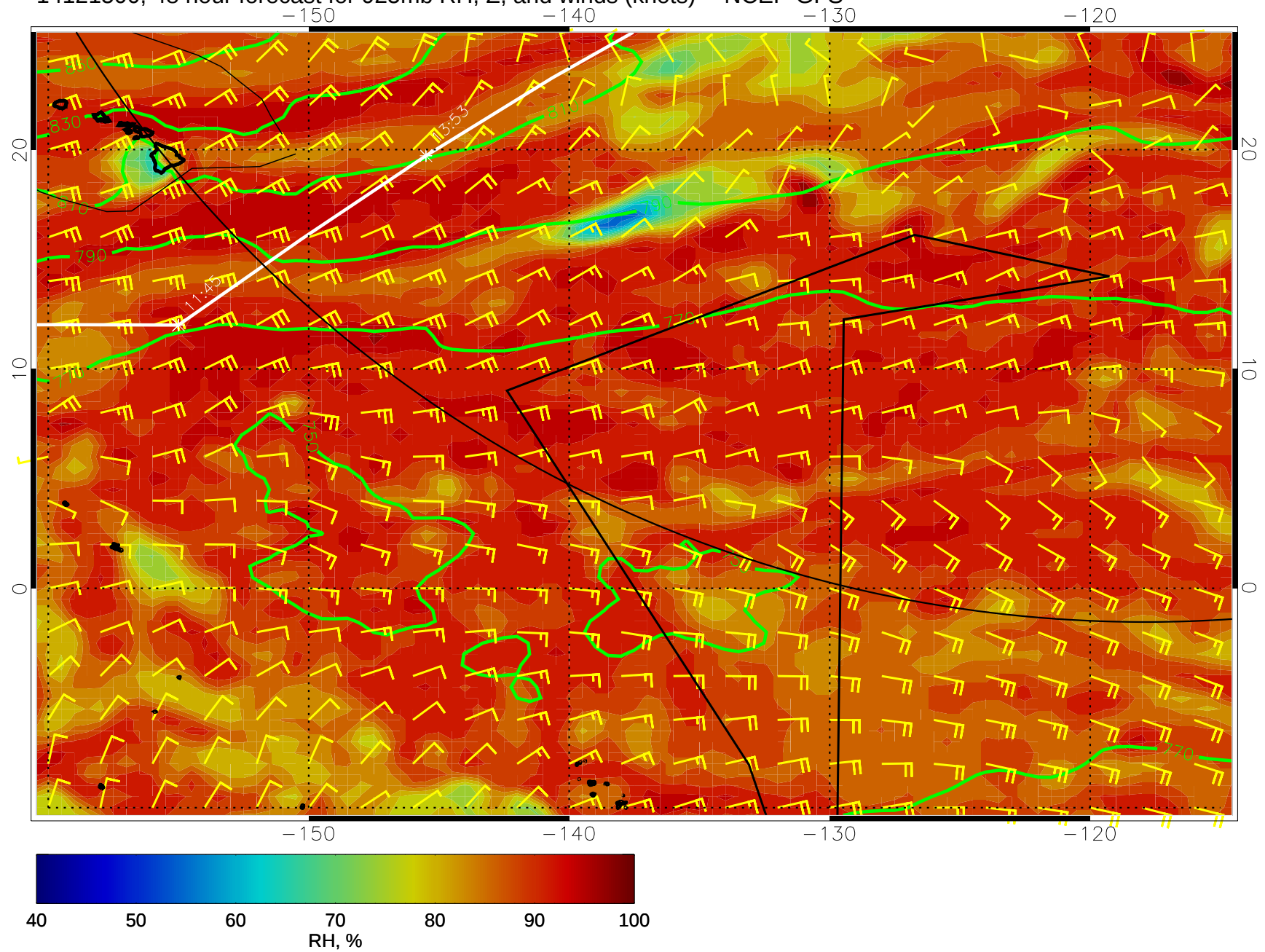
14121500, 48 hour forecast for 925mb RH, Z, and winds (knots) -- NCEP GFS
