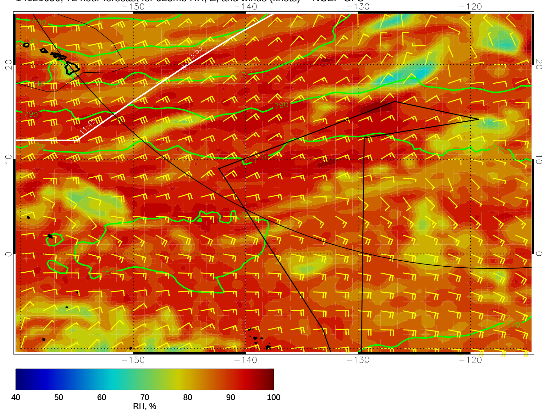
14121600, 72 hour forecast for 925mb RH, Z, and winds (knots) -- NCEP GFS
