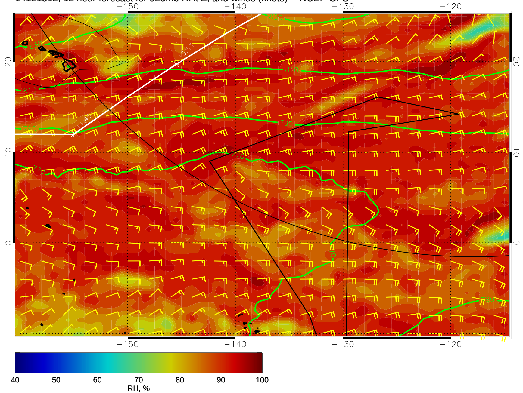
14121312, 12 hour forecast for 925mb RH, Z, and winds (knots) -- NCEP GFS
