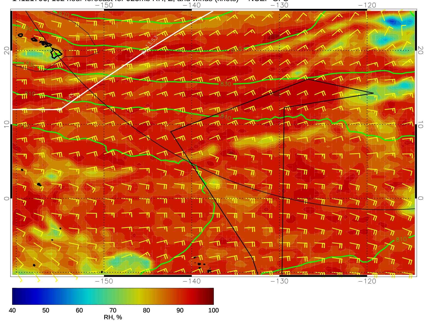
14121706, 102 hour forecast for 925mb RH, Z, and winds (knots) -- NCEP GFS
