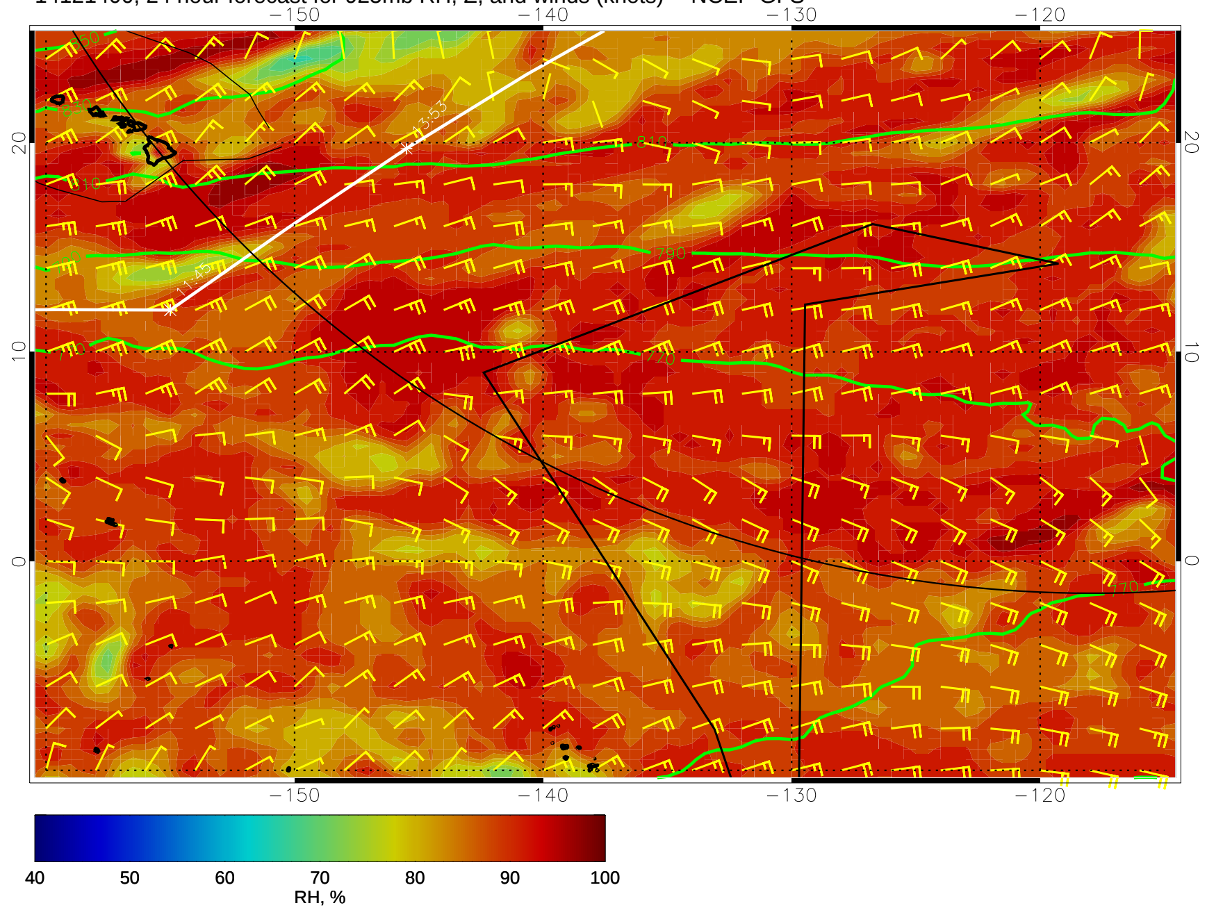
14121400, 24 hour forecast for 925mb RH, Z, and winds (knots) -- NCEP GFS
