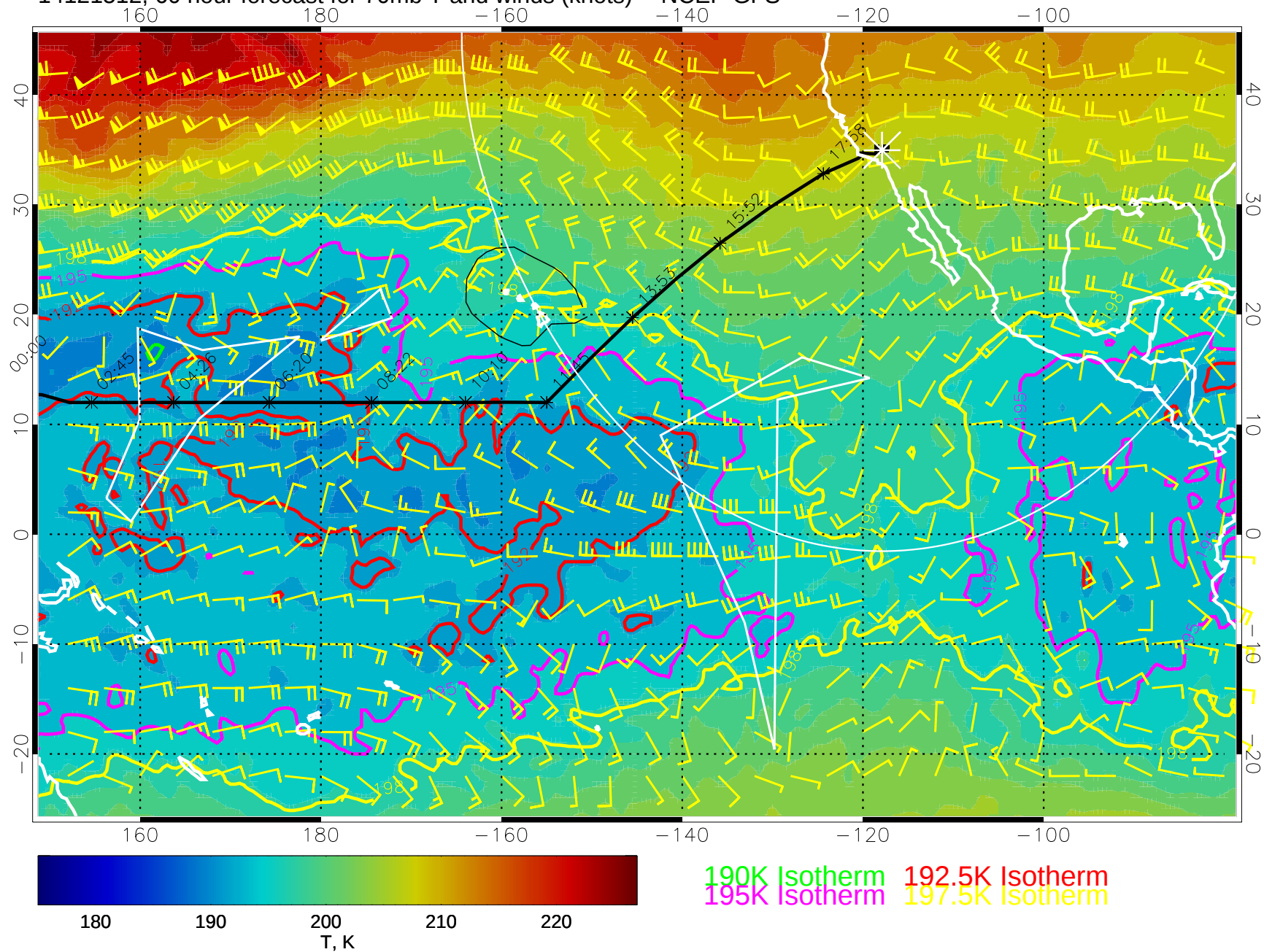
14121512, 60 hour forecast for 70mb T and winds (knots) -- NCEP GFS
