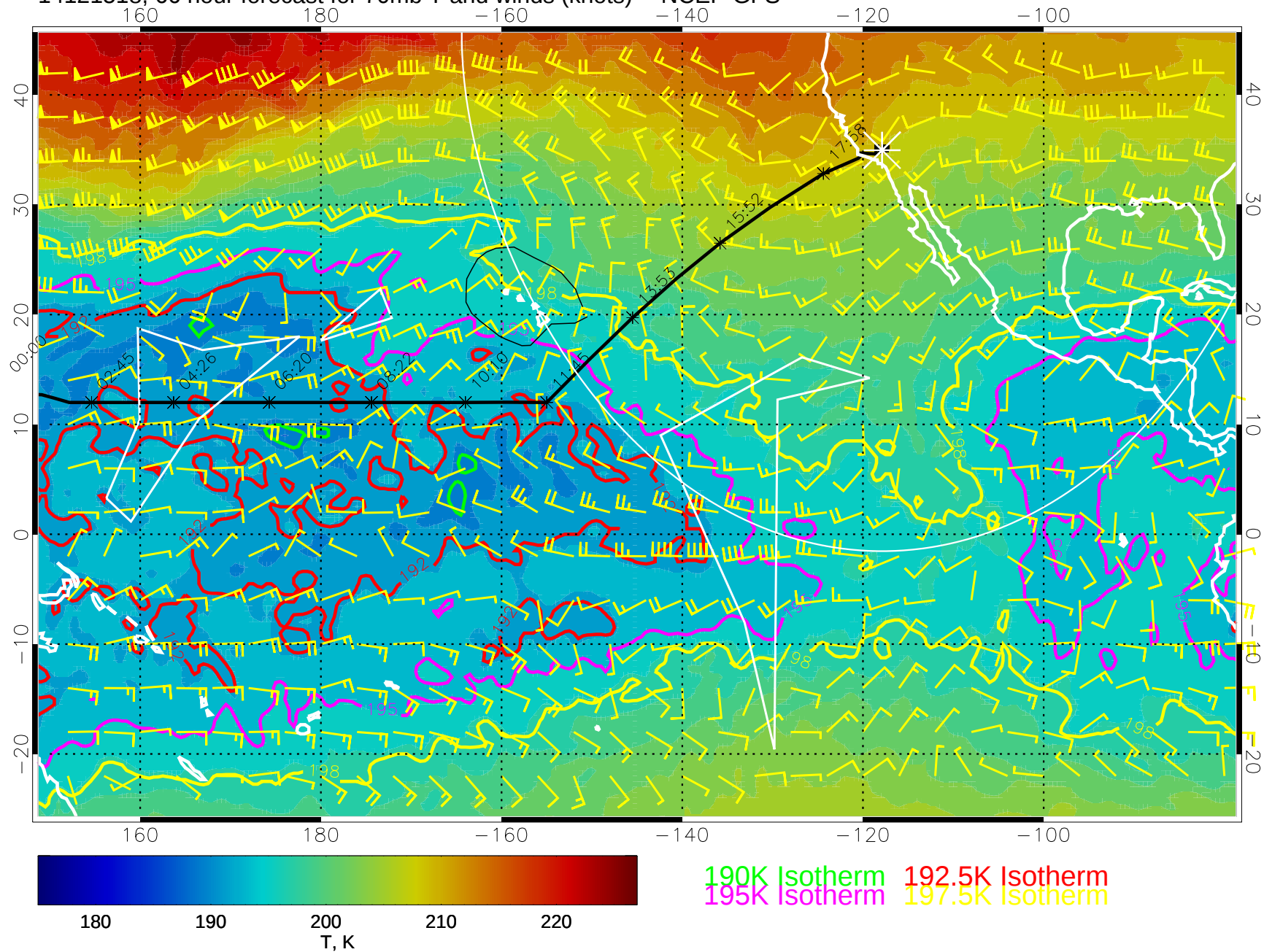
14121518, 66 hour forecast for 70mb T and winds (knots) -- NCEP GFS
