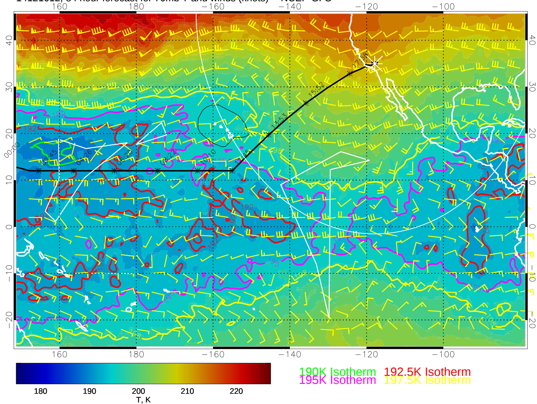
14121612, 84 hour forecast for 70mb T and winds (knots) -- NCEP GFS
