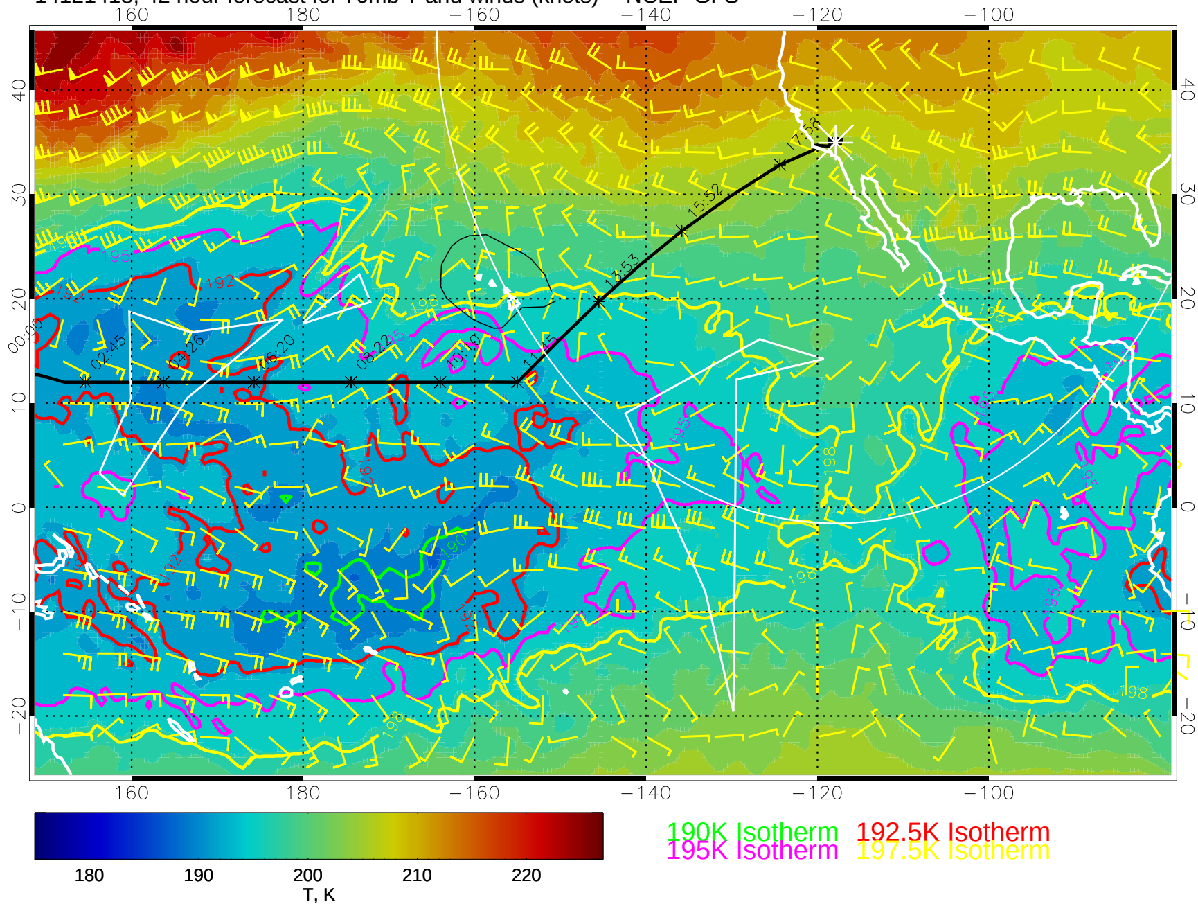
14121418, 42 hour forecast for 70mb T and winds (knots) -- NCEP GFS
