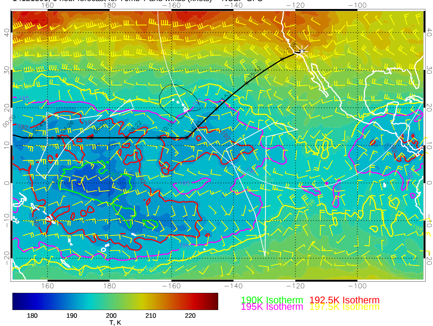
14121306, 6 hour forecast for 70mb T and winds (knots) -- NCEP GFS
