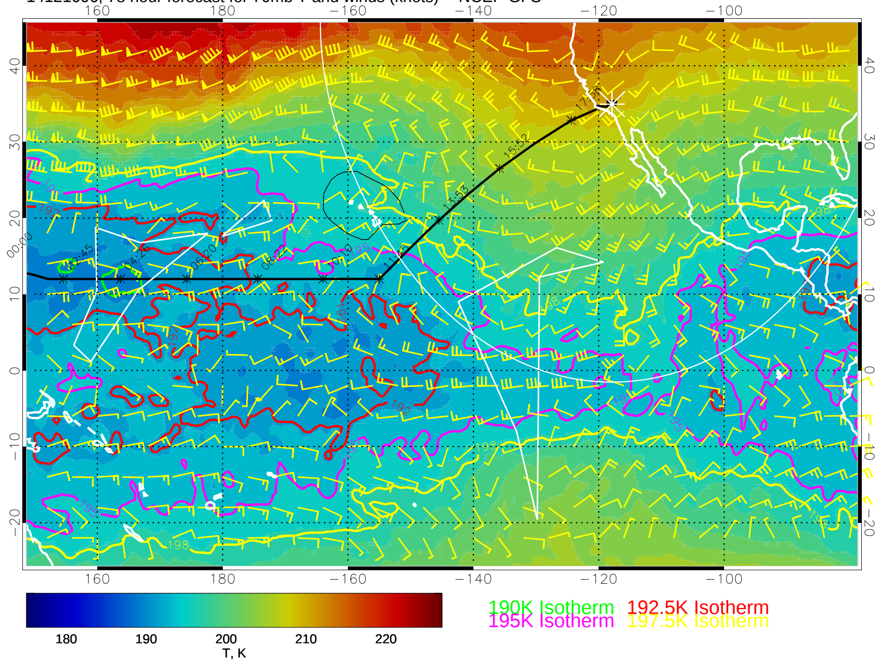
14121606, 78 hour forecast for 70mb T and winds (knots) -- NCEP GFS
