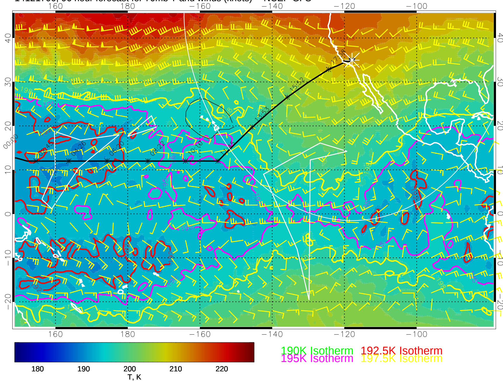
14121700, 96 hour forecast for 70mb T and winds (knots) -- NCEP GFS
