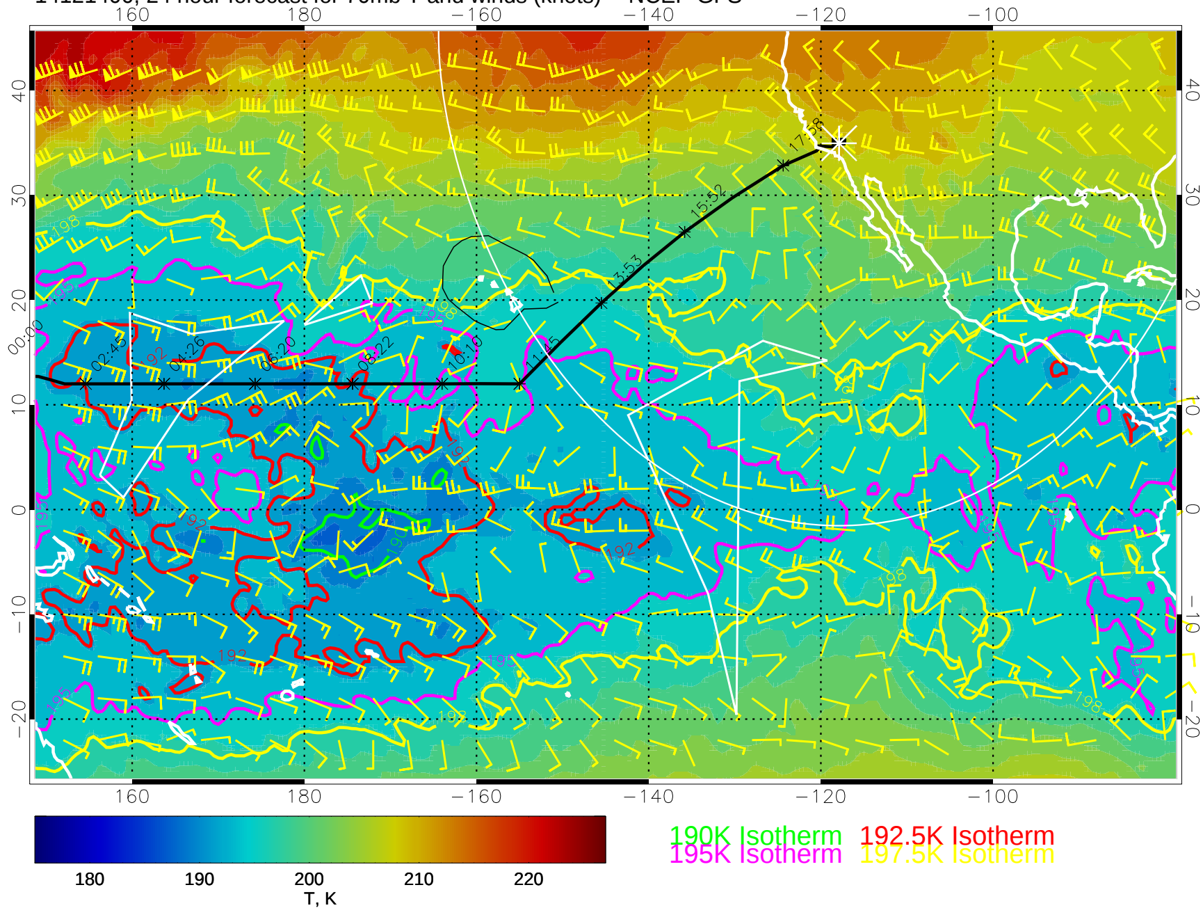
14121400, 24 hour forecast for 70mb T and winds (knots) -- NCEP GFS
