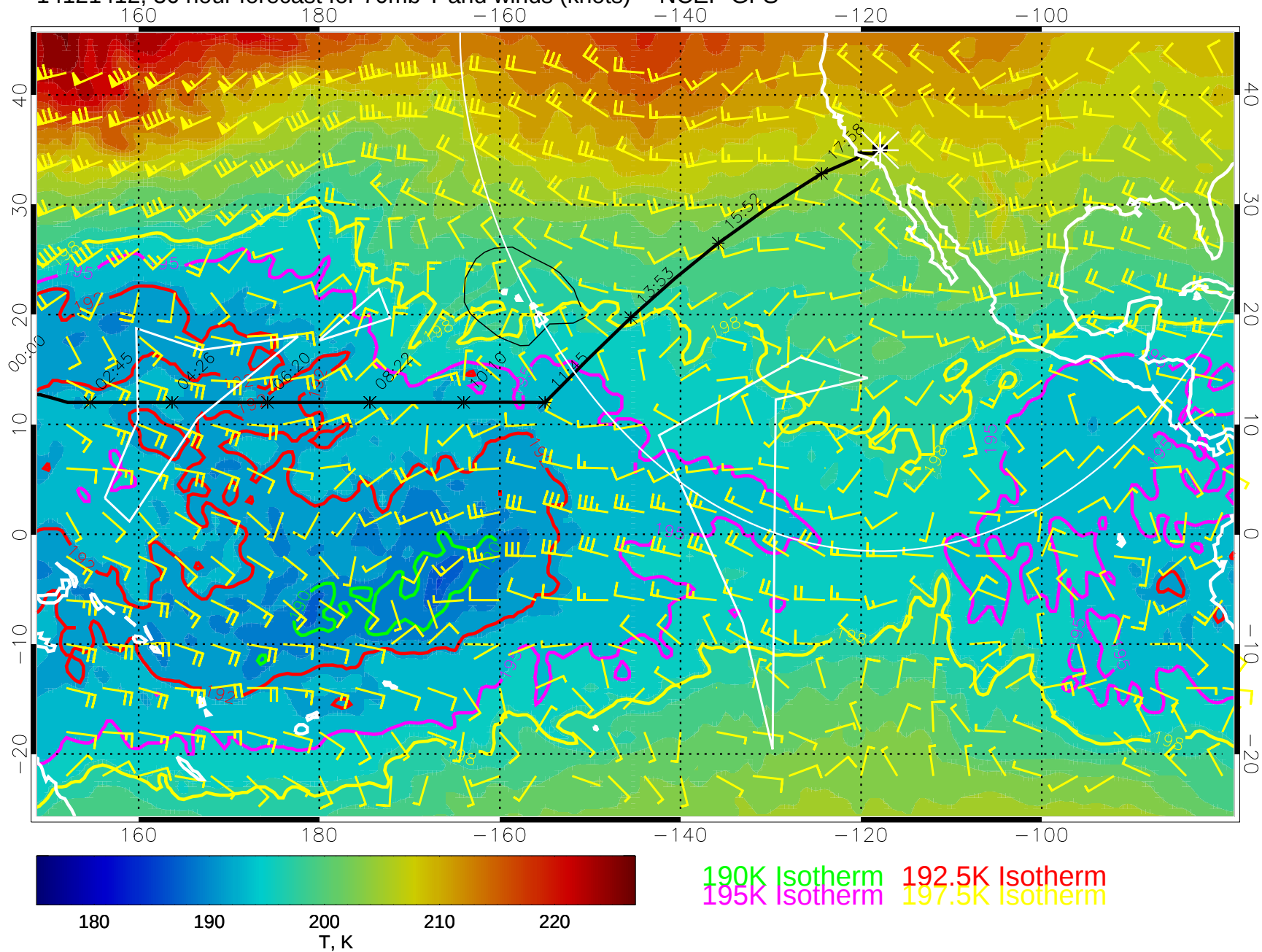
14121412, 36 hour forecast for 70mb T and winds (knots) -- NCEP GFS
