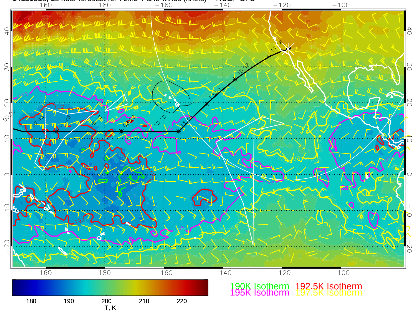
14121318, 18 hour forecast for 70mb T and winds (knots) -- NCEP GFS
