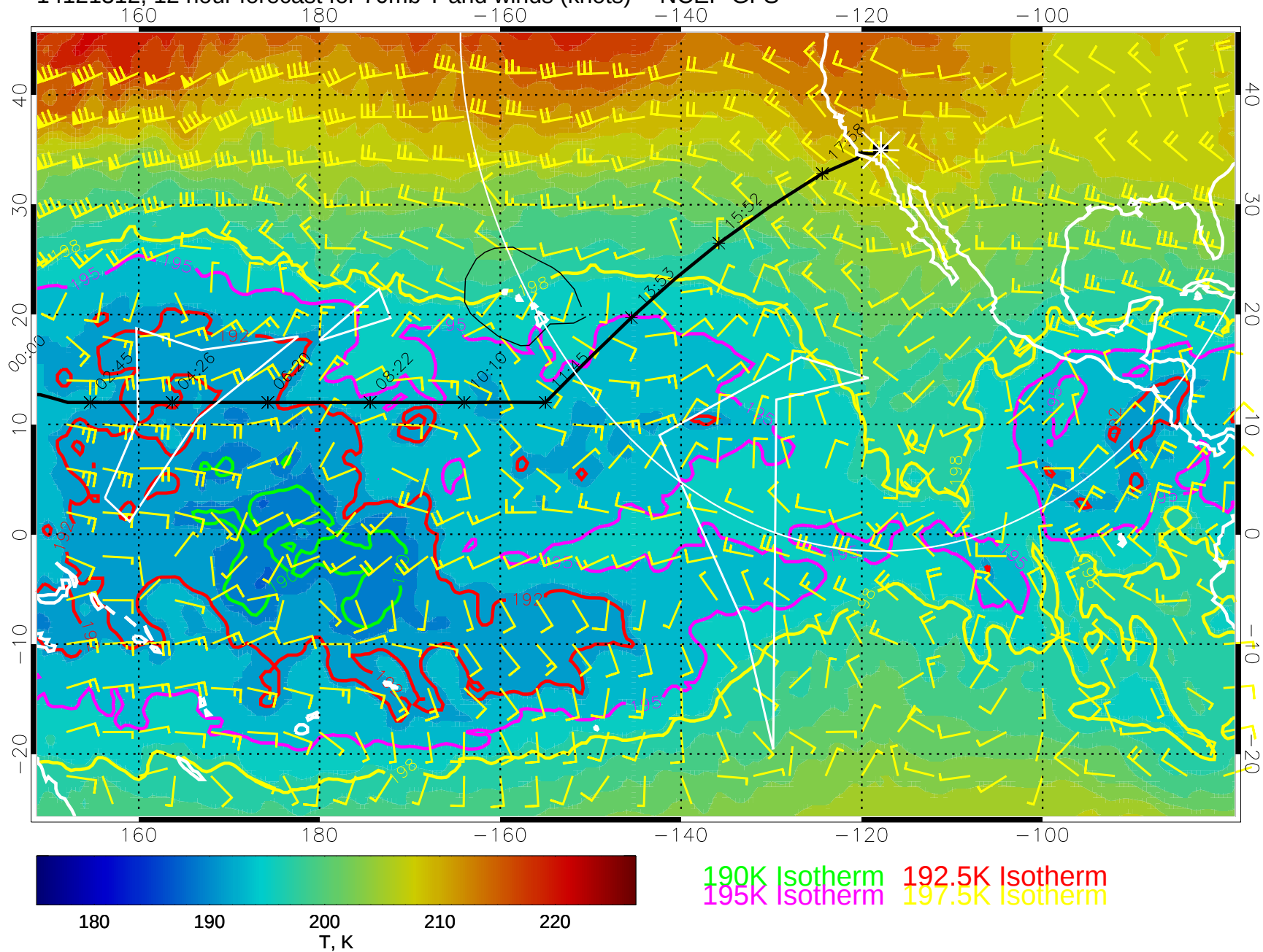
14121312, 12 hour forecast for 70mb T and winds (knots) -- NCEP GFS
