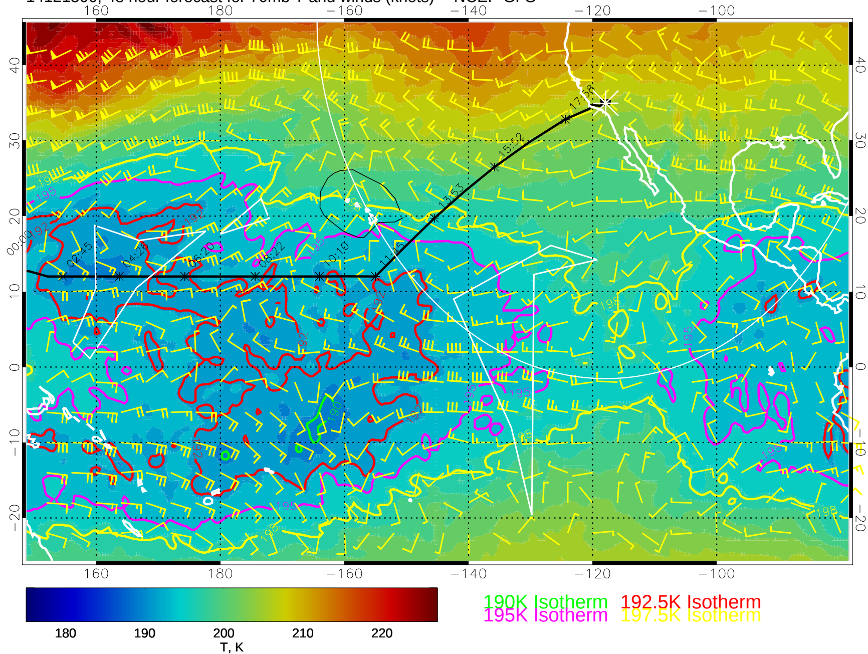
14121500, 48 hour forecast for 70mb T and winds (knots) -- NCEP GFS
