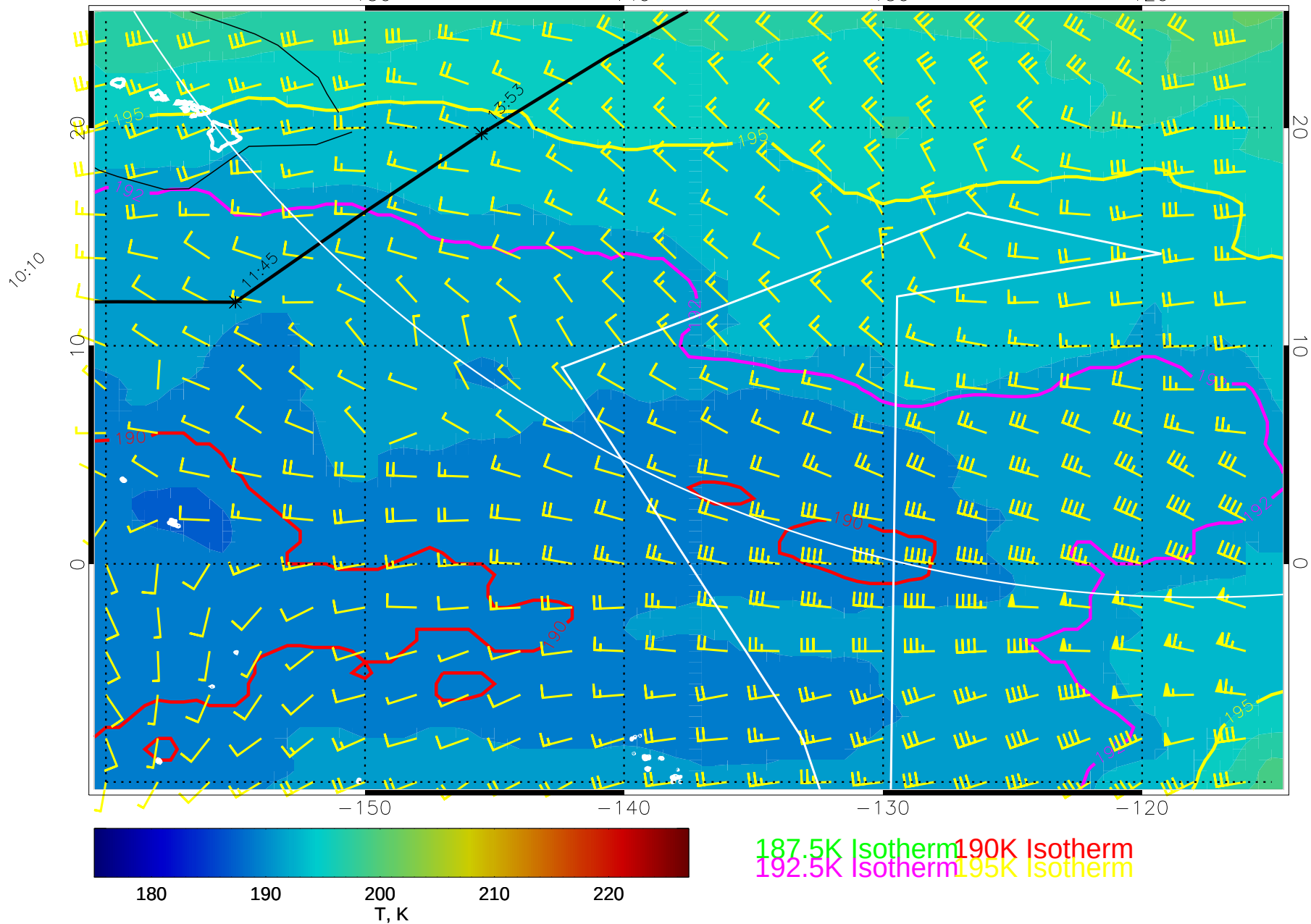
14121312, 12 hour forecast for 100mb T and winds (knots) -- NCEP GFS
