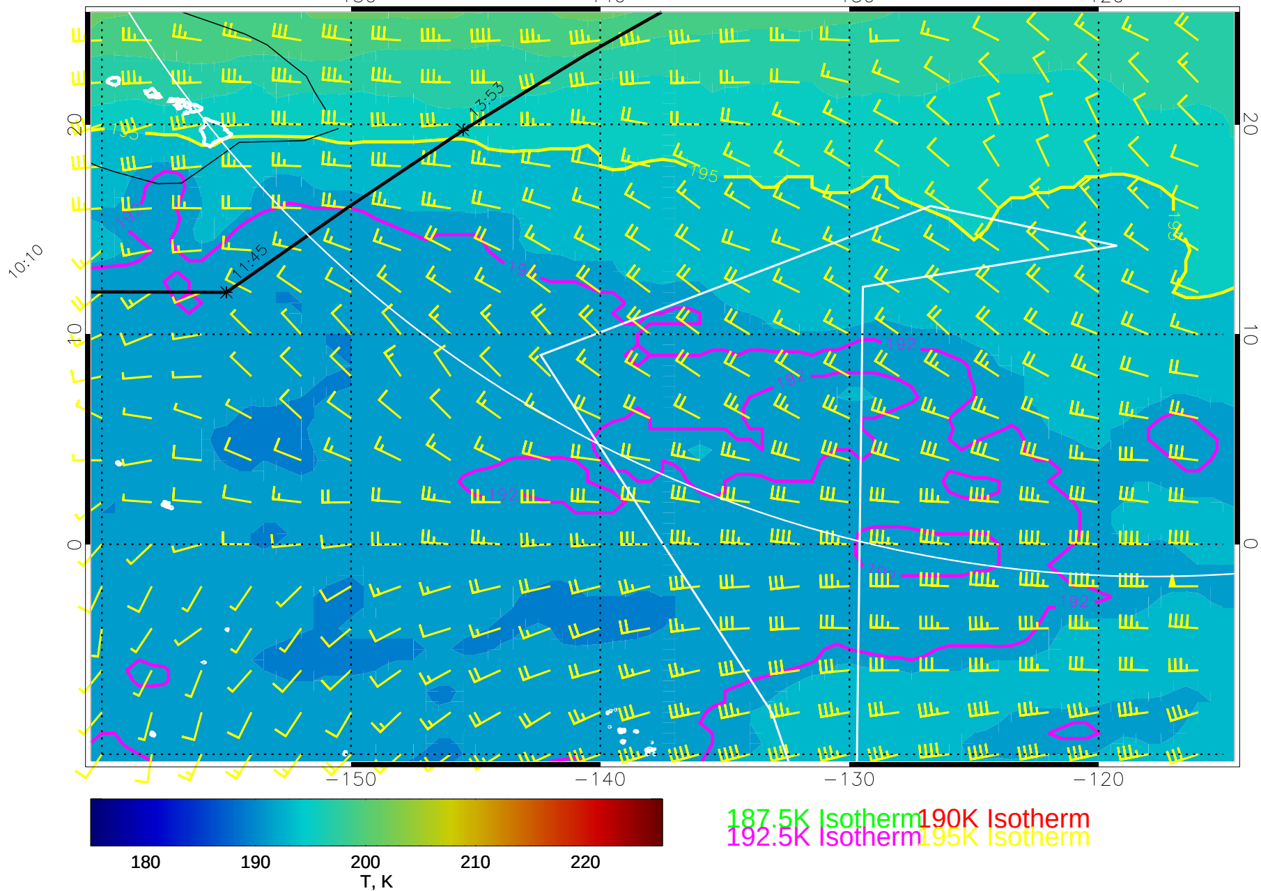
14121412, 36 hour forecast for 100mb T and winds (knots) -- NCEP GFS
