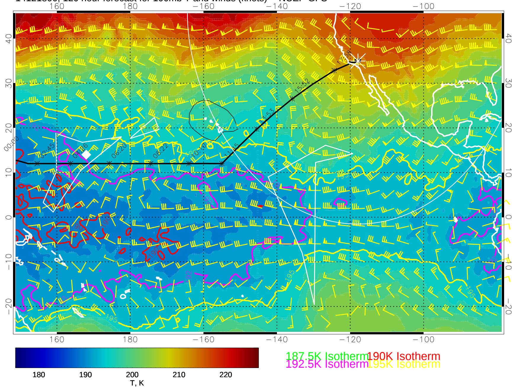
14121800, 120 hour forecast for 100mb T and winds (knots) -- NCEP GFS
