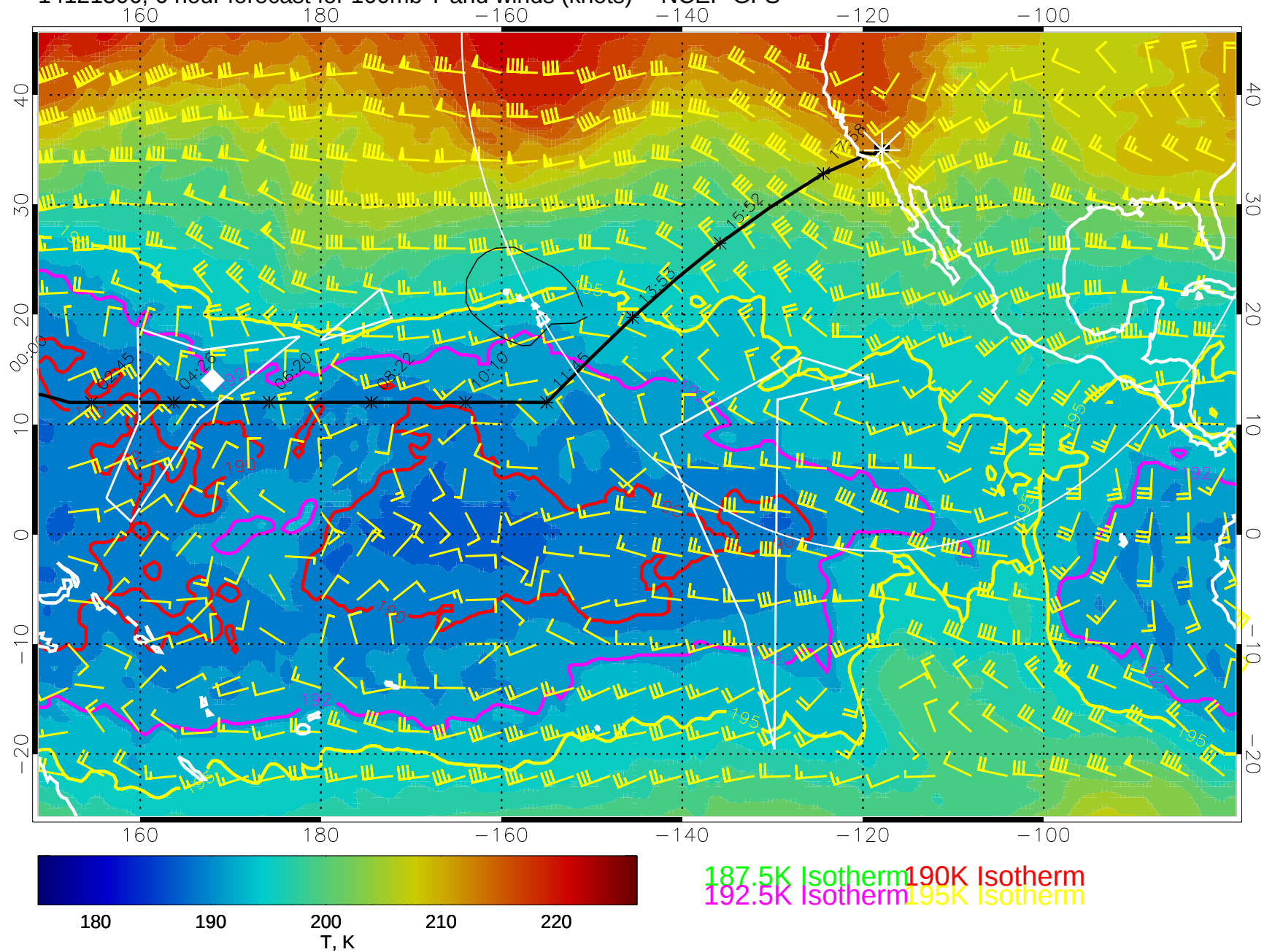
14121306, 6 hour forecast for 100mb T and winds (knots) -- NCEP GFS
