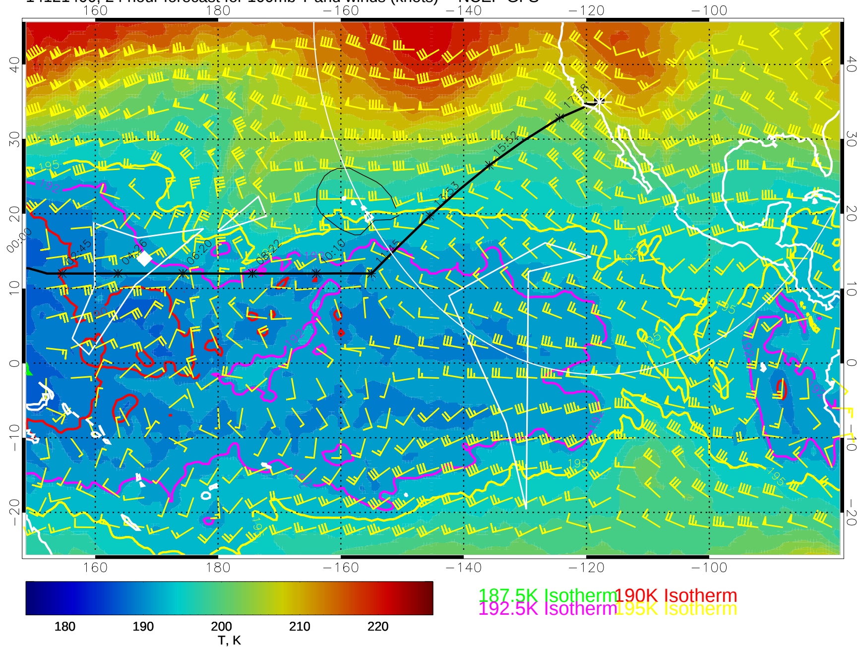
14121400, 24 hour forecast for 100mb T and winds (knots) -- NCEP GFS
