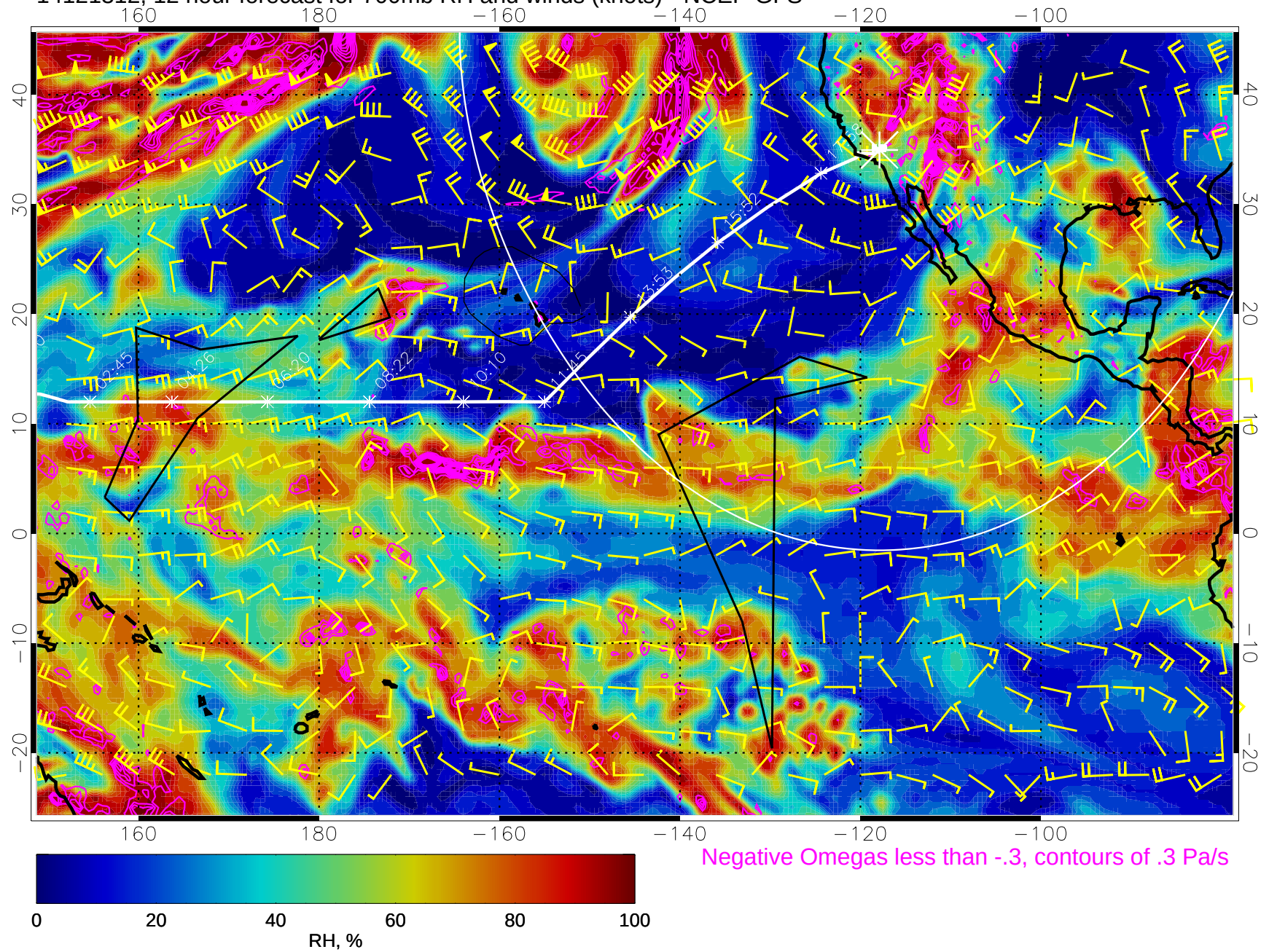
14121312, 12 hour forecast for 700mb RH and winds (knots) - NCEP GFS
