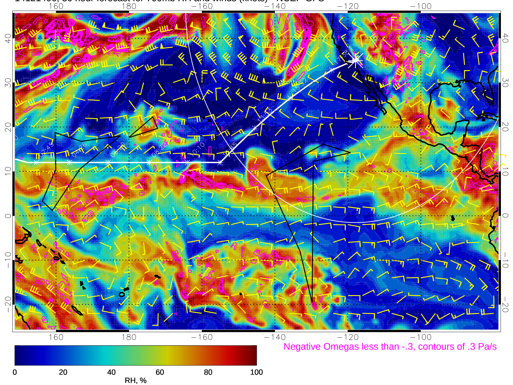
14121406, 30 hour forecast for 700mb RH and winds (knots) - NCEP GFS
