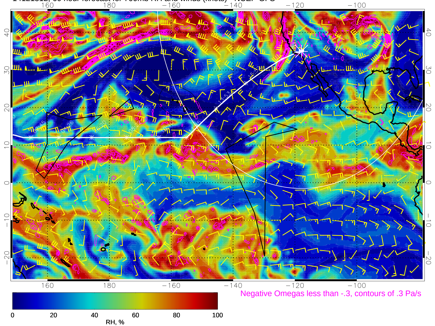
14121512, 60 hour forecast for 700mb RH and winds (knots) - NCEP GFS
