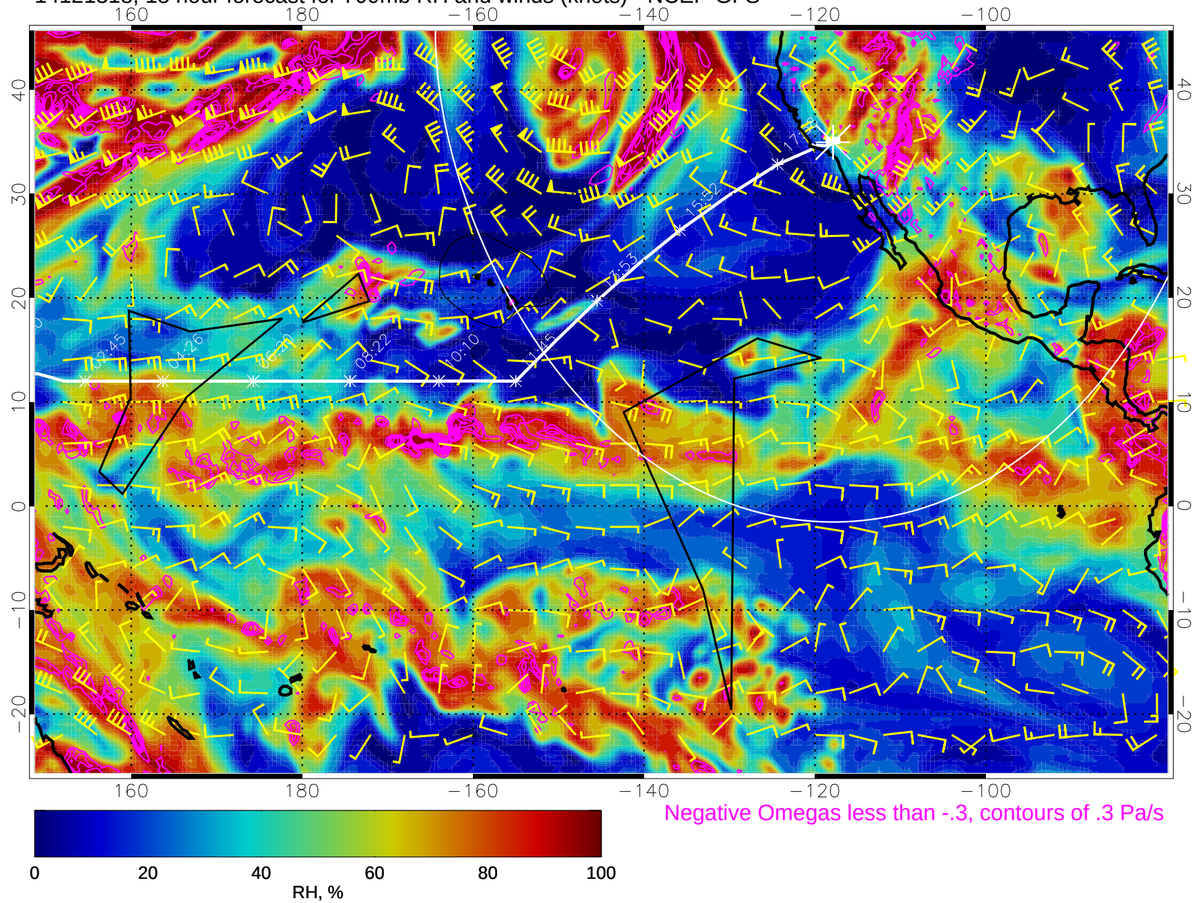
14121318, 18 hour forecast for 700mb RH and winds (knots) - NCEP GFS
