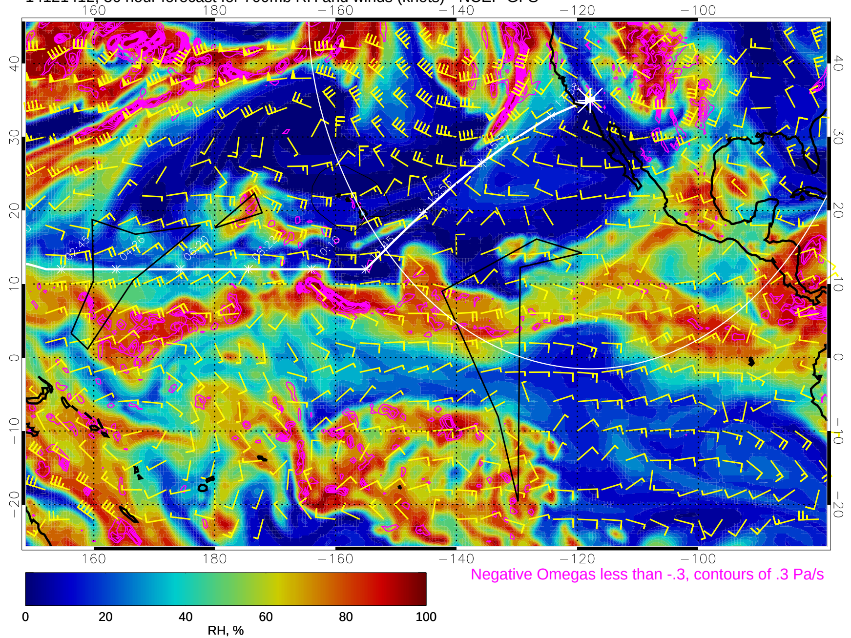
14121412, 36 hour forecast for 700mb RH and winds (knots) - NCEP GFS
