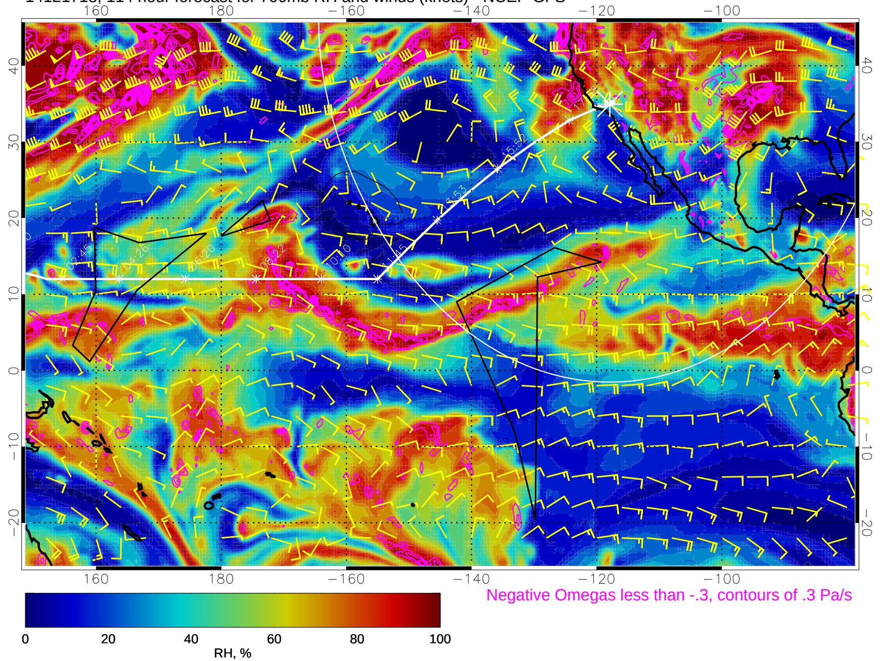
14121718, 114 hour forecast for 700mb RH and winds (knots) - NCEP GFS
