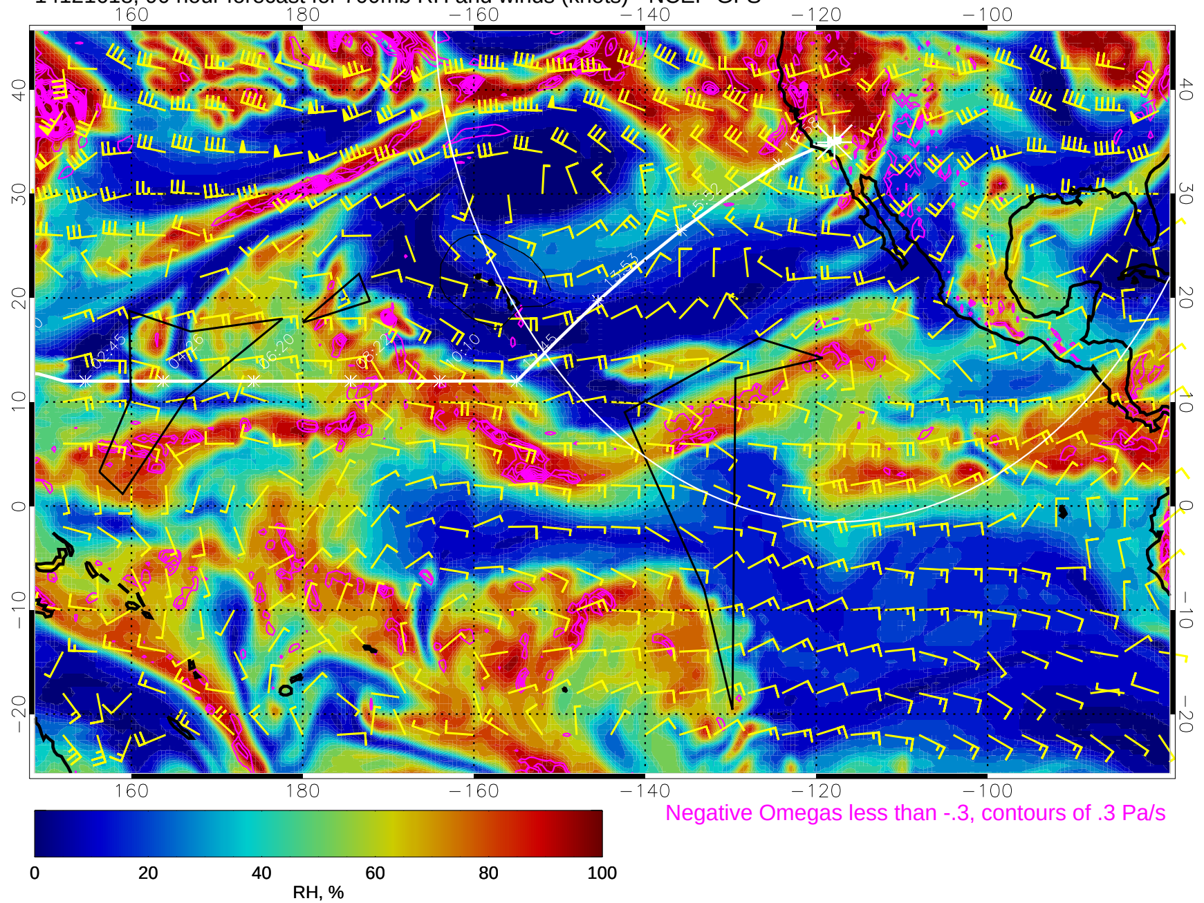
14121618, 90 hour forecast for 700mb RH and winds (knots) - NCEP GFS
