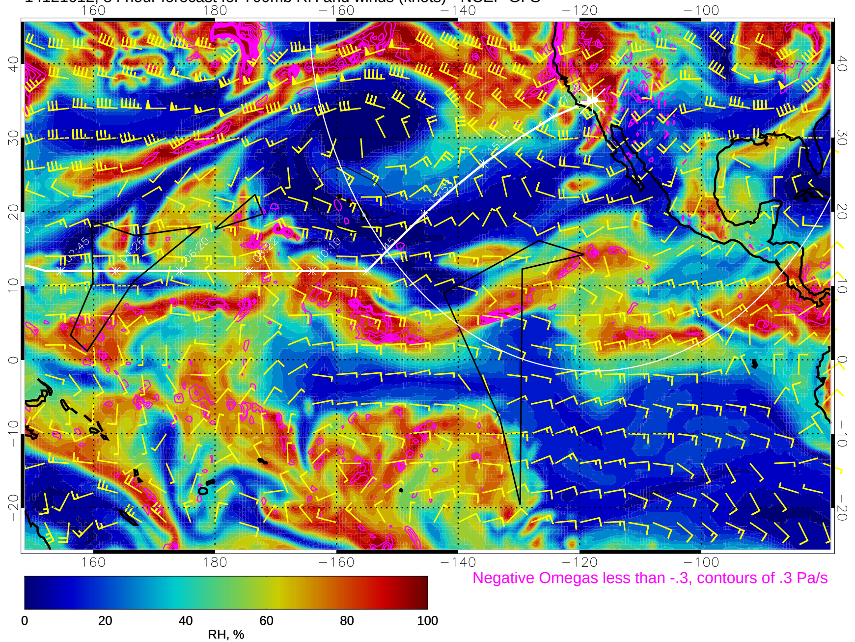
14121612, 84 hour forecast for 700mb RH and winds (knots) - NCEP GFS
