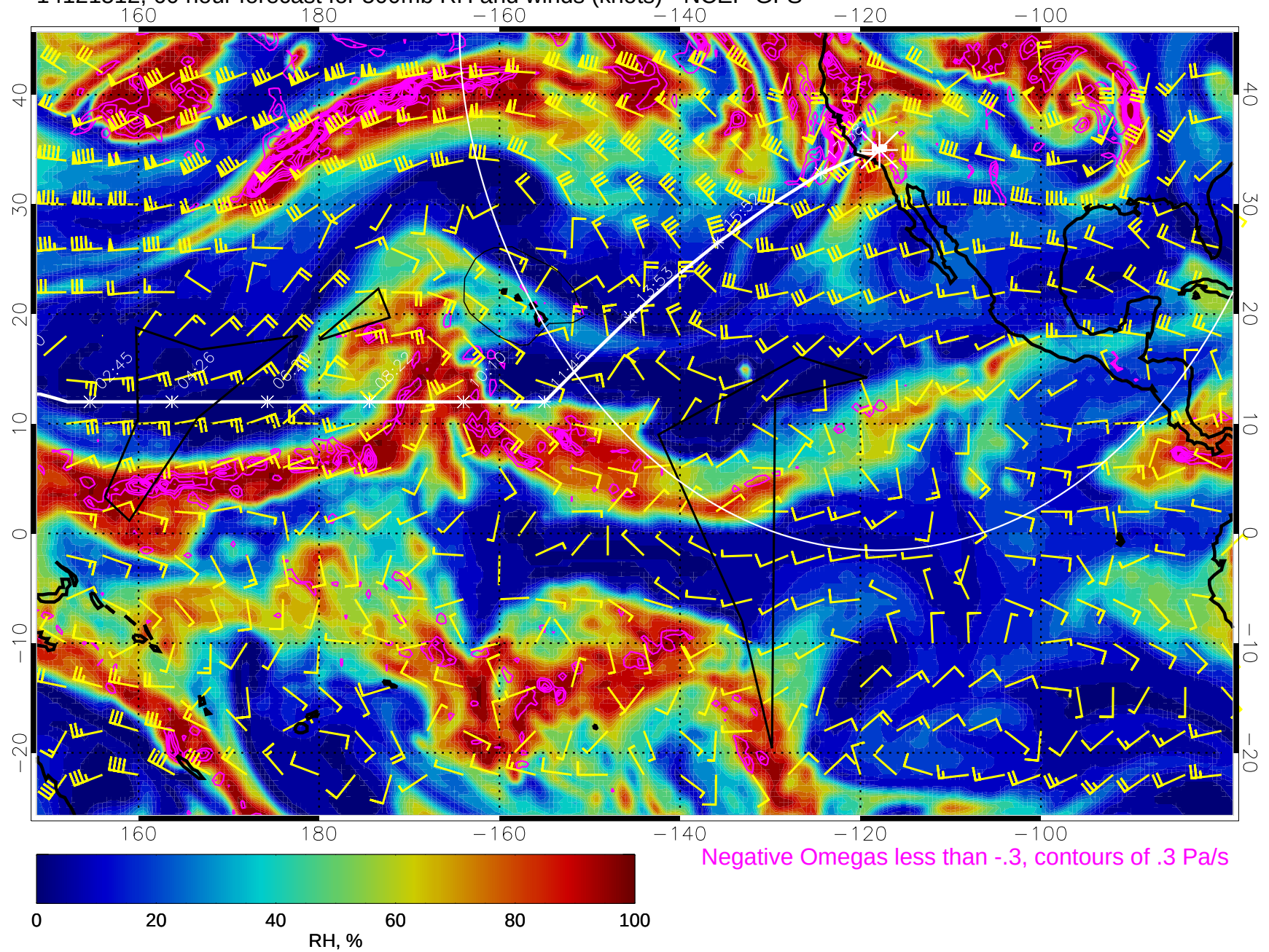
14121512, 60 hour forecast for 500mb RH and winds (knots) - NCEP GFS
