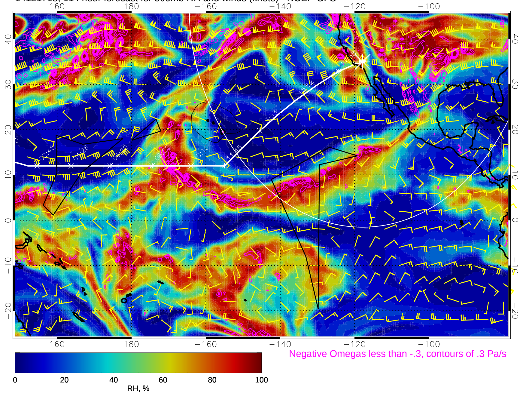
14121718, 114 hour forecast for 500mb RH and winds (knots) - NCEP GFS
