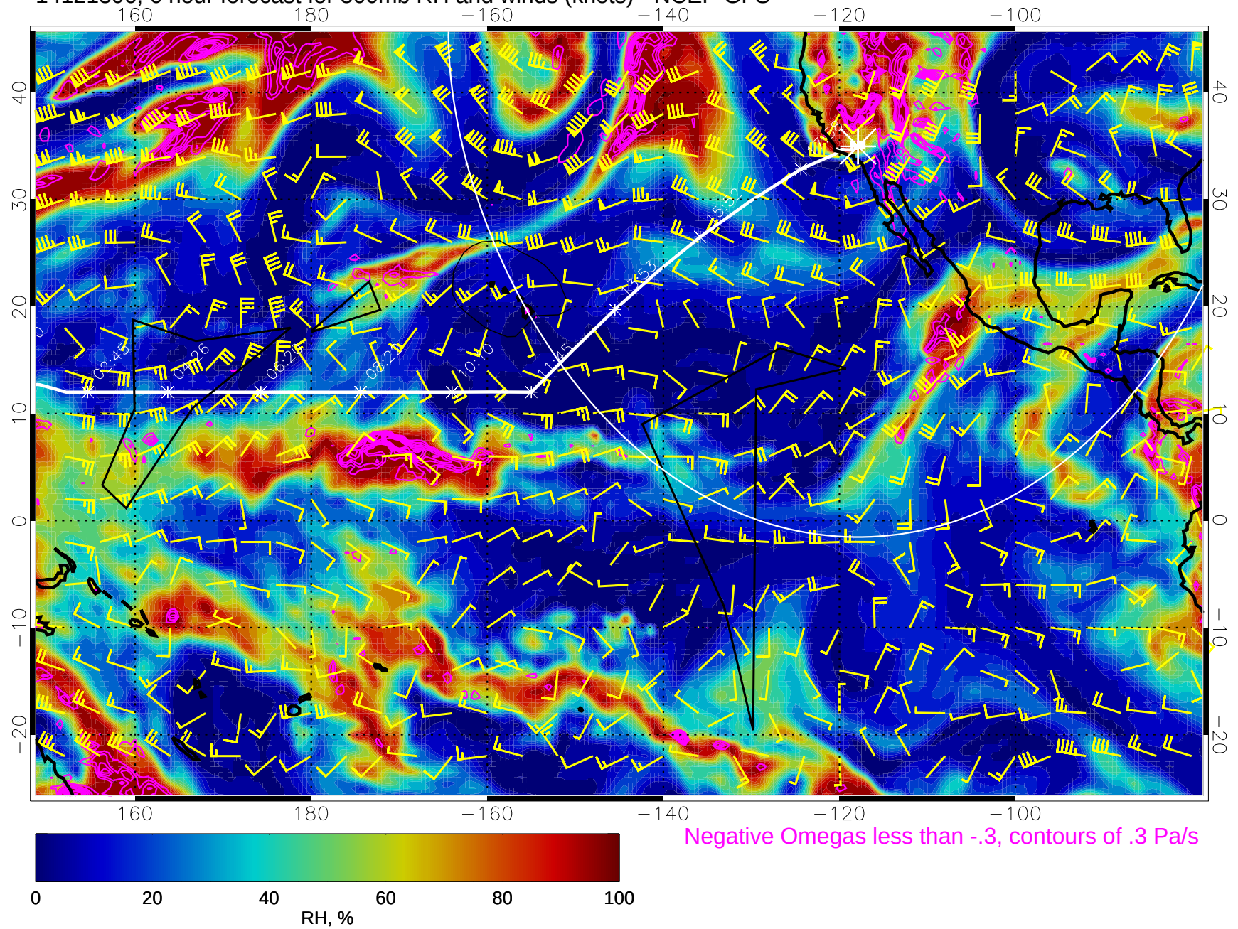
14121306, 6 hour forecast for 500mb RH and winds (knots) - NCEP GFS
