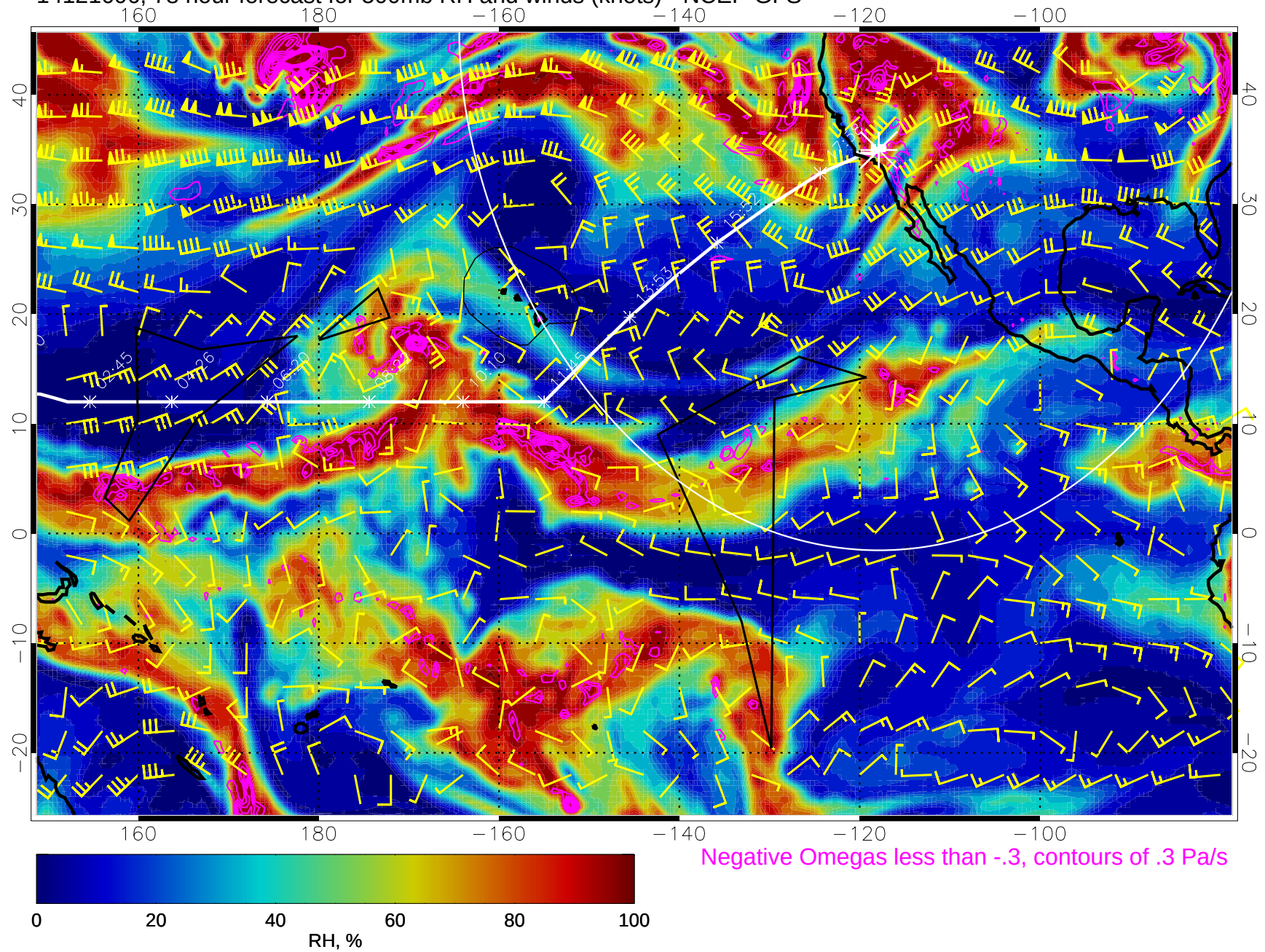
14121606, 78 hour forecast for 500mb RH and winds (knots) - NCEP GFS
