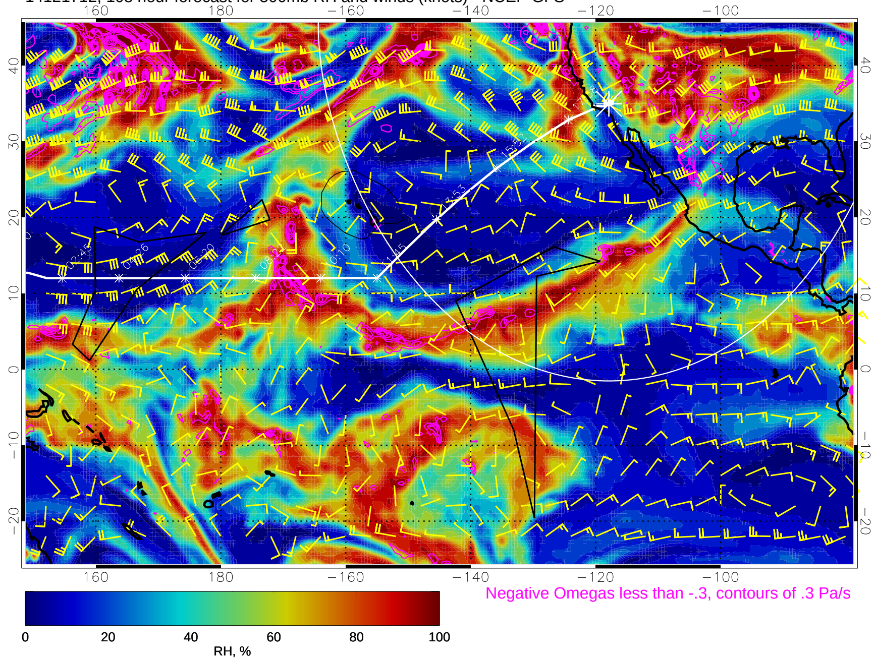
14121712, 108 hour forecast for 500mb RH and winds (knots) - NCEP GFS
