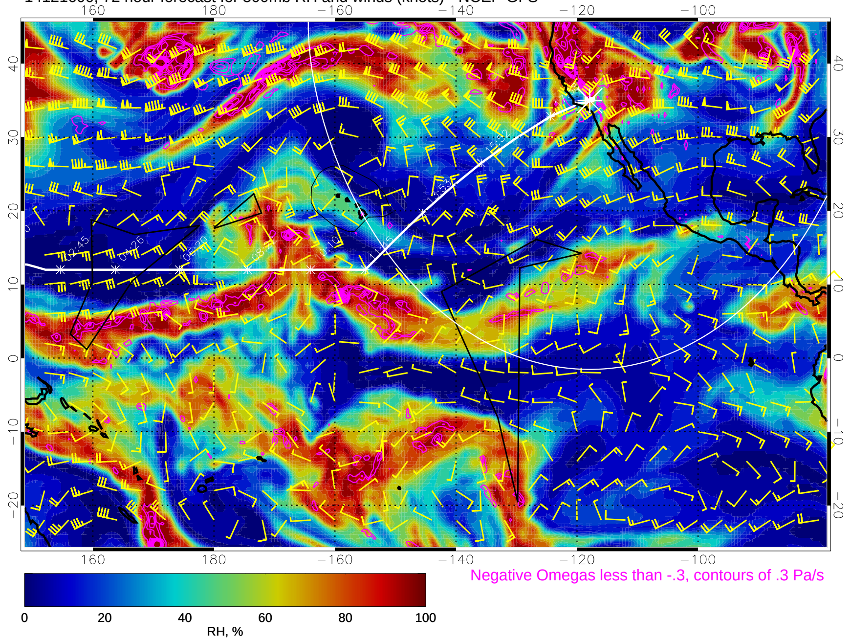
14121600, 72 hour forecast for 500mb RH and winds (knots) - NCEP GFS
