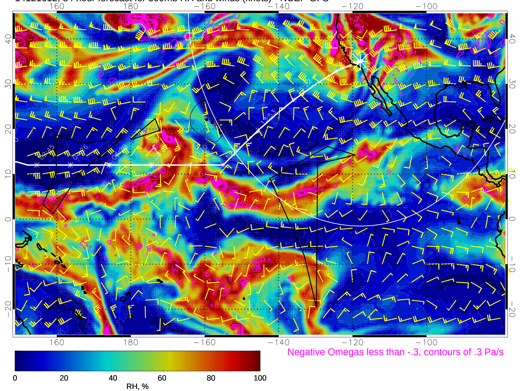
14121612, 84 hour forecast for 500mb RH and winds (knots) - NCEP GFS
