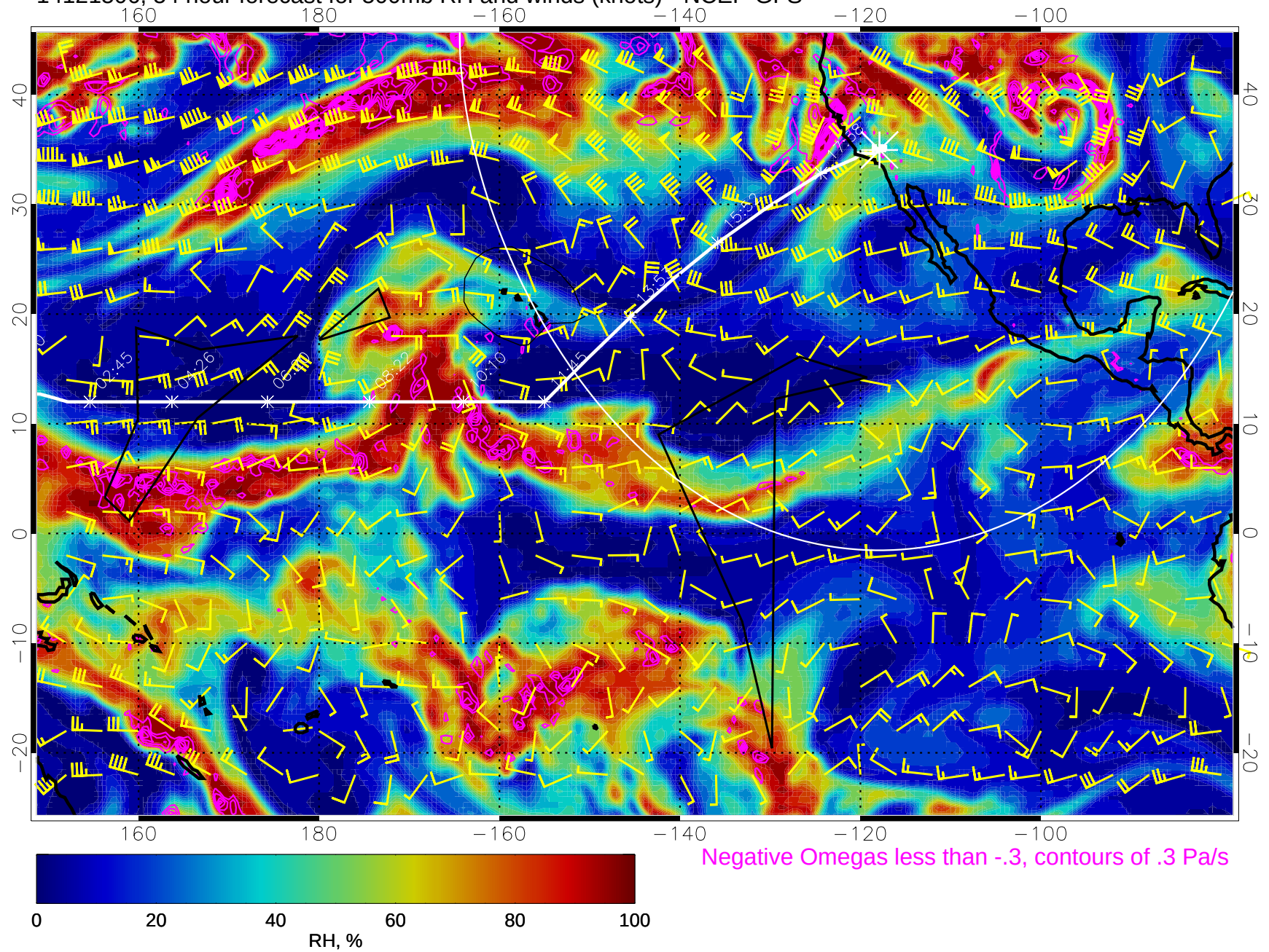
14121506, 54 hour forecast for 500mb RH and winds (knots) - NCEP GFS
