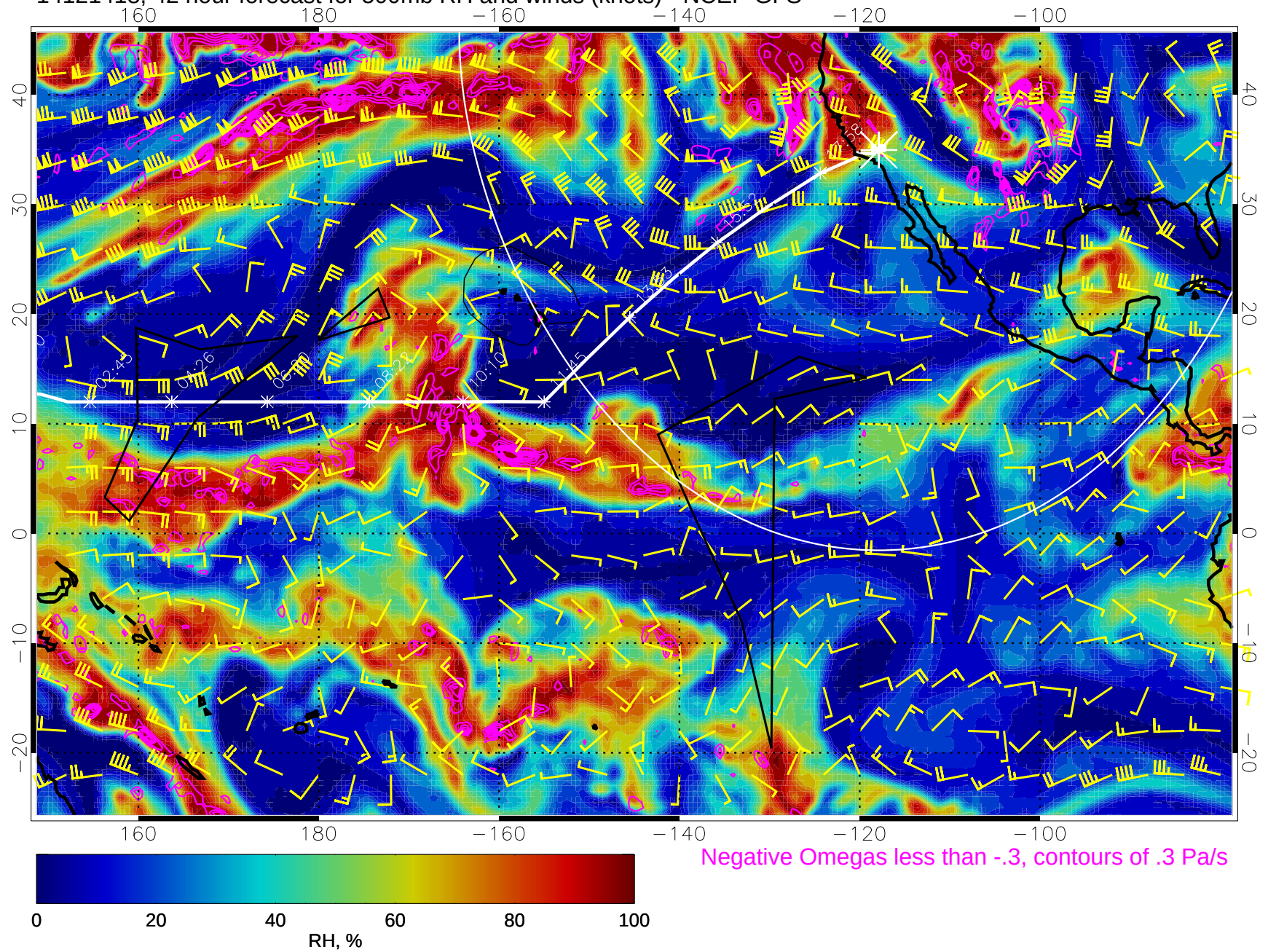
14121418, 42 hour forecast for 500mb RH and winds (knots) - NCEP GFS
