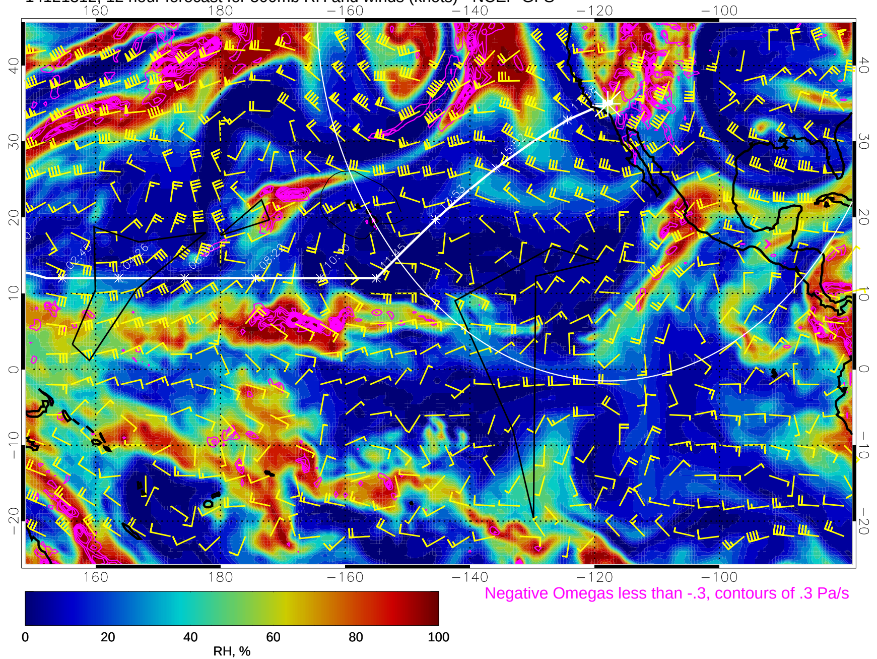
14121312, 12 hour forecast for 500mb RH and winds (knots) - NCEP GFS
