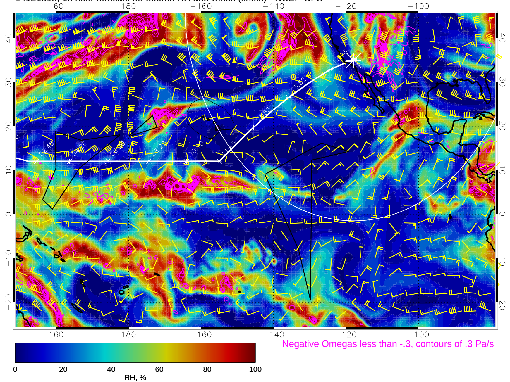
14121318, 18 hour forecast for 500mb RH and winds (knots) - NCEP GFS
