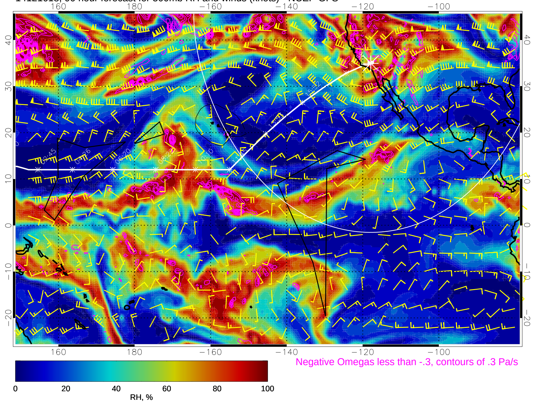
14121618, 90 hour forecast for 500mb RH and winds (knots) - NCEP GFS
