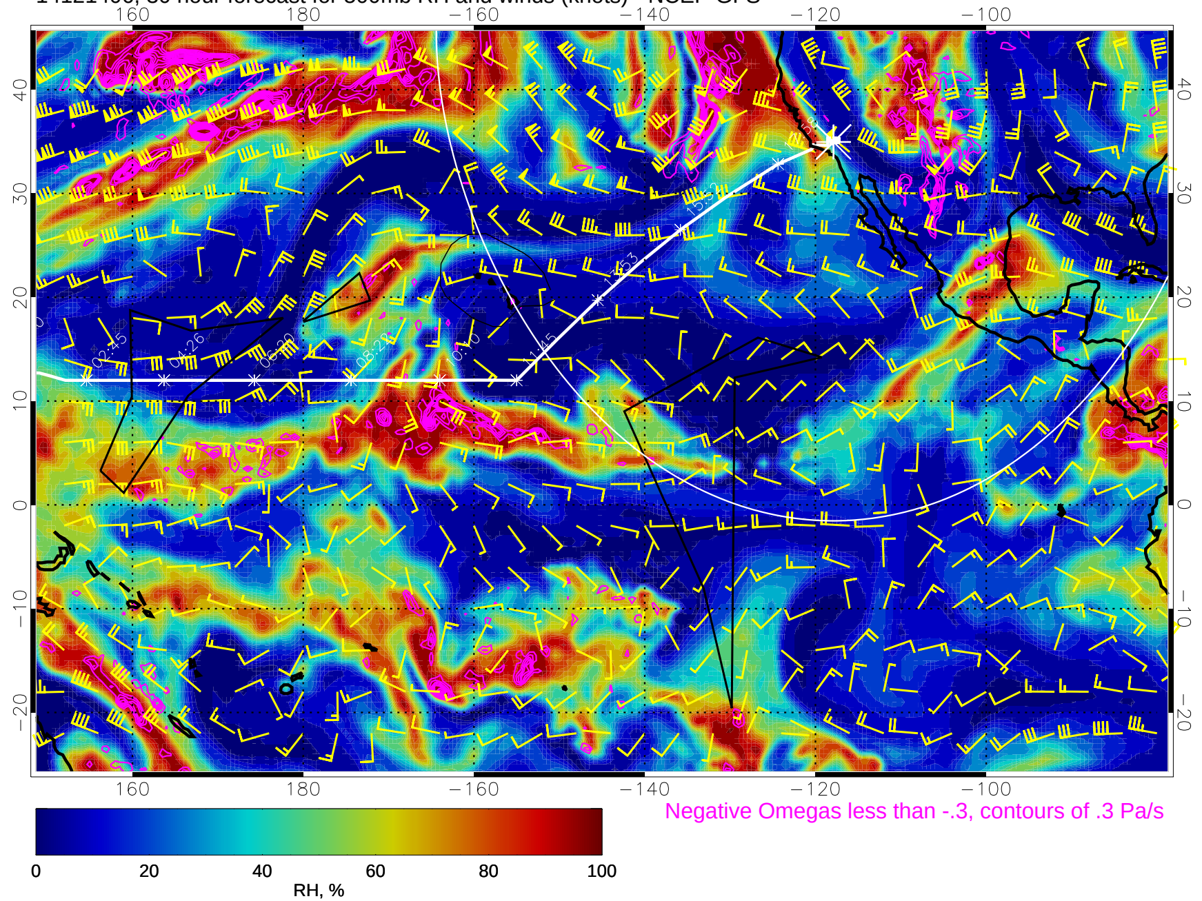
14121406, 30 hour forecast for 500mb RH and winds (knots) - NCEP GFS
